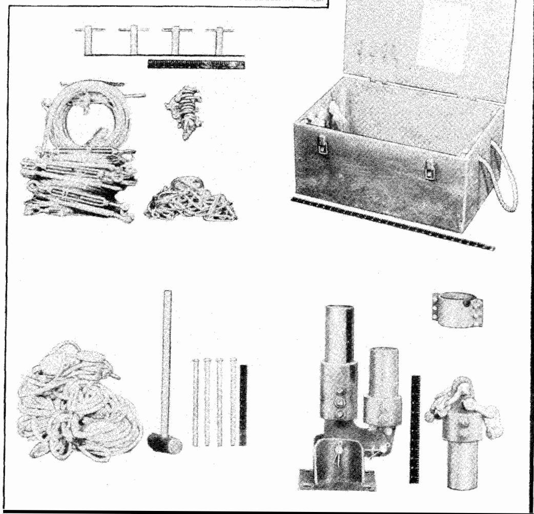
Figure 45 - Stay Box for Antenna Mast MA-7-A, Unpacked; Part of Radio Set SCR-624-T1
