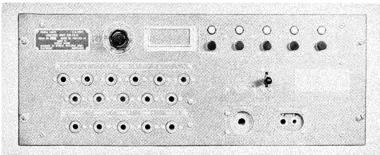
Figure 54 - Control Unit RM-23-A - Front View
