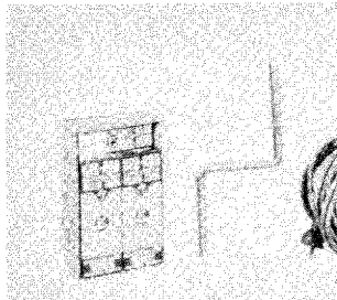
Figure 91 - Chest CH-172-A Unpacked - With Rectifier RA-62 - Spare Tubes, Fuses, Hand Crank, and 25 Foot AC Line Cord; Part of Radio Set SCR-624-A
