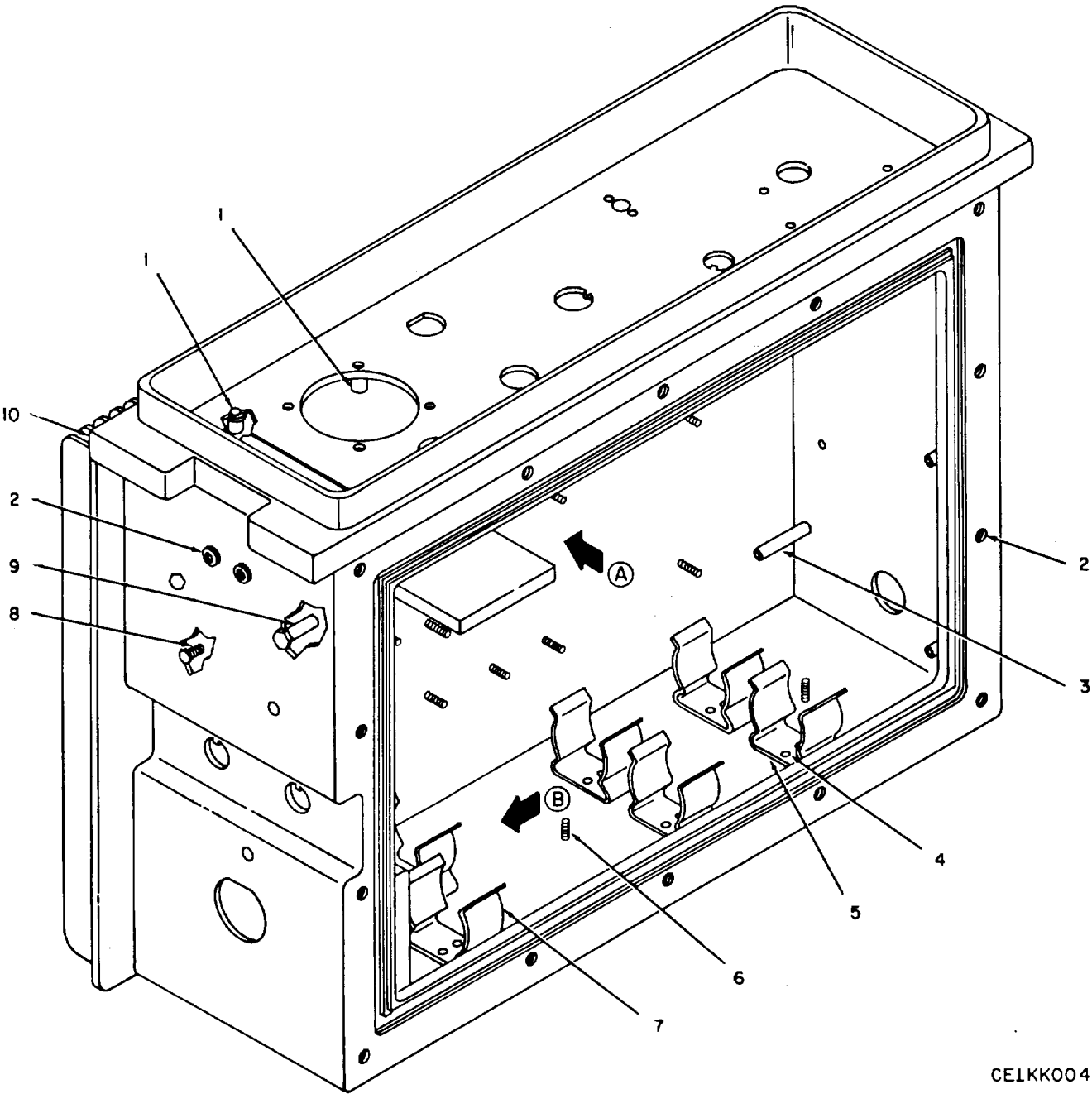
Figure 2. Electrical Equipment Chassis Assembly (Sheet 1 of 2)
