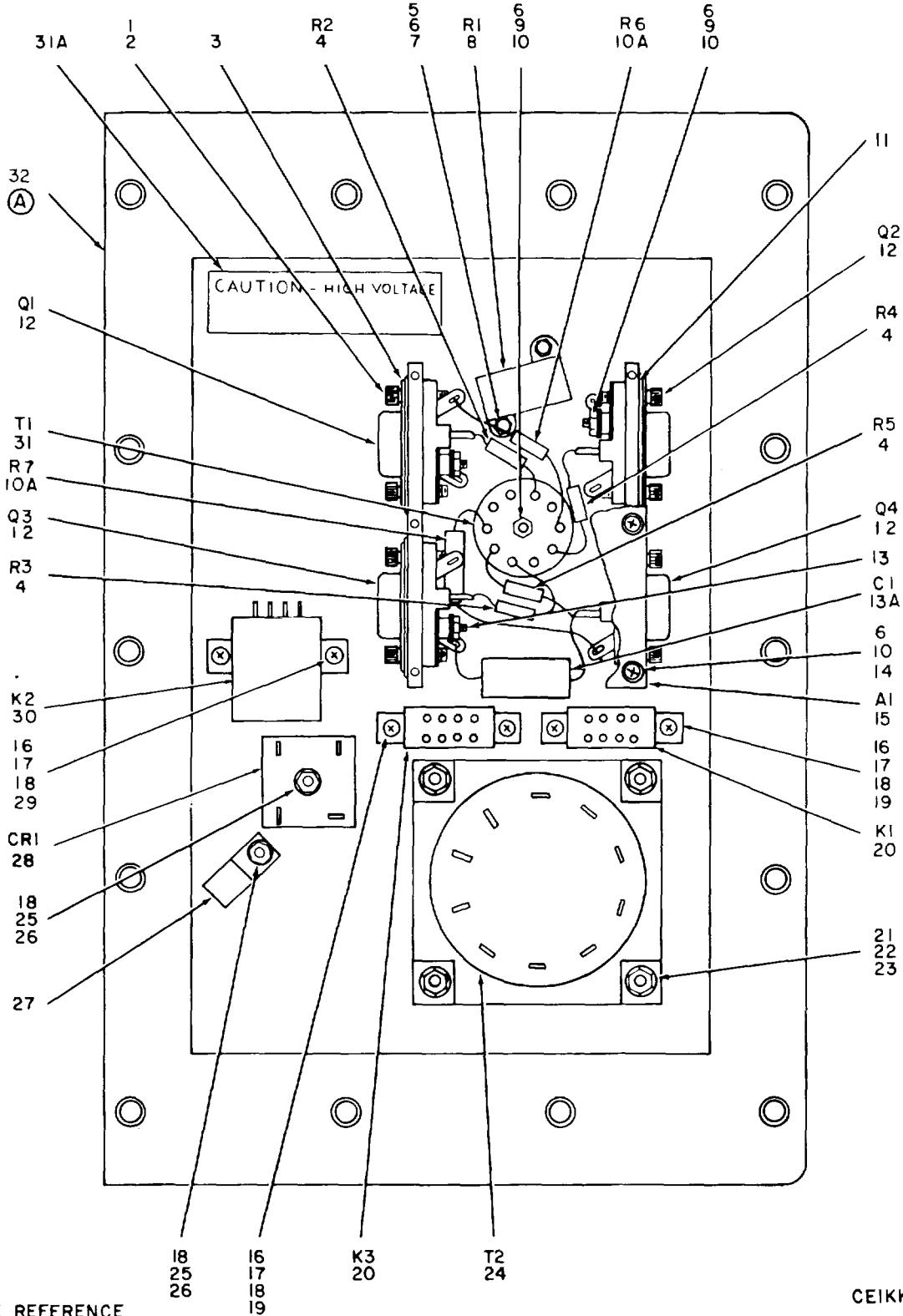
Figure 3. Cover Assembly (A1) (Sheet 1 of 2)
