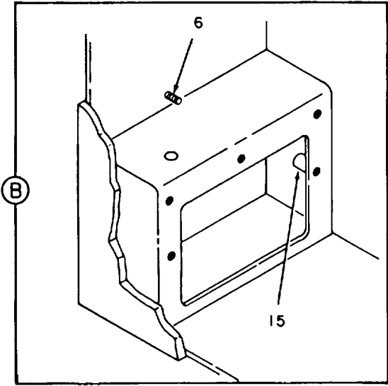
Figure 2. Electrical Equipment Chassis Assembly (Sheet 2 of 2)
