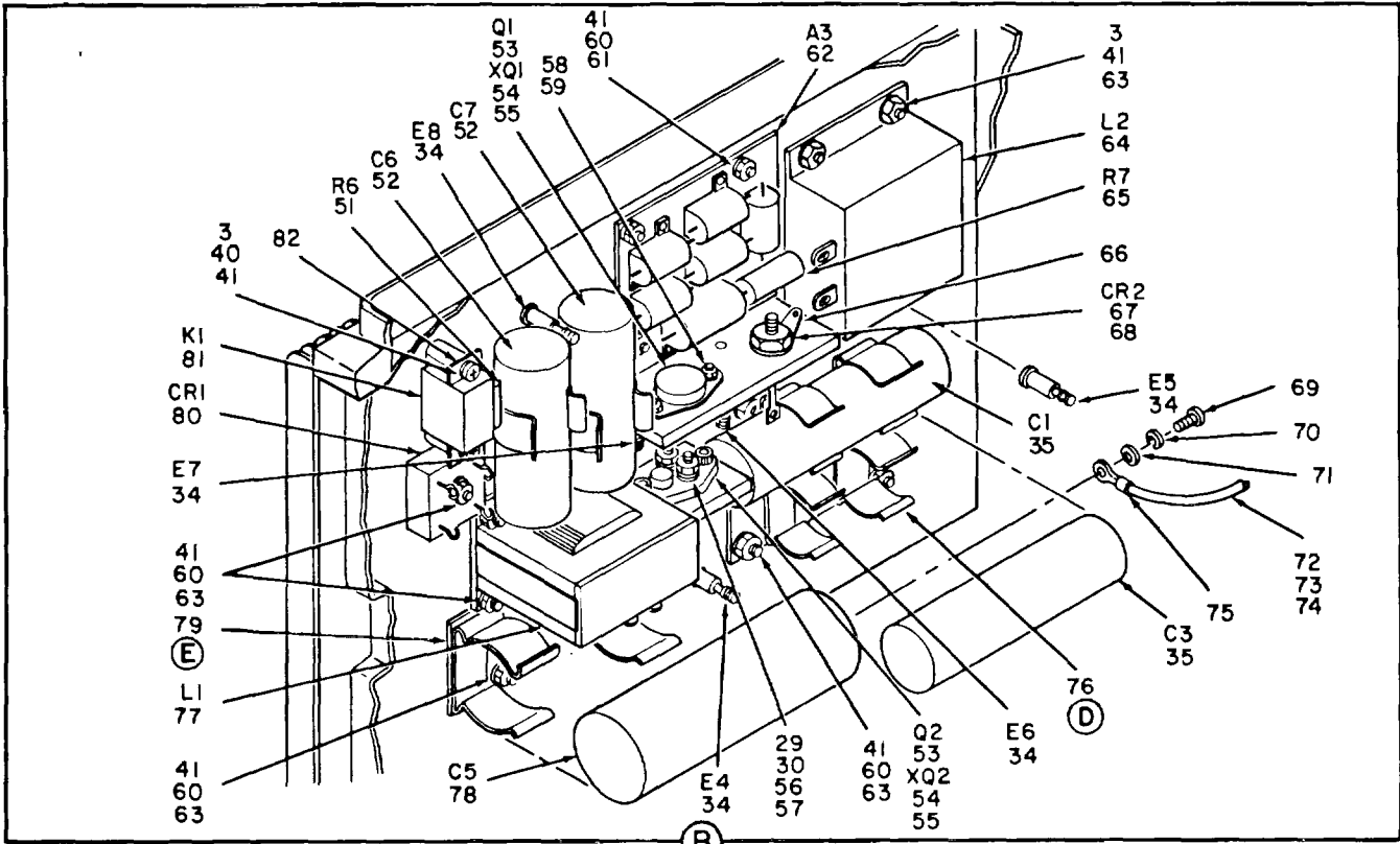
Figure 1. Power Supply PP-6148A/U Sheet 2 of 3)
