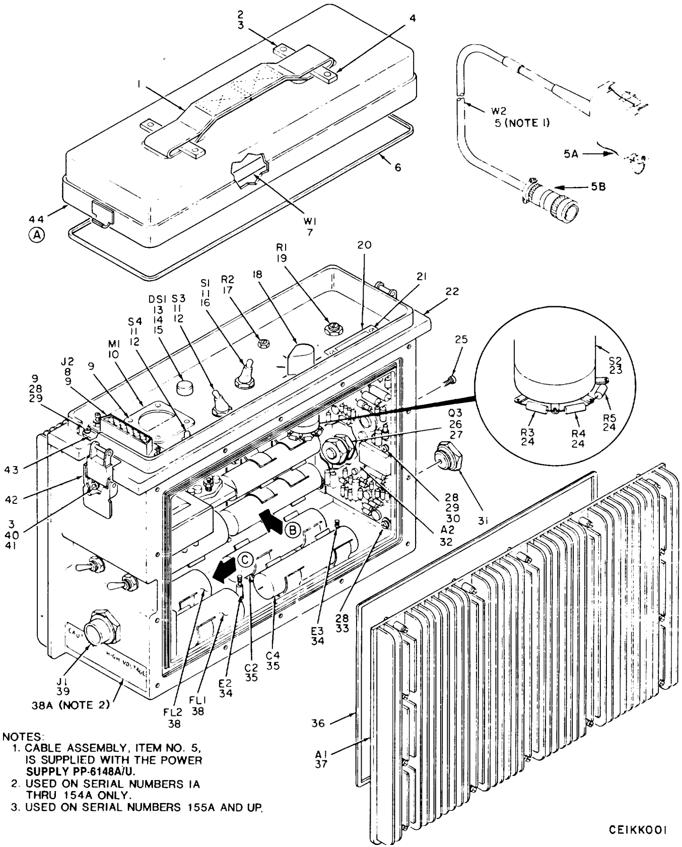
Figure 1. Power Supply PP-6148A/U (Sheet 1 of 3)
