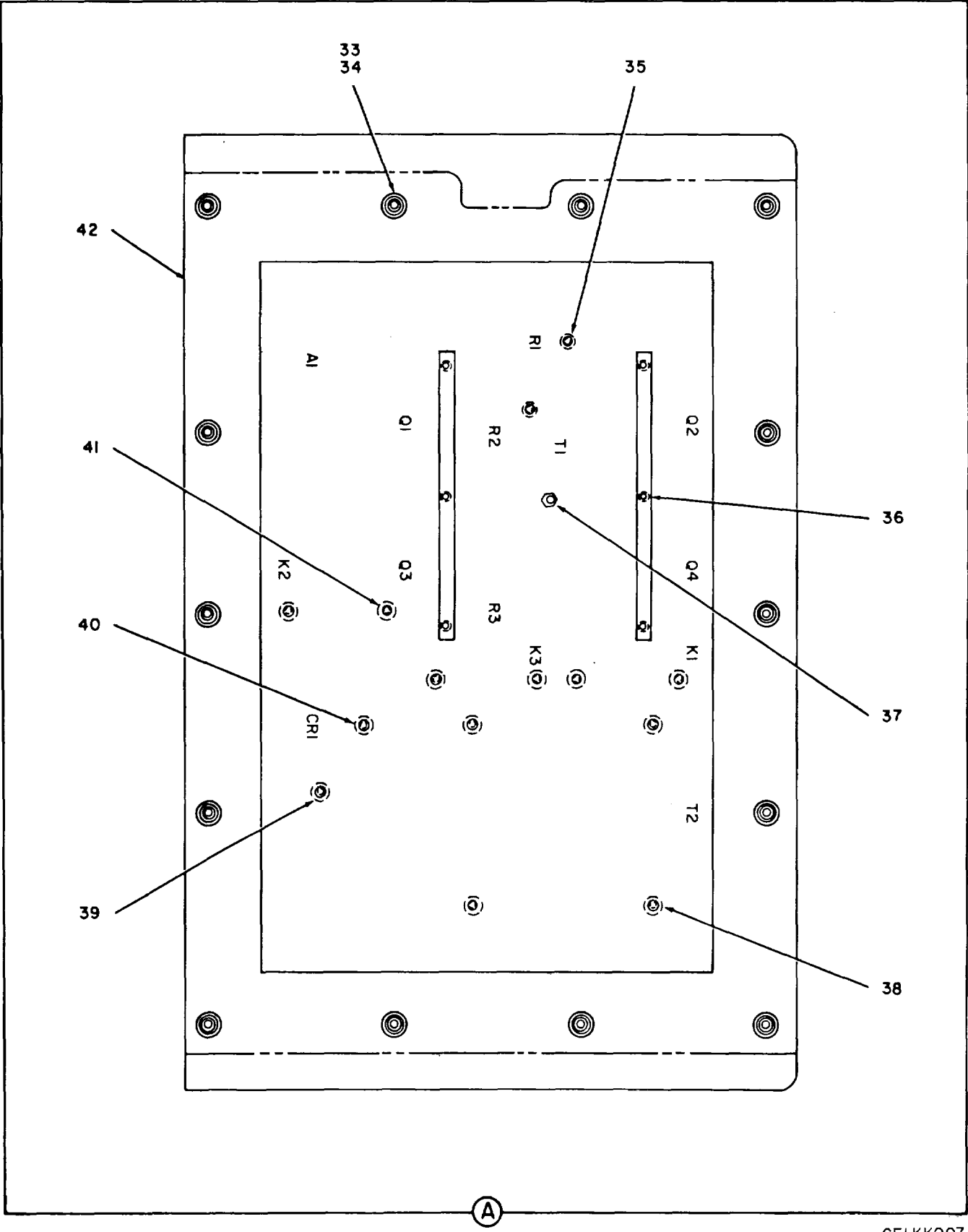
Figure 3. Cover Assembly (A1) (Sheet 2 of 2)
