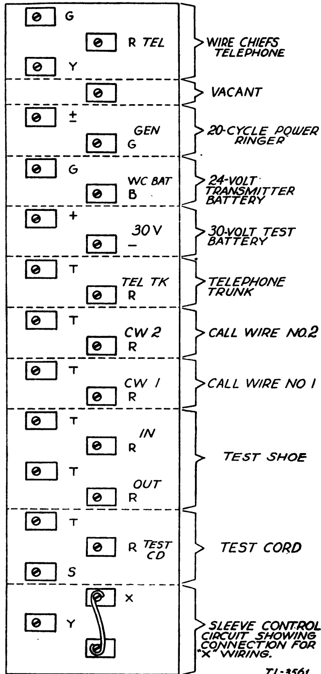
FIGURE 2.—Terminal strip, cabinet BE-70-( ).
