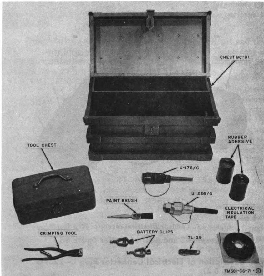
Figure 10.1. (Added) Maintenance Kit, Cable Splicing MK-640/G.
