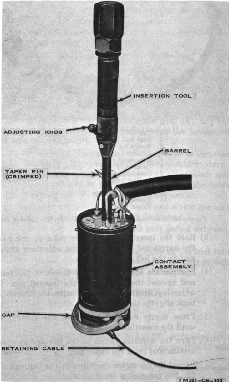
Figure 54. Use of insertion tool.
