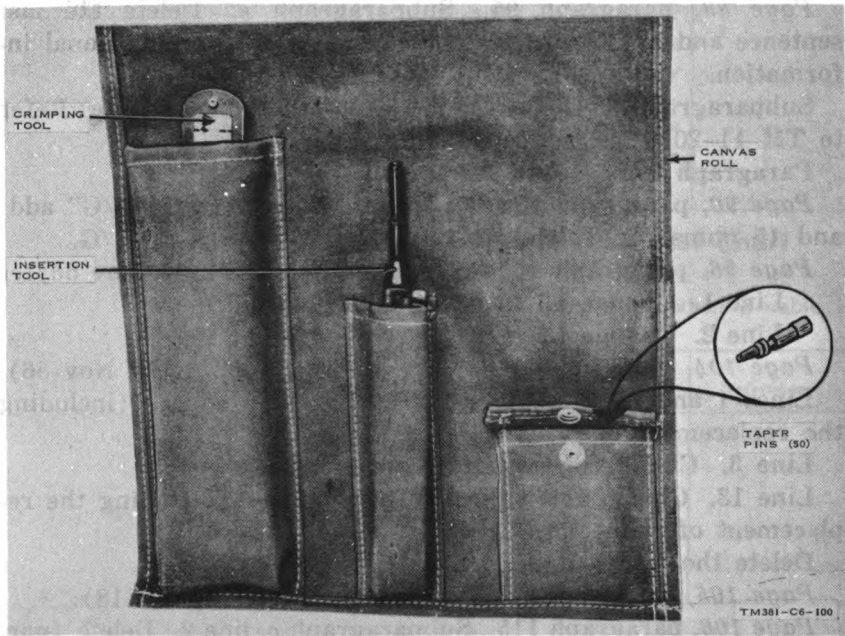
Figure 48. Special tools and materials.
