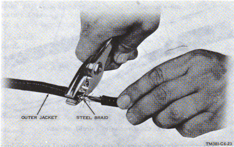
Figure 56. Cutting exposed cable braid.
