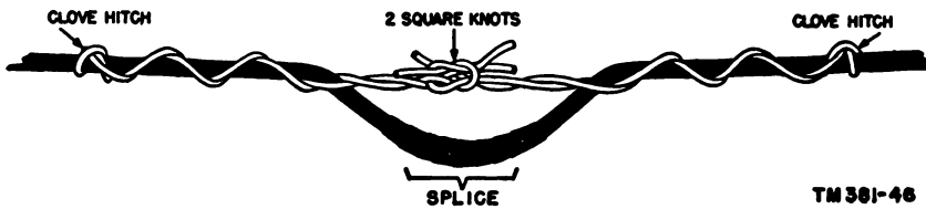
Figure 36. Tension bridge over field splice with basket hitches.
