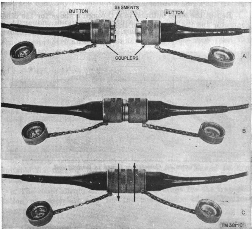
Figure 11. Joining connectors.
