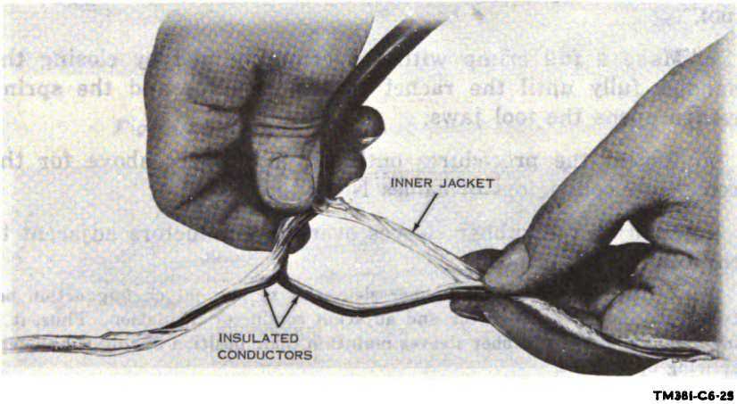
Figure 57. Stripping inner jacket from insulated conductors.
