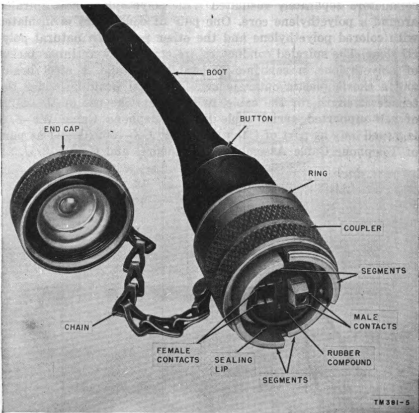
Figure 5. Universal connector.
