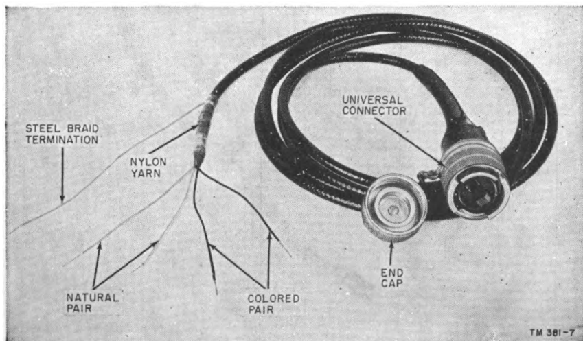
Figure 8. Telephone Cable Assembly CX-1512/U.
