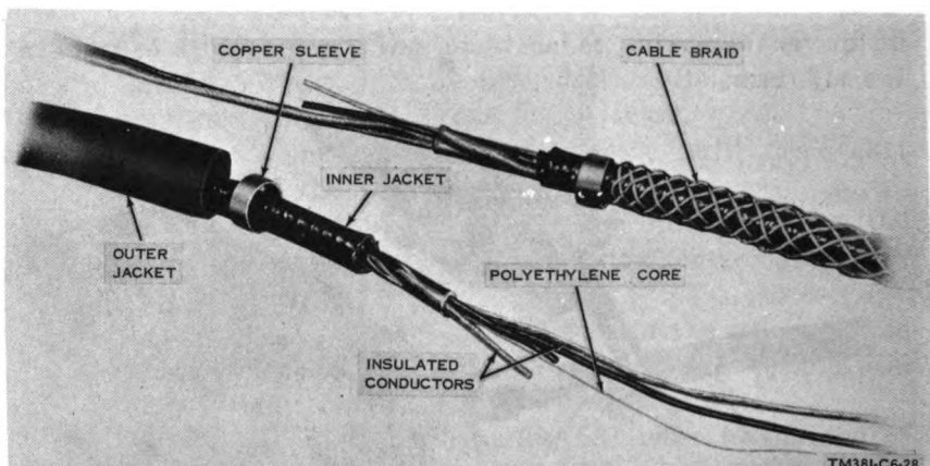
Figure 58. Construction of spiral-four cable.
