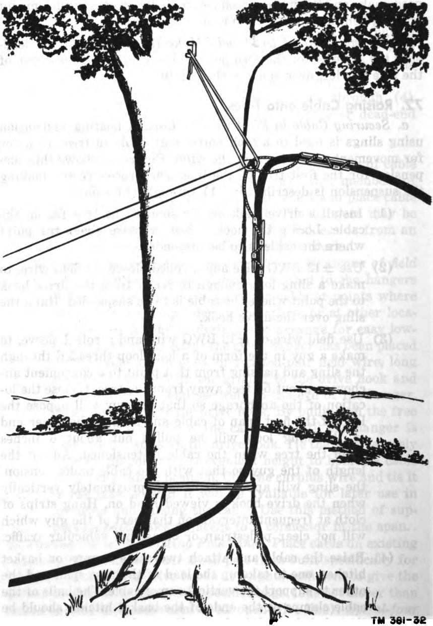
Figure 24. Securing cable to first tree.
