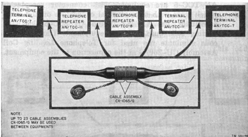
Figure 3. Twelve-channel AN/TCC-7 system using Cable Assemblies CX-1065/G.
