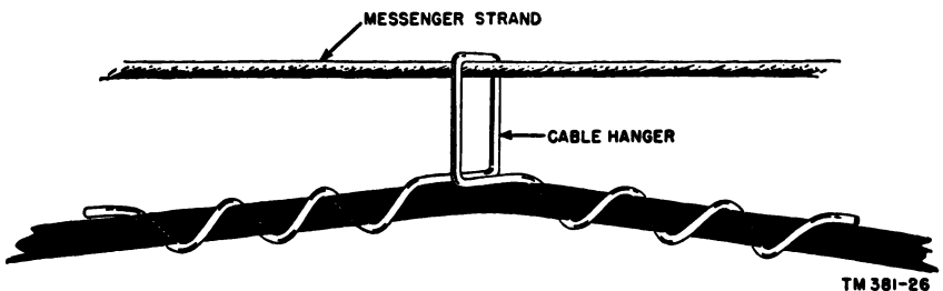
Figure 20. Cable hanger.
