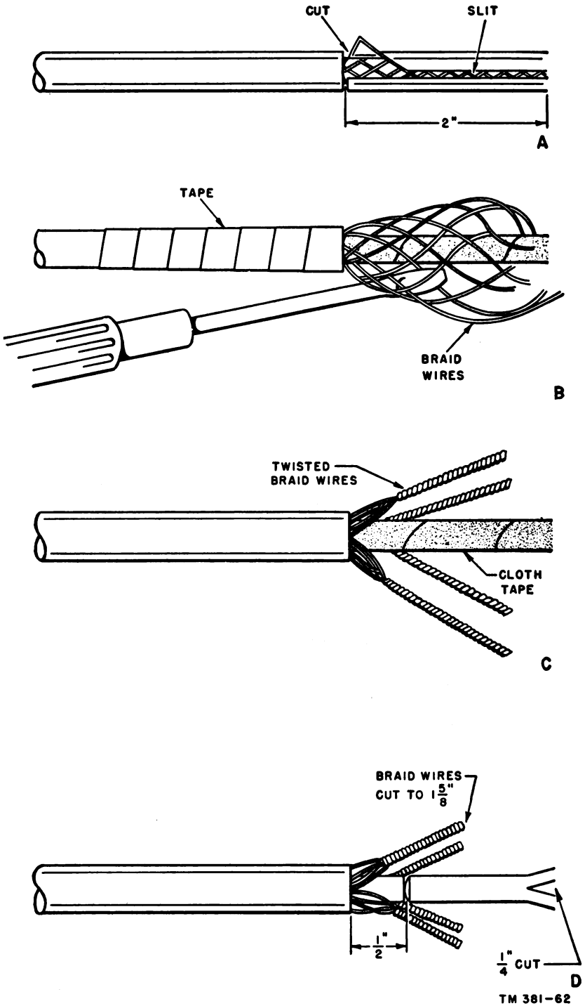
Figure 45. Preparing ends of cable for depot splice.
