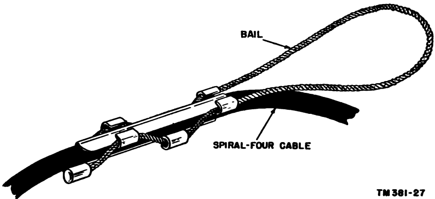
Figure 15. Cable clamp attached to spiral-four cable.
