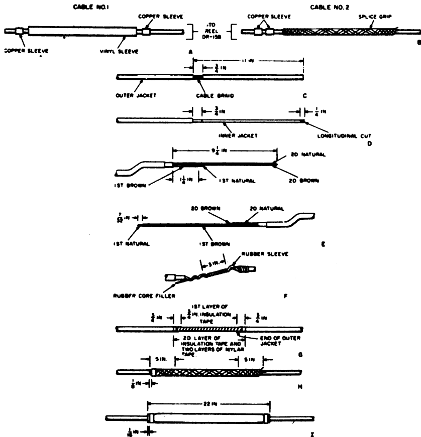
Figure 55. Preparation of spiral-four telephone cable WF-8/F for splicing.
