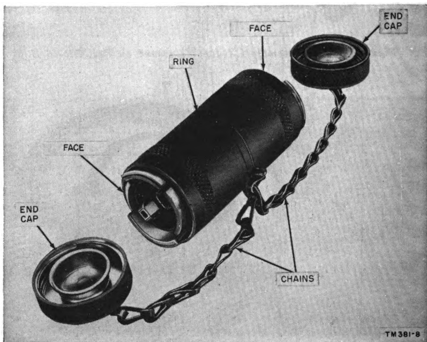
Figure 9. Telephone Loading Coil Assembly CU-260/G.
