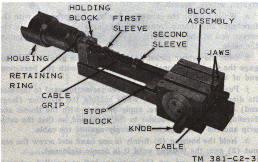
Figure 52. (Added) Use of stretching tool.
