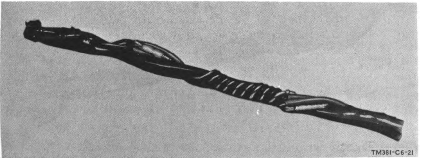
Figure 61. Placement of conductors on core filler.
