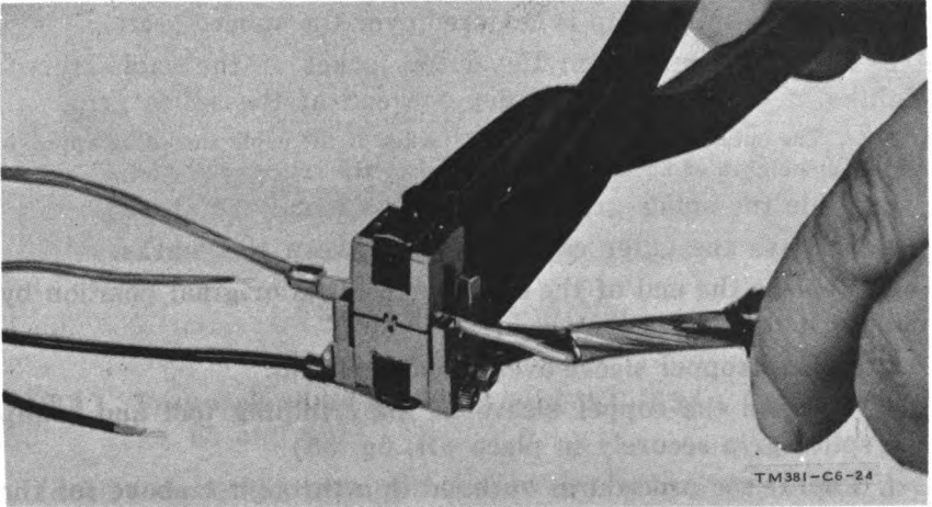
Figure 59. Crimping insulated peeled splice connectors.
