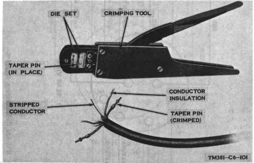
Figure 64. Use of crimping tool.
