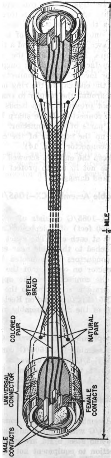
Figure 6. Cable Assembly CX-1065/G, cutaway view.
