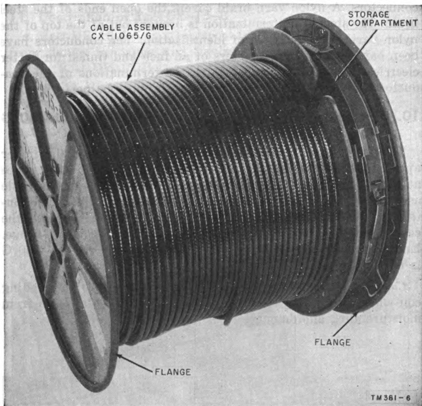
Figure 7. Cable Assembly CX-1065/G, wound on Reel DR-15-B.
