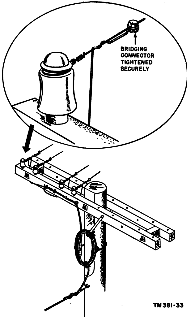
Figure 29. Connecting spiral-four cable to open-wire line.
