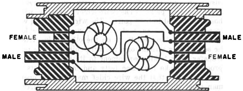
Figure 42. Telephone Loading Coil Assembly CU-260/G, schematic diagram.
