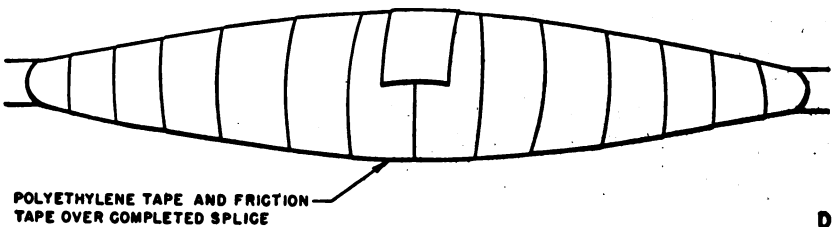
Figure 33. Field splice with sleeves.
