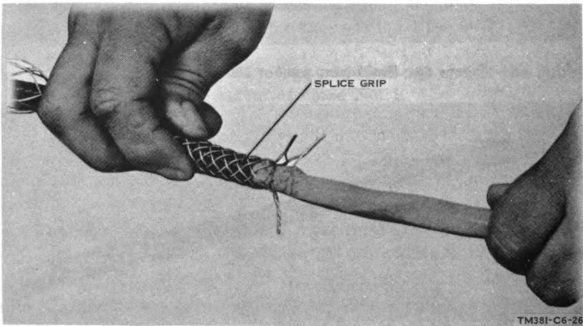
Figure 62. Insertion of splice grip on taped splice.
