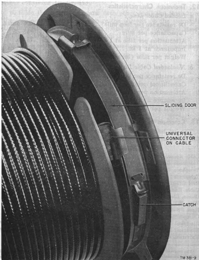
Figure 10. Reel DR-15-B, storage compartment shown with sliding door closed.
