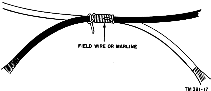
Figure 16. Lashing cable assemblies at connector points.
