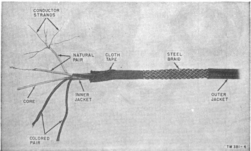
Figure 4. Telephone Cable WF-8/G, construction details.
