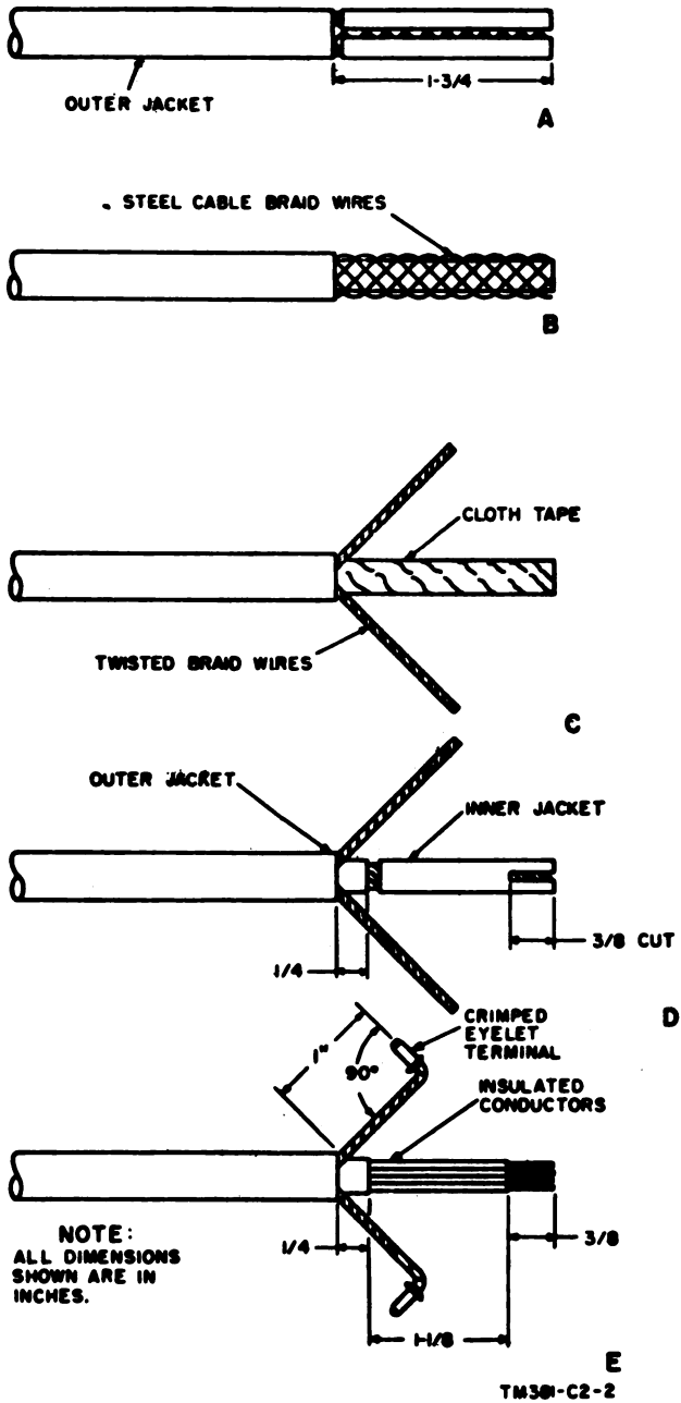
Figure 51. (Added) Preparation of cable end.
