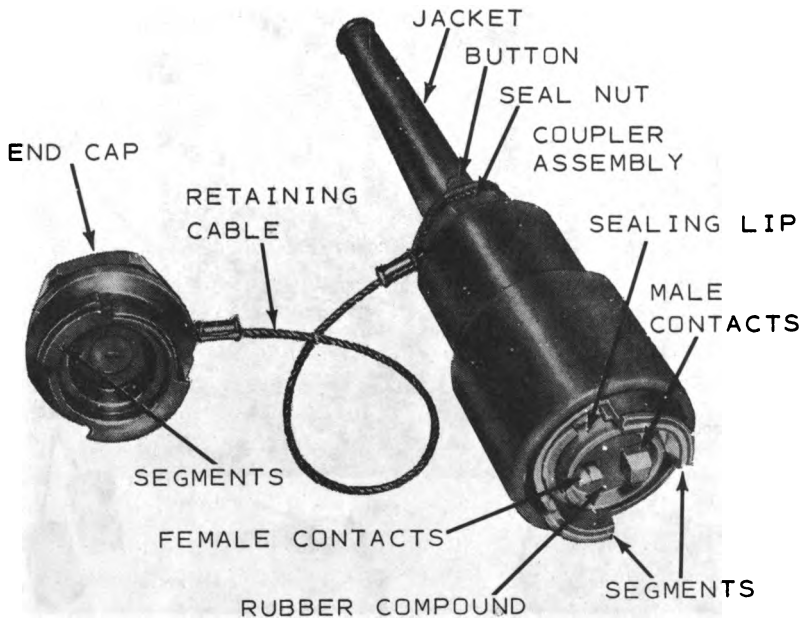
Figure 5.1. (Added) Electrical connector plug U-176/G.
