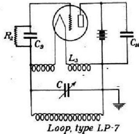
FIGURE 8.—Simplified transmitter circuit.
