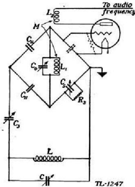
FIGURE 10.—Simplified receiver circuit.
