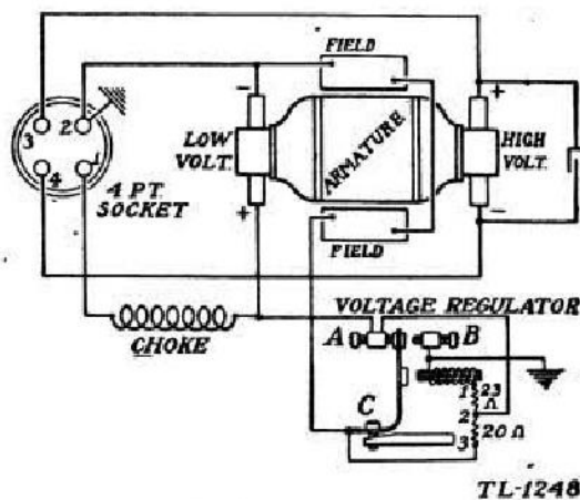
FIGURE 11.—Wiring diagram GN-35.
