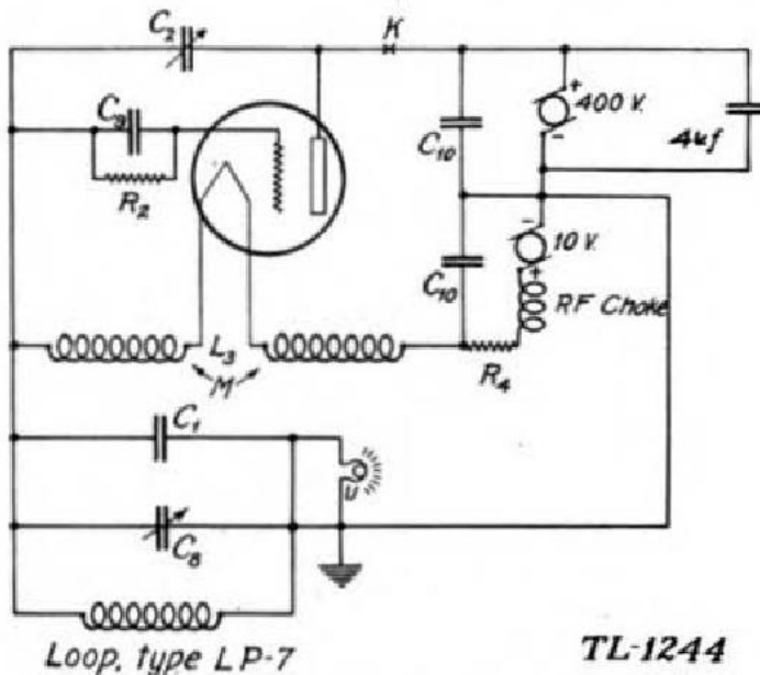
FIGURE 7.—Schematic transmitter circuit.
