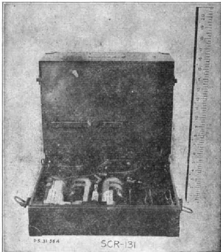
FIGURE 4.—Radio receiver and transmitter BC-148 (151), showing interior of battery-compartment box.
