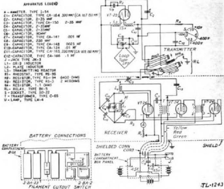
FIGURE 6.—Circuit diagram, SCR-131 (161).
