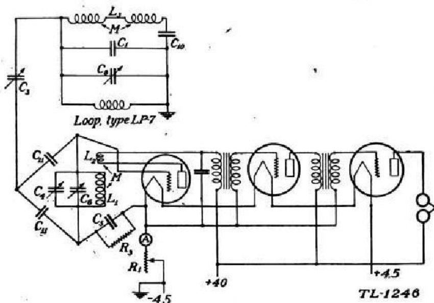
FIGURE 9.—Schematic receiver circuit.
