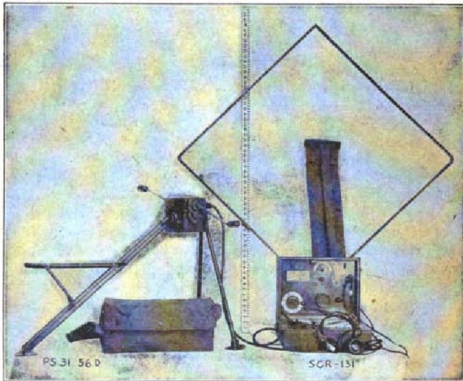
FIGURE 1.—Radio set SCR-131 (161), set up for operation.
