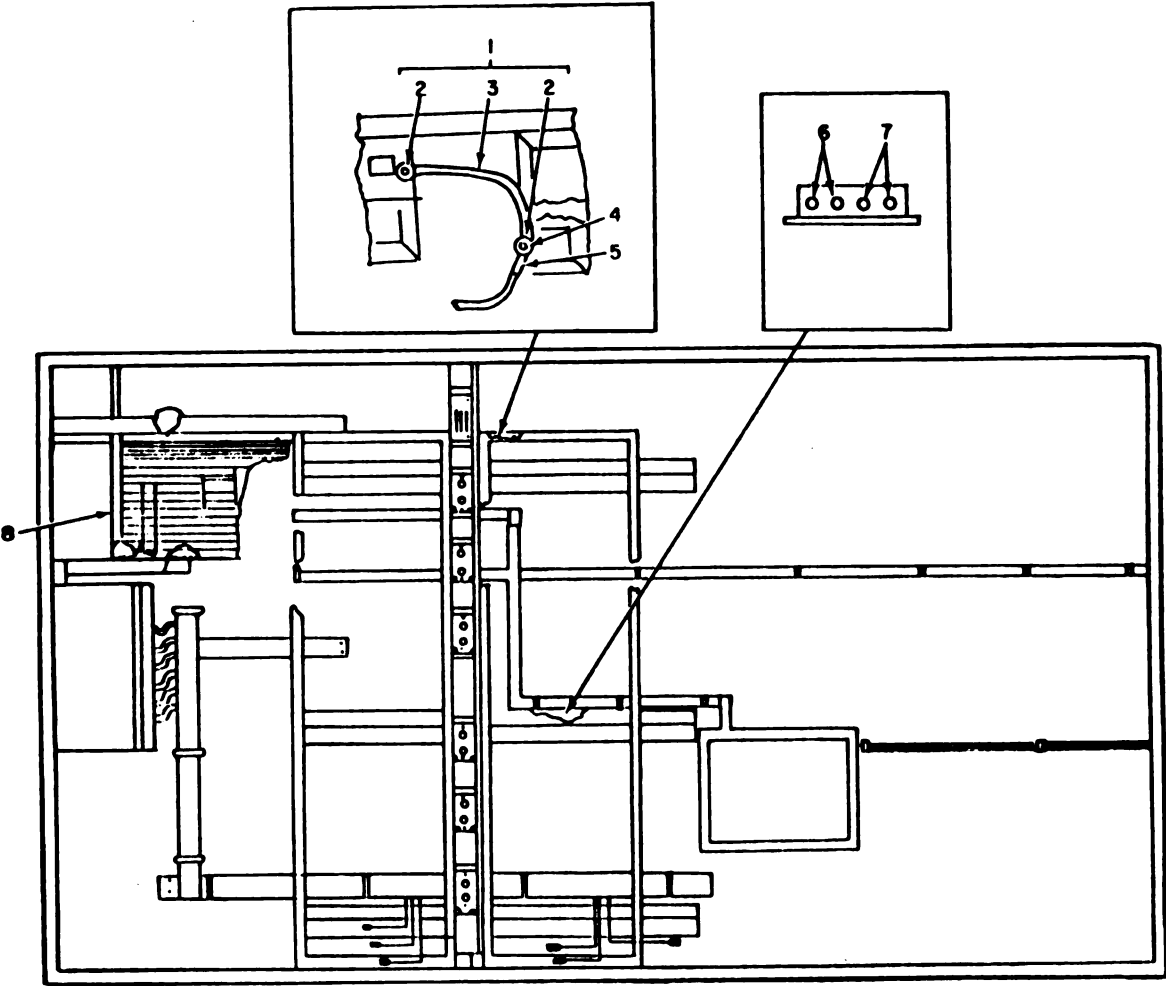
ROAD SIDE VIEW (FOR S330B SHELTER)
