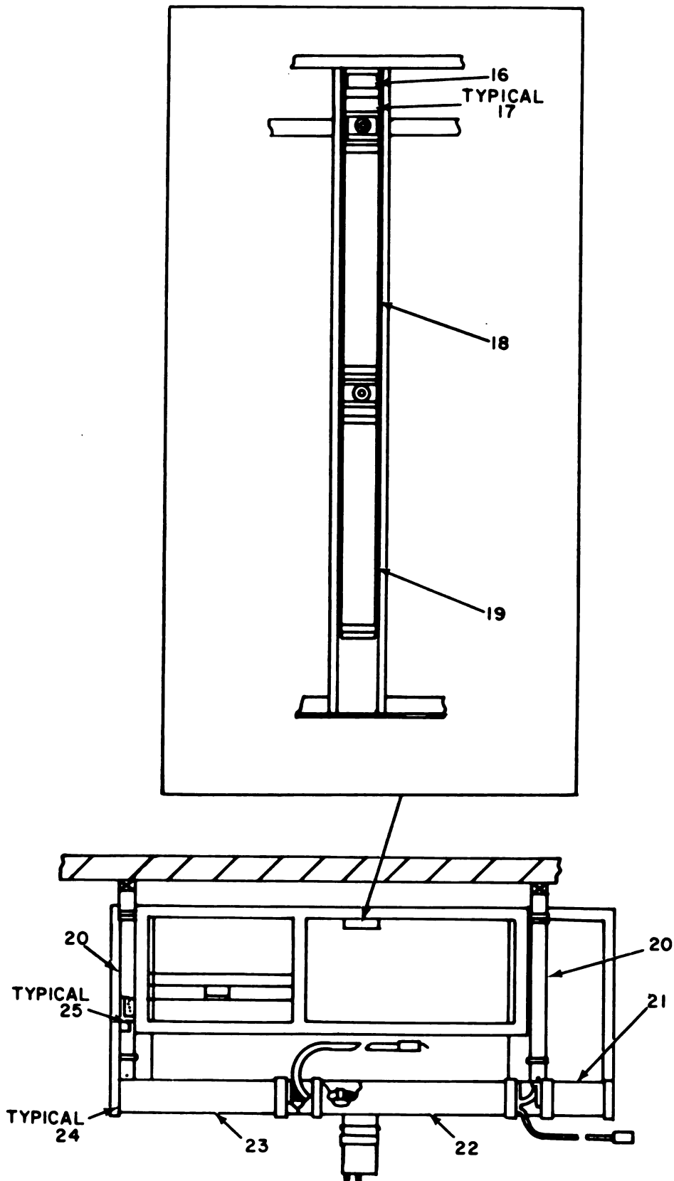
INTERNAL TOP VIEW
