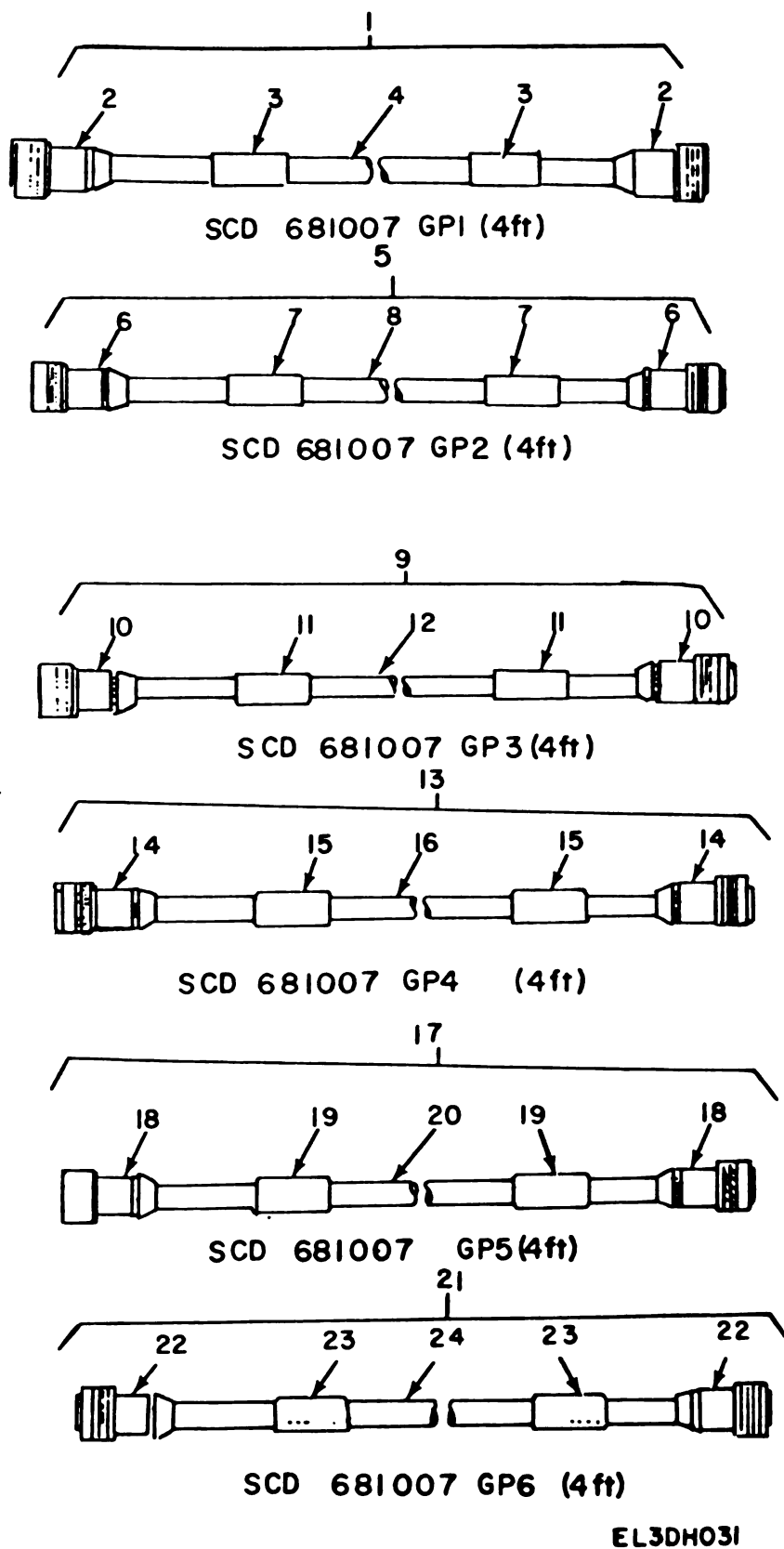
Figure 19. Cable Assemblies Used in Conjunction with Shelter, Electrical Equipment S-330B/TRC-117 (Sheet 1 of 3).
