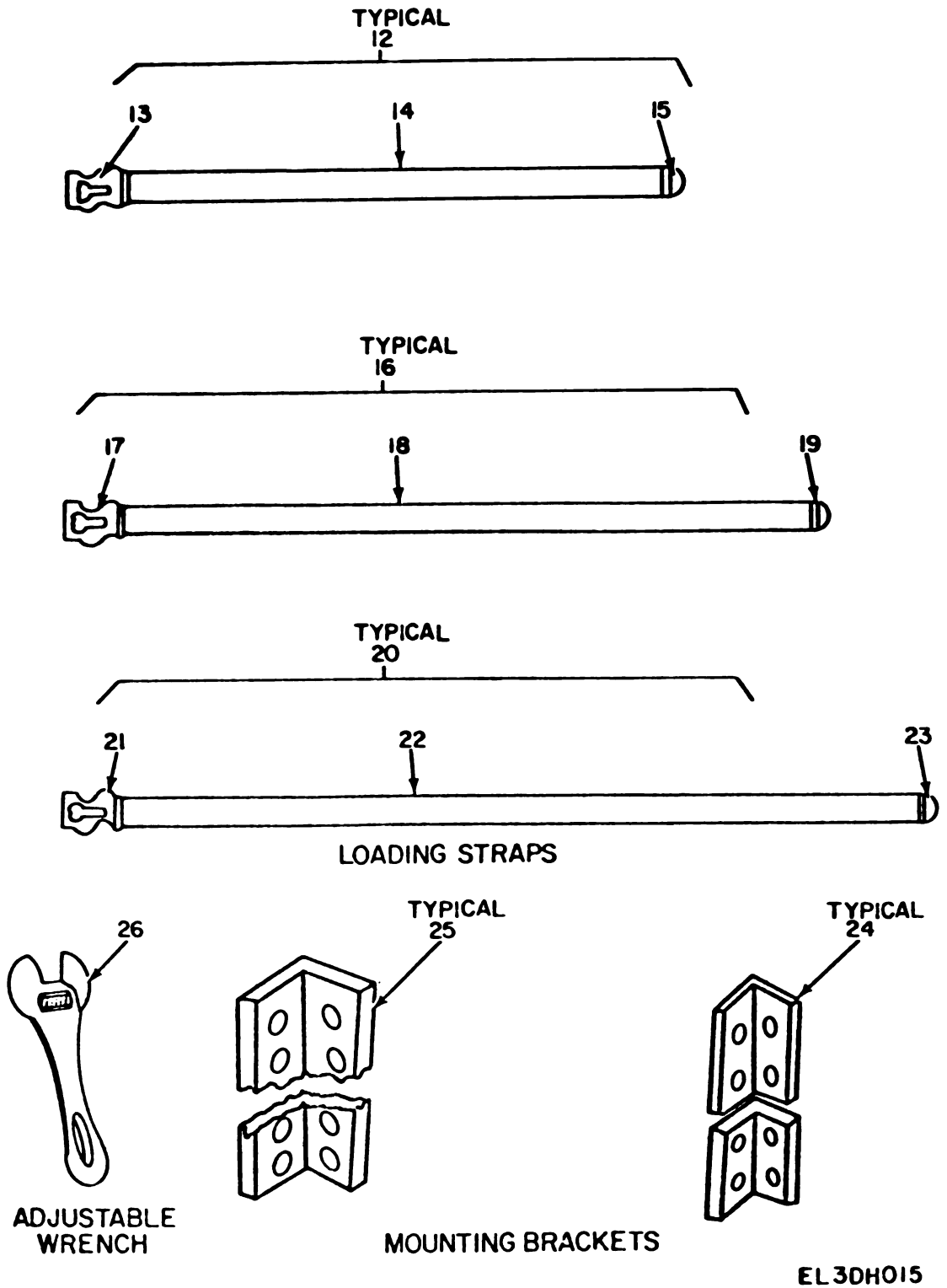
Figure 8. Miscellaneous Components (Sheet 2 of 3).
