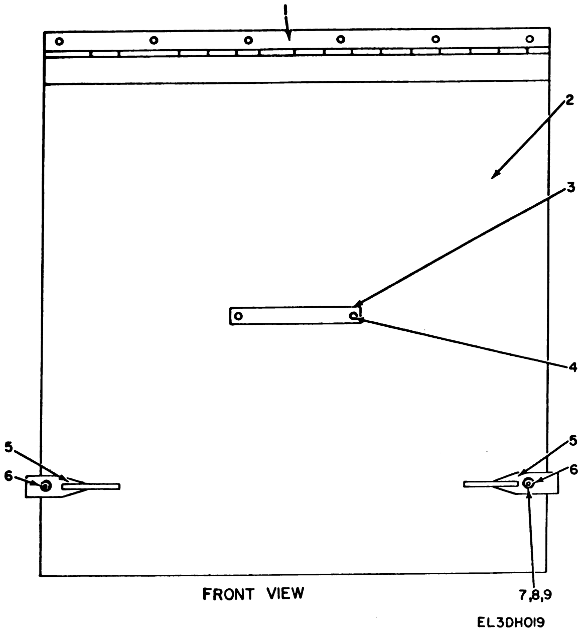
Figure 10. Power and Signal Entrance Cover Assembly (Sheet 1. of 2).
