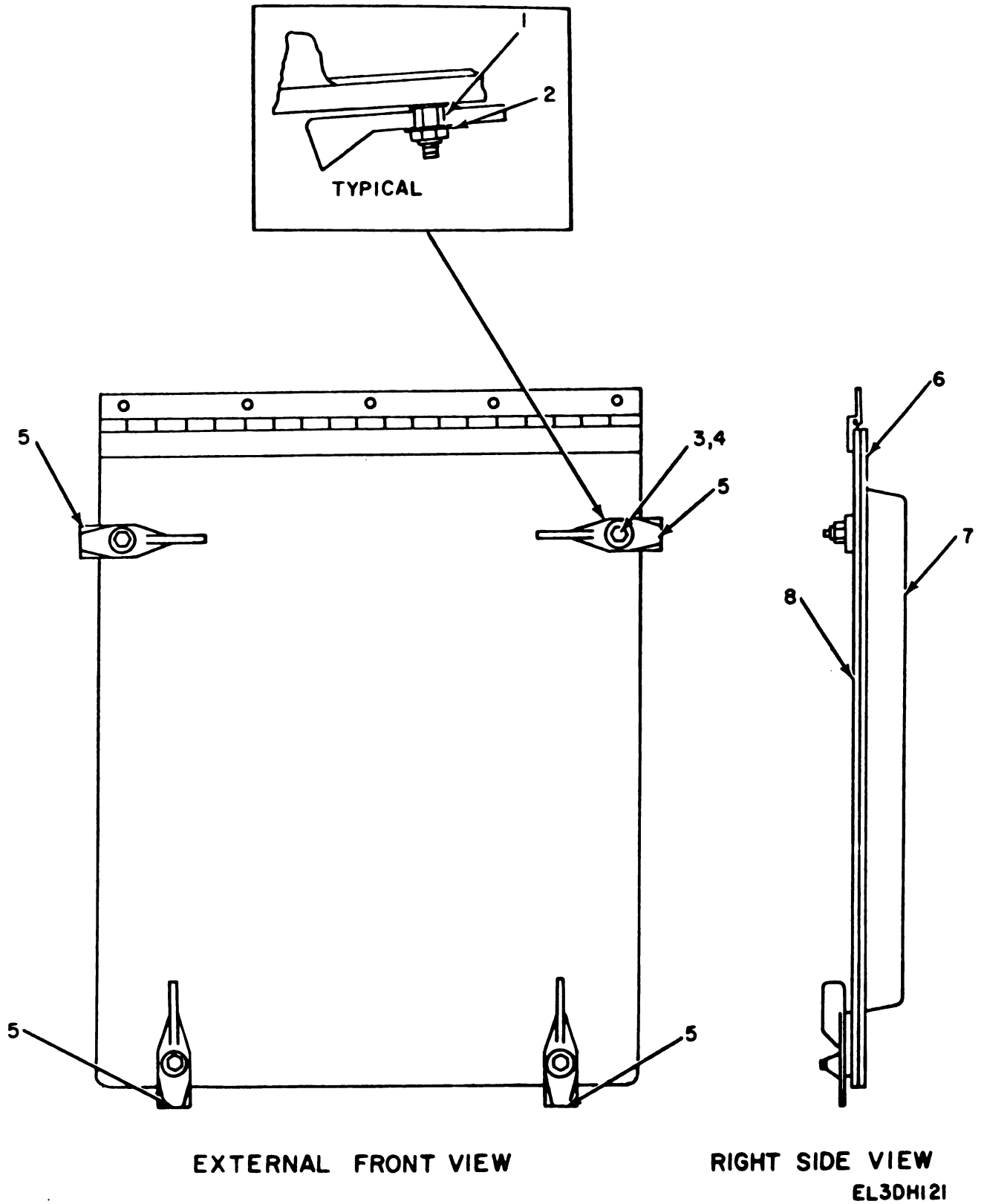
Figure 84. Cover Assembly External Front and Right Side Views.
