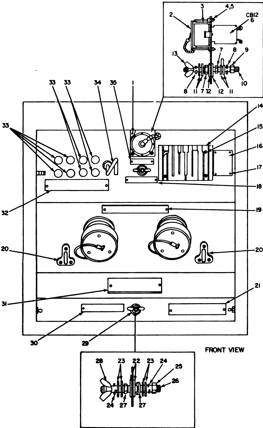
POWER ENTRANCE BOX
