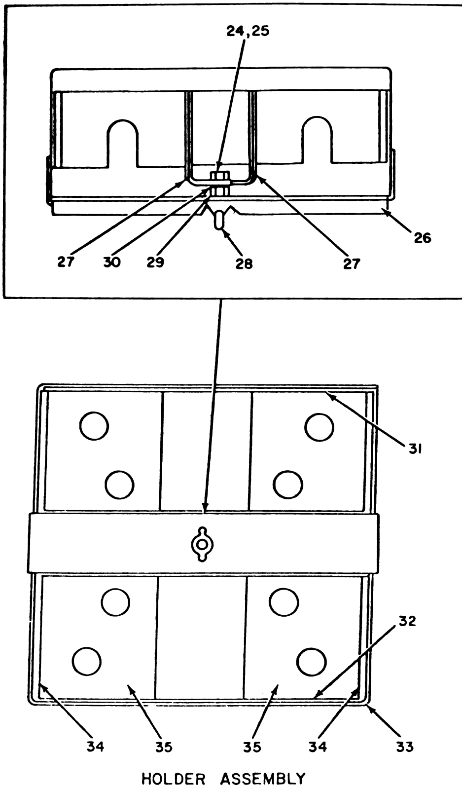
Figure 78. Rack Assembly and Holder Assembly (Sheet 3 of 3).
