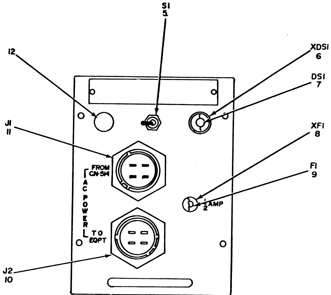
SLIDE ASSEMBLY, FRONT VIEW
