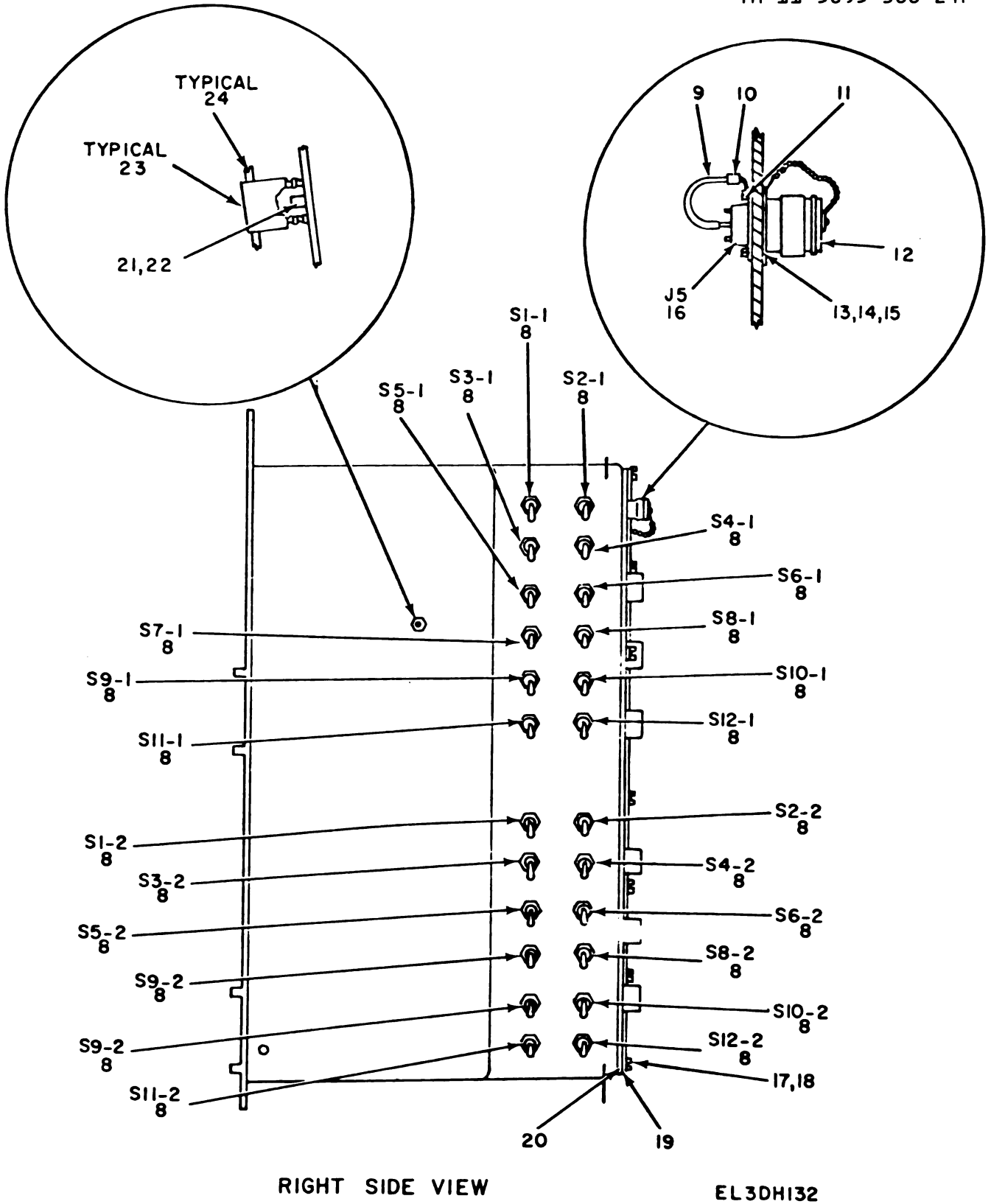
Figure 90. Signal Entrance Box, Roadside System 2 (Sheet 2 of 3).
