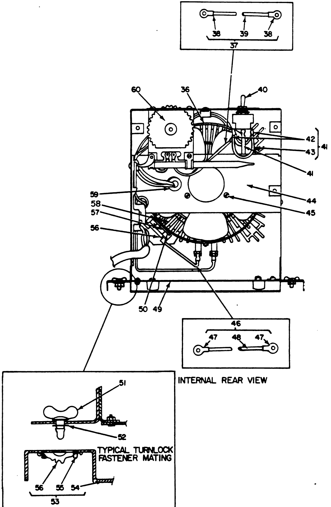
Figure 22. Heater Assembly (Sheet 2 of 3).
