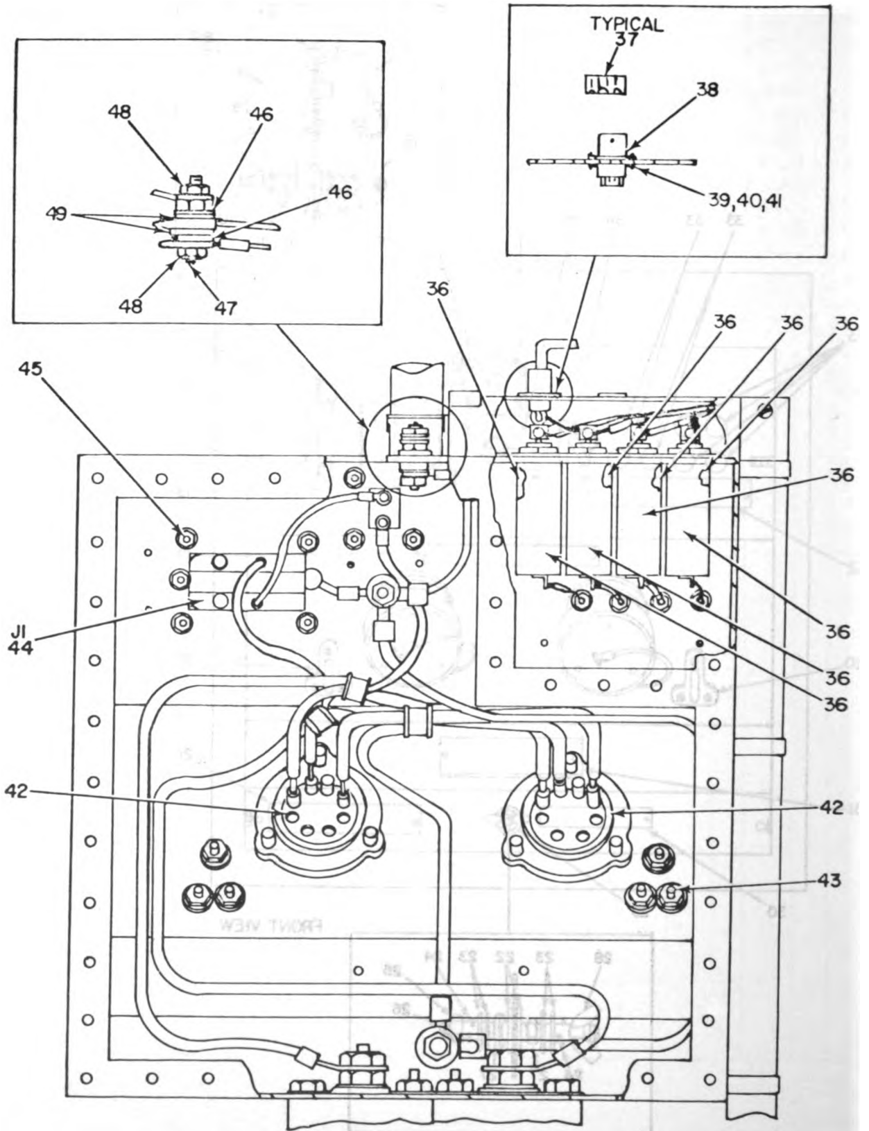
Figure 53. Power Entrance Box (Sheet 2 of 2).
