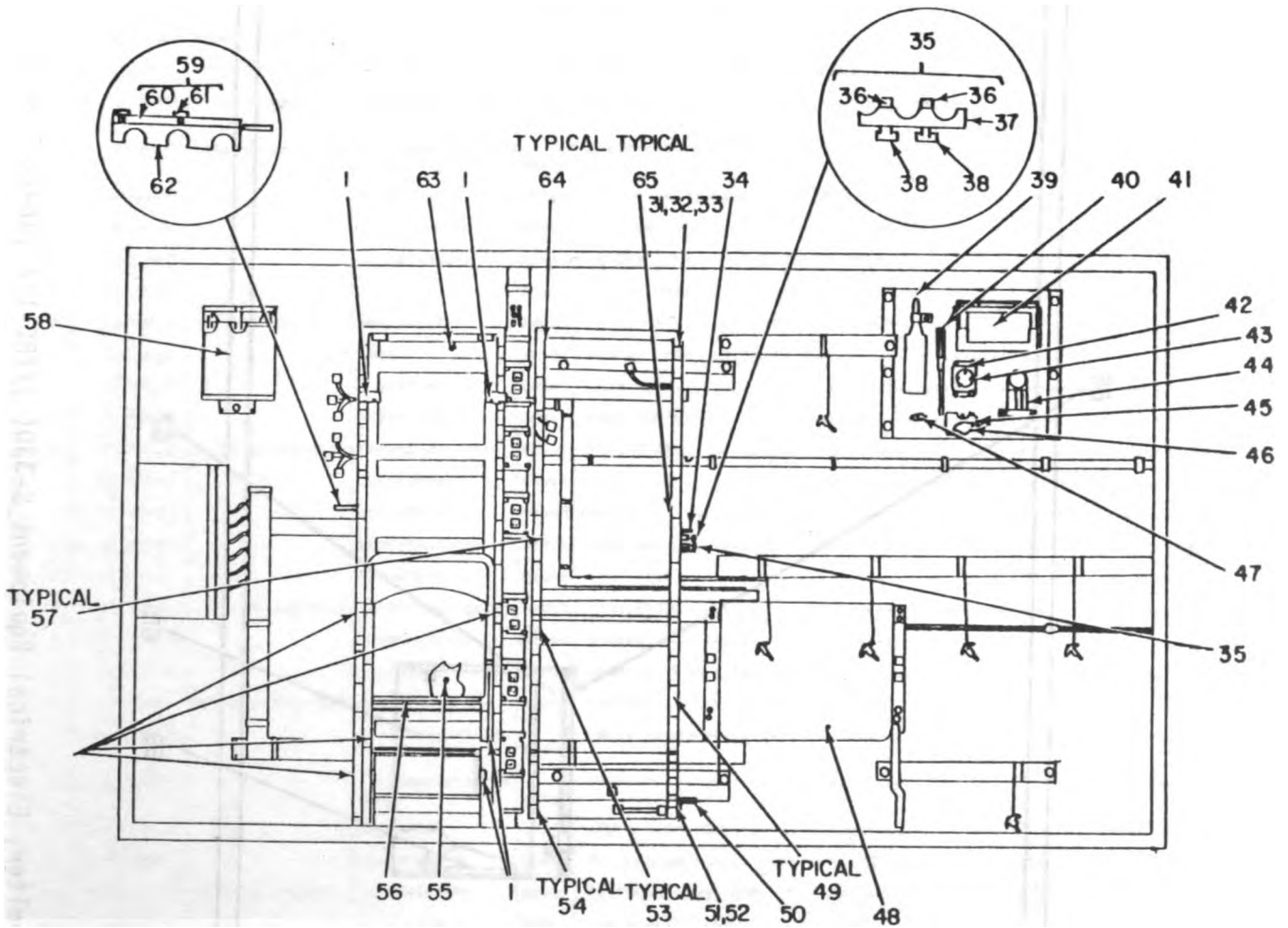
INTERIOR ROADSIDE WALL
