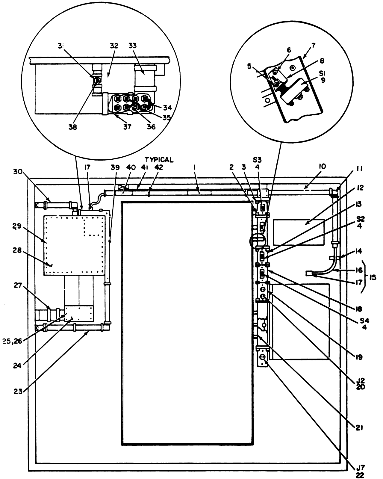
Figure 33. Rear Electrical Utilities Installation.
