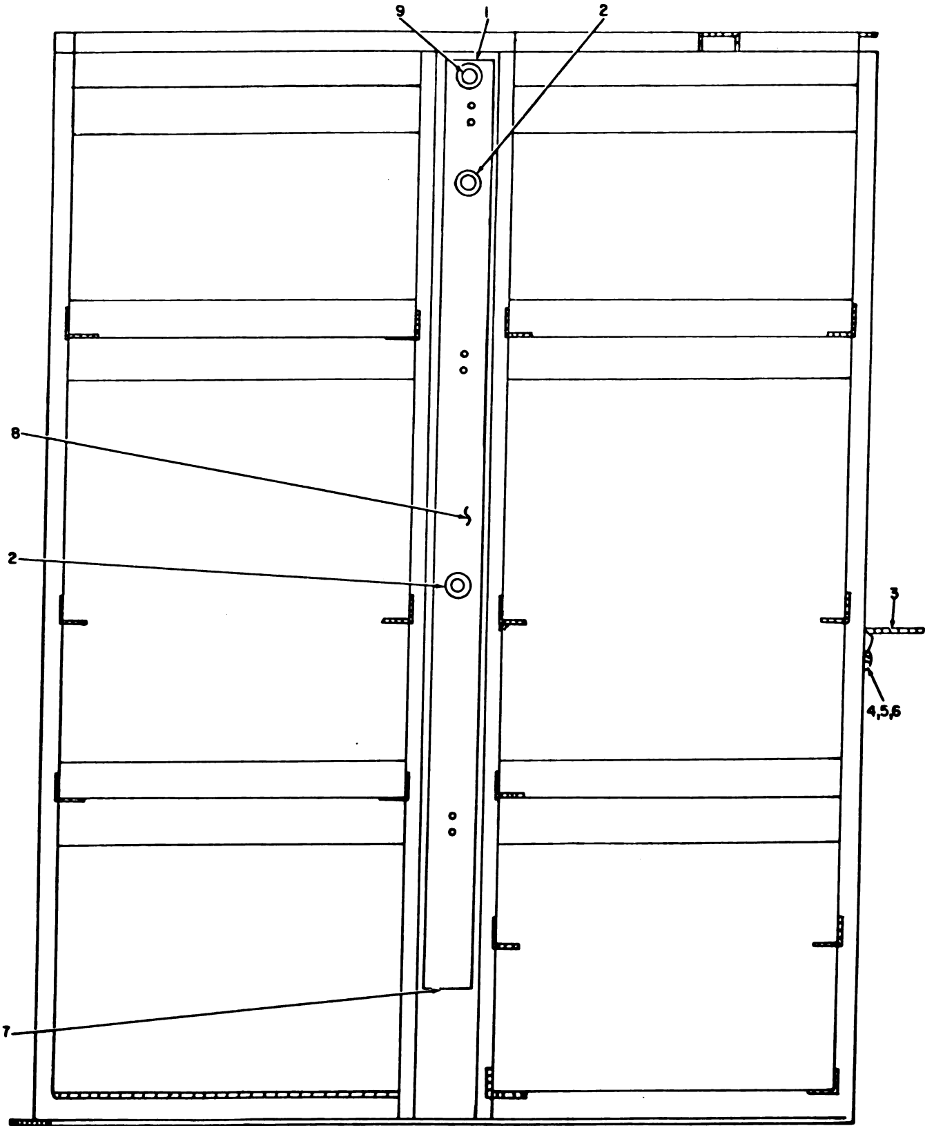
REAR VIEW
