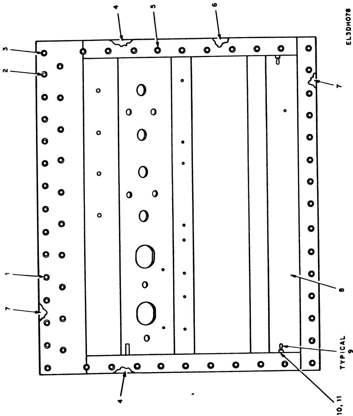
Figure 52. Cover Bracket Installation.
