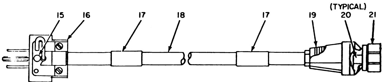
CABLE ASSEMBLY, POWER ELECTRIC SCC547175 (4 FT)
