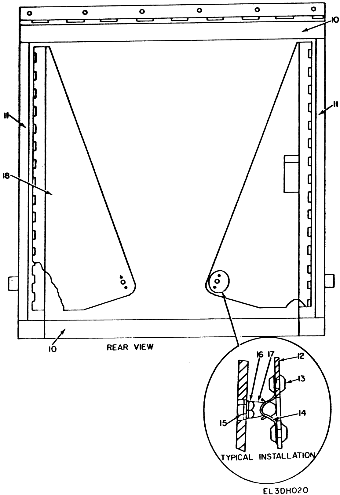
- Figure 10. Power and Signal Entrance Cover Assembly (Sheet 2 of 2).
