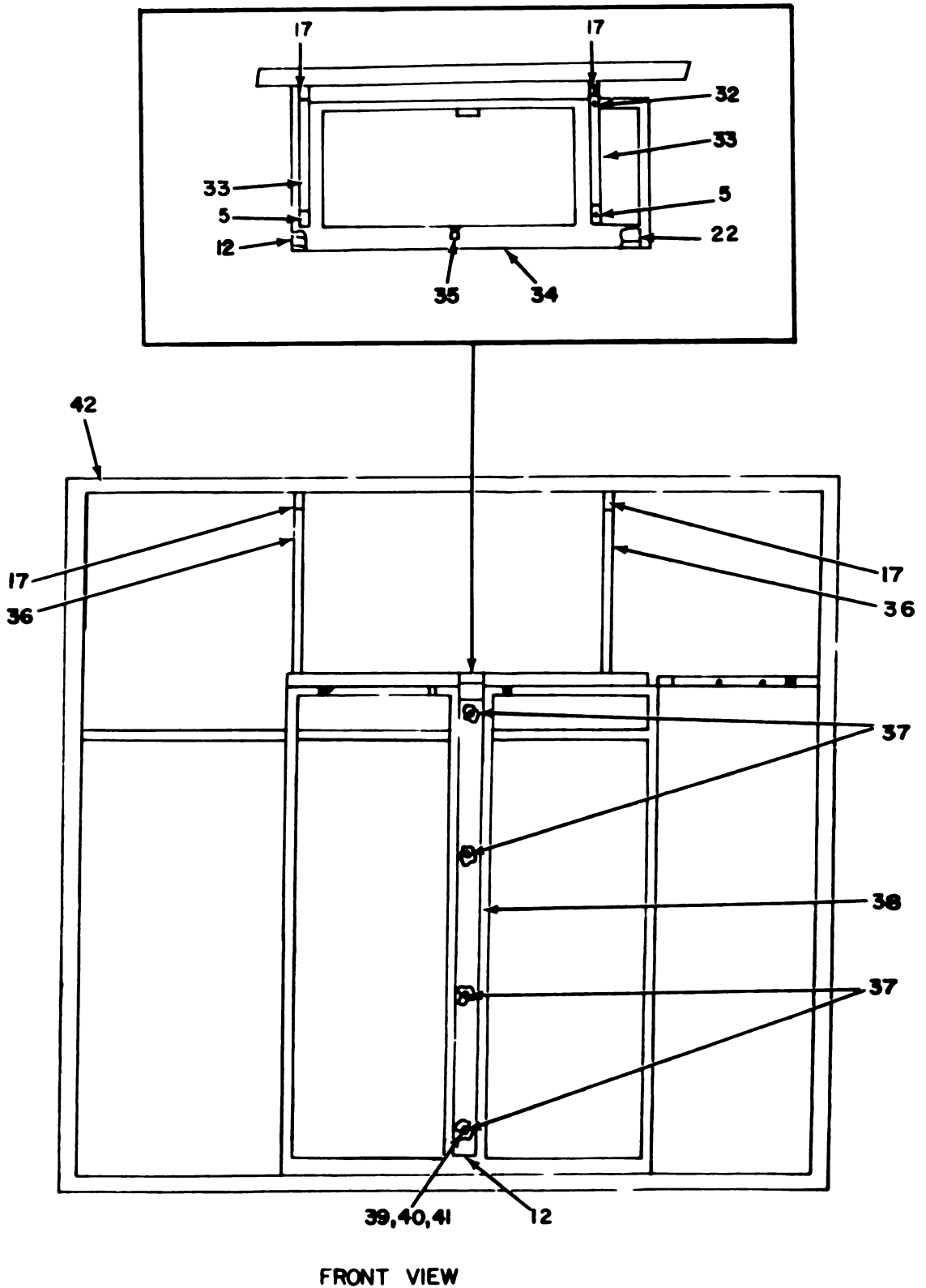
Figure 57. Front View of Electrical Utilities Installation in Electrical Equipment Shelter S-330B/TRC-117 (Sheet 2 of 2).
