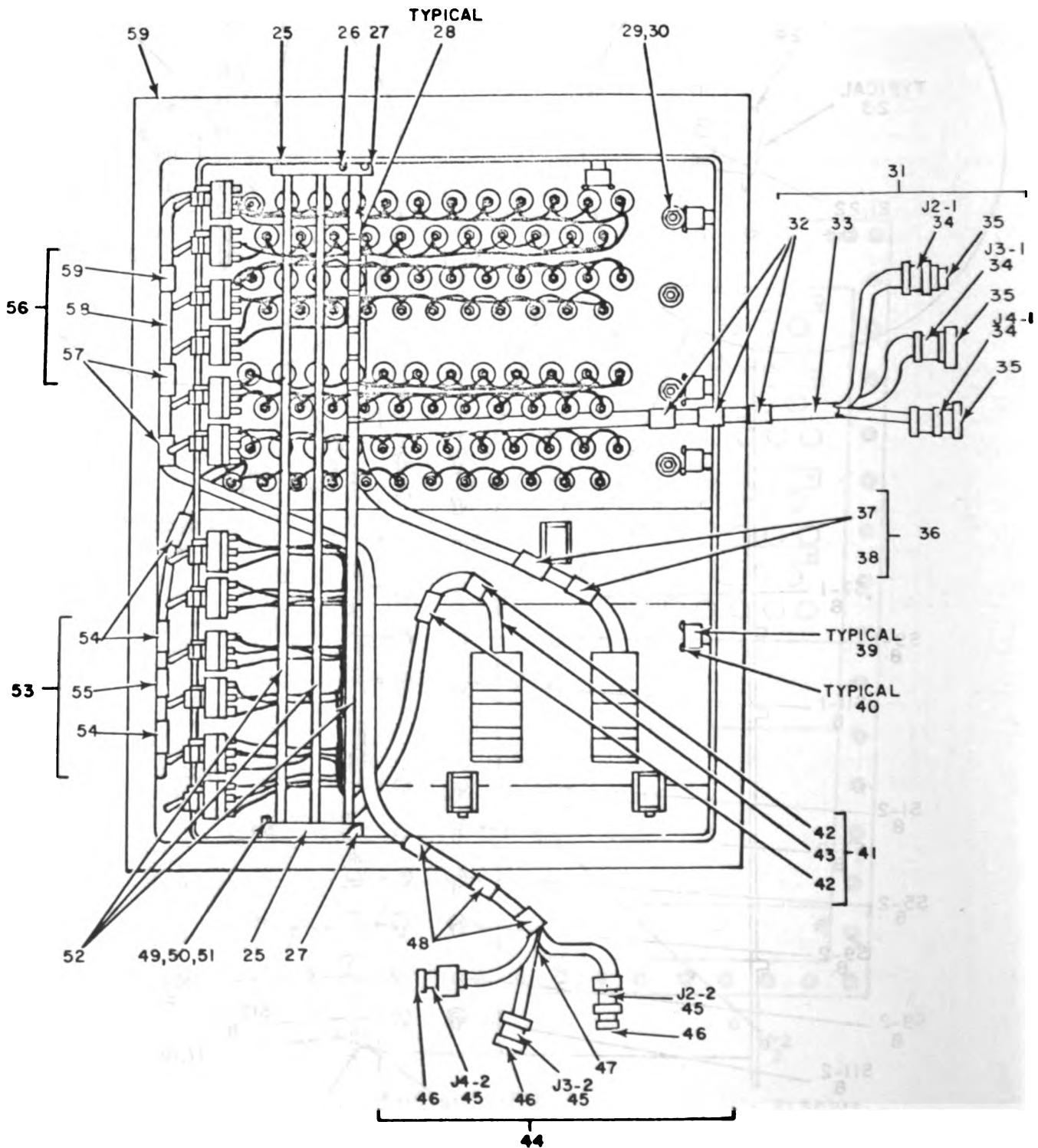
REAR VIEW
