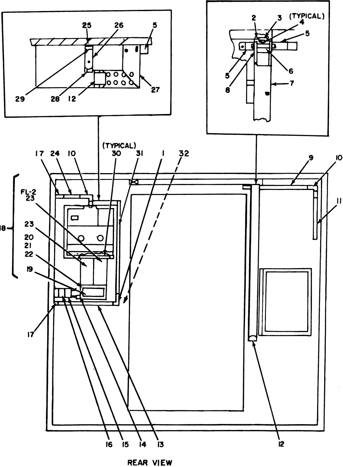
Figure 57. Rear View of Electrical Utilities Installation in Electrical Equipment Shelter S-330B/TRC-117 (Sheet 1 of 2).
