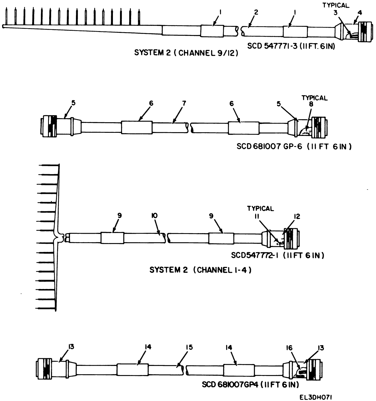
Figure 47. Special Purpose Electrical Cable Assemblies SCD 547771-3, SCD 547772-1, SCD 681007 GP-4 and GP-6.
