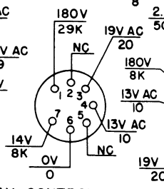
RELAY CONTROL V210 6C4W
