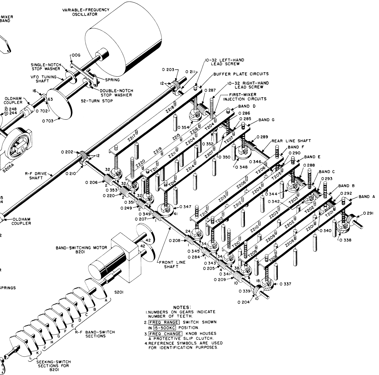
Figure 45. Tuning system, exploded view.
