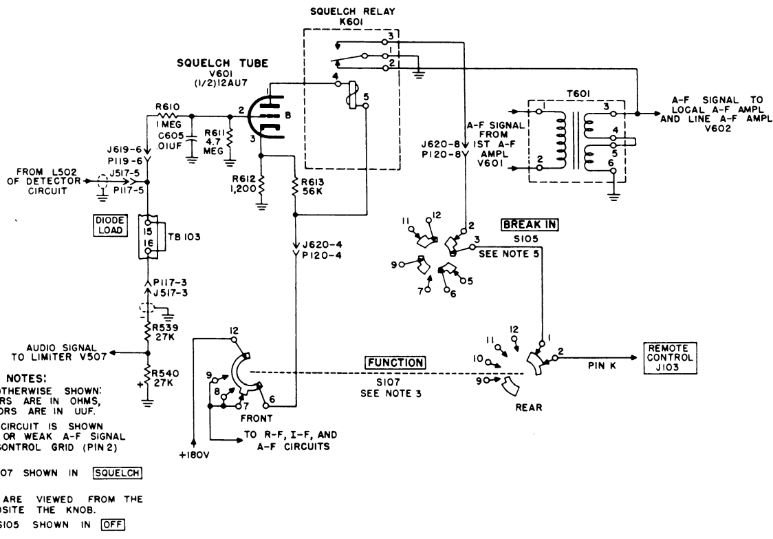
Figure 34. Squelch circuit, schematic diagram.
