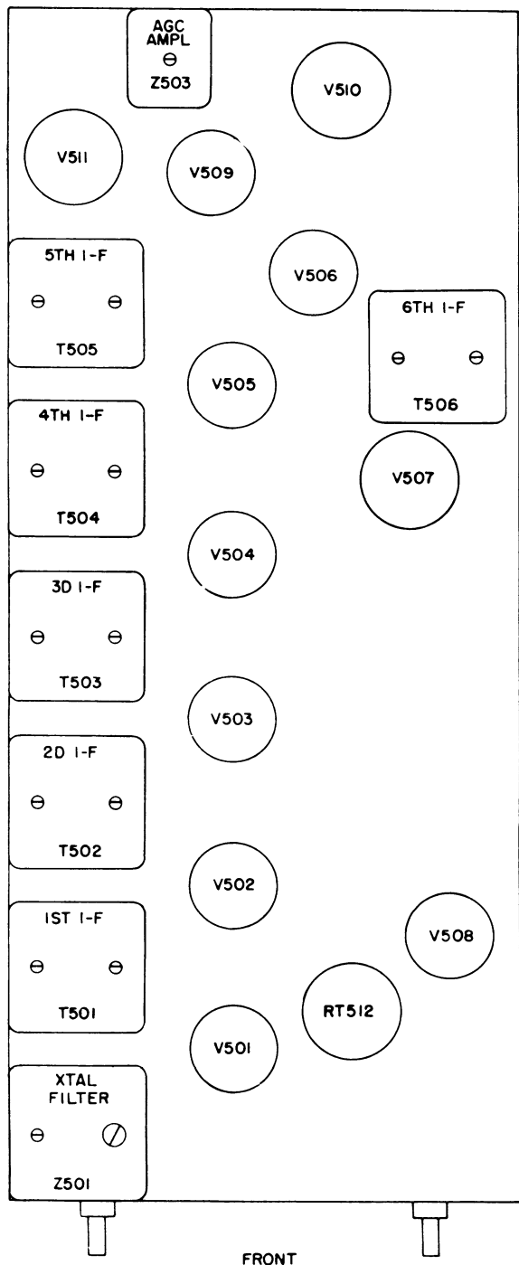
Figure 80. If. subchassis, location of tubes and trimmers.
