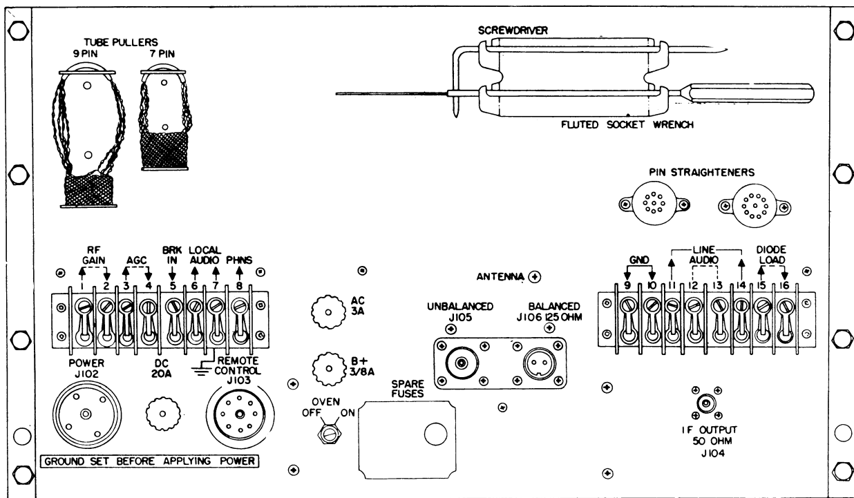
Figure 7. Back panel.
