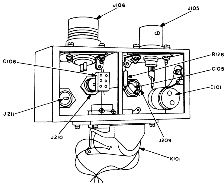
Figure 72. Antenna box, interior view.
