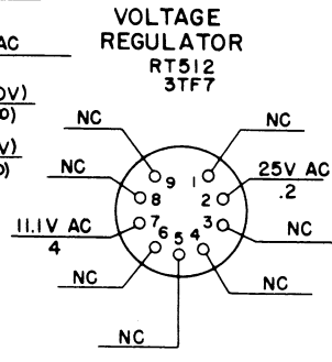
Figure 66. Tube-socket voltages and resistances, top deck.
