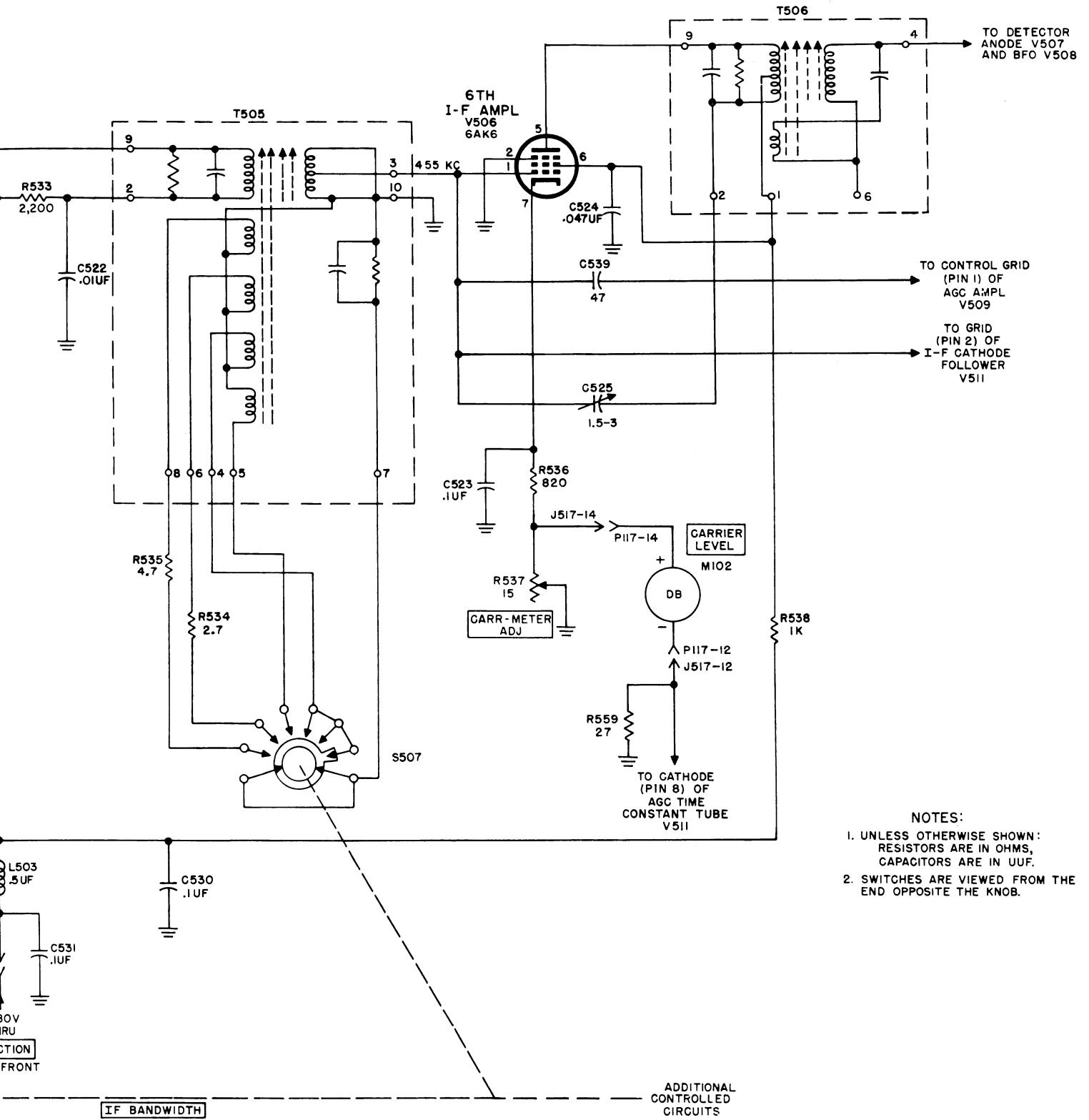
and sixth if. amplifiers, schematic diagram.
