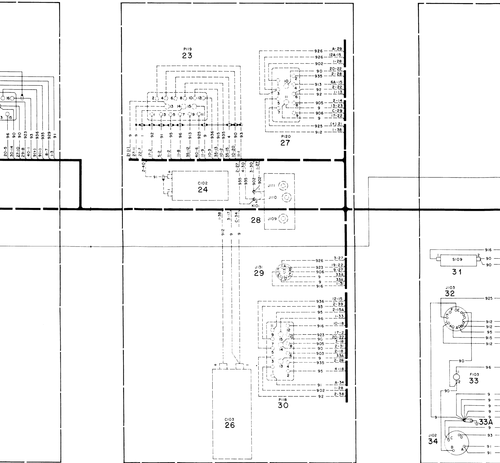
Figure 90. Wiring diagram.
