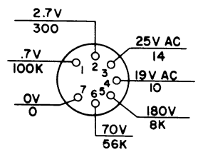
2D MIXER V205 6BE6
