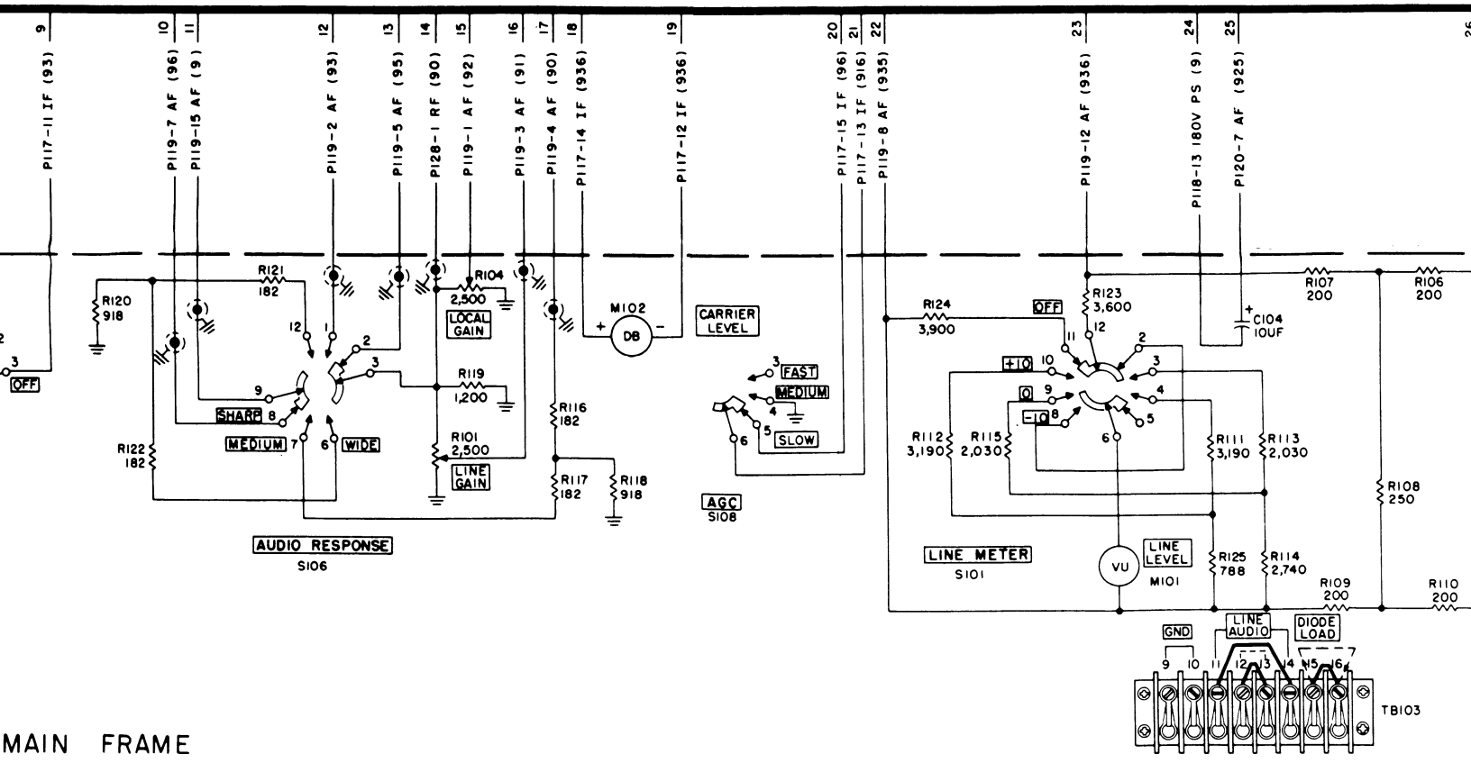
Figure 88. Subcassis and interconnection diagram.
