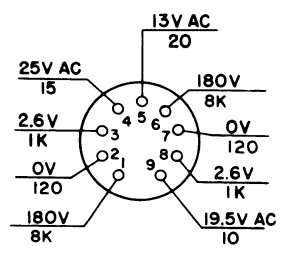
1ST MIXER V204 12AT7
