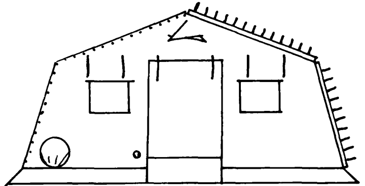
Figure 31. Endwall fabric
