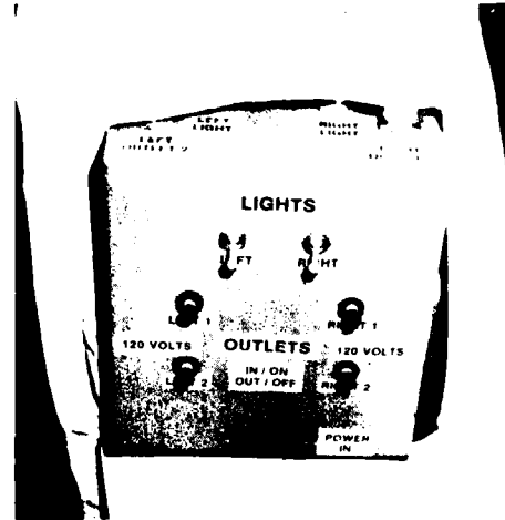
Figure 48. Distribution box fits through hole in liner
