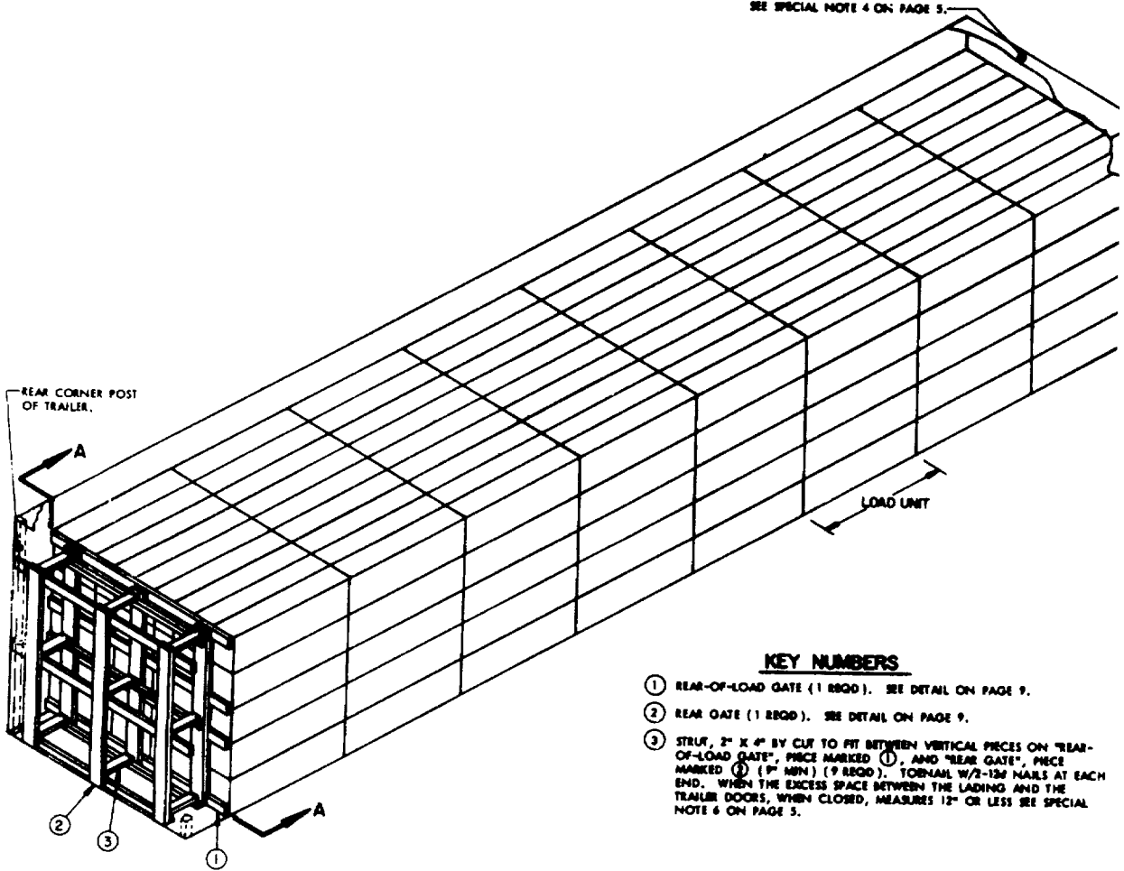
ISOMETRIC VIEW
