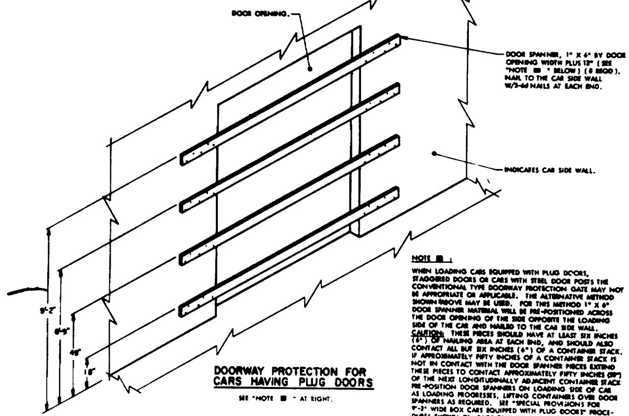
Figure 7-2--Continued (sheet 20 of 25)
