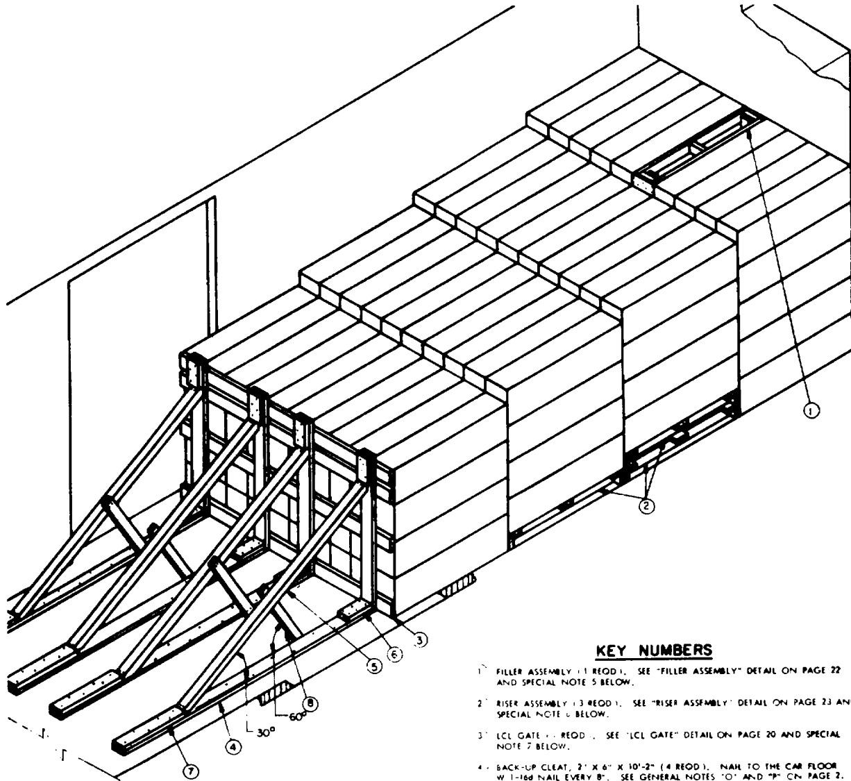
ISOMETRIC VIEW DEPICTING A 169 UNIT LCL LOAD.
