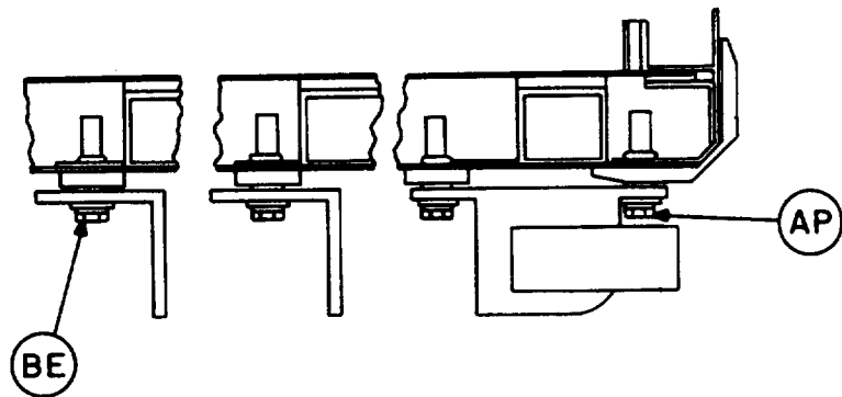
SECTION P-P
