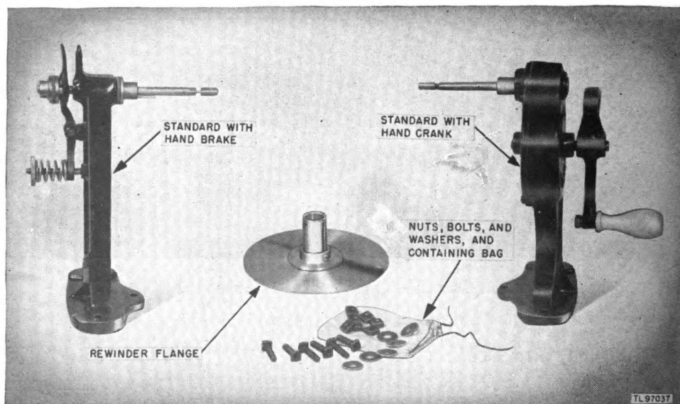
Figure 54. Rewinder PH-92.
