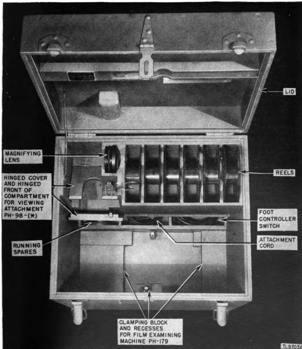
Figure 53. Case CS-77-(*) of Film Viewer PH-97-(*).
