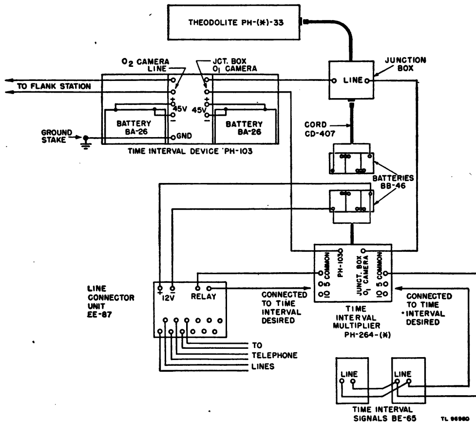
Figure 20. Cording diagram of battery station components of spotting components of Spotting Set PH-32-(*).
