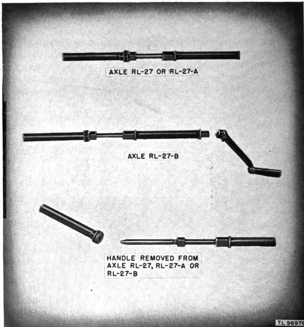
Figure 16. Axle RL-27-(*).
