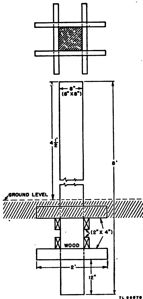
Figure 19. Wooden support for phototheodolite.
