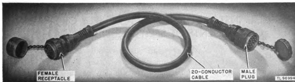
Figure 39. Cord CX-229/TVQ-1.
