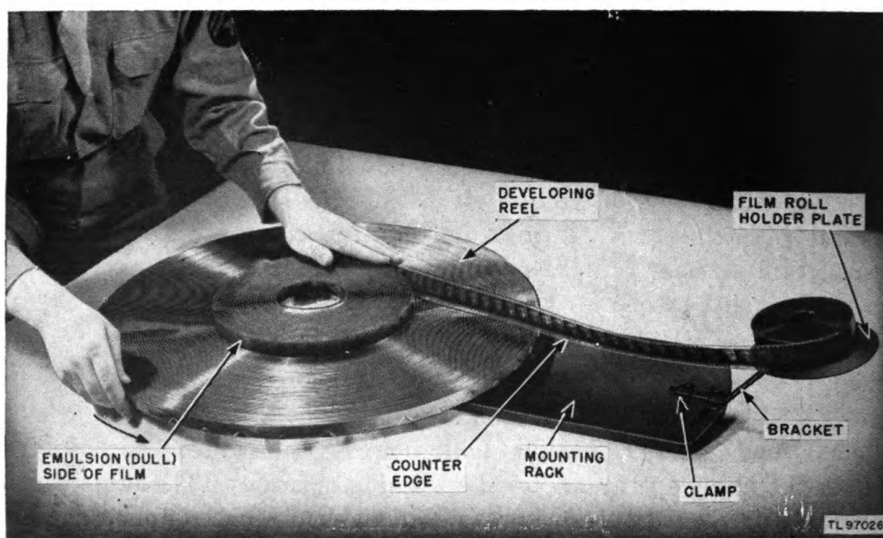
Figure 46. Loading film on developing reel.
