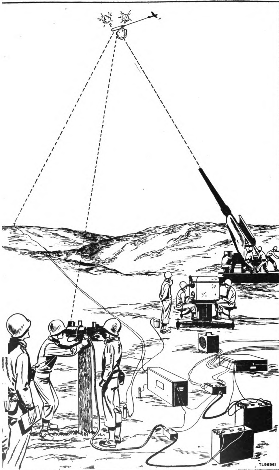
Figure 1. Spotting Set PH-32-B, PH-32-C, PH-32-D, or PH-32-F in use. The battery station phototheodolite with associated equipment is shown in the foreground, with the gun director and anti-aircraft gun shown in the middle right. The flank station, 4,000 to 5,000 yards distant, is shown in the left background. The broken lines indicate the theodolite lines of sight and the gun line of fire to the target.
