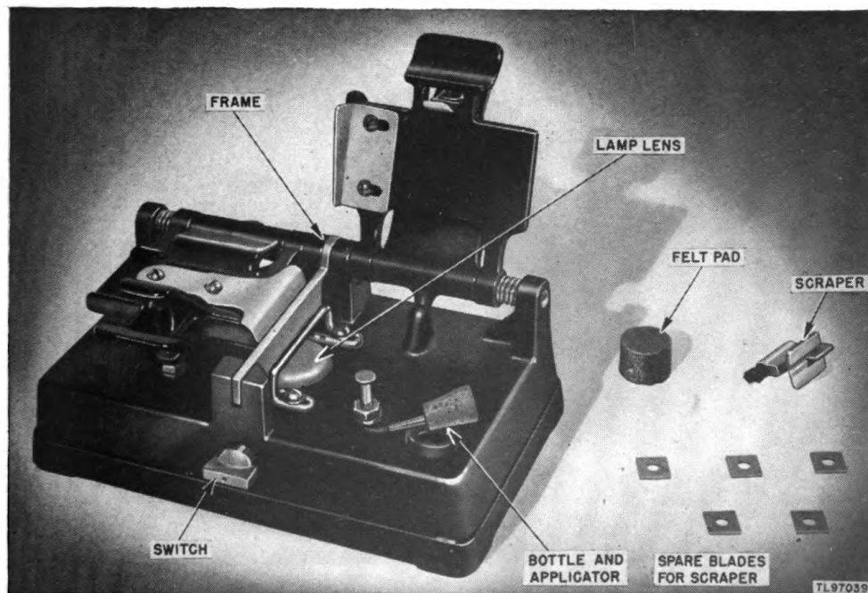
Figure 56. Splicer PH-91-A.
