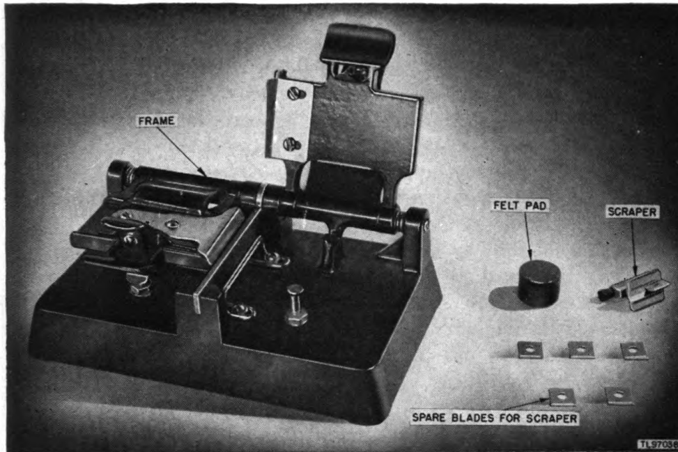
Figure 55. Splicer PH-91.
