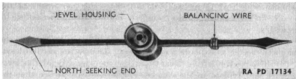
FIGURE 10.—Magnetic needle, assembly.
