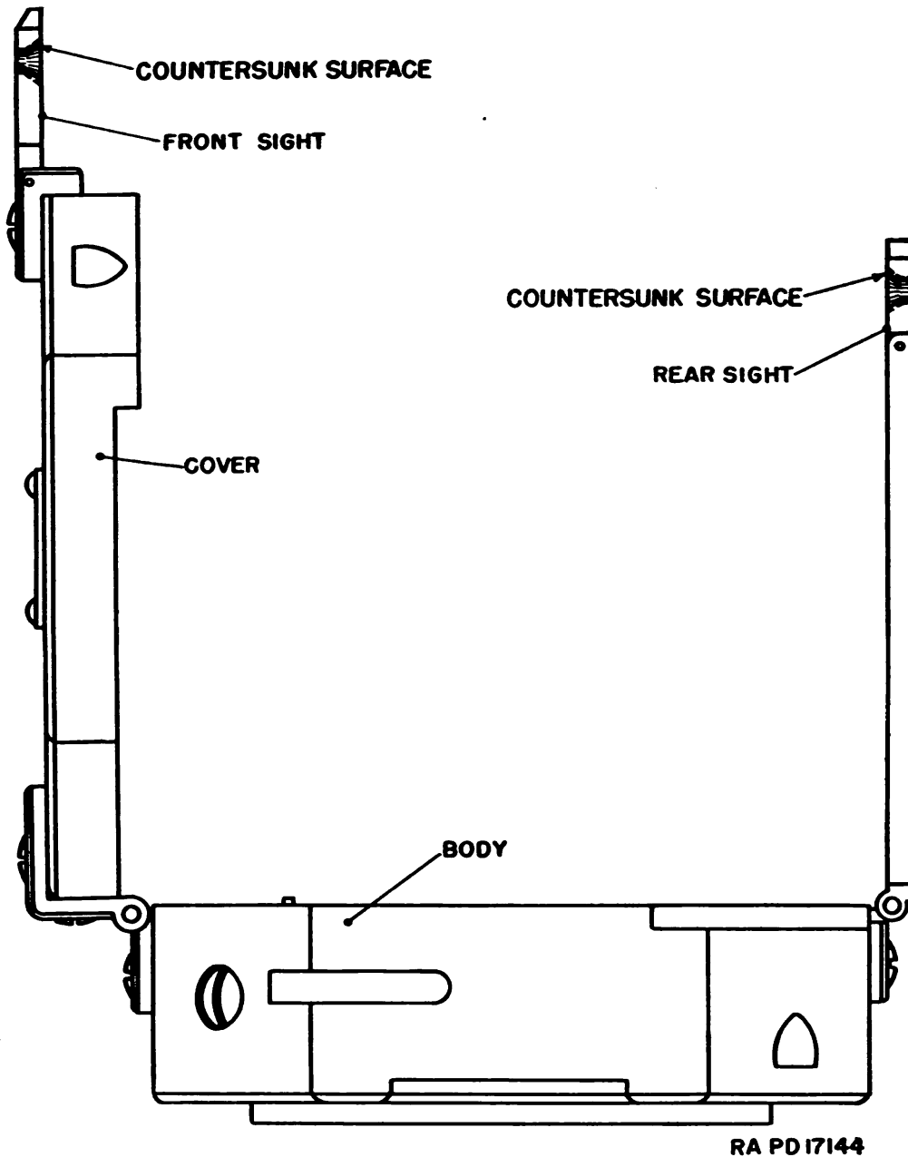
FIGURE 17.—Location of countersunk surfaces of front and rear sights.
