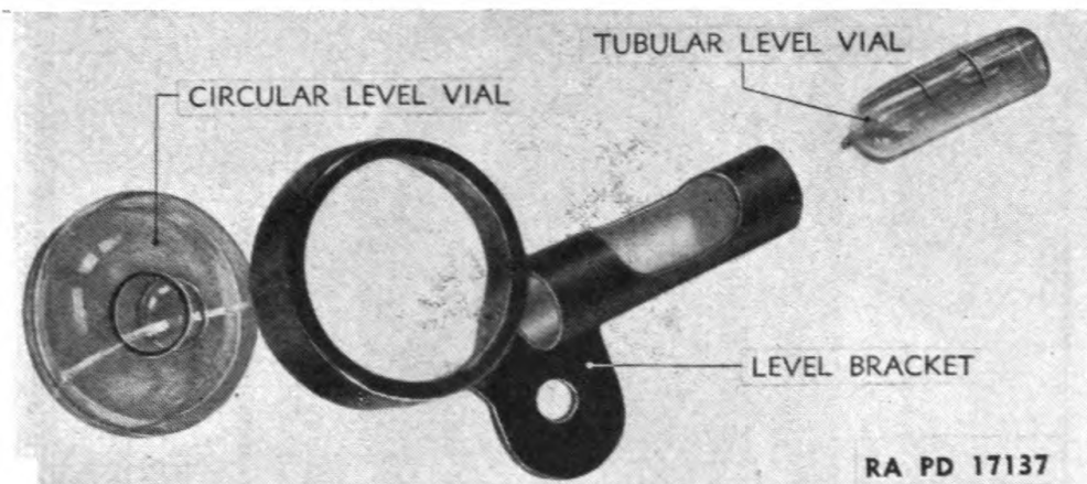
FIGURE 15.—Disassembly of level vials.
