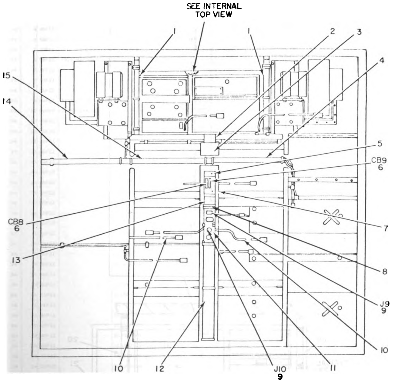
TOP VIEW
