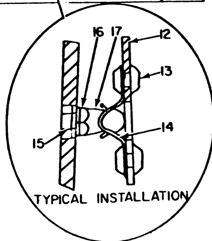
- Figure 10. Power and Signal Entrance Cover Assembly (Sheet 2 of 2).
