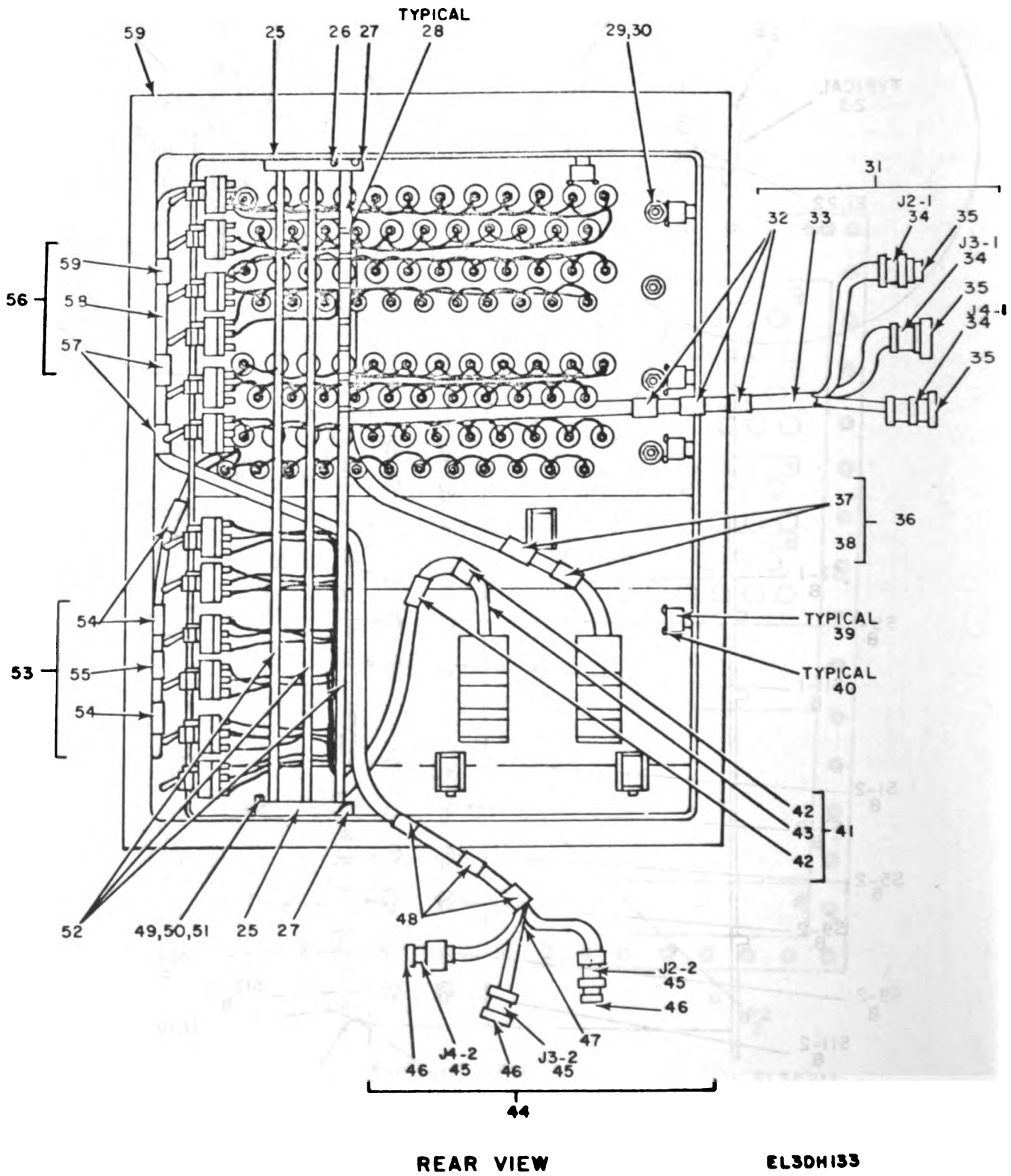
Figure 90. Signal Entrance Box, Roadside System 2 (Sheet 3 of 3).
