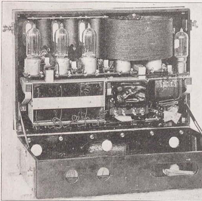
FIG. 2. Mounting of Apparatus in SCR-68 Set Box.
