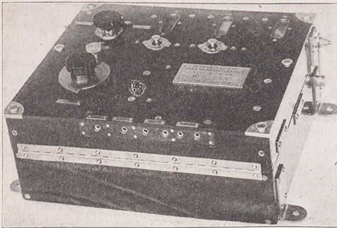
FIG. 6. Operating Panel of SCR-59 Receiving Set Box
