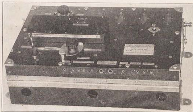
FIG. 1. Operating Panel of SCR-68 Radio Telephone Set.
