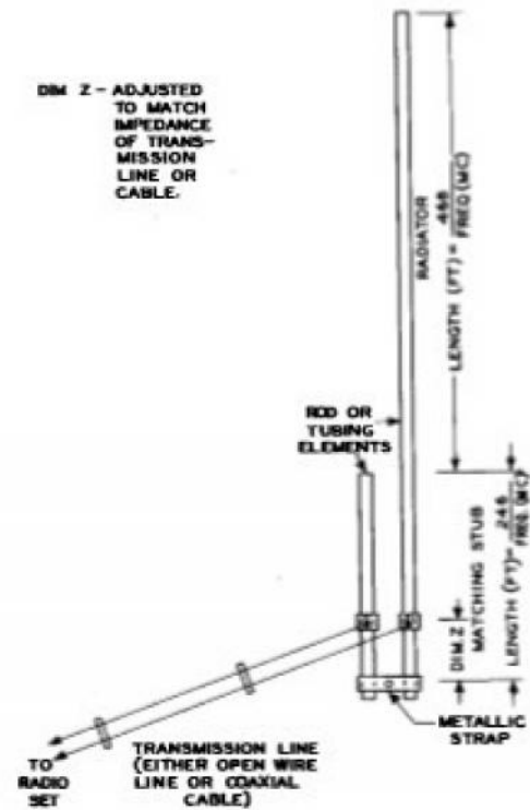
FIGURE 1465. Half-wave J Antenna
