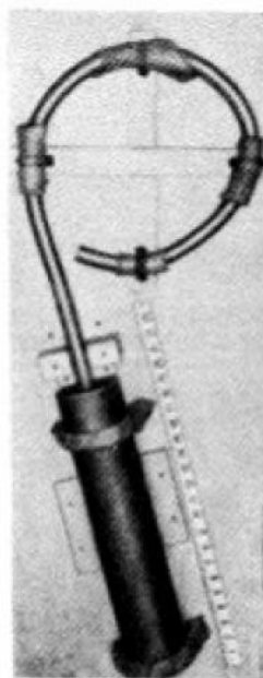
FIGURE 606. Loading Coil Case 124C (Western Electric Co.)
