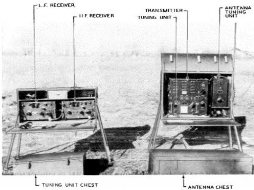
FIGURE 1404. Radio Set SCR-177-B
