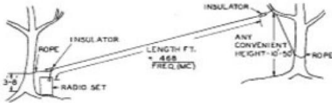
FIGURE 1466. Sloping Wire Antenna
