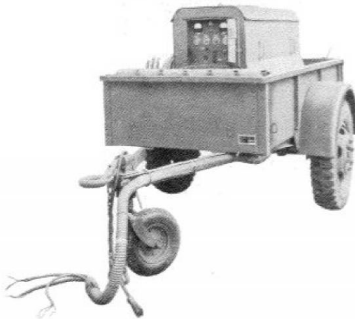
FIGURE 1203. Power Unit PE-95-( ) Part of Trailer K-52-( )
