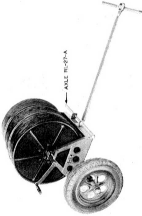
FIGURE 609. Reel Cart RL-35 and 3 Reels DR-4
