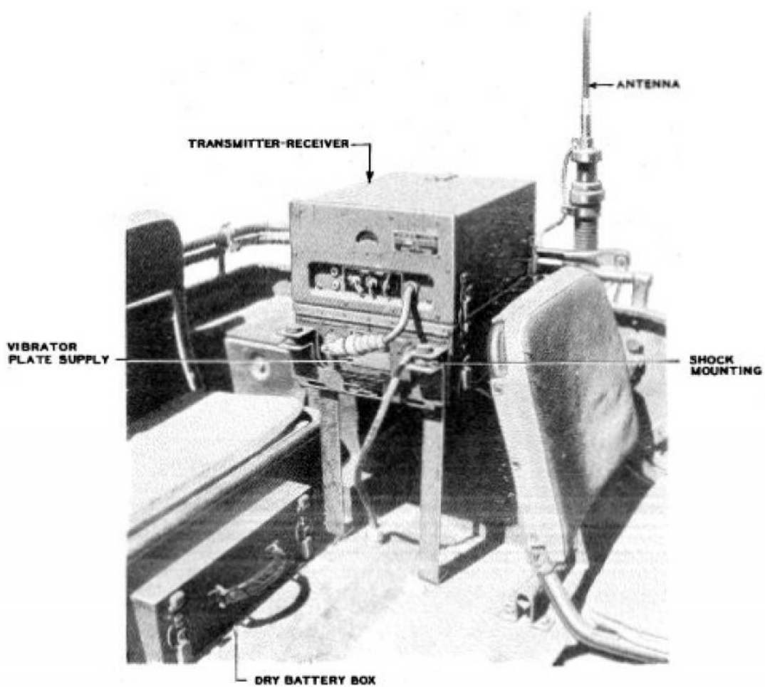
FIGURE 1428. Radio Set SCR-510
