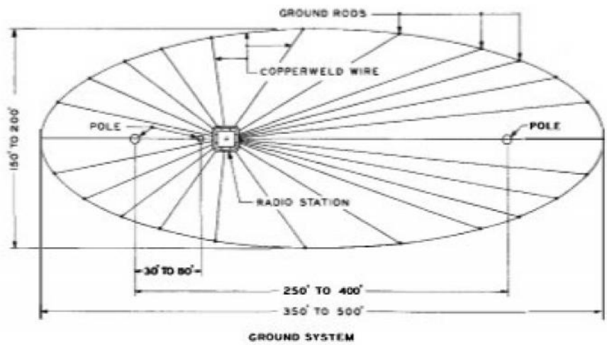
FIGURE 1538. Intermediate Frequency Flat Top Antenna
