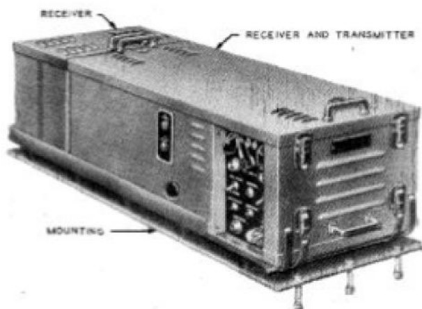
FIGURE 1418. Radio Set SCR-293
