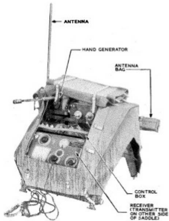
FIGURE 1412. Radio Set SCR-203
