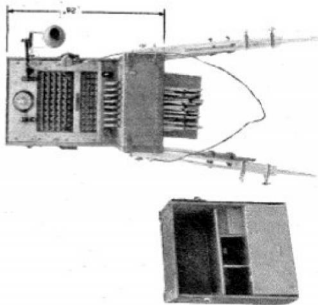
FIGURE 404. Switchboard BD-14
