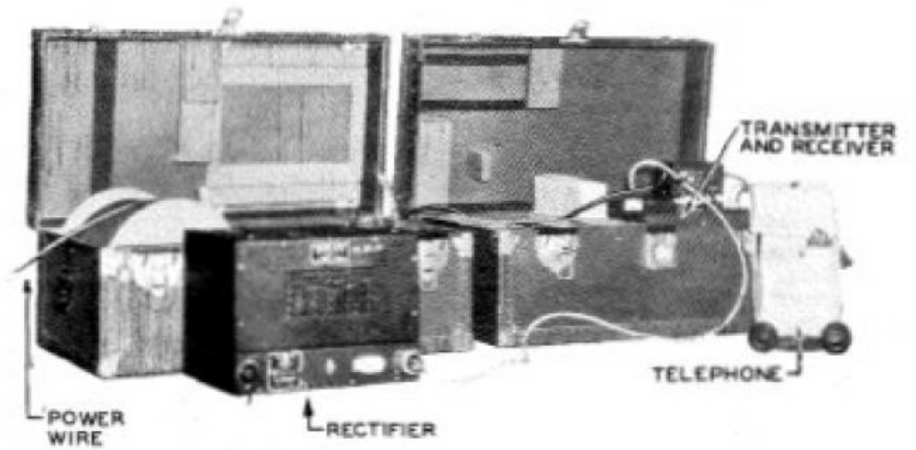
FIGURE 1439. Radio Set SCR-624
