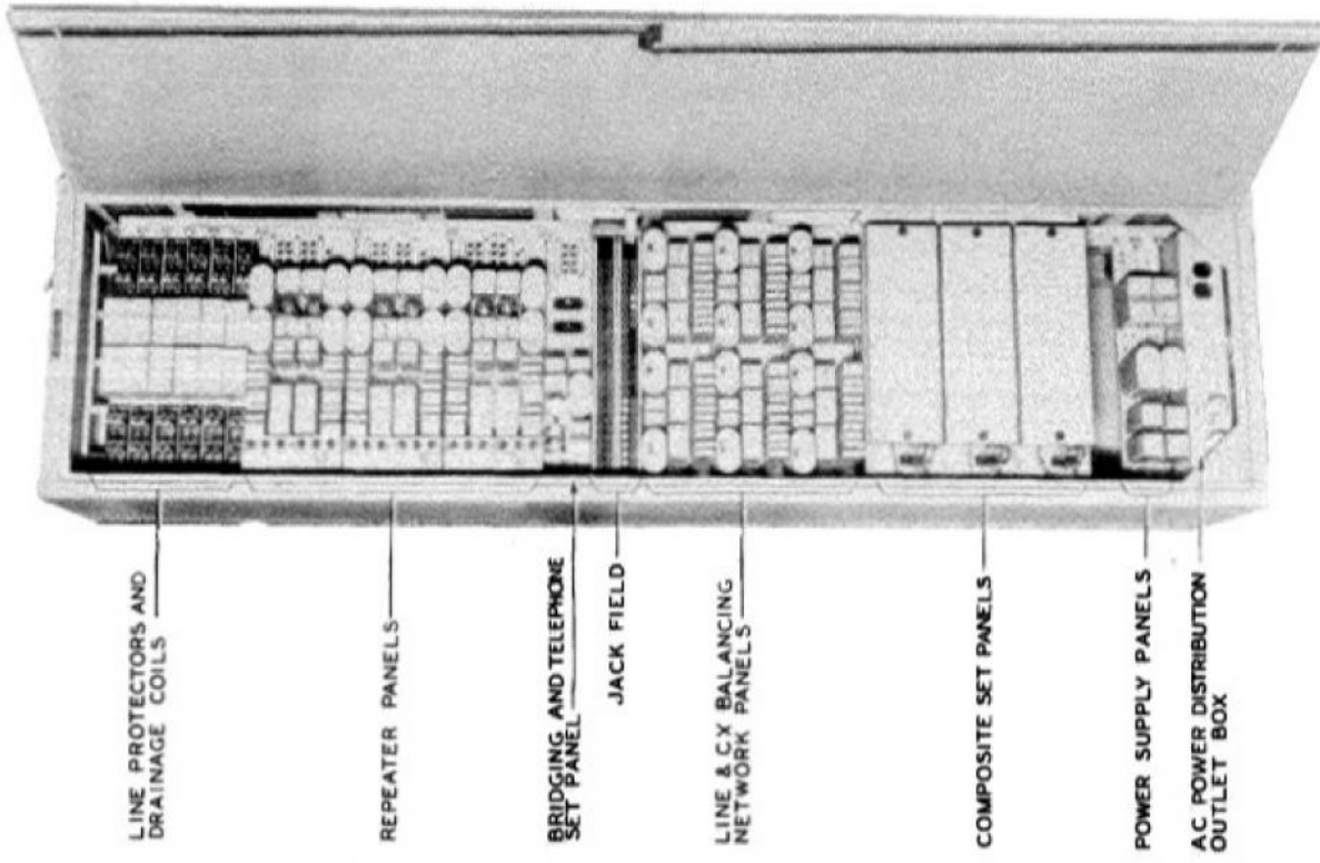
FIGURE 916. Repeater Package; Telephone; V.F. (Triple) X-61821K
