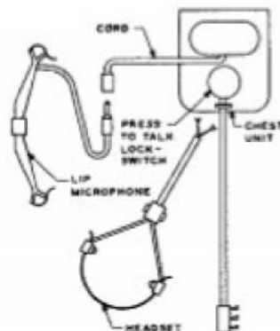
FIGURE 322. Chest Set TD-3
