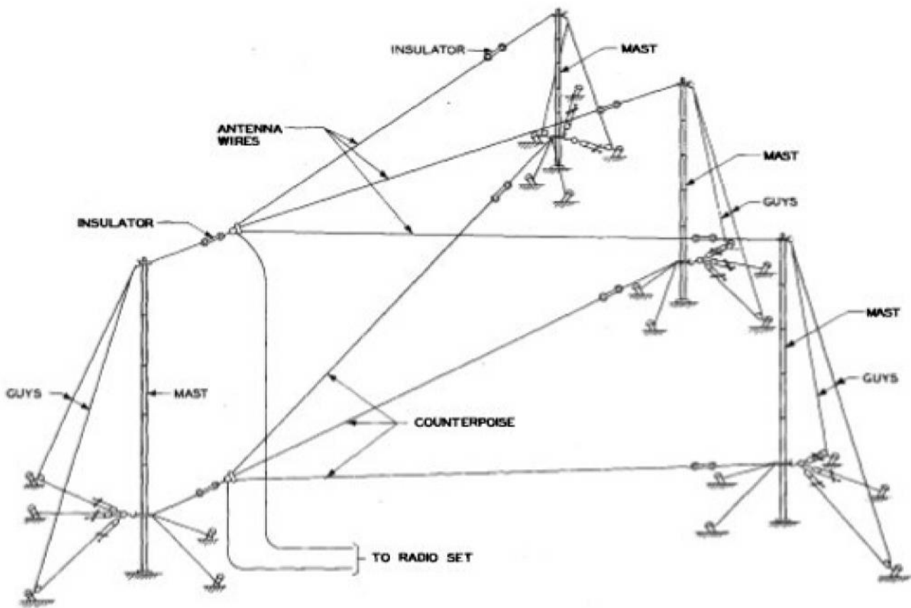
FIGURE 1459. Crowfoot Antenna
