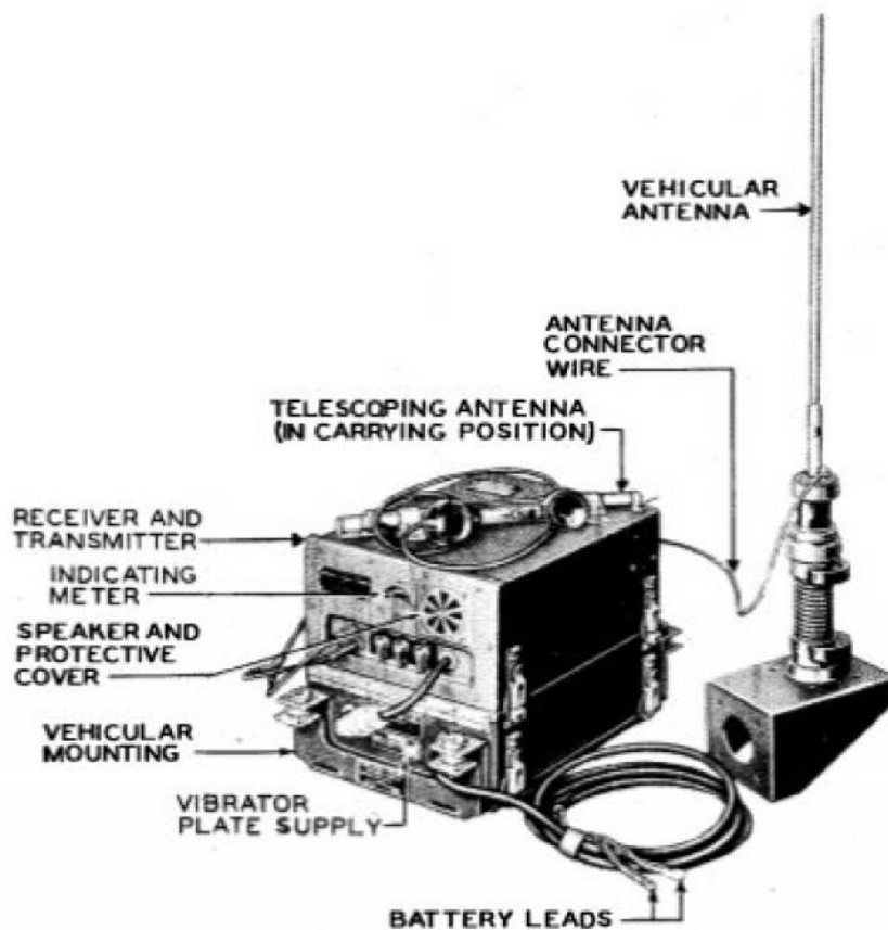
FIGURE 1437. Radio Set SCR-610
