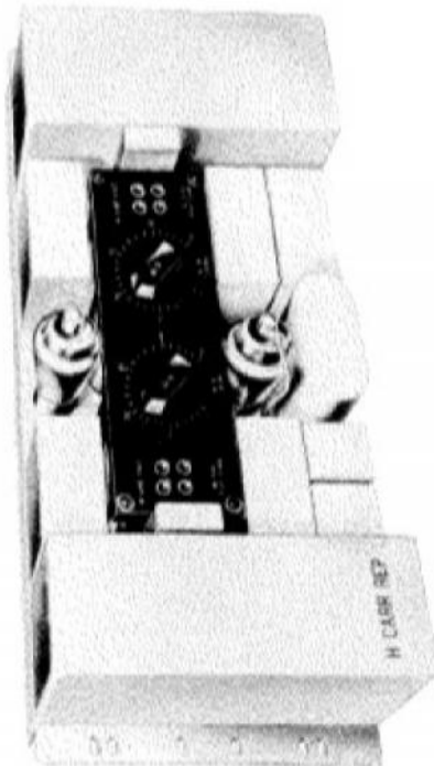
FIGURE 920. Repeater Package: Telephone; H Carrier X-66217B
