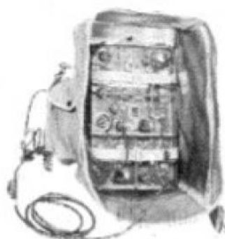
Receiver and Transmitter BC-1306
