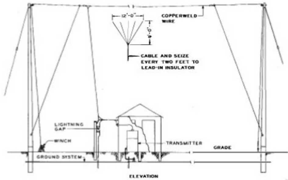
INTERMEDIATE FREQUENCY FLAT TOP ANTENNA
