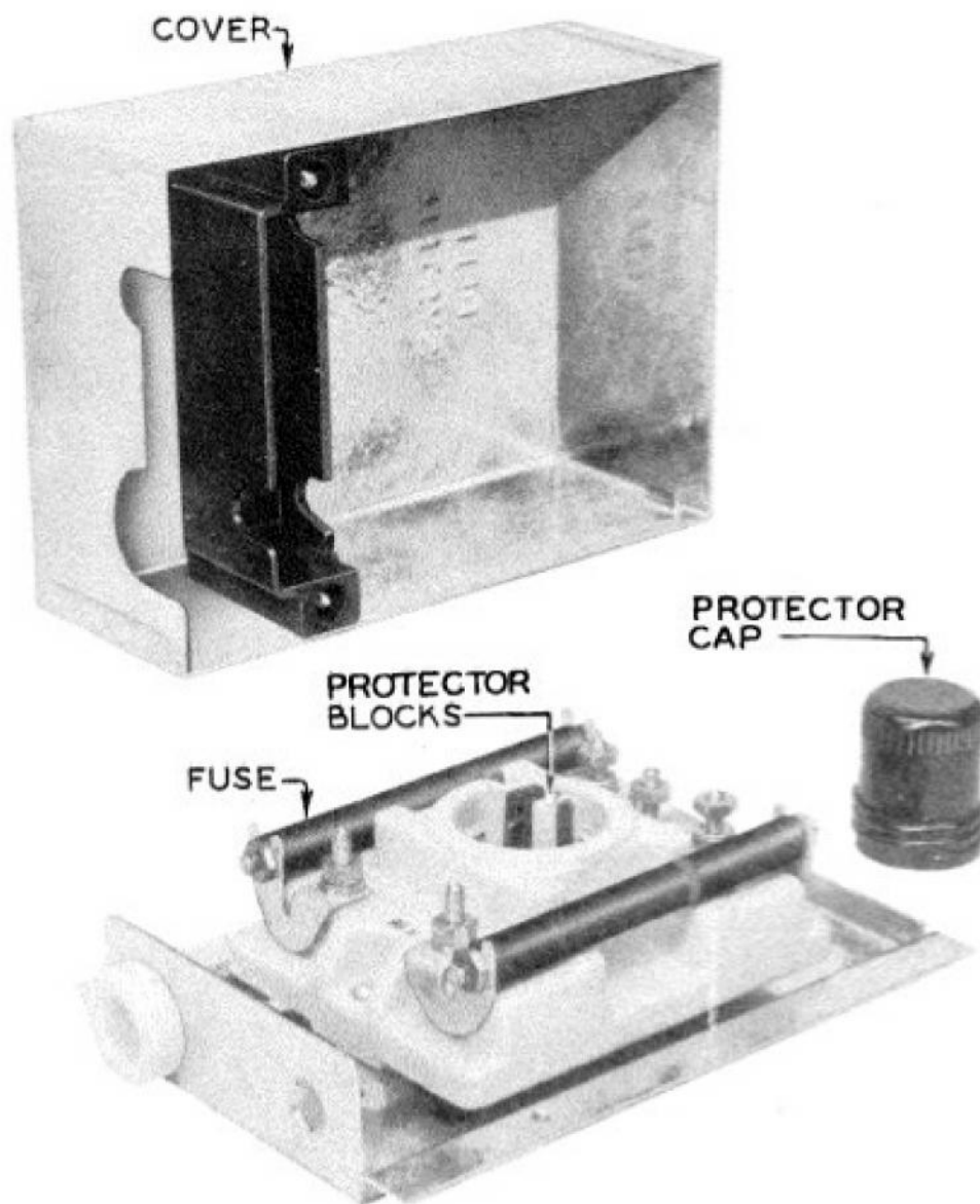
FIGURE 814. Telephone Protector (Western Electric Co. 1093A)
