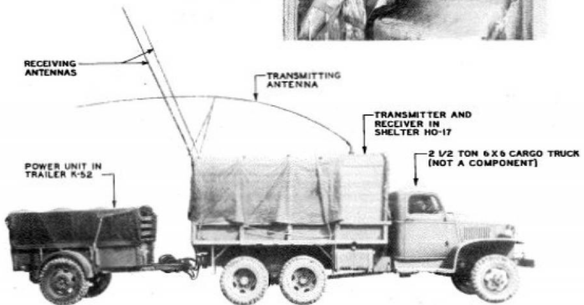
FIGURE 1423. Radio Set SCR-399
