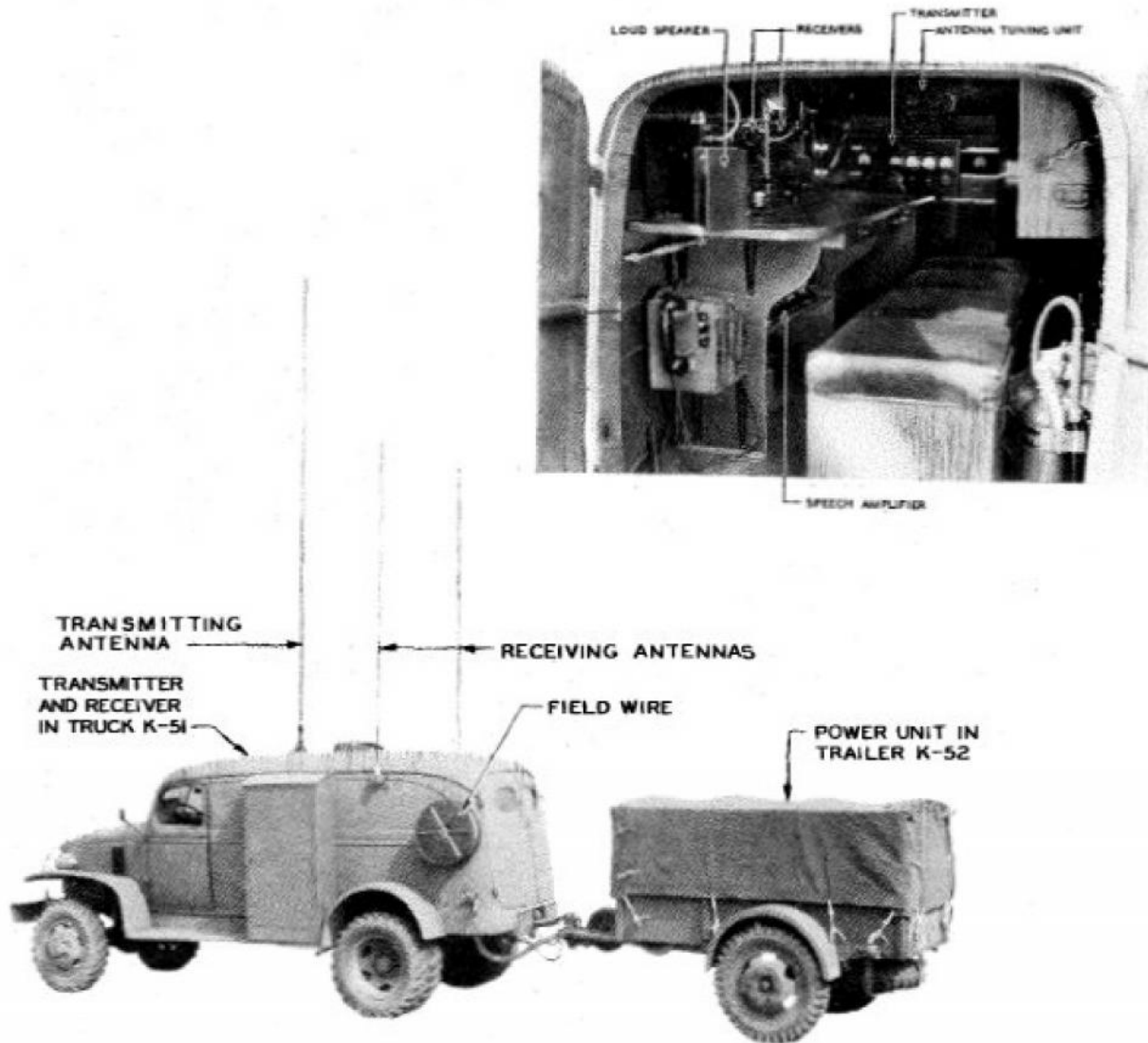
FIGURE 1421. Radio Set SCR-299
