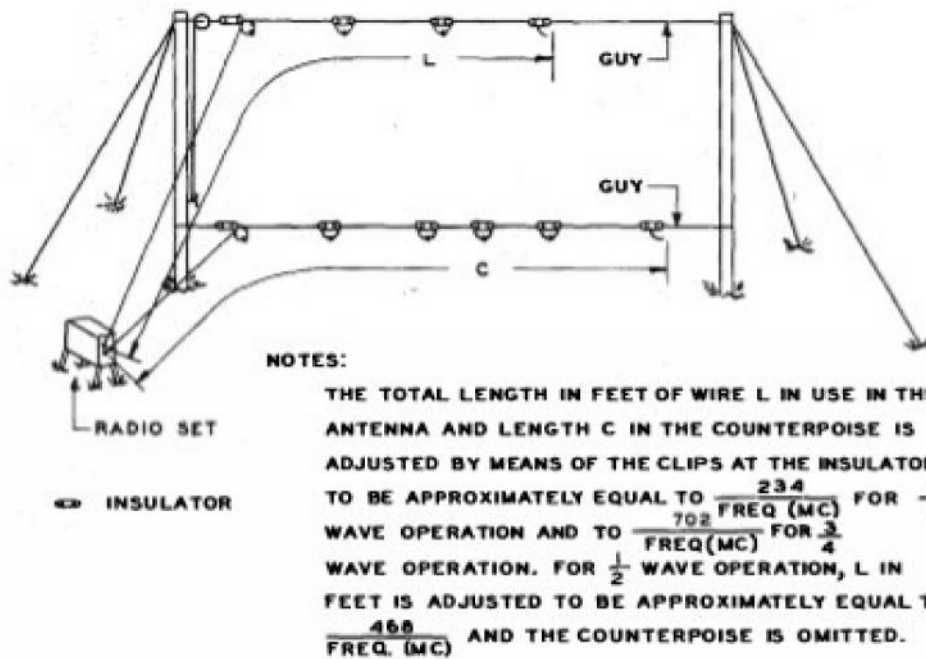
FIGURE 1458. Inverted L Antenna
