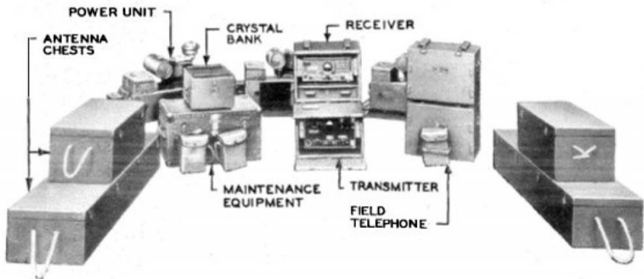
FIGURE 1451. Radio Terminal Set AN/TRC-3
