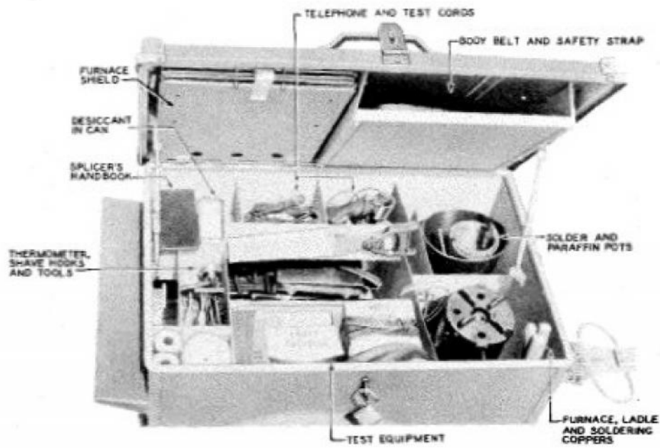
FIGURE 619. Trailer K-38 With Cable Splicer's Tool Equipment TX-56
