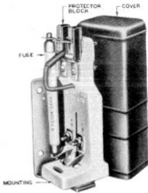
FIGURE 810. Telephone Protector (Cook 0-9)
