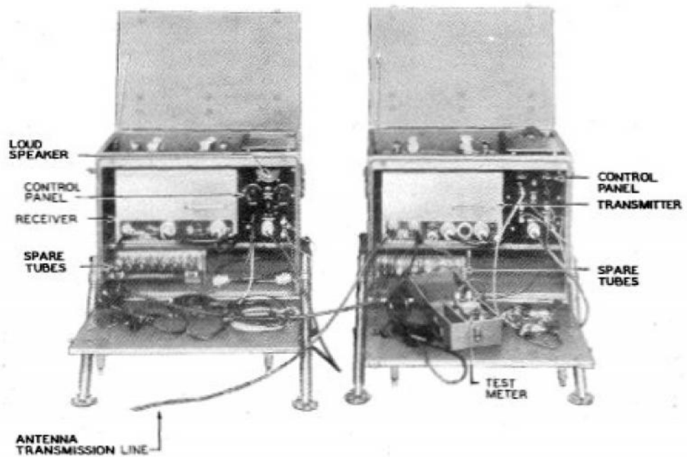
FIGURE 1447. Radio Set AN/CRC-3
