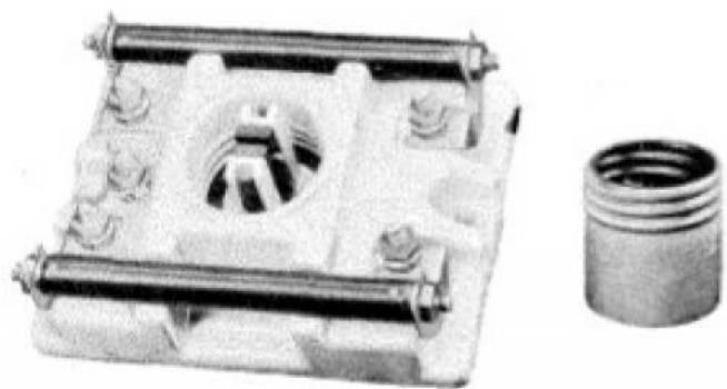
FIGURE 813. Telephone Protector (Western Electric Co. 98A)
