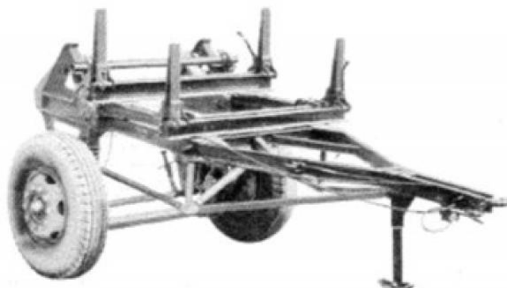
FIGURE 618. Trailer K-37
