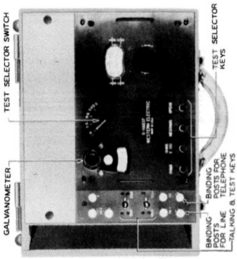
FIGURE 1313. Test Set TS-27/TSM
