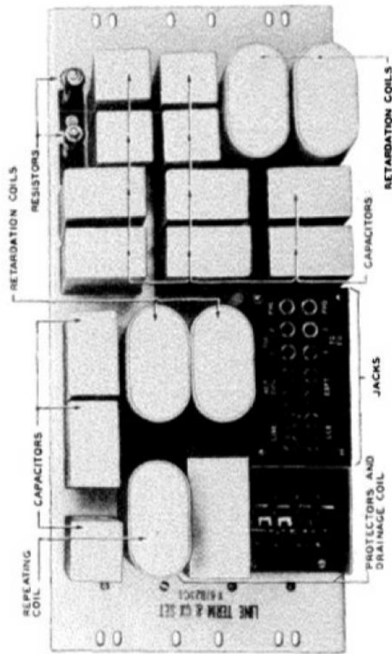
FIGURE 914. Panel; Line Terminating and Composite; Telephone X-61823C
