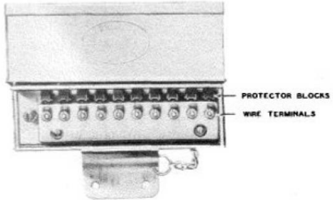
FIGURE 818. Cable Protector (Reliable 222)
