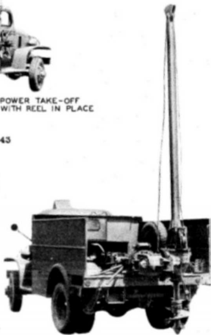
FIGURE 621. Truck K-44-B
