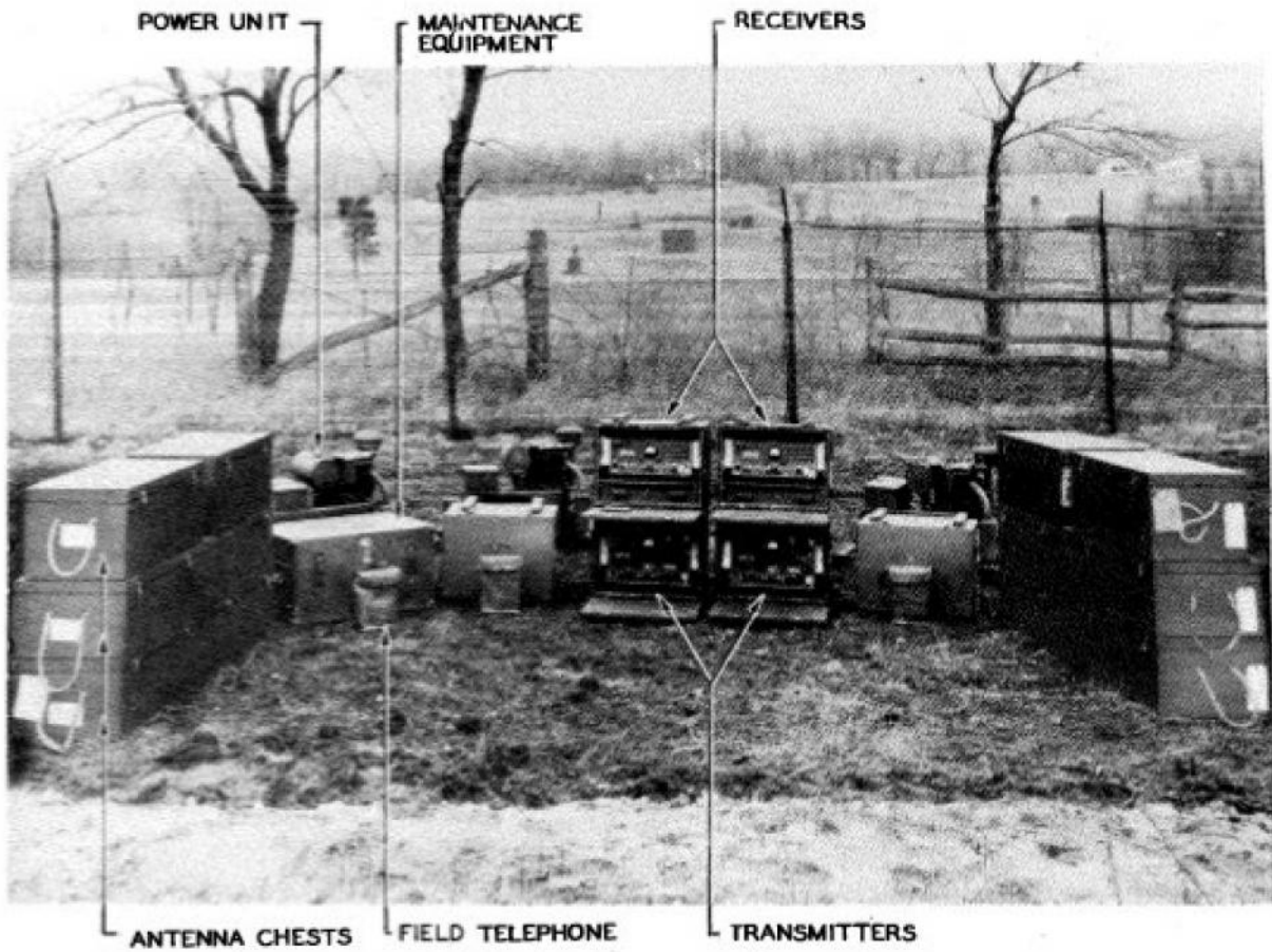
FIGURE 1452. Radio Relay Set AN/TRC-4
