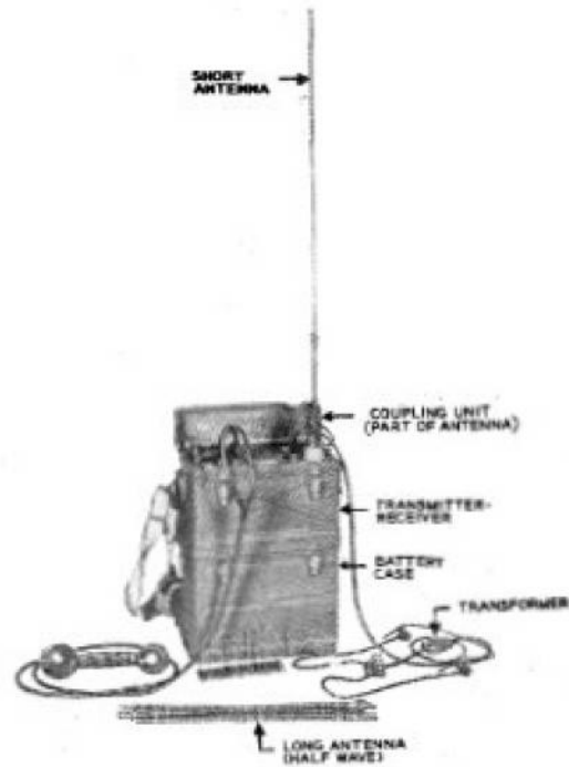
FIGURE 1422. Radio Set SCR-300
