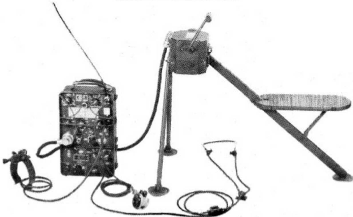
FIGURE 1441. Radio Set SCR-694-AW (Receiver removed from case)
