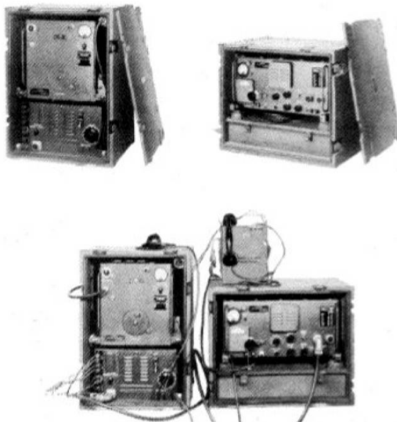
FIGURE 1455. Radio Terminal Set AN/TRC-11
