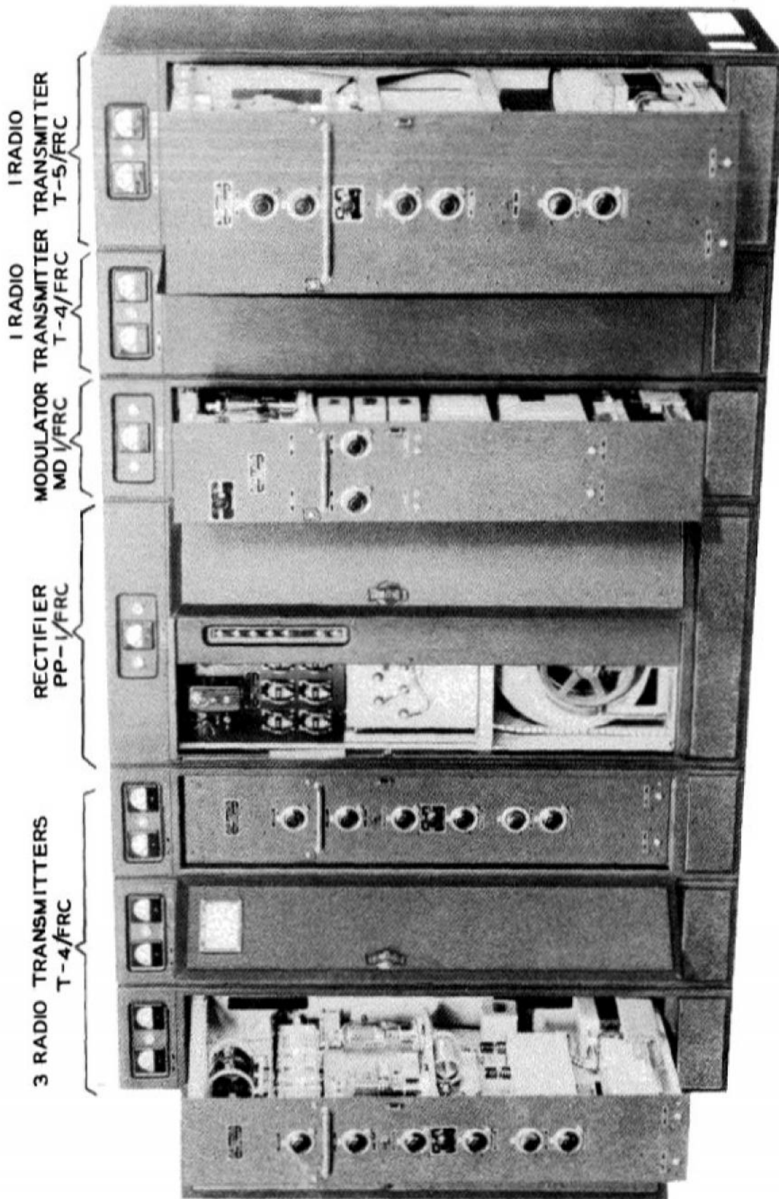
FIGURE 1505. Radio Transmitter T-4/FRC and T-5/FRC Installation
