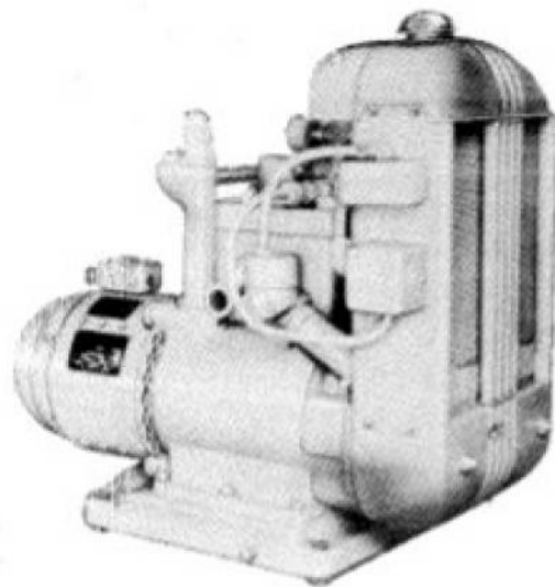
FIGURE 1229. Engine Generator (Onan W3M-13)
