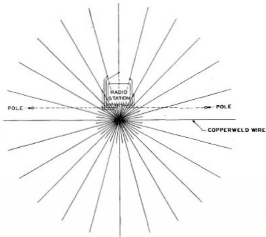
GROUND SYSTEM FOR DOUBLE CAGE ANTENNA INSTALLATION
