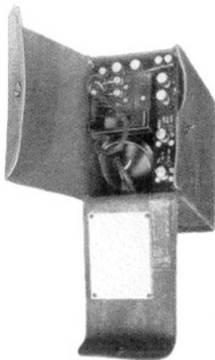
FIGURE 912. Telephone Unit EE-105
