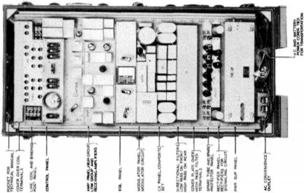
FIGURE 909. Converter CF-4-( )
