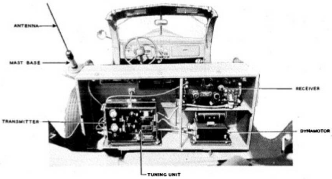
FIGURE 1415. Radio Set SCR-245
