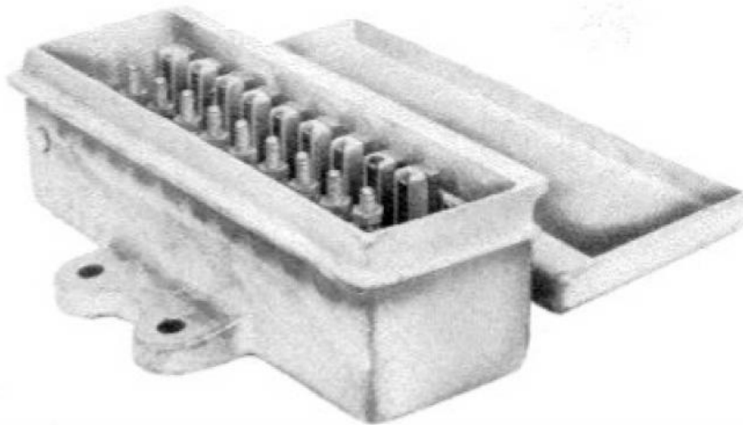
FIGURE 819. Cable Protector (Western Electric Co. 83A)
