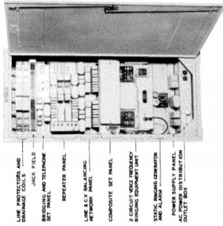
FIGURE 915. Repeater Package; Telephone; V.F. (Single) X-61821J
