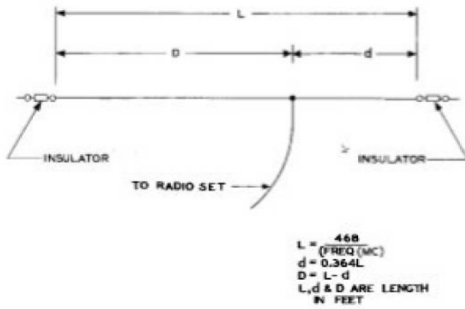
FIGURE 1464. Single Wire Fed Half-wave Antenna
