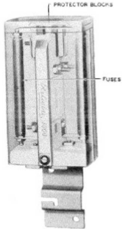
FIGURE 812. Telephone Protector (Reliable 1000)
