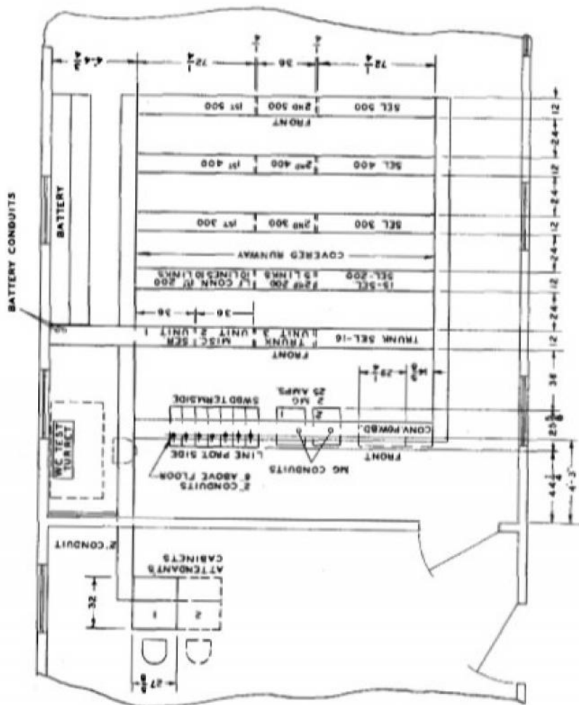
FIGURE 424. No. 1000 Switchboard - Floor Plan (North Electric Manufacturing Co.)
