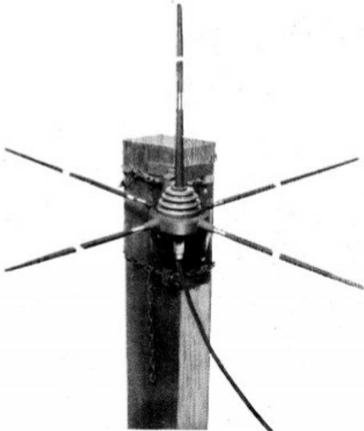
FIGURE 1472. Ground Plane Antenna
