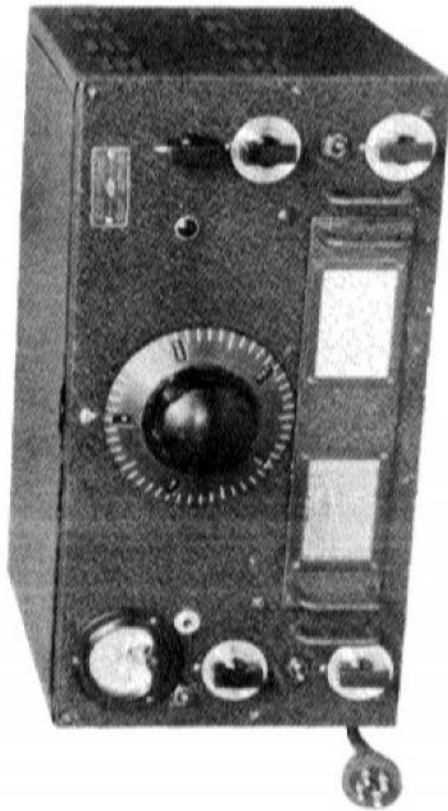
FIGURE 1526. Radio Receiver (National HR0)
