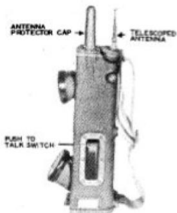
FIGURE 1431. Radio Set SCR-536
