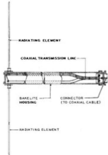
FIGURES 1467. Balanced Half-wave Dipole Antenna
