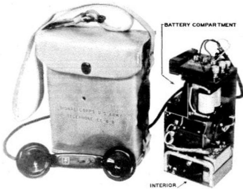
FIGURE 324. Telephone EE-8- ( )
