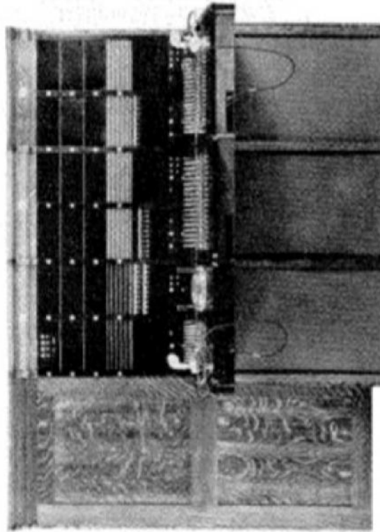
FIGURE 433. No. 12-1600 Switchboard (Kellogg Switchboard & Supply Co.)
