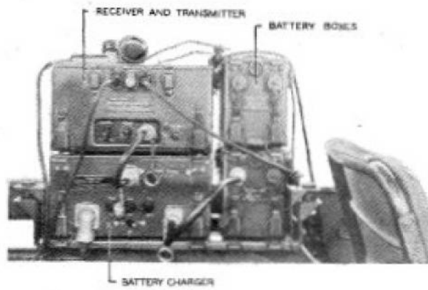
FIGURE 1438. Radio Set SCR-619
