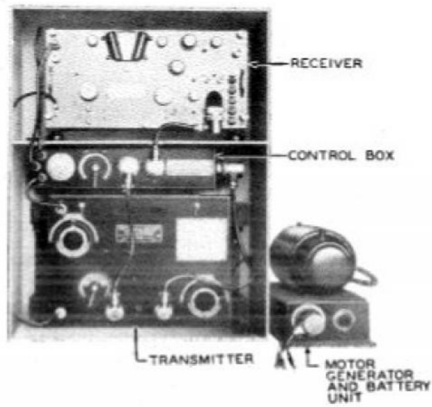
FIGURE 1413. Radio Set SCR-209
