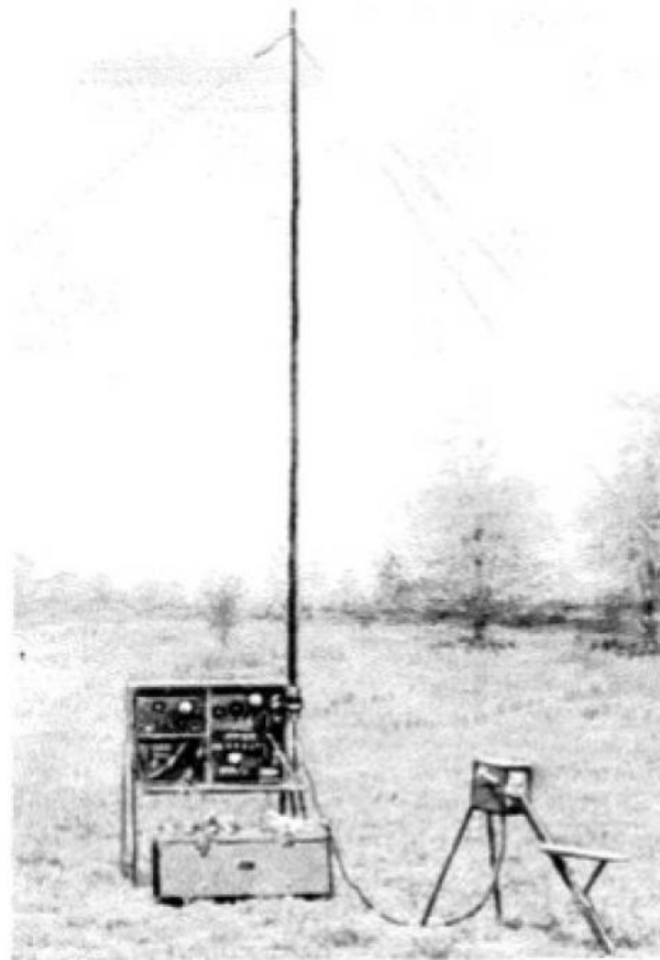
FIGURE 1405. Radio Set SCR-178 or 179
