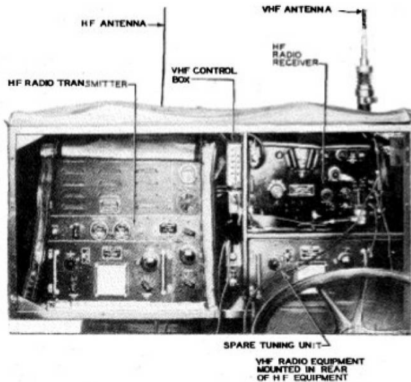
FIGURE 1457. Radio Set AN/VRC-1
