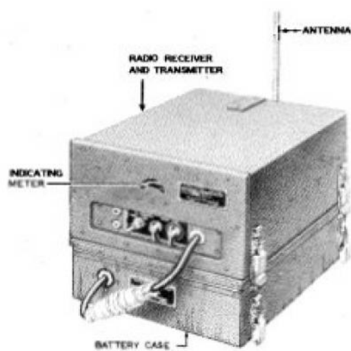
FIGURE 1427. Radio Set SCR-509
