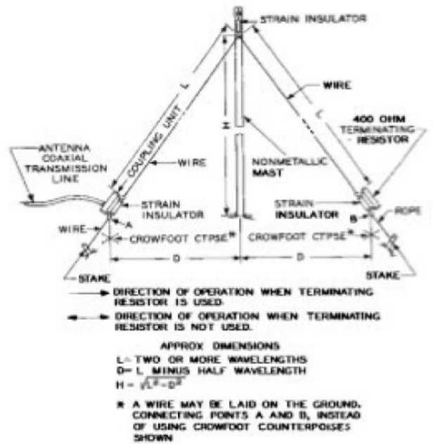
FIGURE 1469. Vertical Half Rhombic Antenna
