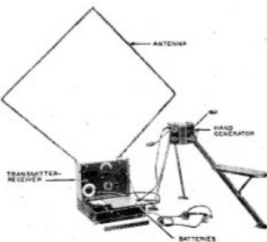
FIGURE 1401. Radio Set SCR-131 or 161
