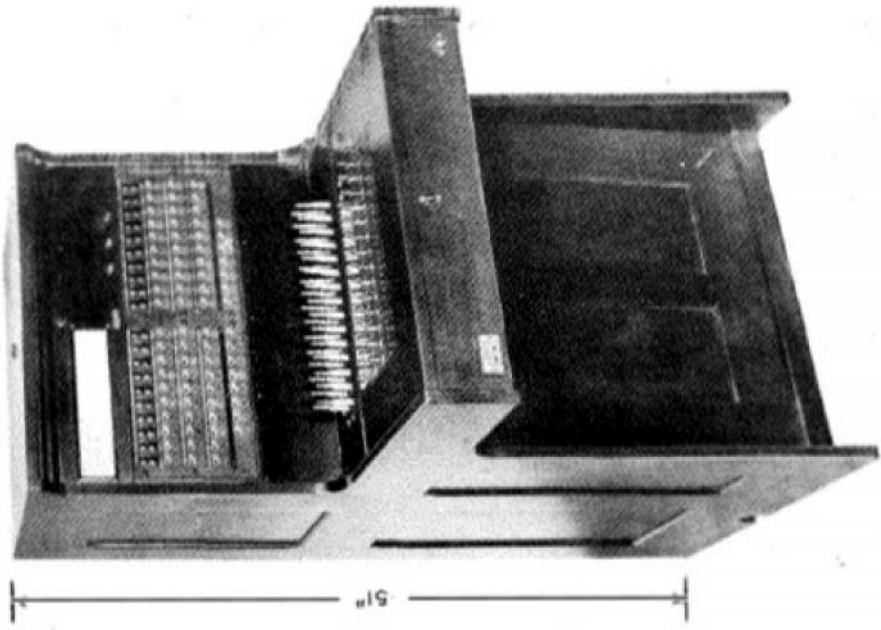
FIGURE 415. No. 550SC Switchboard (Modified) (Western Electric Co.)
