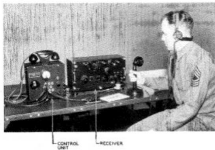
FIGURE 1407. Radio Set SCR-188-A
