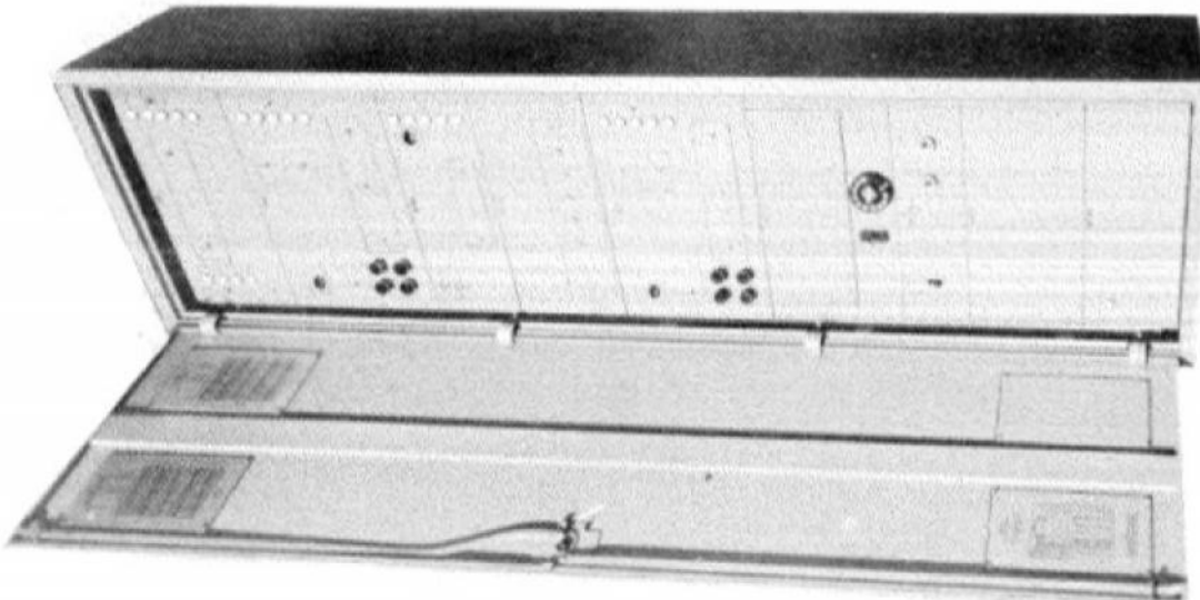
FIGURE 1493. Radio Receiver BC-779-( ) (Hammarlund Super Pro)
