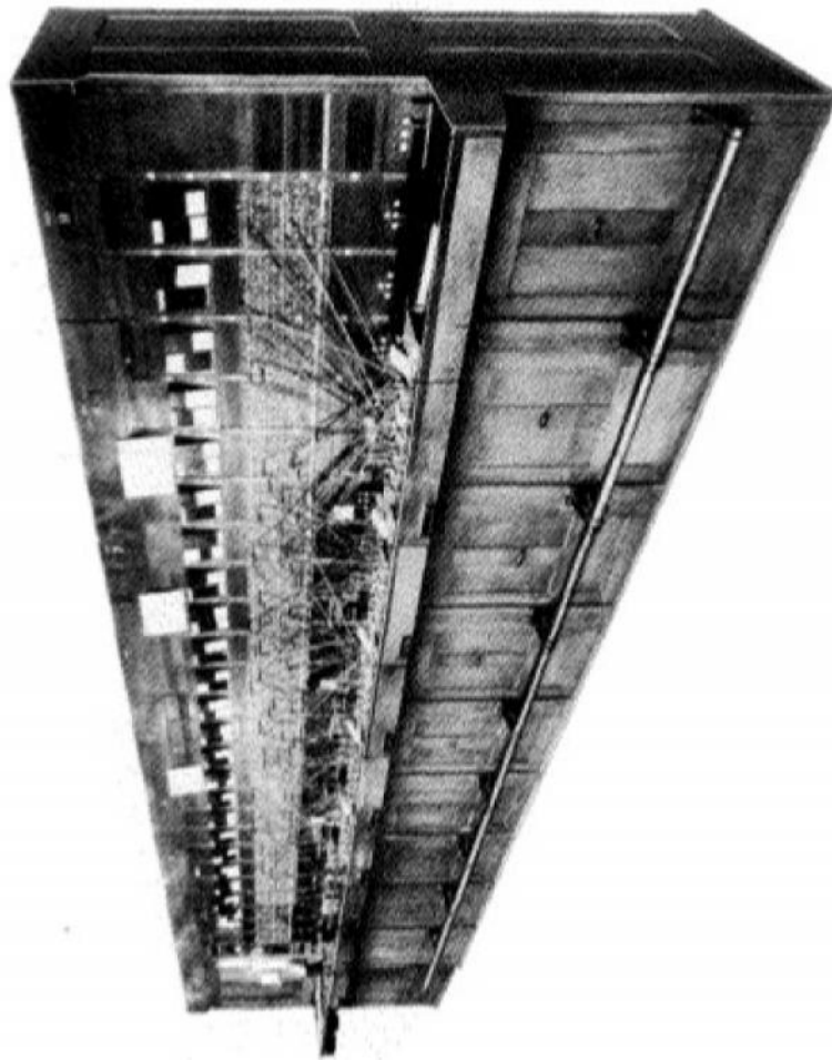
FIGURE 436. No. 11 Switchboard (Western Electric Co.)
