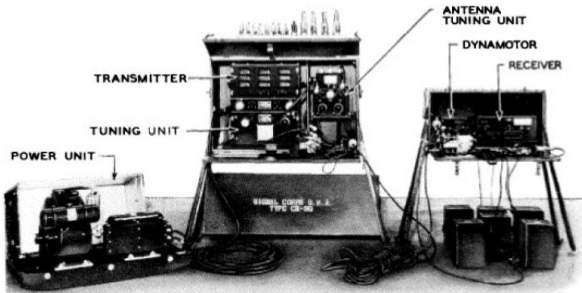
FIGURE 1406. Radio Set SCR-188
