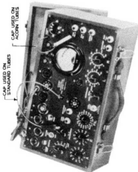
FIGURE 1307. Tube Tester I-177
