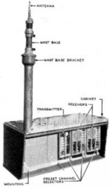
FIGURE 1426. Radio Set SCR-508
