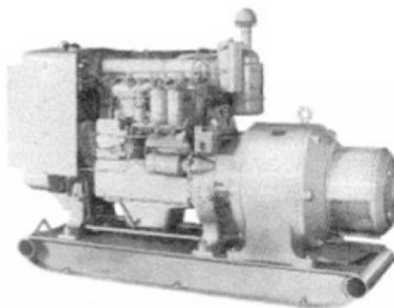
FIGURE 1215. Power Unit PE-85-M
