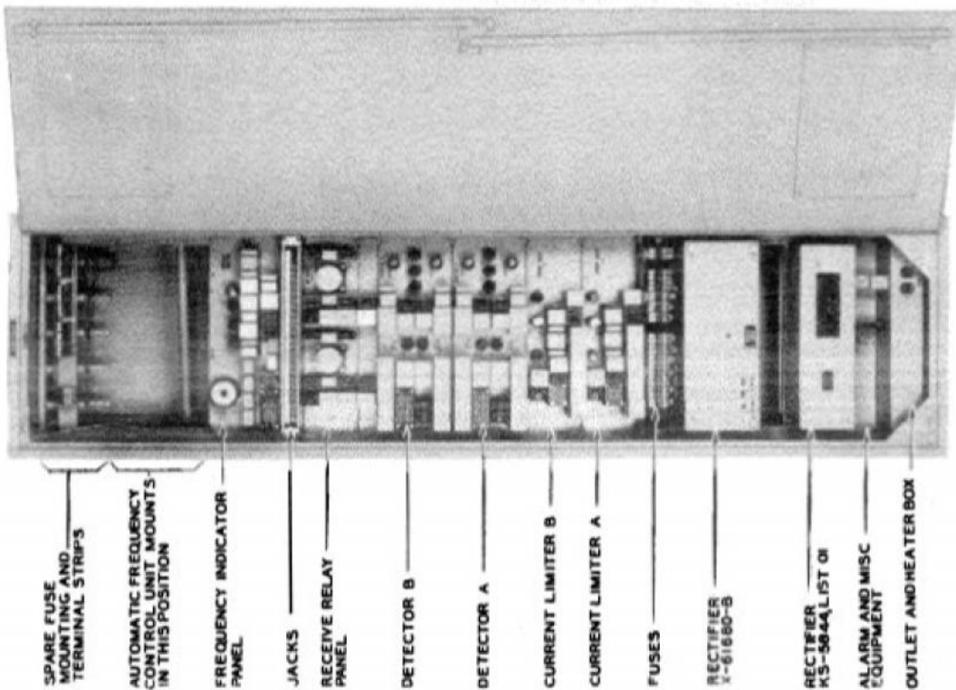
FIGURE 1022. Radioteletype Terminal Equipment AN/FGC-1
