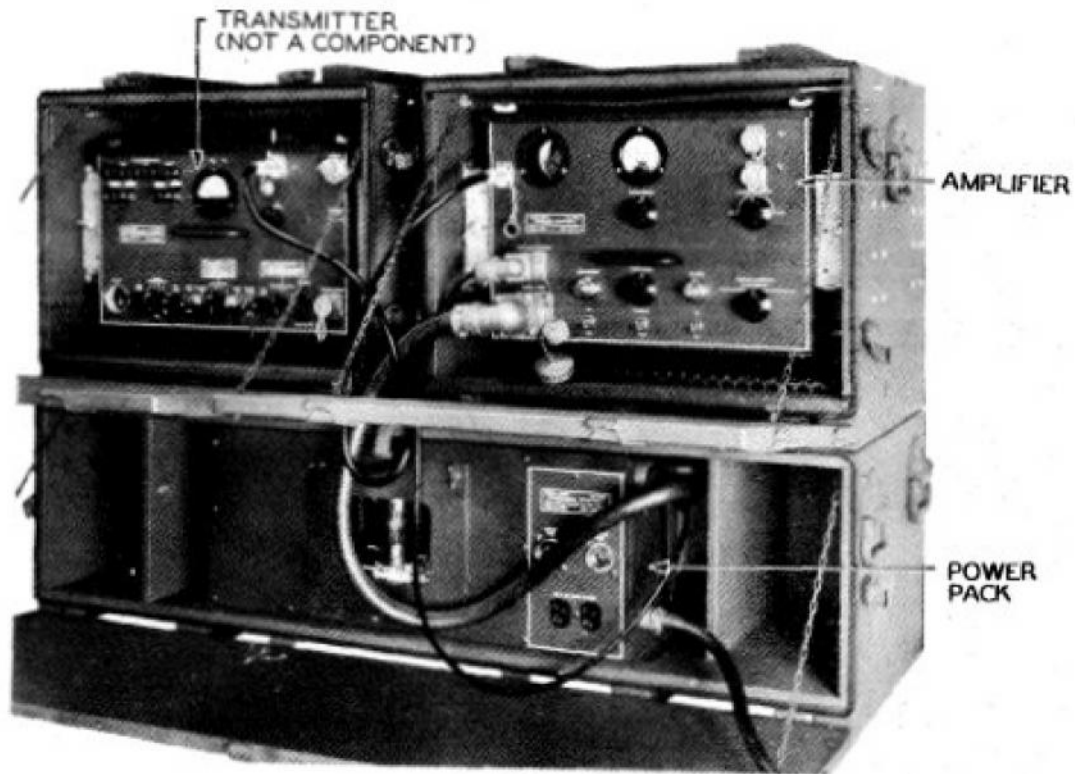
FIGURE 1448. Amplifier Equipment AN/TRA-1
