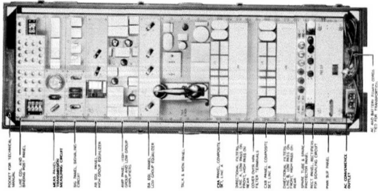
FIGURE 910. Repeater CF-5-( )
