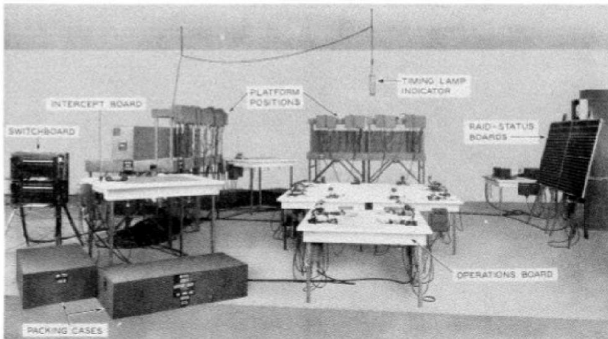
FIGURE 503. Operations Center AN/TTQ-1
