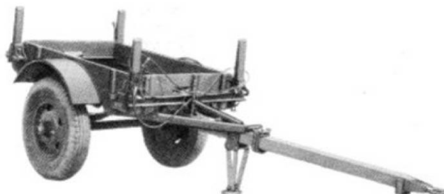
FIGURE 617. Trailer K-36
