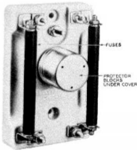
FIGURE 811. Telephone Protector (Reliable 955)
