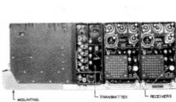
FIGURE 1443. Radio Set SCR-808
