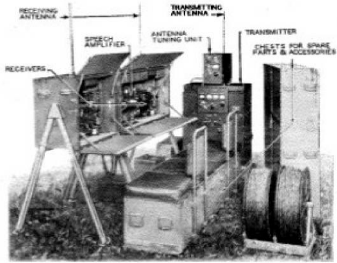
FIGURE 1424. Radio Set SCR-499
