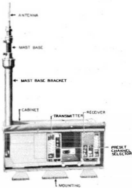
FIGURE 1440. Radio Set SCR-628
