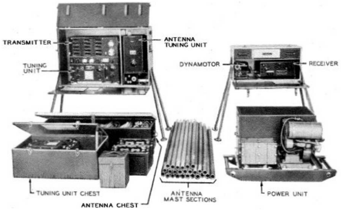
FIGURE 1403. Radio Set SCR-177-A
