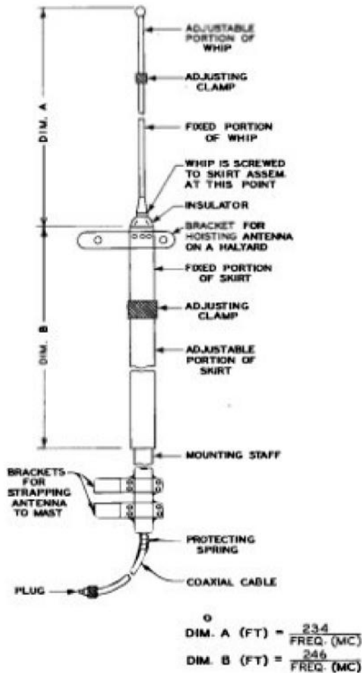
FIGURE 1468. Adjustable Coaxial Antenna
