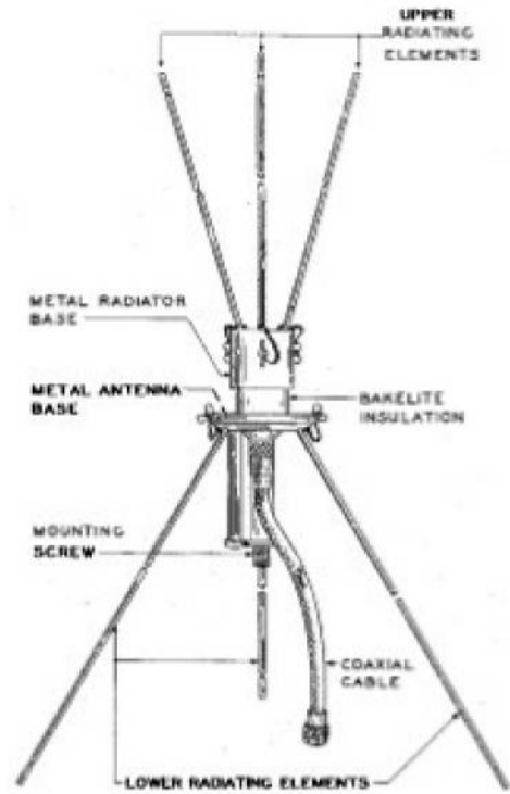
FIGURE 1471. Vertical Conical Dipole Antenna
