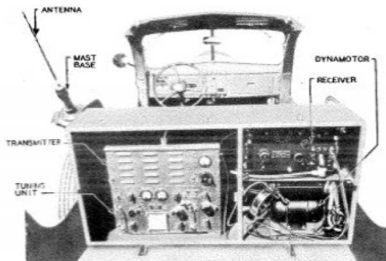
FIGURE 1408. Radio Set SCR-193-( )
