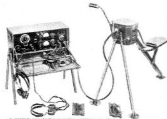
FIGURE 1417. Radio Set SCR-288
