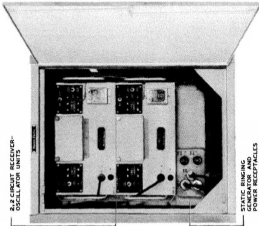
FIGURE 917. Ringer Package; Voice Frequency; 4 Circuit X-61820A
