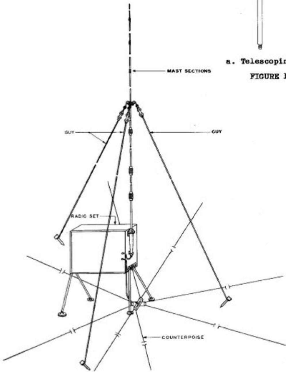
FIGURE 1460. Whip Antenna and Counterpoise
