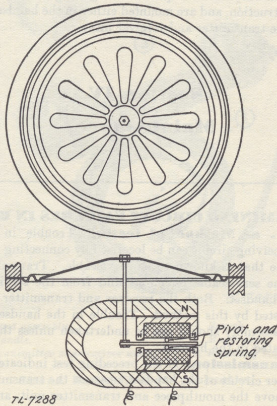
Figure 6. Schematic drawing of a sound-powered transmitter and receiver unit.
