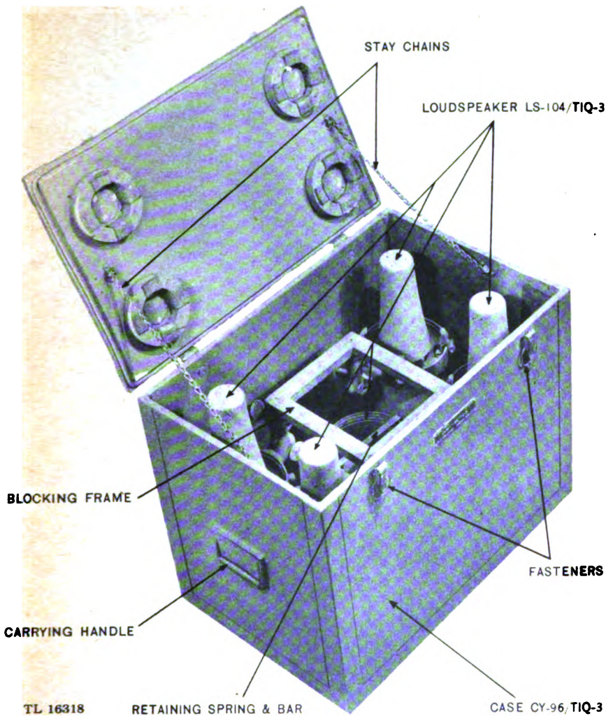
Figure 6. Case CY-96/TIQ-3 and Loudspeakers LS-104/TIQ-3.
