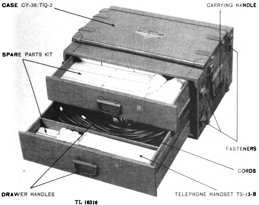
Figure 4. Spare parts Case CY-38/TIQ-2.
