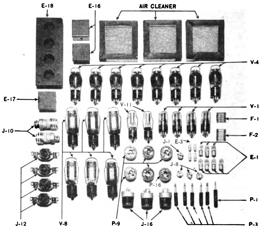
Figure 5. Spare parts for Public Address Set AN/TIQ-3.
