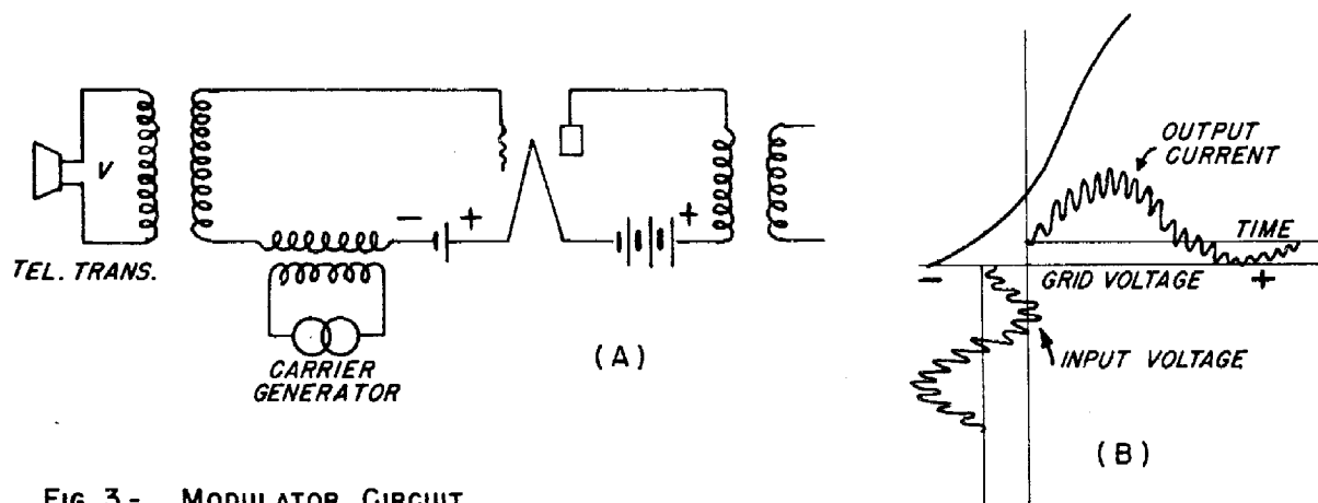
FIG. 3 - MODULATOR CIRCUIT
