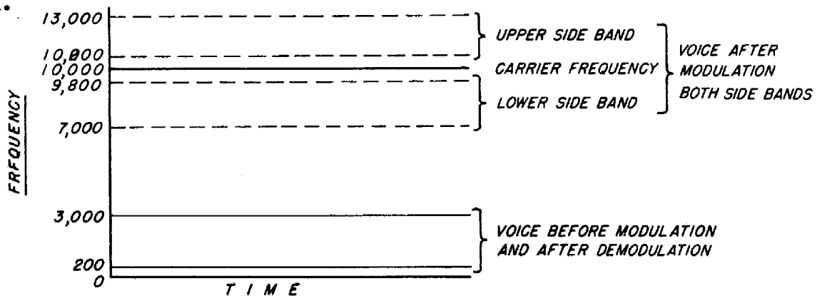
FIG. 4 - FREQUENCY CHANGES DURING MODULATION AND DEMODULATION
