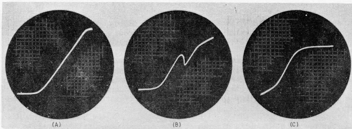
FIG. 4- CHARACTERISTIC CURVES SHOWN ON THE OSCILLOSCOPE SCREEN FOR (A) TRIODE, (B) TETRODE, AND (C) PENTODE.
