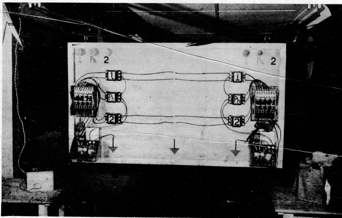
"INSTRUCTION BOARD" USED TO DEMONSTRATE EFFECT OF VARIOUS LINE TROUBLES UPON OPERATION OF TELEPHONE AND TELEGRAPH EQUIPMENT.
