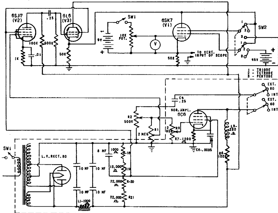
FIG. 2- SCHEMATIC DIAGRAM OF THE DEMONSTRATOR.
