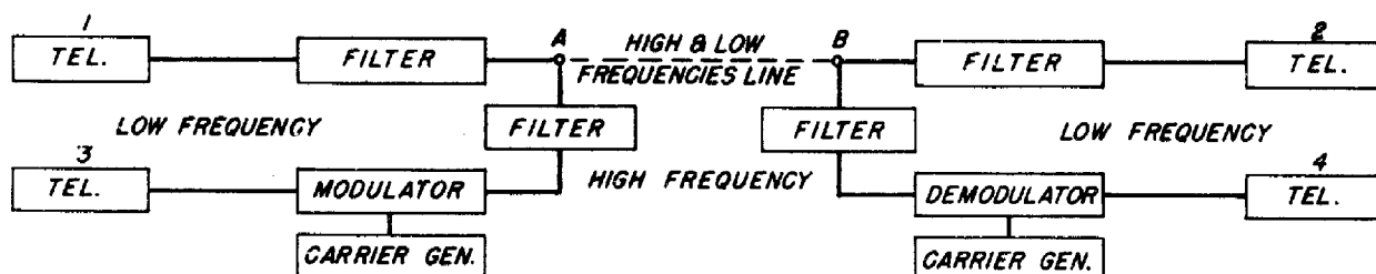
FIG. 1- SIMPLIFIED DIAGRAM OF SINGLE CHANNEL CARRIER SYSTEM
