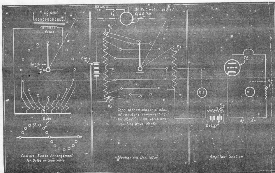
FIG. 2- SCHEMATIC DIAGRAM OF THE V.T. DEMONSTRATOR.
