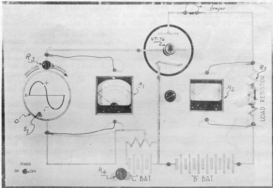
FIG. 1- THE V.T. DEMONSTRATOR.
