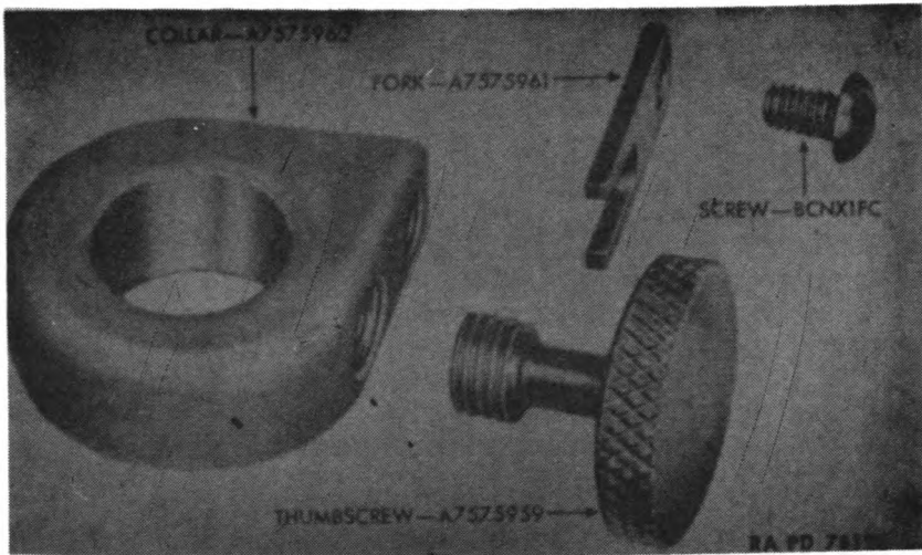
Figure 27—Tripod M15—Collar Assembly—Disassembled
