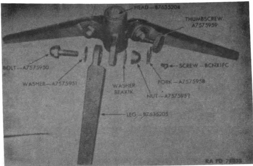
Figure 28—Tripod M15—Leg Assembly—Partially Disassembled
