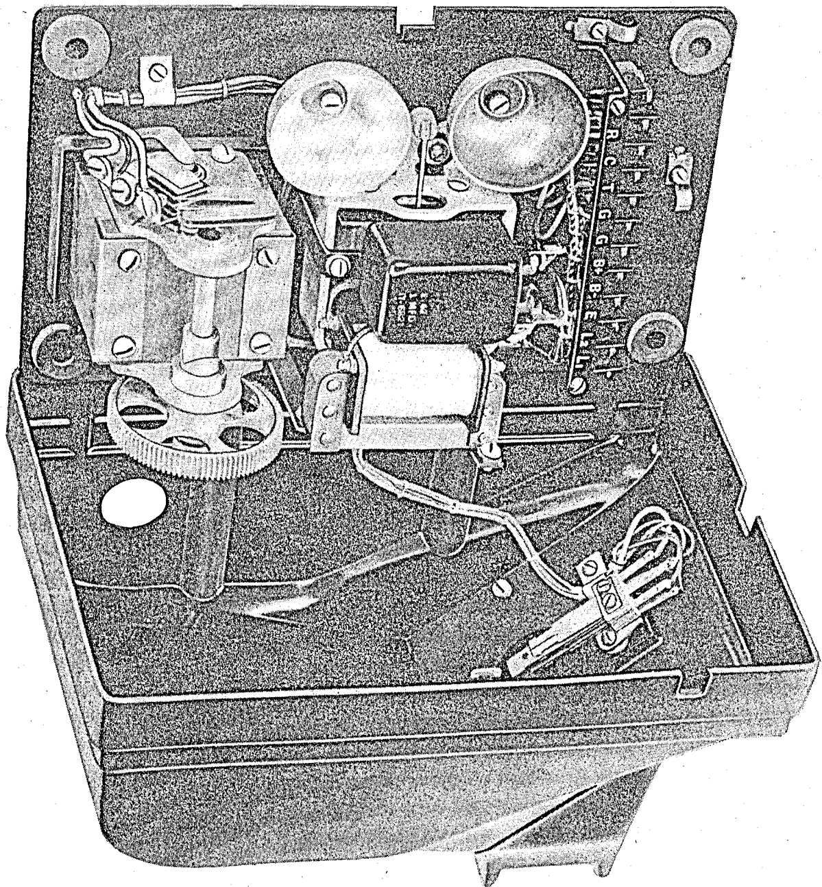
MAGNETO TELEPHONE FTR 701AB, INTERIOR VIEW.
