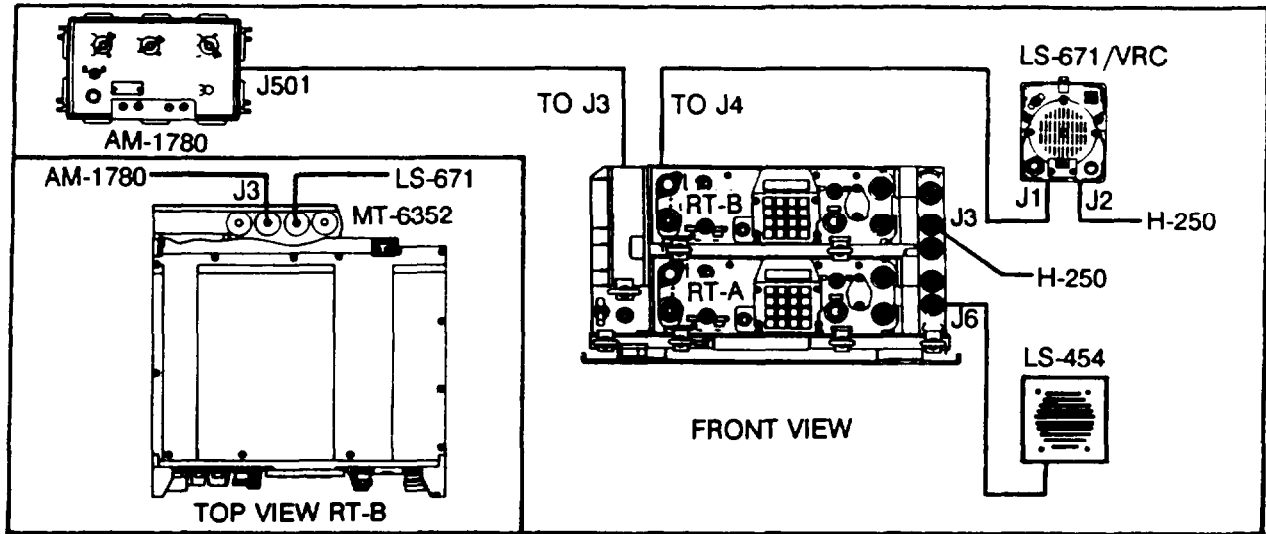
Figure 1. LS-671 Cabling to Dual Radio Set
