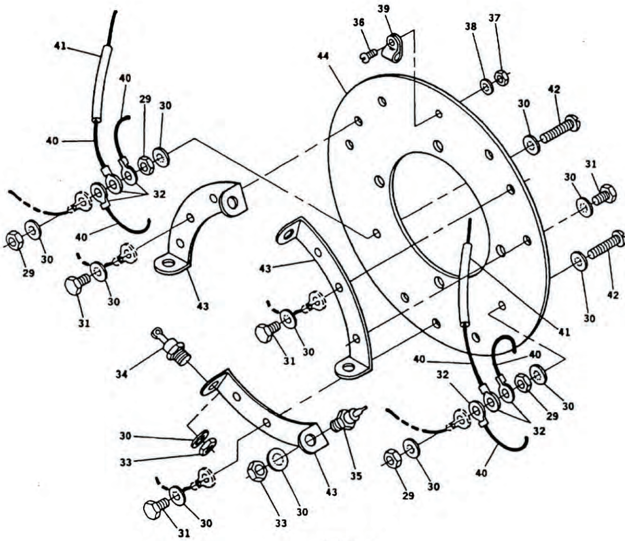
Figure 26. Generator Assembly, 400 Hz (Sheet 2 of 2).
