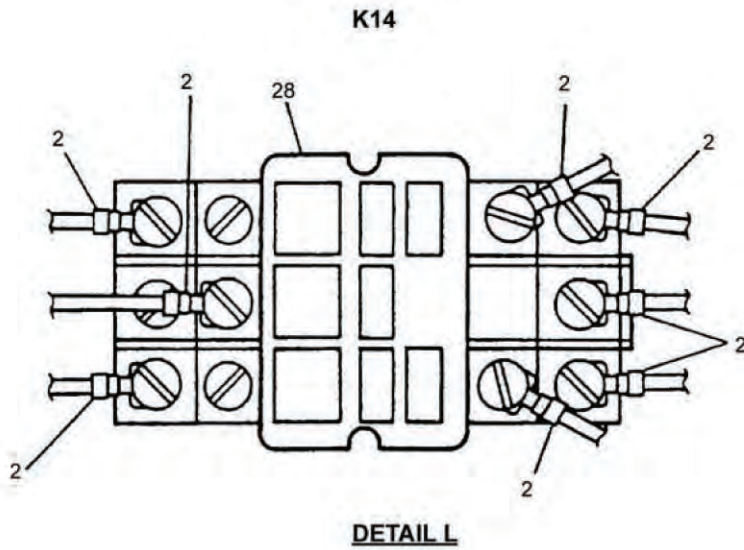
Figure 8. Control Box Harness Assembly (Sheet 11 of 25).
