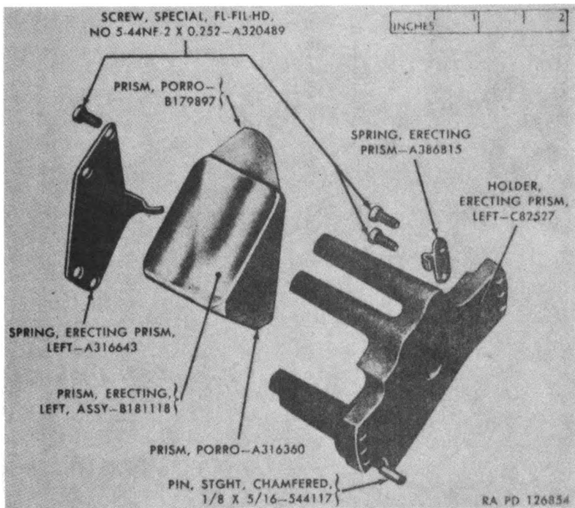
Figure 167. Left erecting prism holder assembly C82526 — exploded view.
