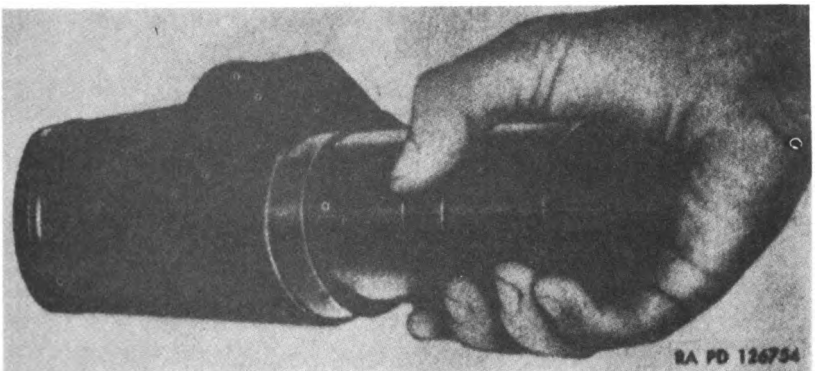
Figure 70. Using wrench 41-W-5726-296 to remove objective retaining ring.
