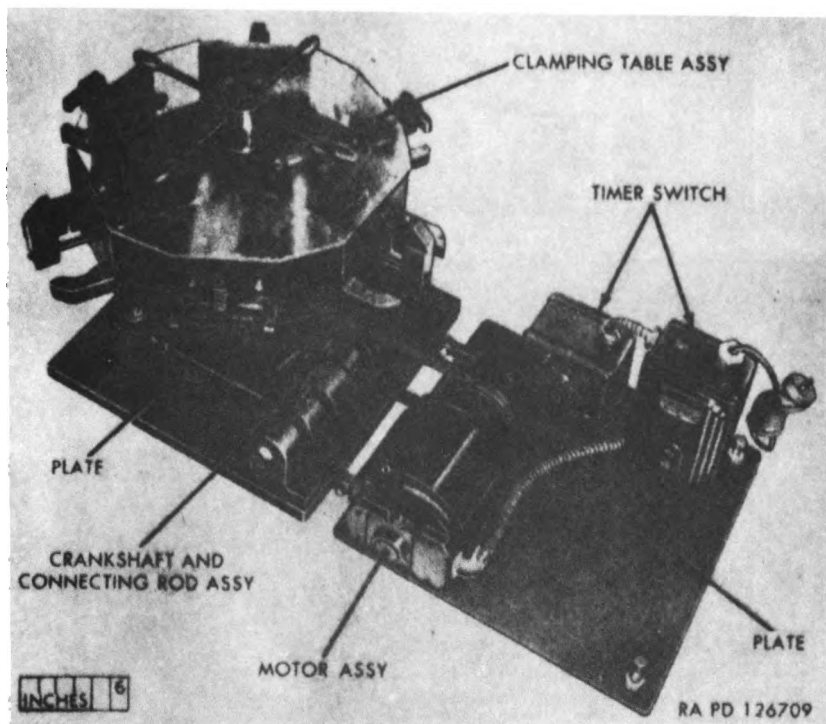
Figure 19. Binocular vibration tester 17-T-5549-925.
