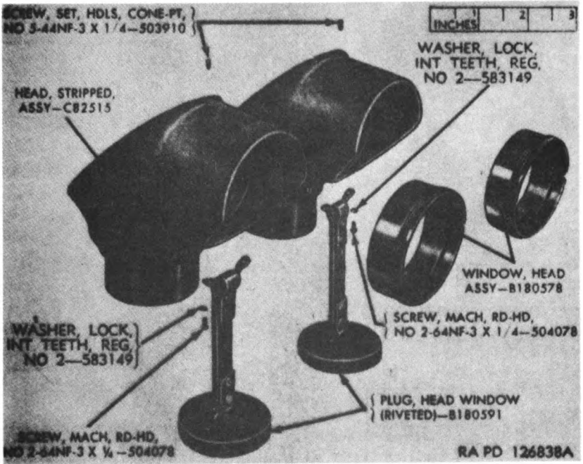
Figure 161. Head assembly C82516 — partial exploded view.
