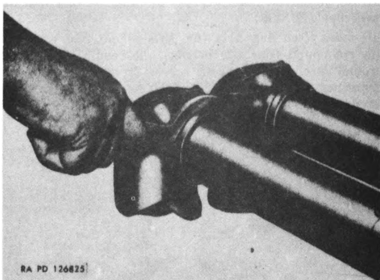
Figure 138. Using spanner wrench 41-W-3249-740 to remove head assembly C82616.
