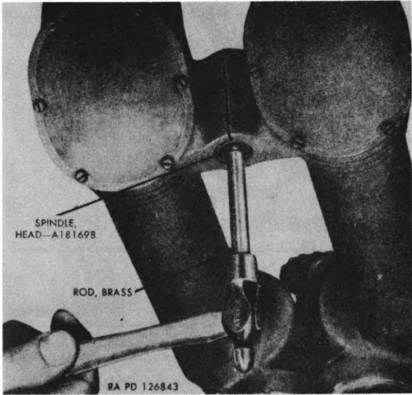
Figure 158. Removing telescope head spindle A181698.
