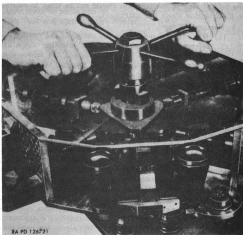
Figure 37. Binocular mounted on binocular vibration tester 17-T-5649-926.
