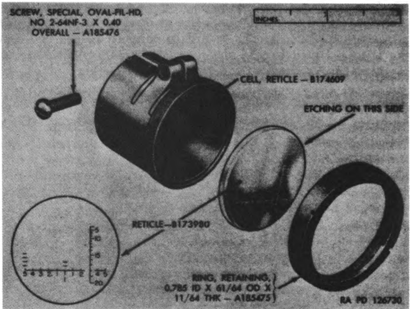
Figure 45. Reticle assembly — B174002 — exploded view.
