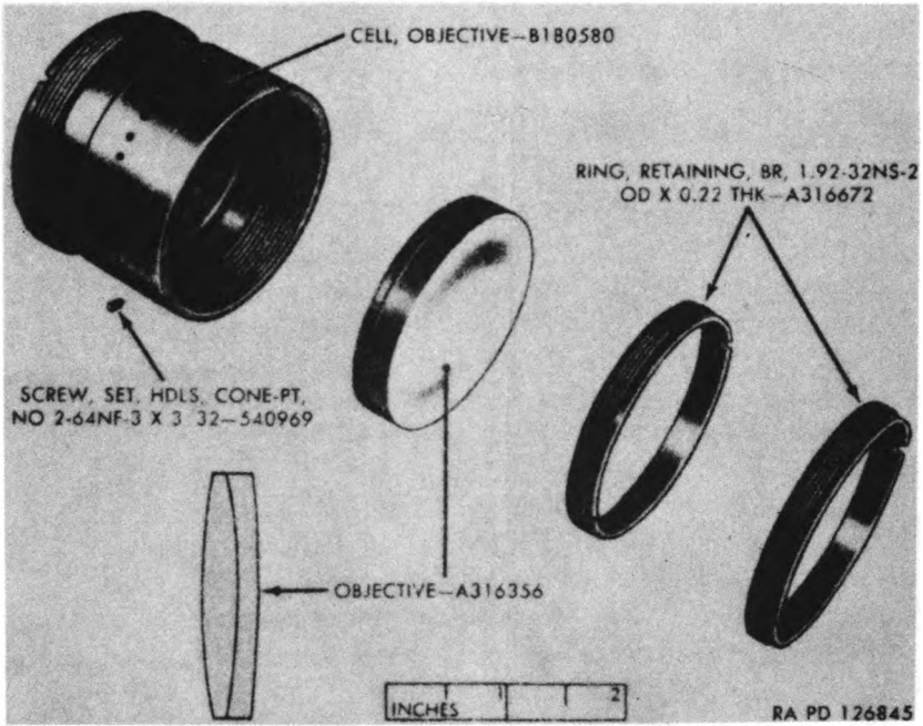
Figure 168. Objective assembly B180589 — exploded view.
