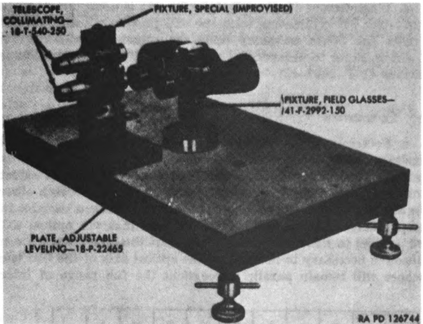
Figure 59. Binocular and improvised fixture in position for collimating at 67-MM setting of interpupillary scale or for checking tilt of reticle.
