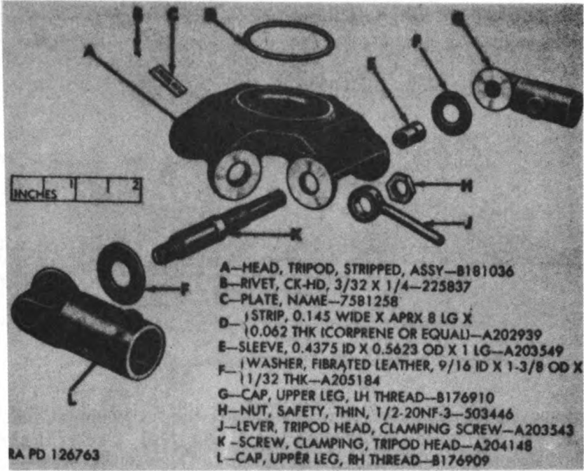
Figure 180. Tripod head assembly C81221 — exploded view.
