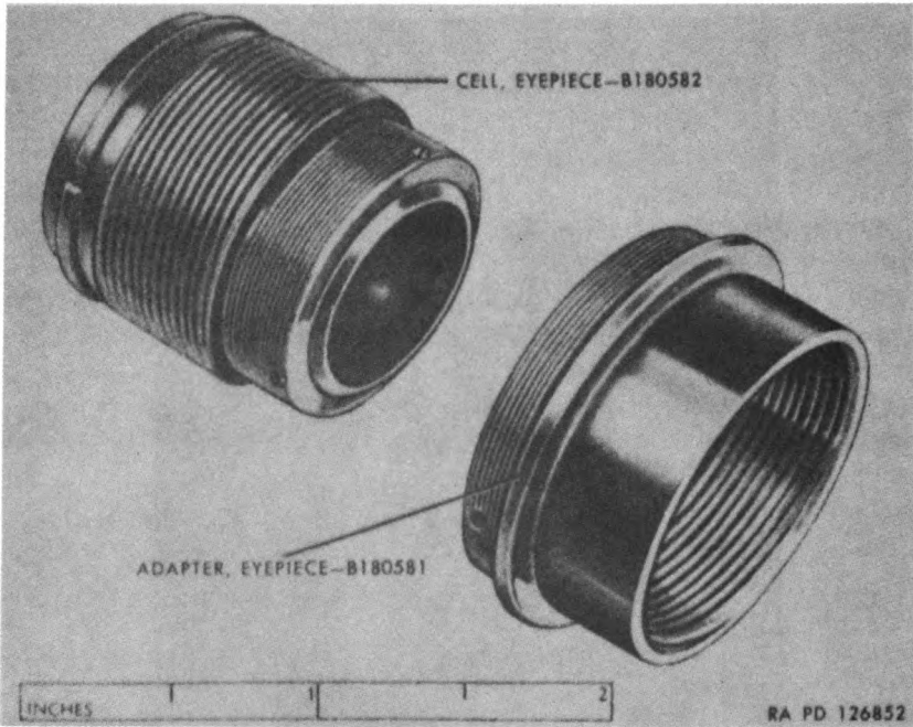
Figure 165. Eyepiece cell assembly 7657458 — exploded view.
