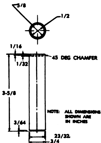
Figure 28. Sealing compound applicator.
