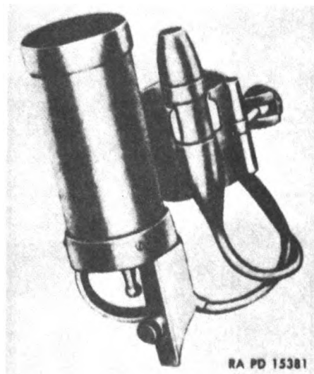
Figure 182. Instrument light M28 — assembled view.
