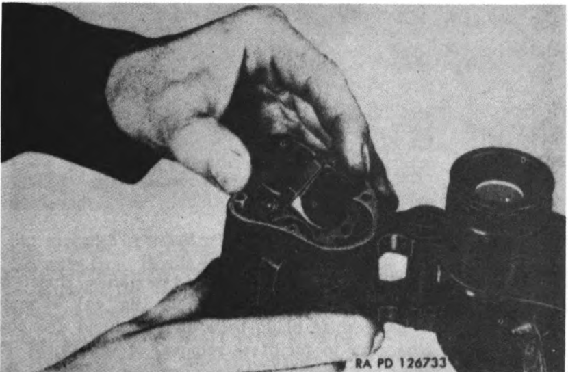
Figure 48. Removing or installing prism shelf assembly.
