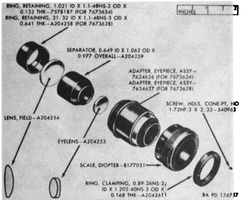
Figure 75. Eyepiece assemblies 7679634 (left, M16 only) and 7679628 — exploded view.
