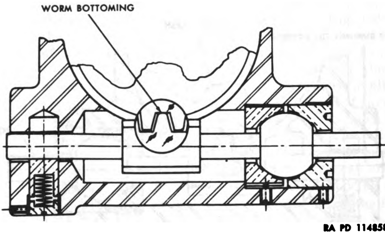
Figure 180. Worm bottoming in worm gear.
