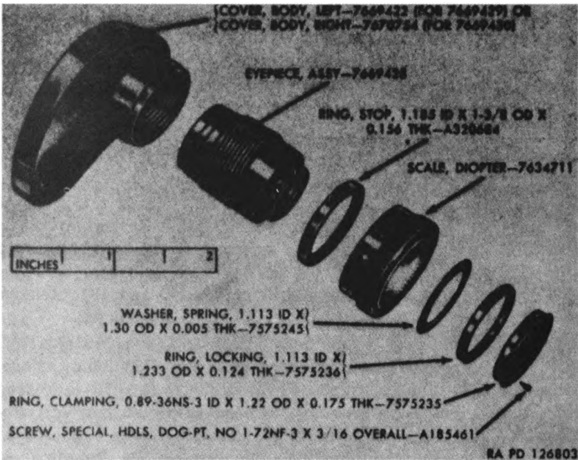
Figure 116. Body cover with eyepiece assembly 7669432 (left, M15) or 7669430 (right, M15) — exploded view.
