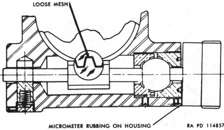
Figure 189. Micrometer rubbing on housing.
