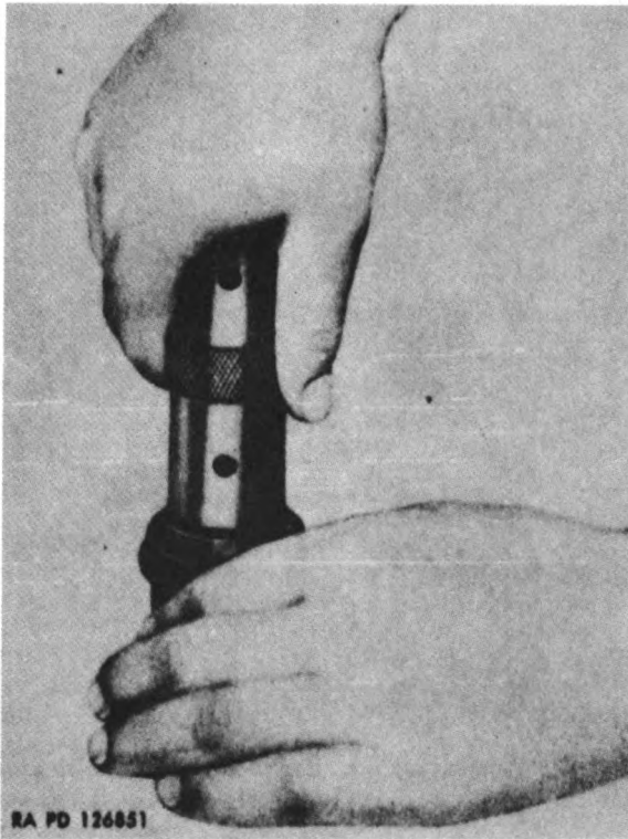
Figure 164. Using tubular wrench 41-W-5726-140 to remove eyepiece retaining ring A318640.
