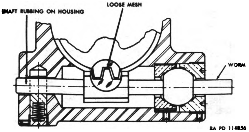
Figure 188. Shaft rubbing on housing.
