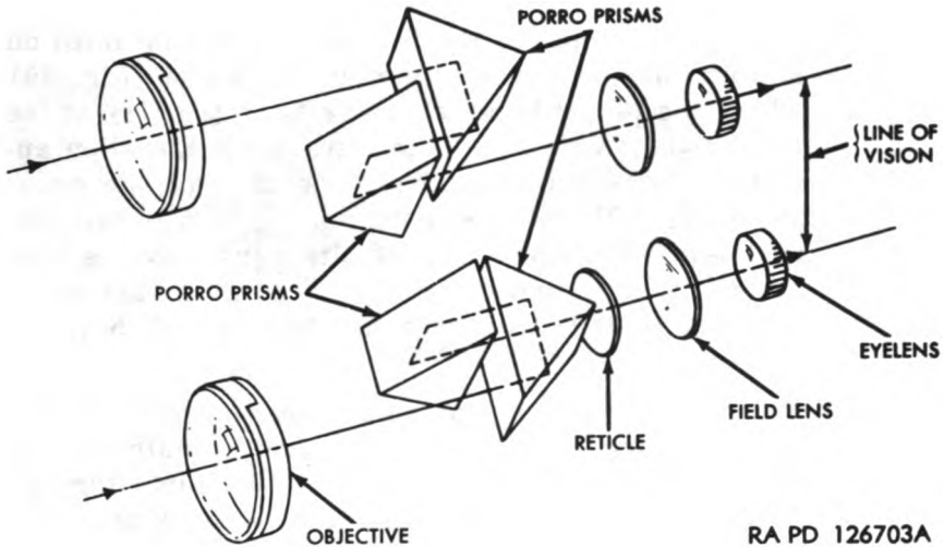
Figure 12. Optical system of typical binocular.
