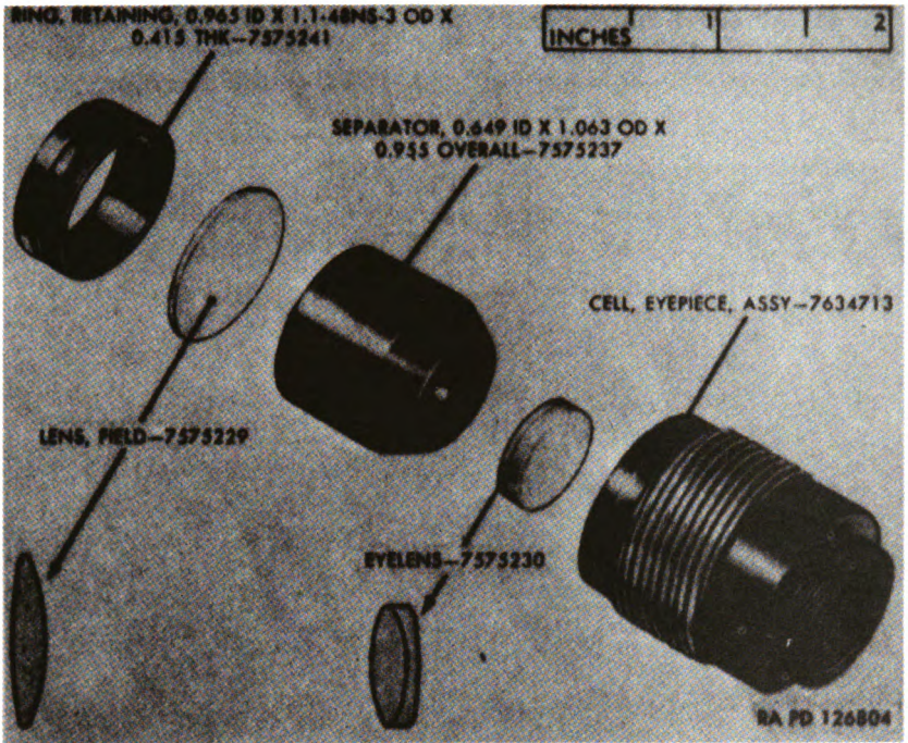
Figure 117. Eyepiece assembly 7669488 (M16 or M16A1) — exploded view.
