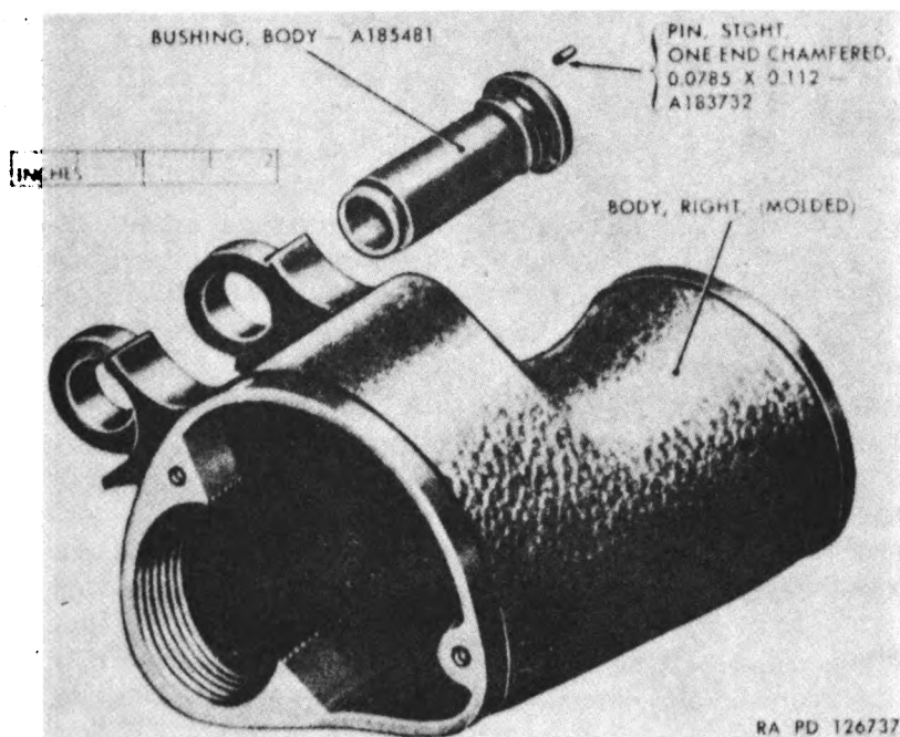
Figure 62. Right body assembly C79398 — exploded view.
