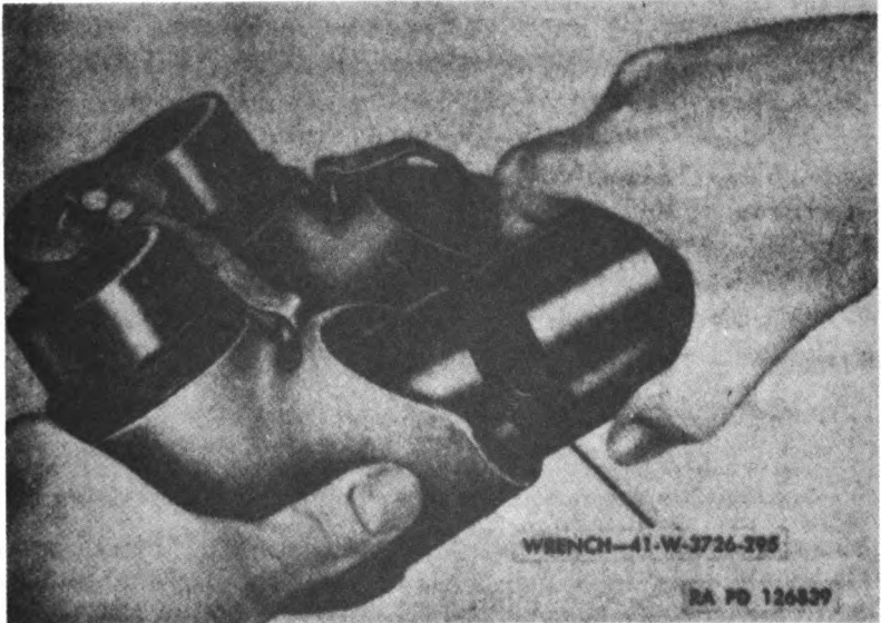
Figure 162. Using tubular wrench 41-W-3726-395 to remove window assembly.
