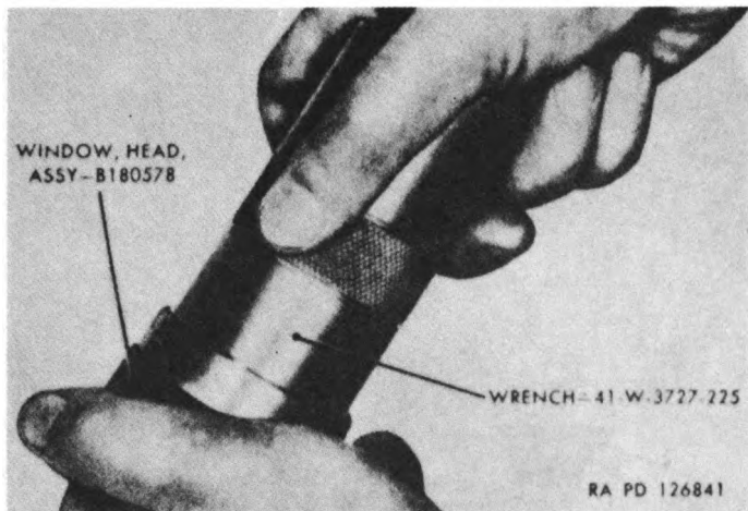
Figure 164. Using wrench 41-W-3727-225 to remove head window retaining ring A316842.
