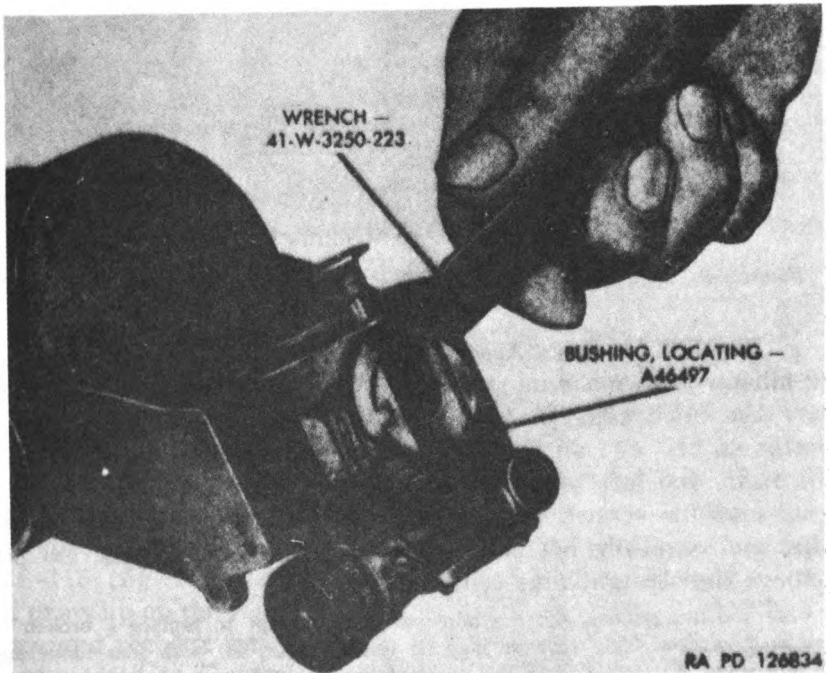
Figure 147. Using spanner wrench 41-W-3250-223 on locating bushing. 234418 O-14—53
