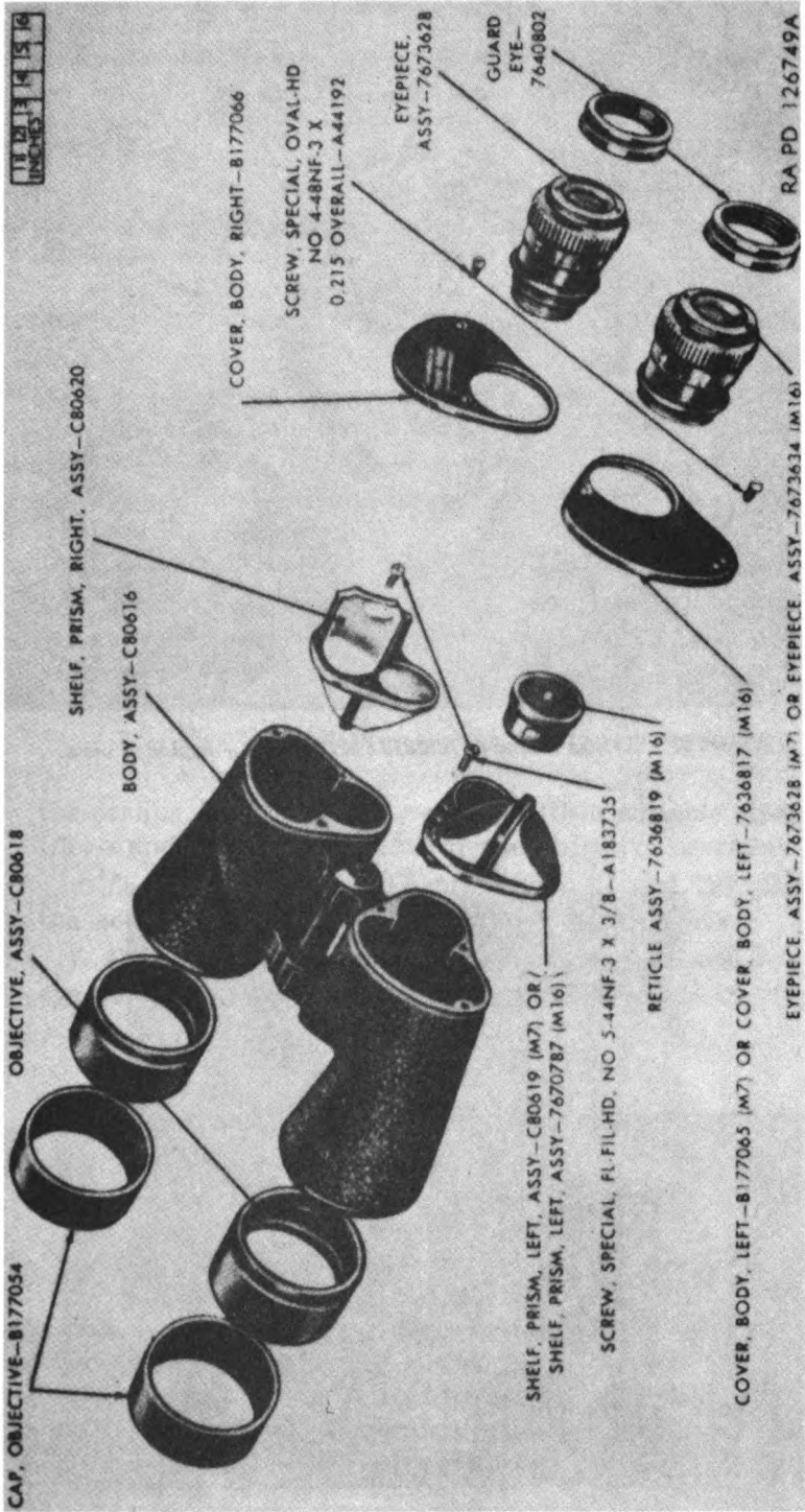
Figure 66. Binocular M7 or M16 — exploded view.
