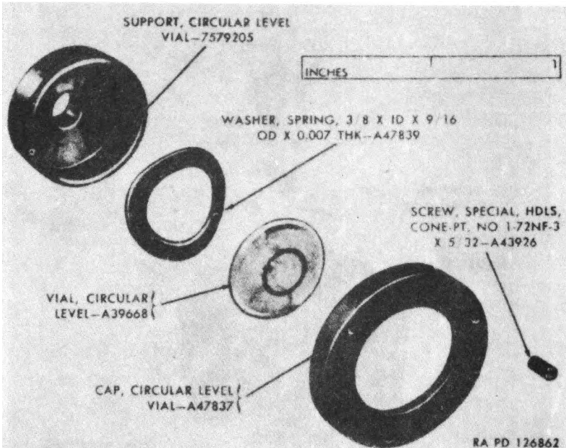
Figure 175. Circular level assembly 7645C11 — exploded view.
