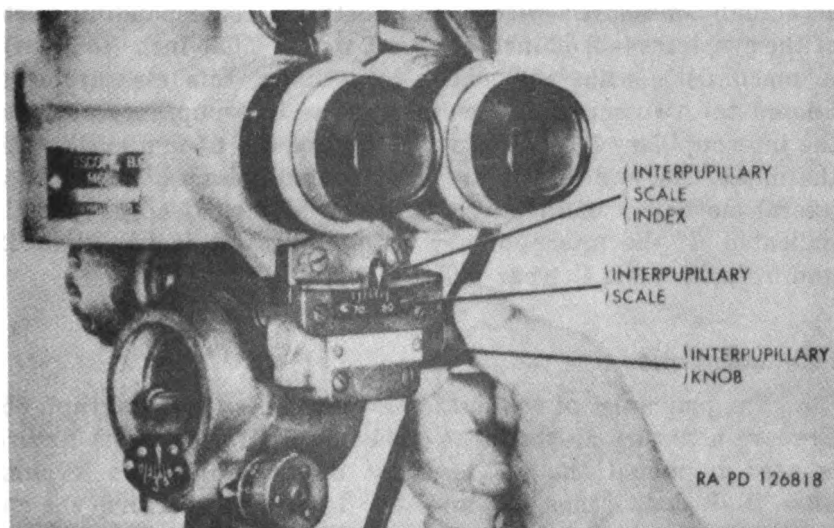
Figure 188. Adjusting interpupillary scale.
