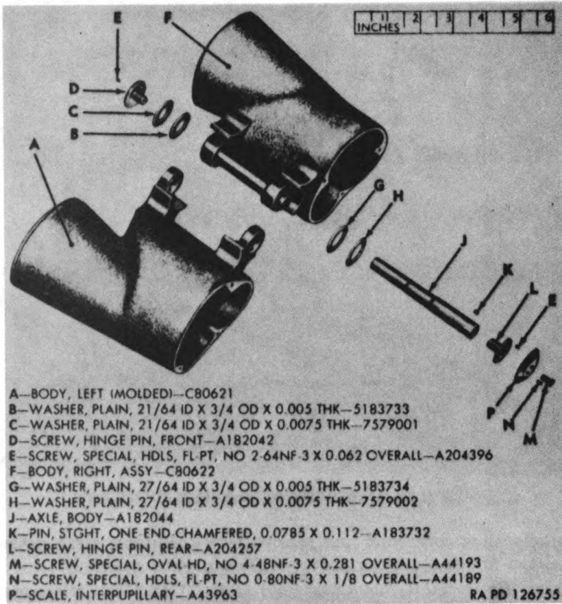
Figure 71. Body assembly C80616 — exploded view.
