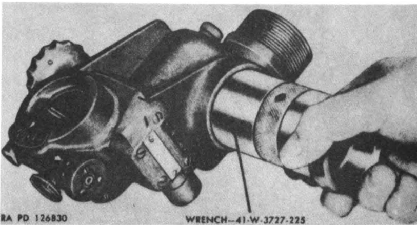
Figure 143. Removing retaining ring A31668 with wrench 41-W-3727-225.
