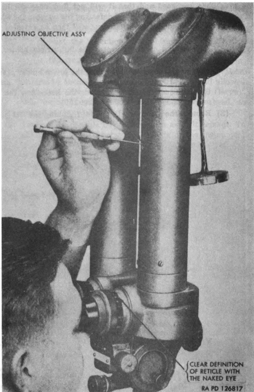
Figure 191. Eliminating parallax.
