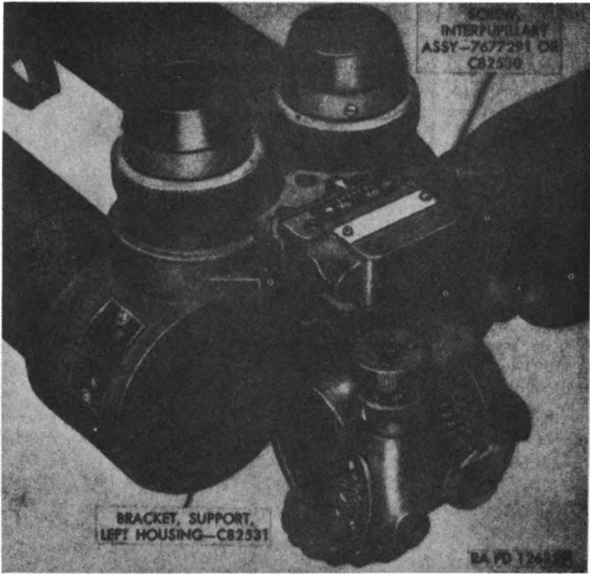
Figure 142. Removing interpillary screw assembly and left housing support bracket.
