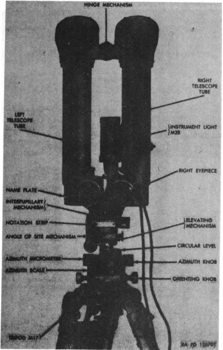
Figure 10. BC telescope M65 — rear view.
