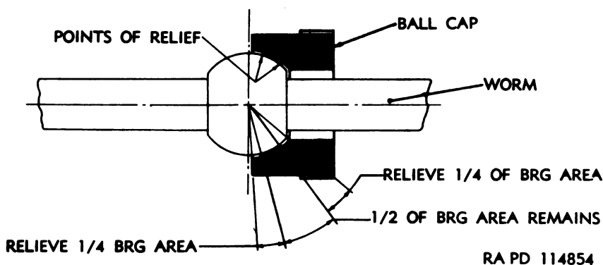
Figure 188. Points of relief on ball cap.
