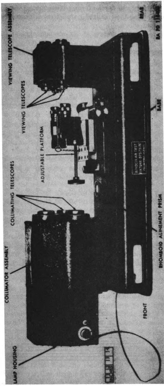
Figure 20. Binocular testing fixture 41-F-9887-487.
