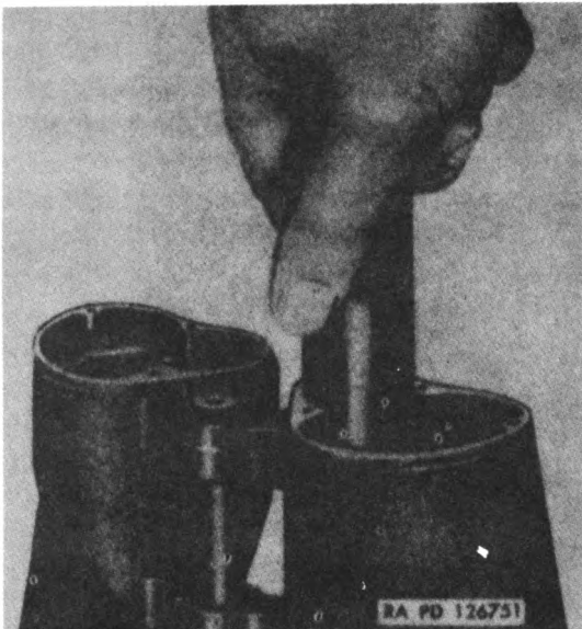
Figure 68. Using wrench 41-W-5726-106 to remove retaining ring (M16 only).
