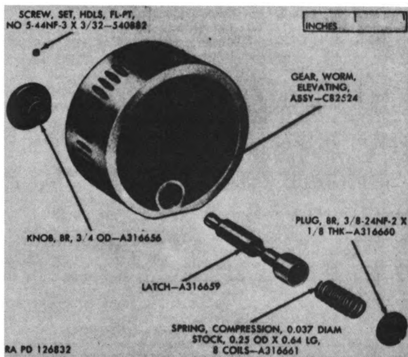
Figure 145. Latch assembly C82523 — exploded view.
