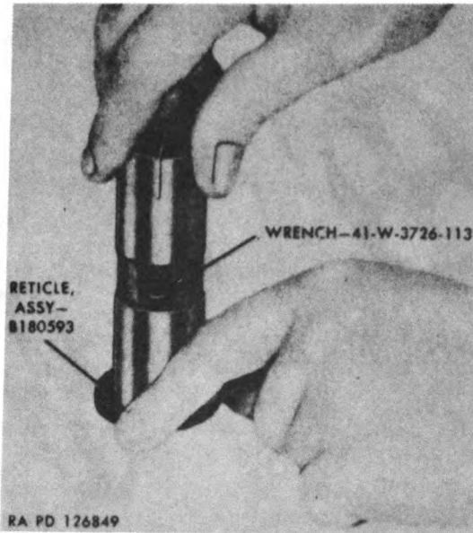
Figure 162. Using tubular wrench 41-W-3726-113 to remove reticle retaining ring A316667.
