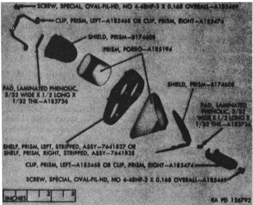
Figure 106. Prism shelf assembly C78990 (right) or C131937 (left) exploded view.
