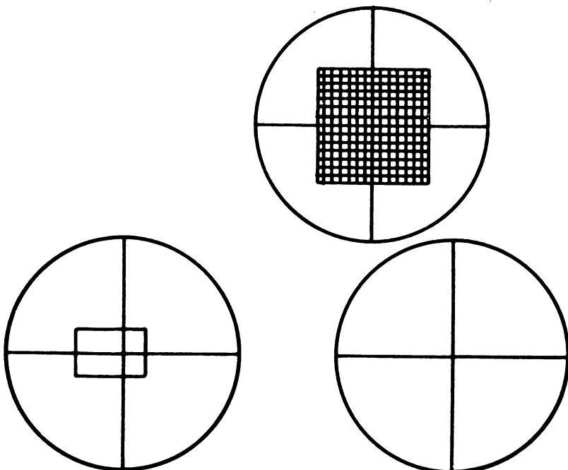
Figure 22. Reticles of fixture 41-F-2957-457 as viewed through collimating telescopes.
