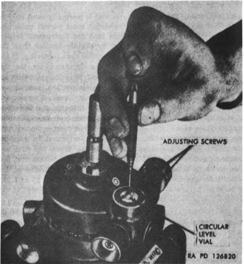
Figure 197. Adjusting circular level vial.
