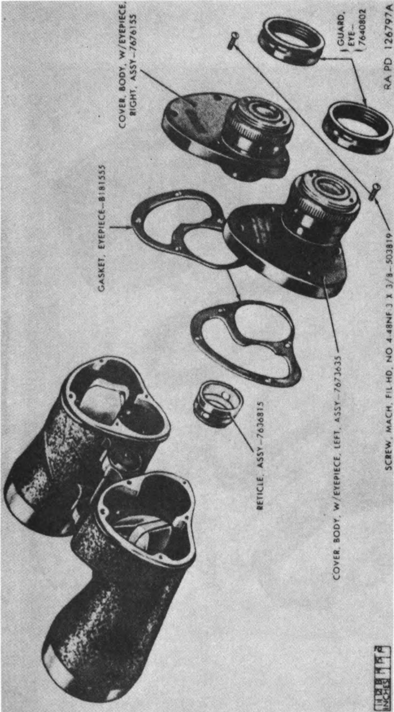
Figure 110. Binocular M17A1 — partial exploded view.
