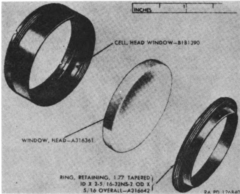
Figure 163. Head window assembly B180578 — exploded view.
