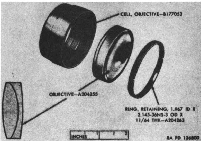
Figure 113. Objective assembly C131157 — exploded view.
