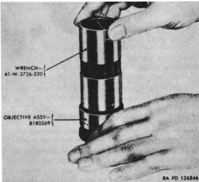
Figure 169. Using tubular wrench 41-W-3726-220 to remove objective retaining ring A316672.
