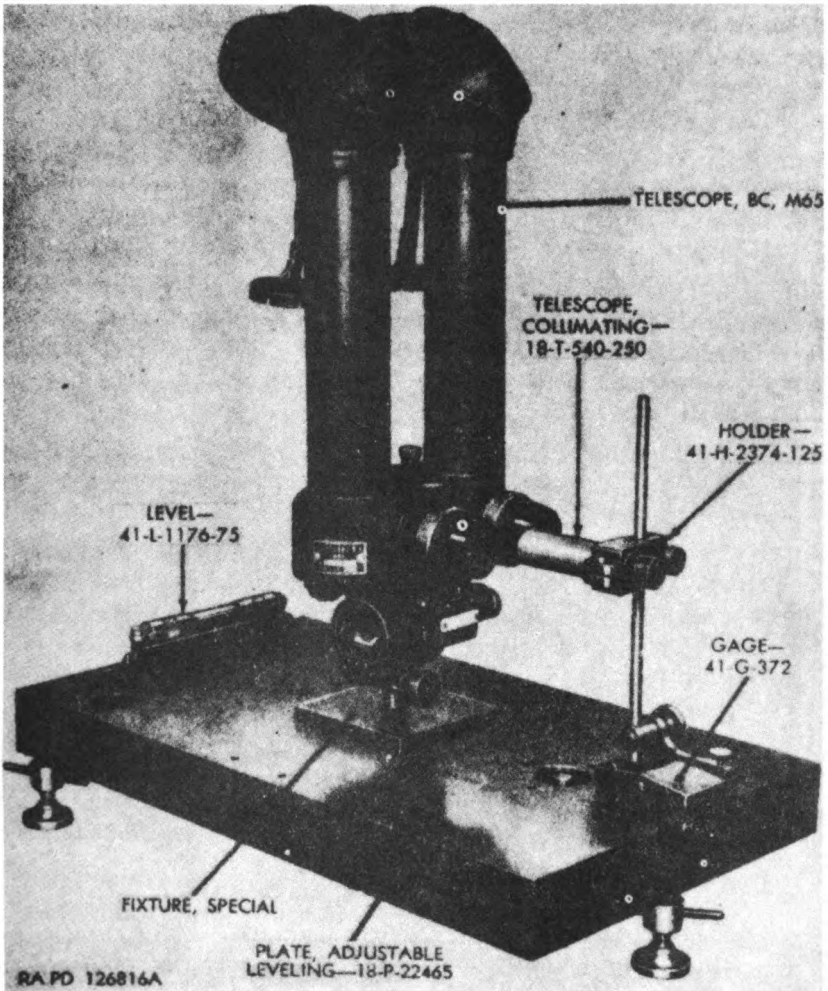
Figure 190. BC telescope M65 in position for collimating.
