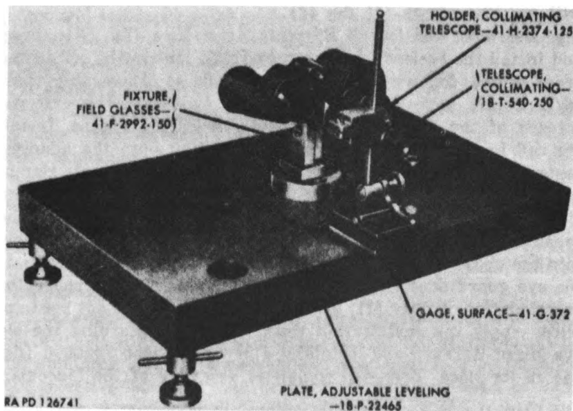
Figure 56. Adjusting for tilt of field of view.
