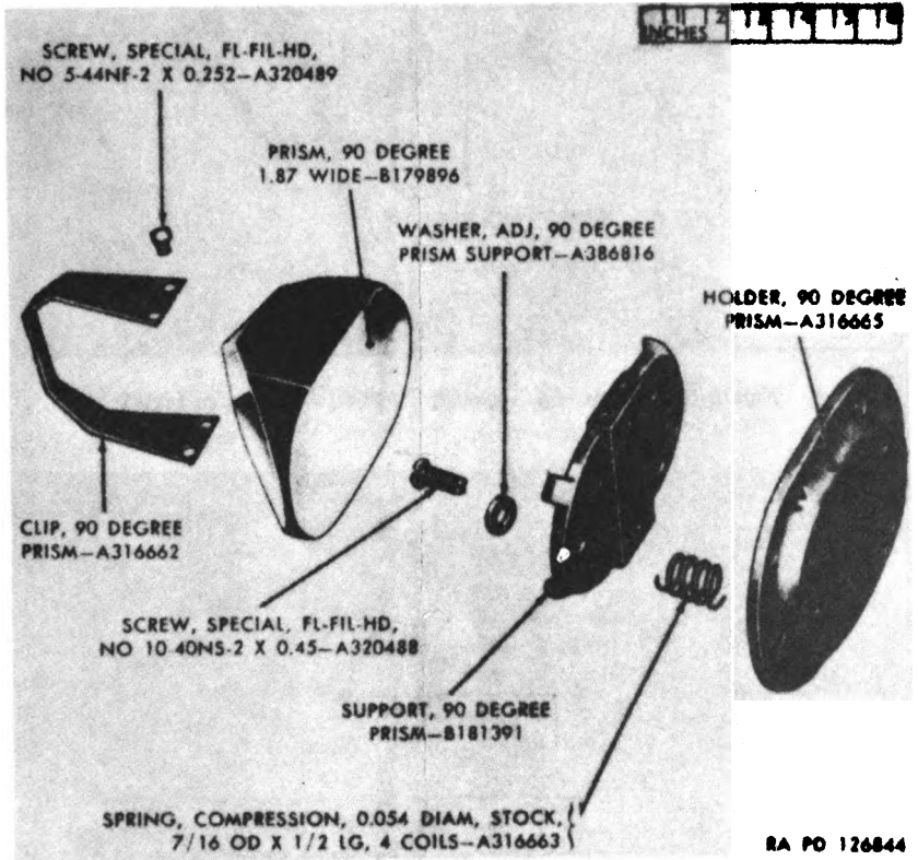
Figure 167. 90° prism holder assembly C191126 — exploded view.
