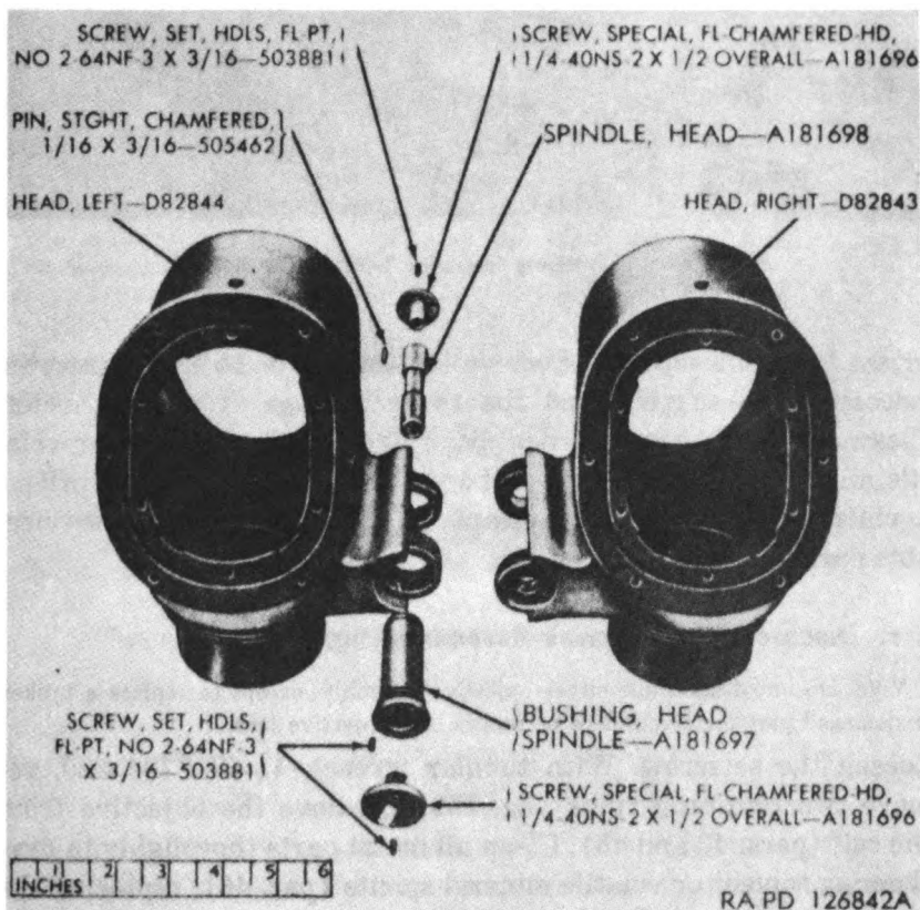
Figure 165. Left and right stripped head assembly C82515 — exploded view.
