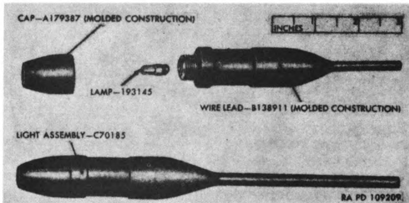
Figure 184. Hand light assembly C70185 — partial exploded view.
