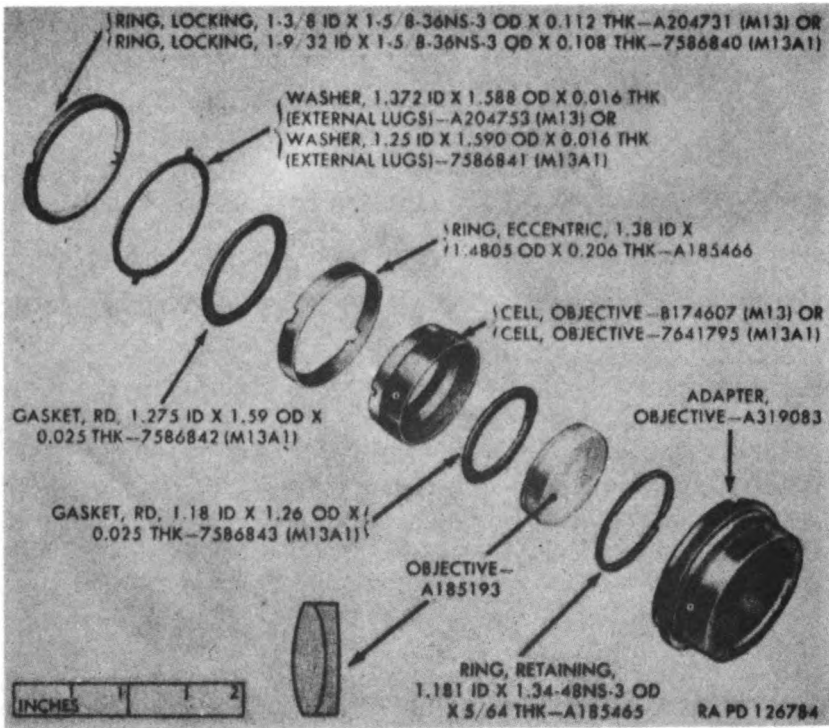
Figure 97. Objective assembly C131334 or 7674286 — exploded view.
