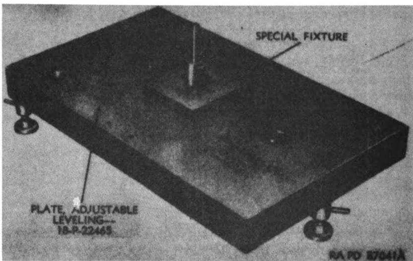
Figure 189. Special fixture in position on leveling plate.
