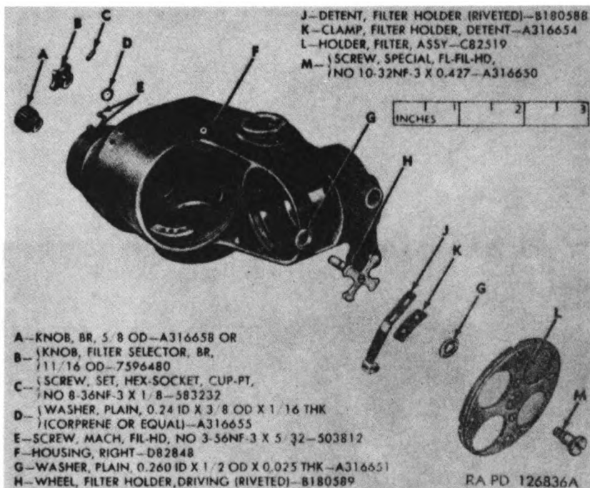
Figure 149. Right housing with filter holder assembly D7492 — exploded view.
