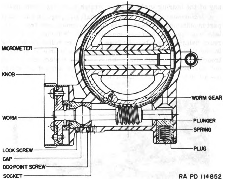
Figure 124. Typical worm and worm gear mechanism.
