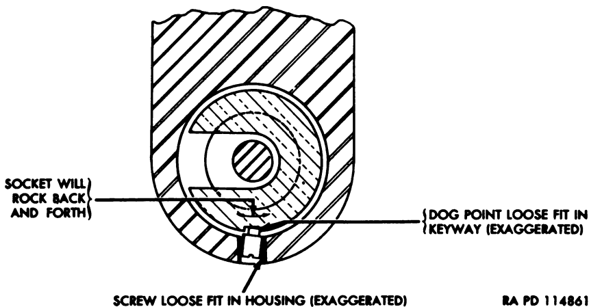
Figure 133. Dog-point screw loose in threads in housing.
