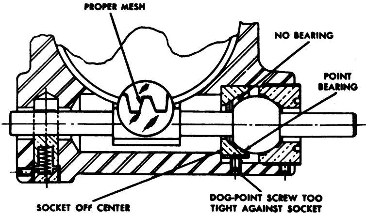
Figure 138. Dog-point screw tight against socket.
