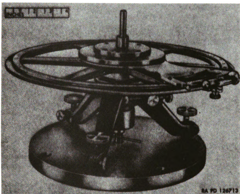
Figure 25. Azimuth testing fixture 41-F-2995.
