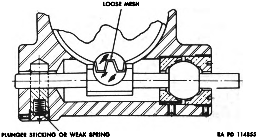
Figure 187. Plunger sticking on weak spring.
