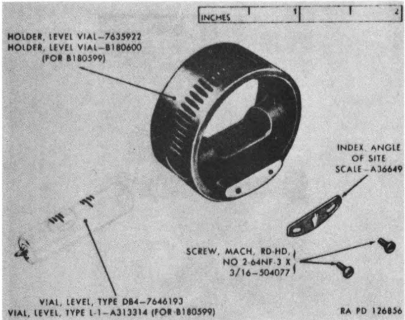
Figure 189. Level vial holder assembly 7635921 or B180599 — exploded view.
