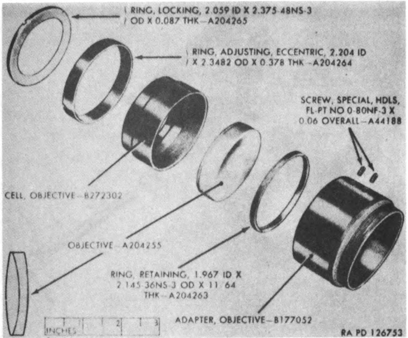
Figure 69. Objective assembly C80618 — exploded view.
