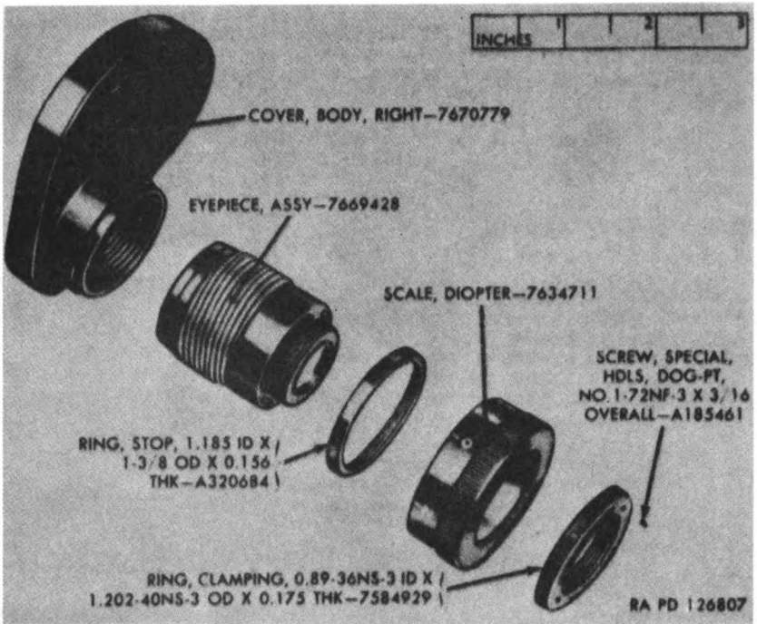
Figure 180. Right body cover and eyepiece assembly 7673696 (M17) — exploded view.
