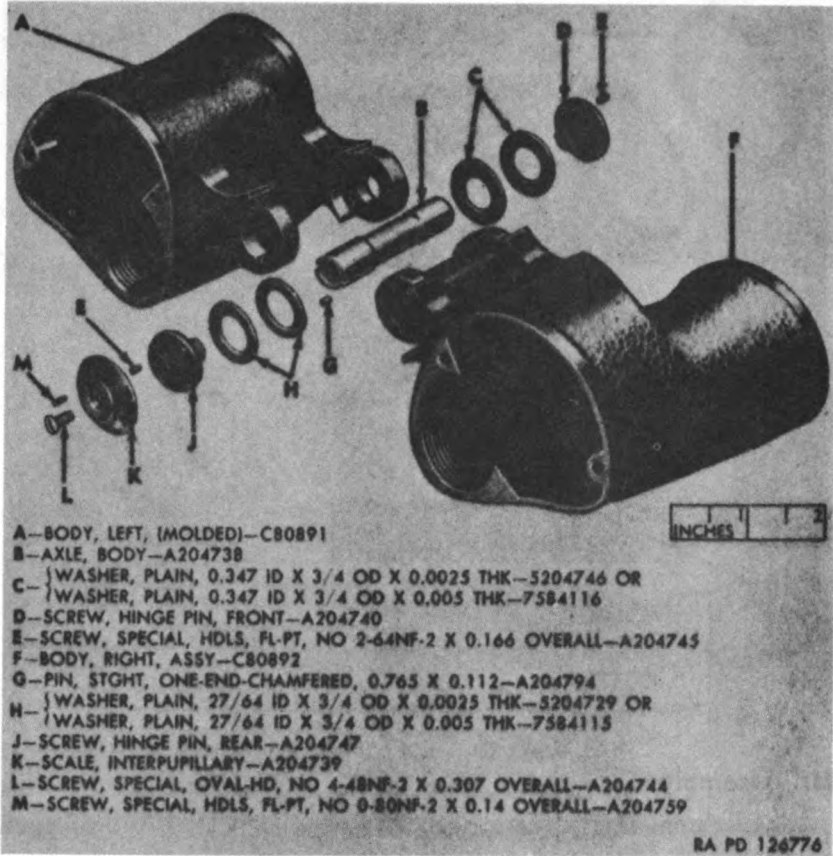
Figure 89. Body assembly — C8086 — exploded view.
