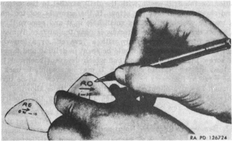
Figure 40. Marking prism pairs.
