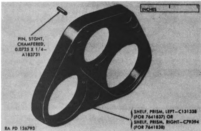
Figure 108. Stripped prism shelf assembly 7641837 (left) or 7641838 (right) — exploded view.
