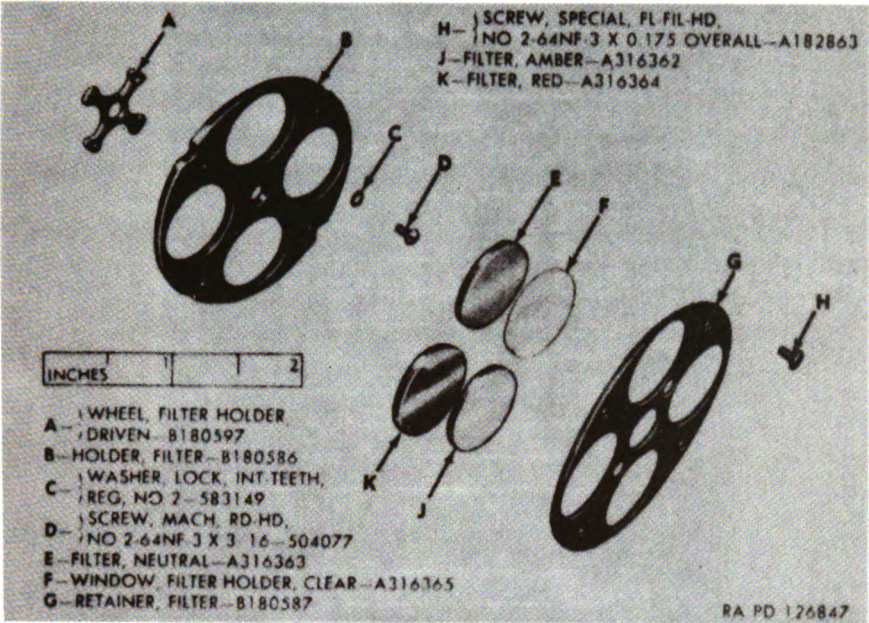
Figure 160. Filter holder assembly C82519 — exploded view.
