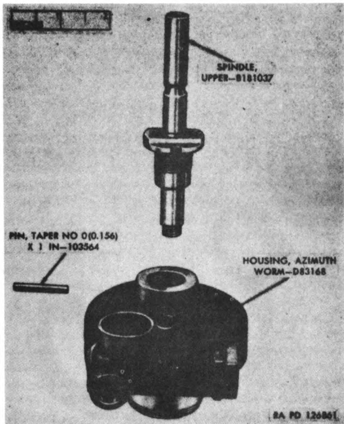
Figure 174. Spindle assembly C130600 — exploded view.
