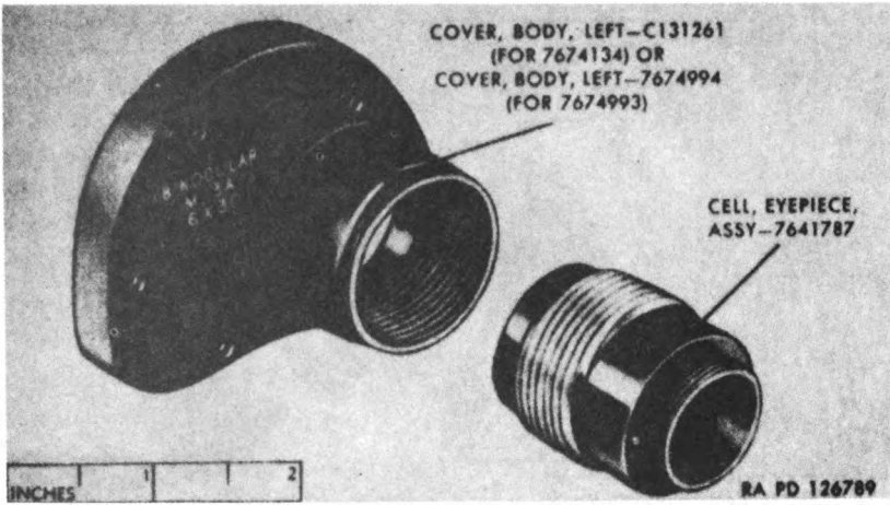
Figure 102. Left body cover assembly 7674134 (M1S) or 7674993 (M1SA1) — exploded view.
