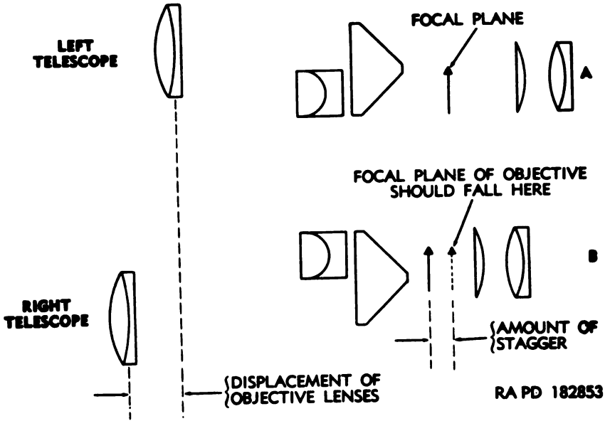
Figure 68. Stagger due to improperly matched objective cells.
