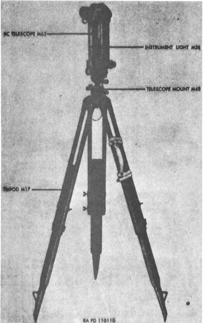
Figure 6. BC telescope M65 with equipment.
