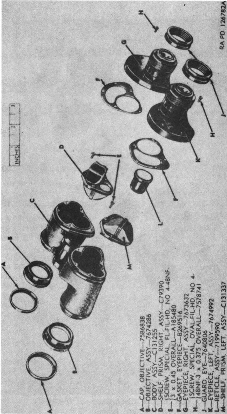
Figure 96. Binocular M19A1 — exploded view.
