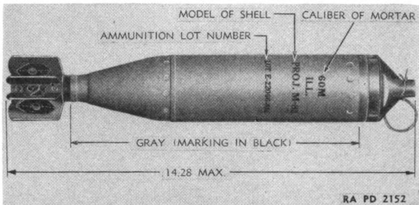
Figure 12 1/2.—Shell, illuminating, 60-mm, with fuze, time, fixed, M65.
