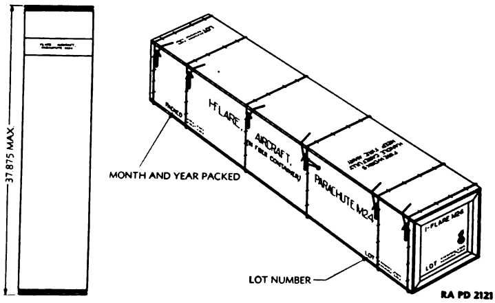
FIGURE 4.—Typical packings and markings.
