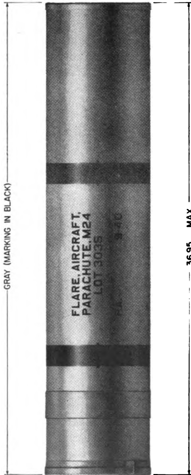
FIGURE 6.—Flare, aircraft, parachute, M24.
