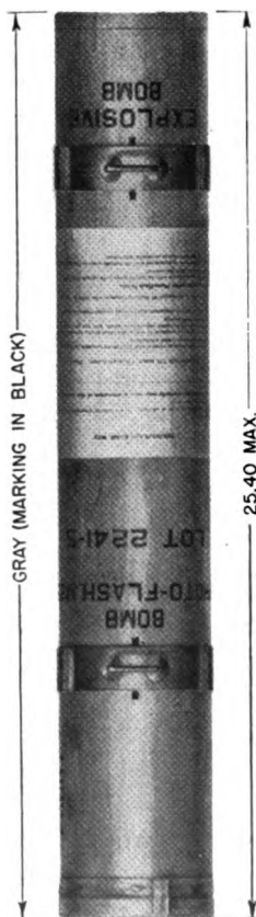
FIGURE 9.—Bomb, photoflash, M23A1.
