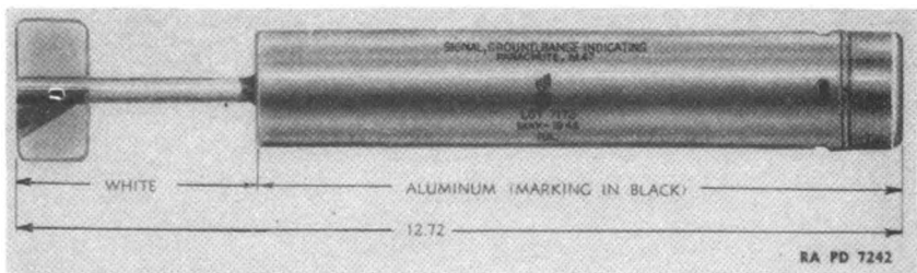
Figure 13 1/2.—Signal, ground, range indicating, parachute, M47.
