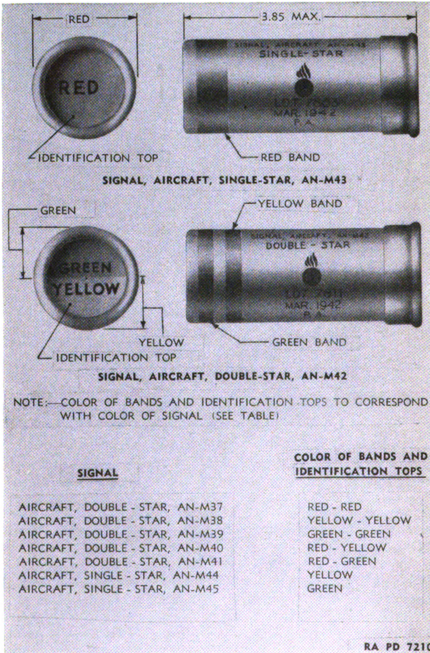
Figure 10½.—Aircraft signals (cartridge type).
