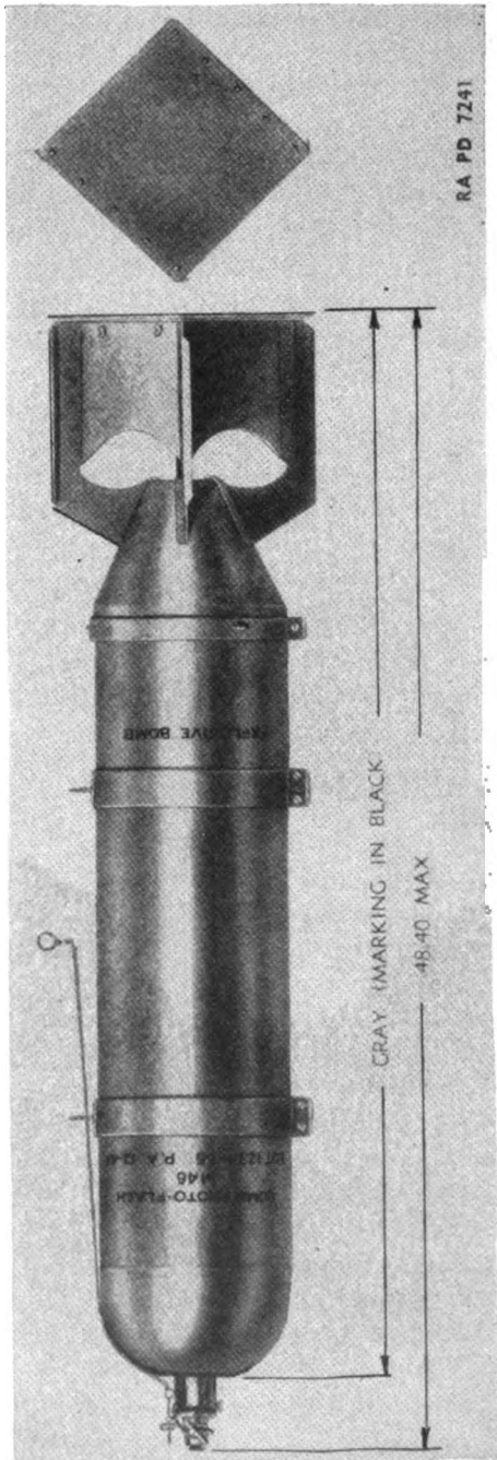
Figure 9 1/4.—Bomb, photoflash, M46.
