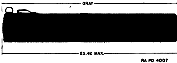
FIGURE 7.—Flare, aircraft, parachute, M8A1.
