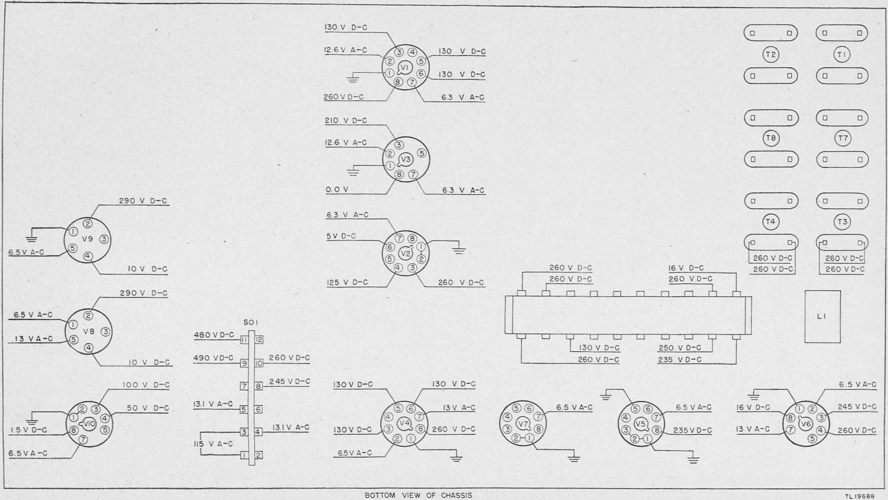
Figure 14. Radio Receiver and Transmitter BC-669-(*), transmit position, socket voltage lay-out diagram.
