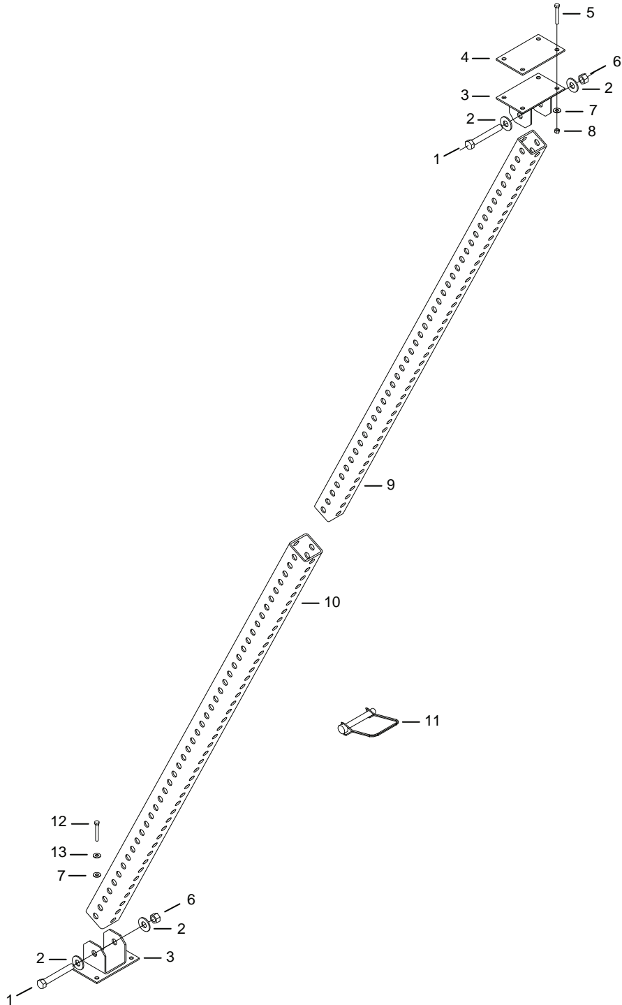
Figure 111. Support Arm Assembly.
