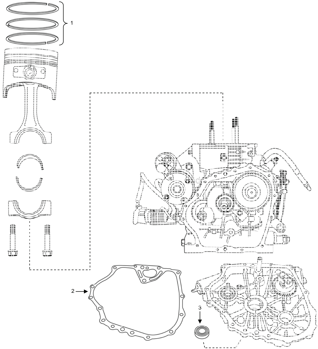
Figure 12. Crankcase Gasket and Piston Rings.
