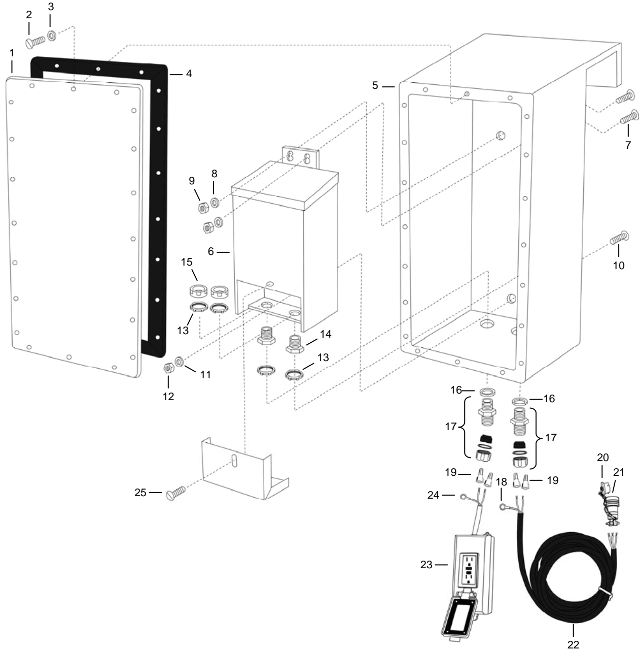
Figure 87. General Purpose Transformer.
