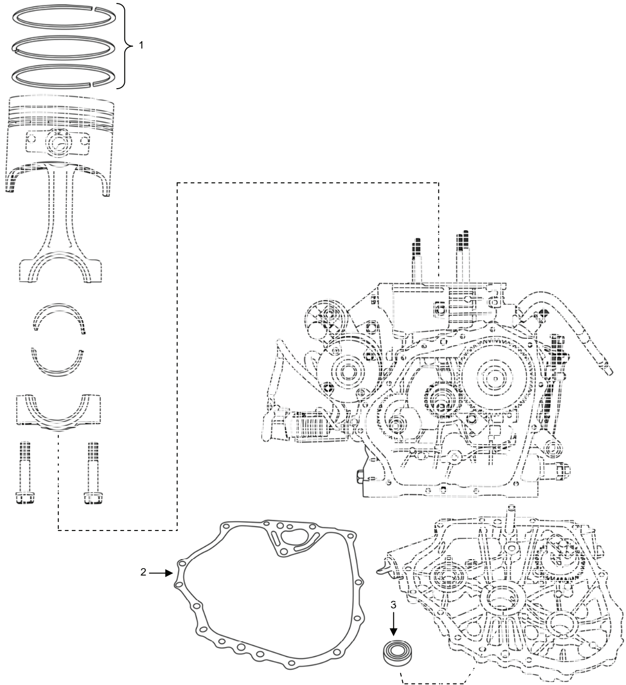
Figure 100. Crankcase Gasket and Piston Rings.
