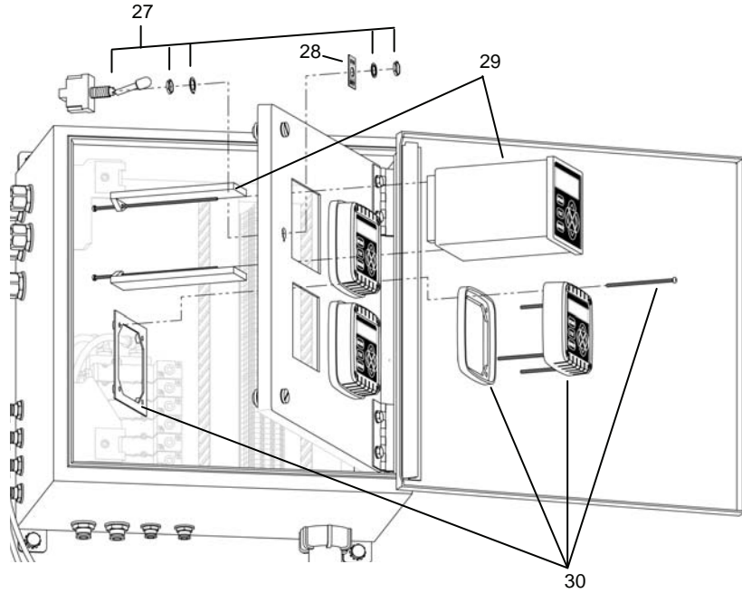
Figure 81. Instrument / Solenoid Panel (Sheet 3 of 3).
