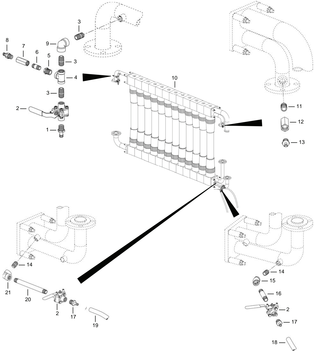
Figure 32. MF Module / Adapter Assembly (Front View).
