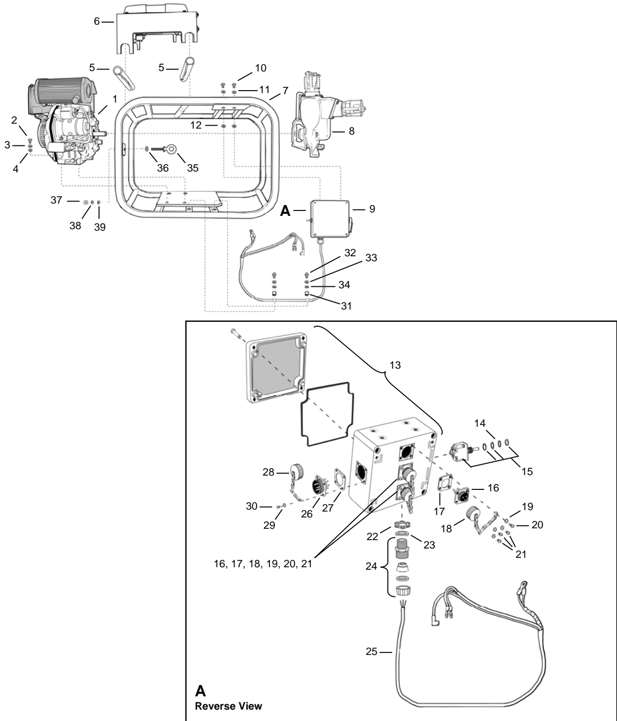
Figure 5. Diesel Engine Pump Assembly P-1.
