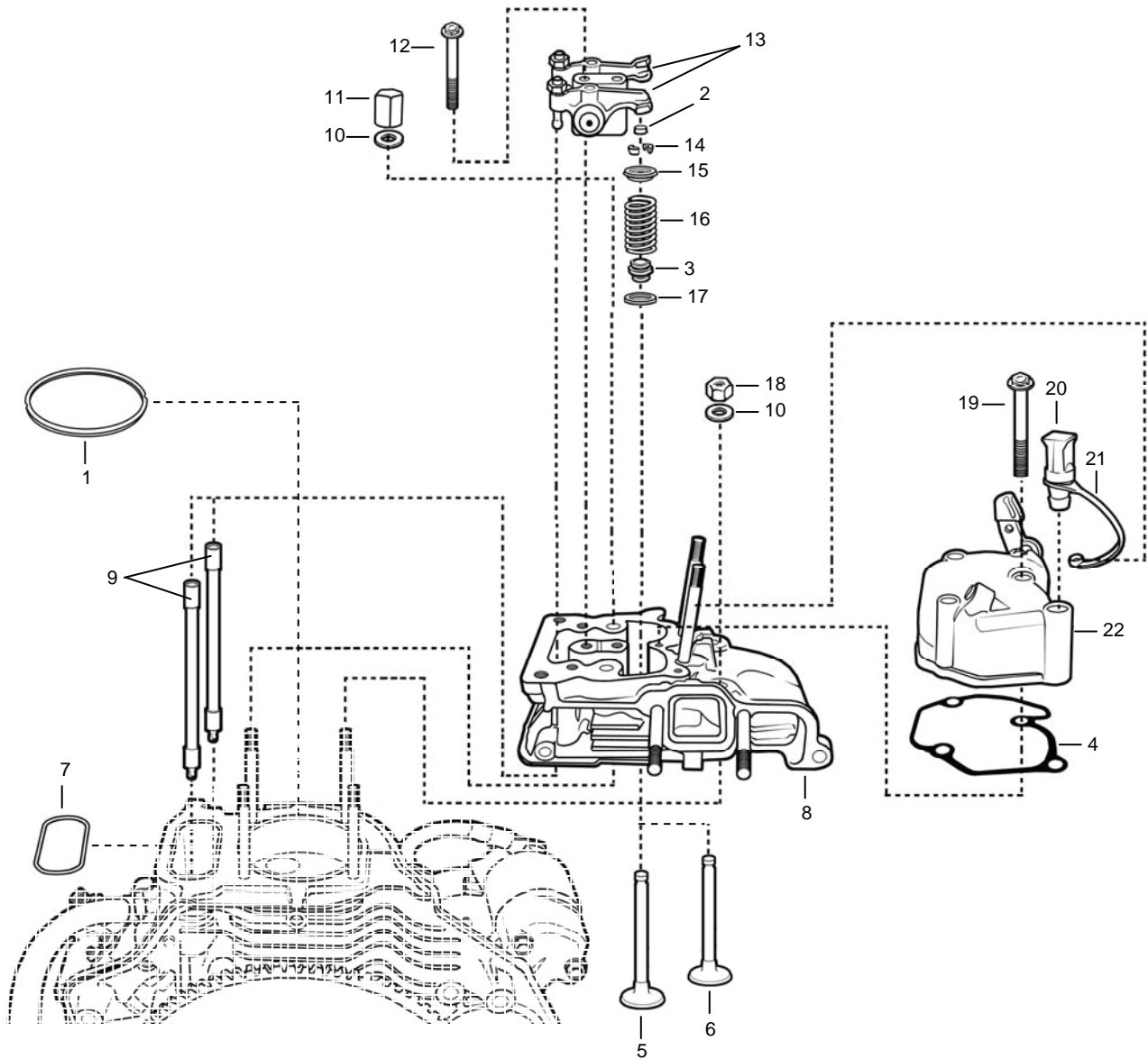
Figure 11. Cylinder Head Valves and Gaskets.
