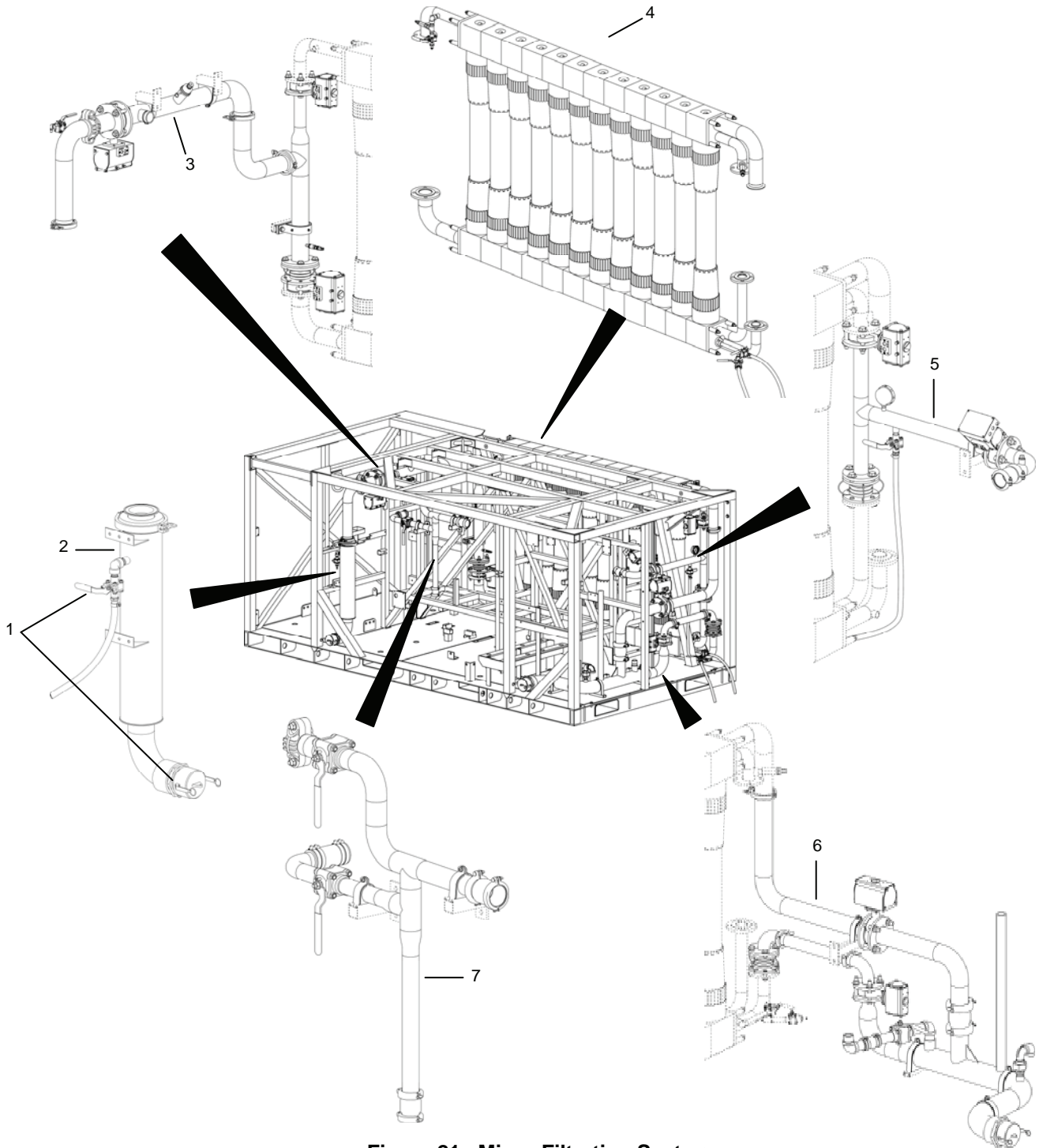
Figure 21. Micro-Filtration System.
