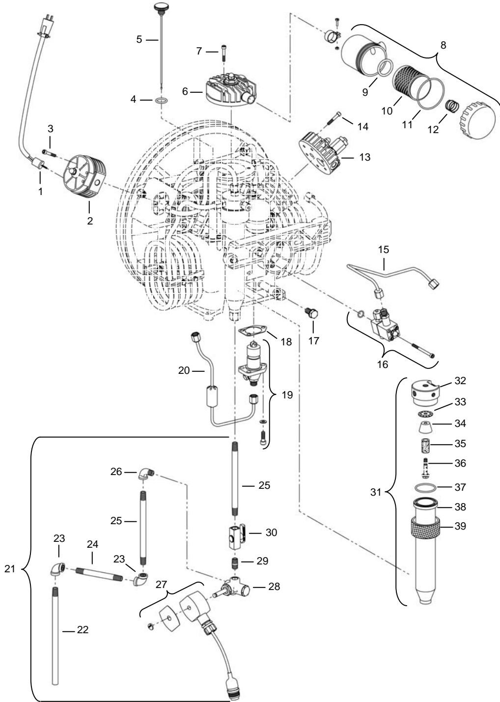
Figure 62. Air Compressor.
