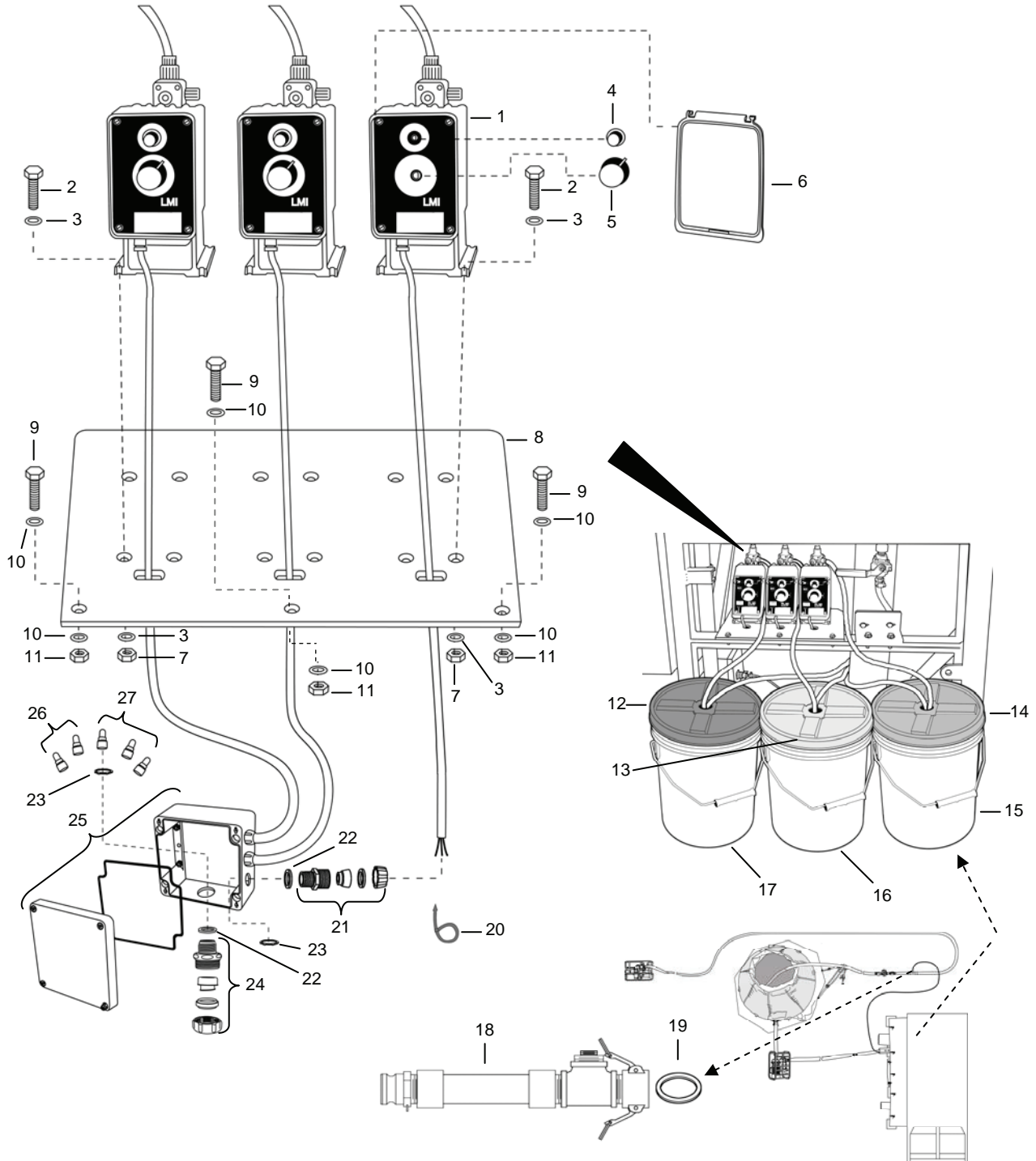
Figure 58. Chemical Injection System.
