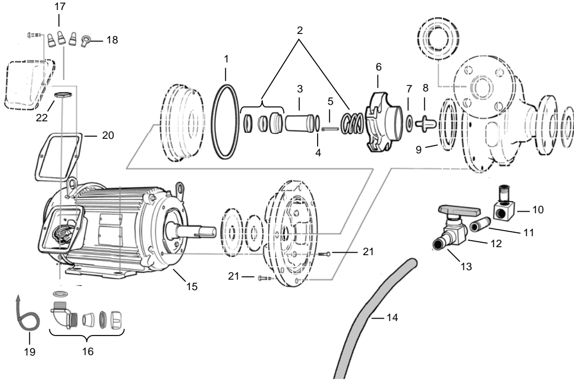
Figure 43. P-4 RO Feed Pump and Motor.
