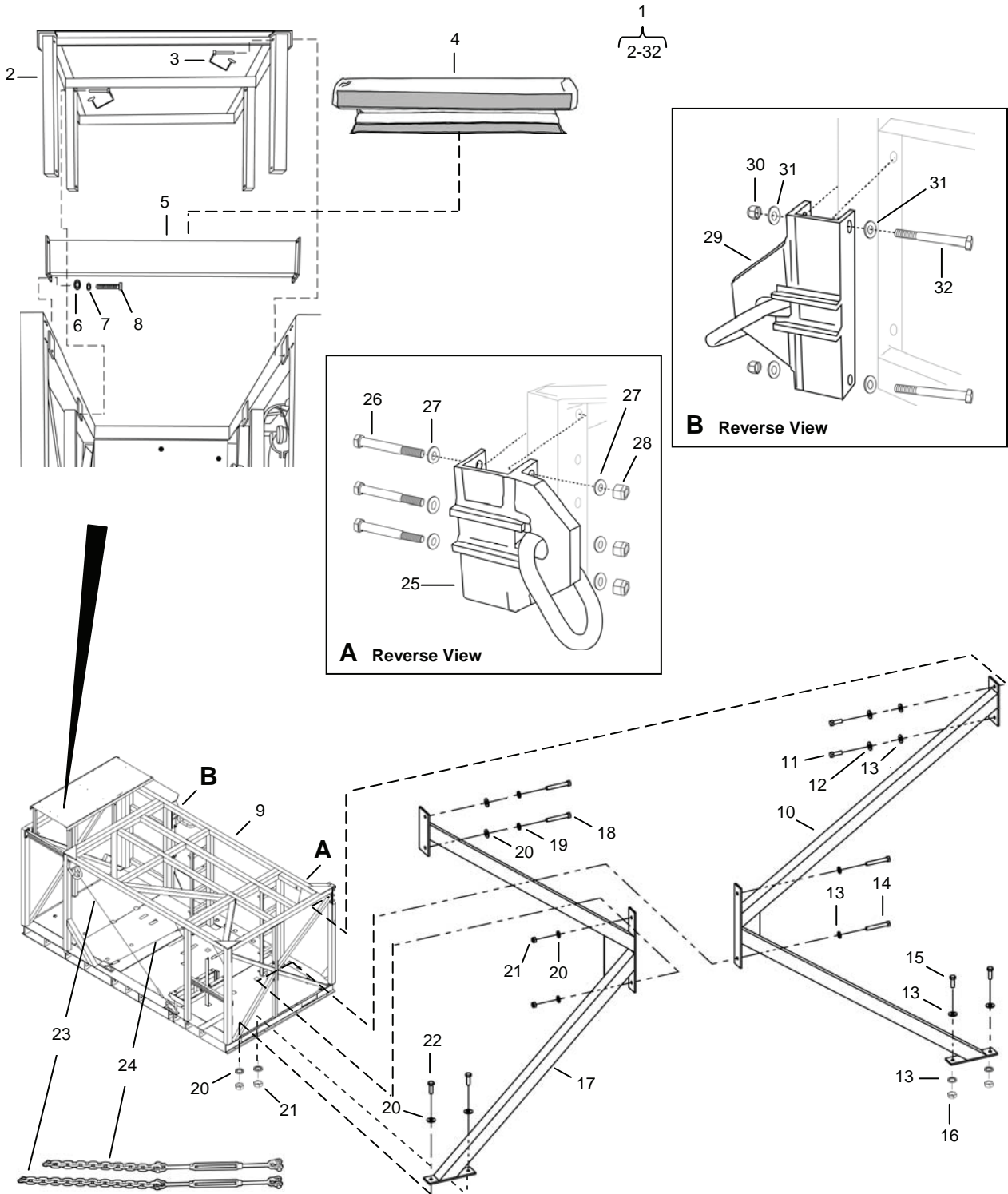
Figure 83. Marine Corps TWPS Skid.
