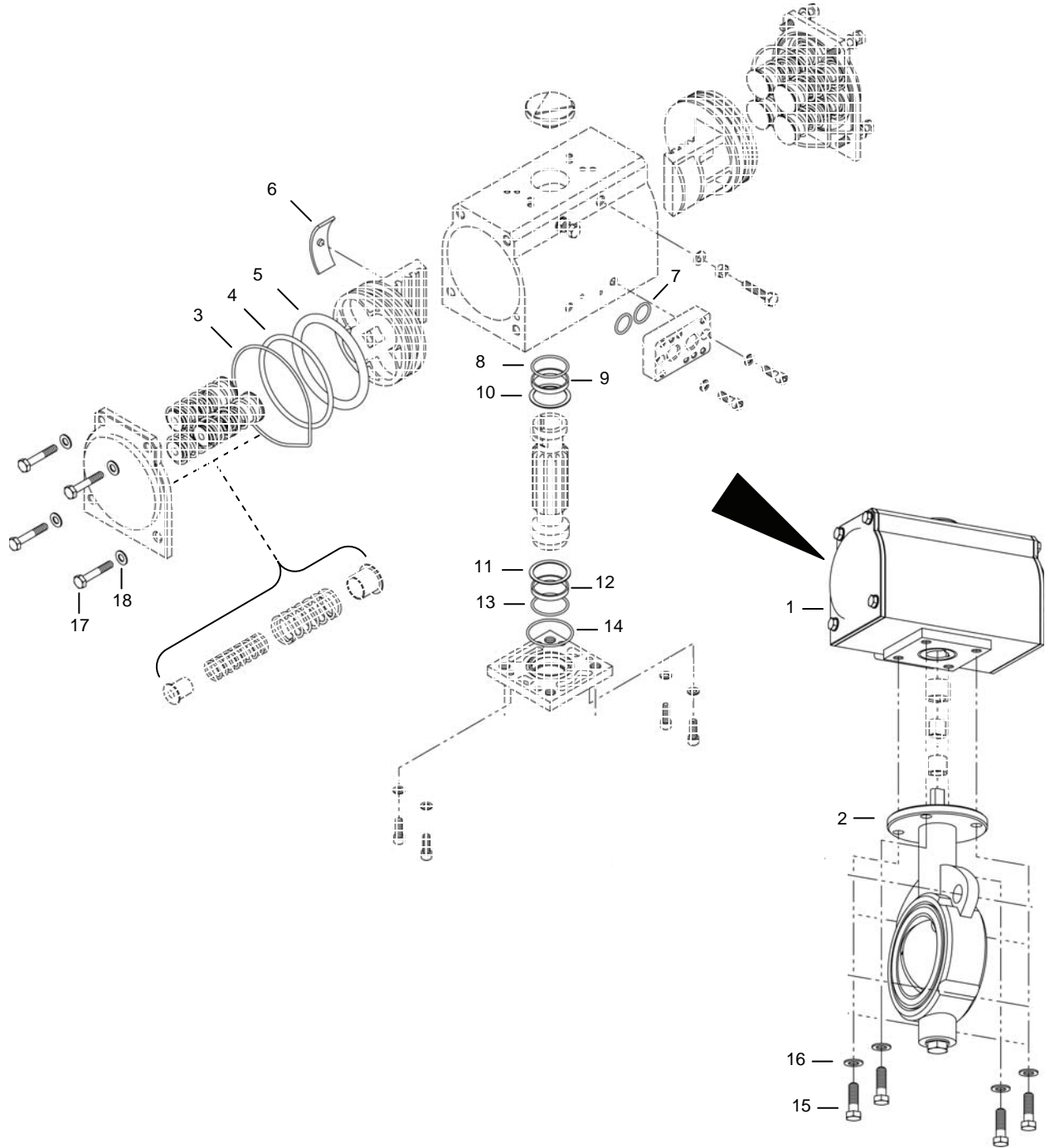
Figure 29. Valve Assembly V-112.
