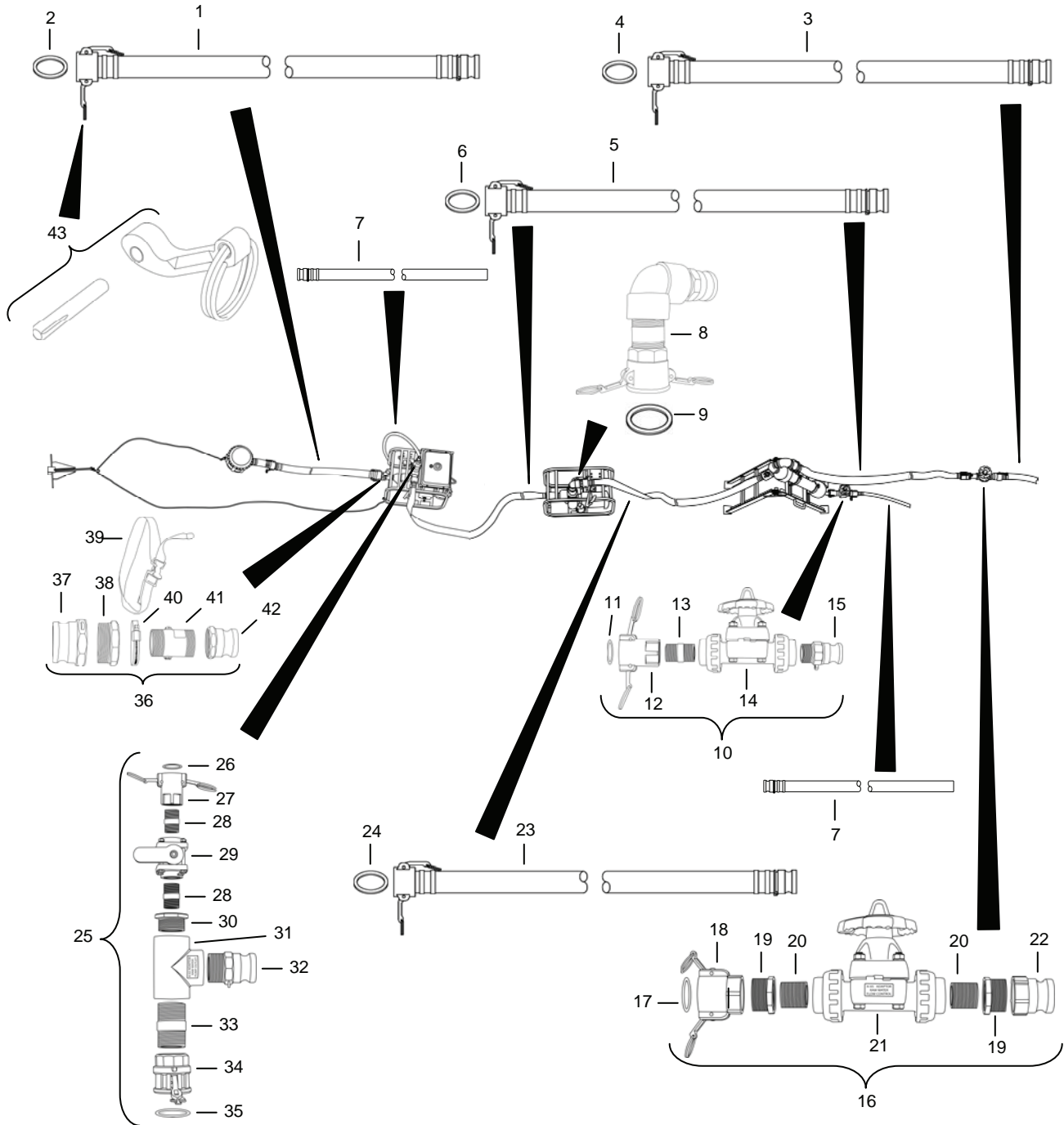
Figure 4. Hose Assemblies and Adaptors.
