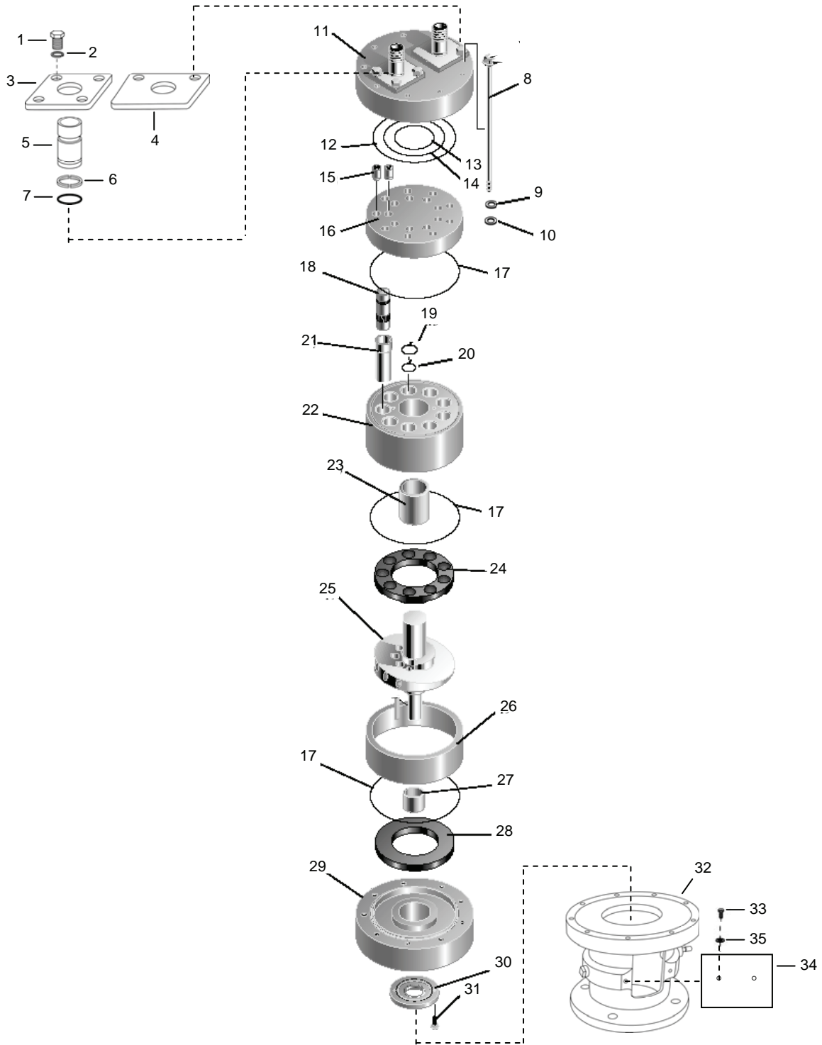
Figure 46. High-Pressure Pump (Sheet 1 of 2).
