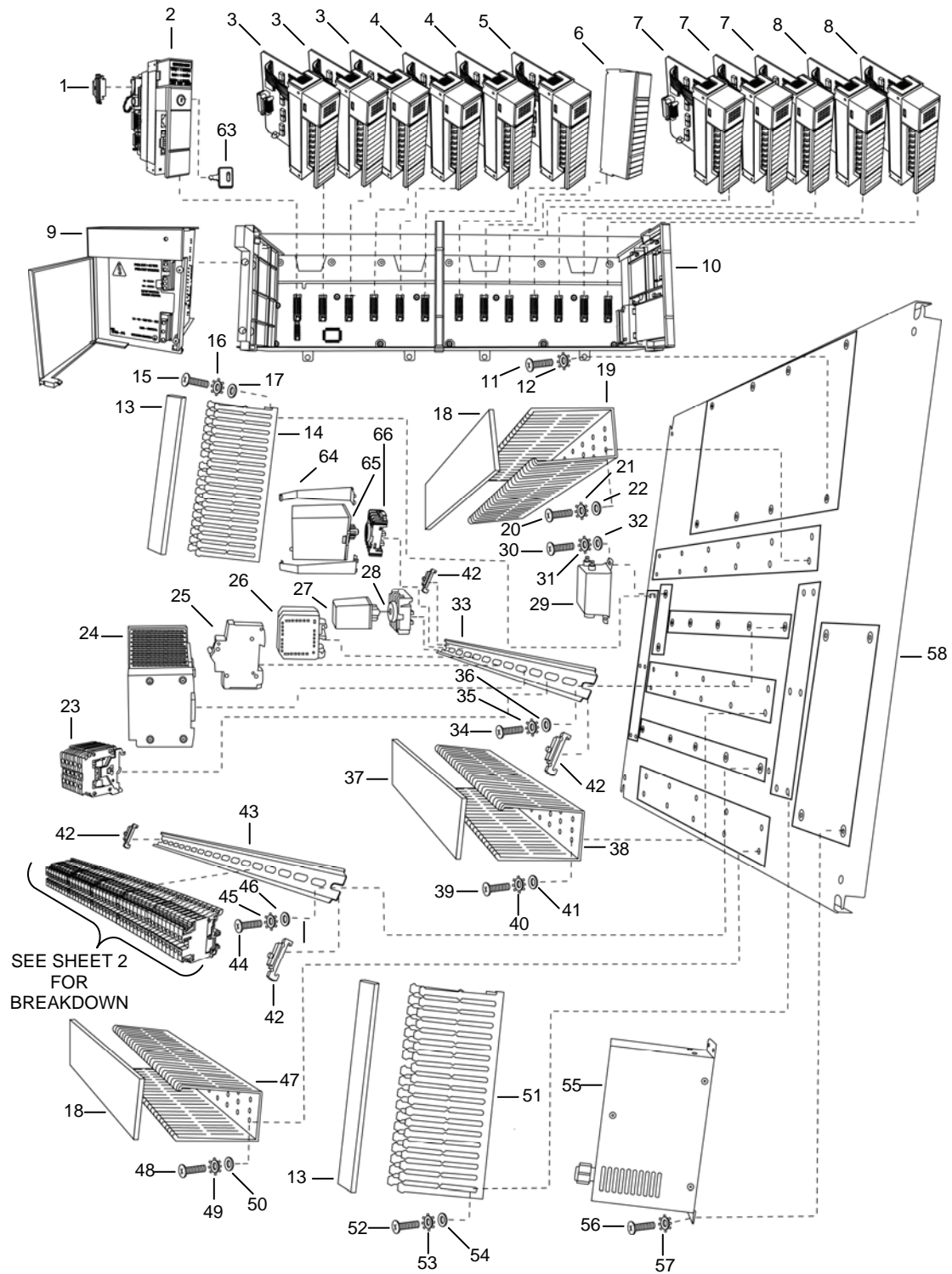
Figure 76. Sub Panel Assembly (Sheet 1 of 2).
