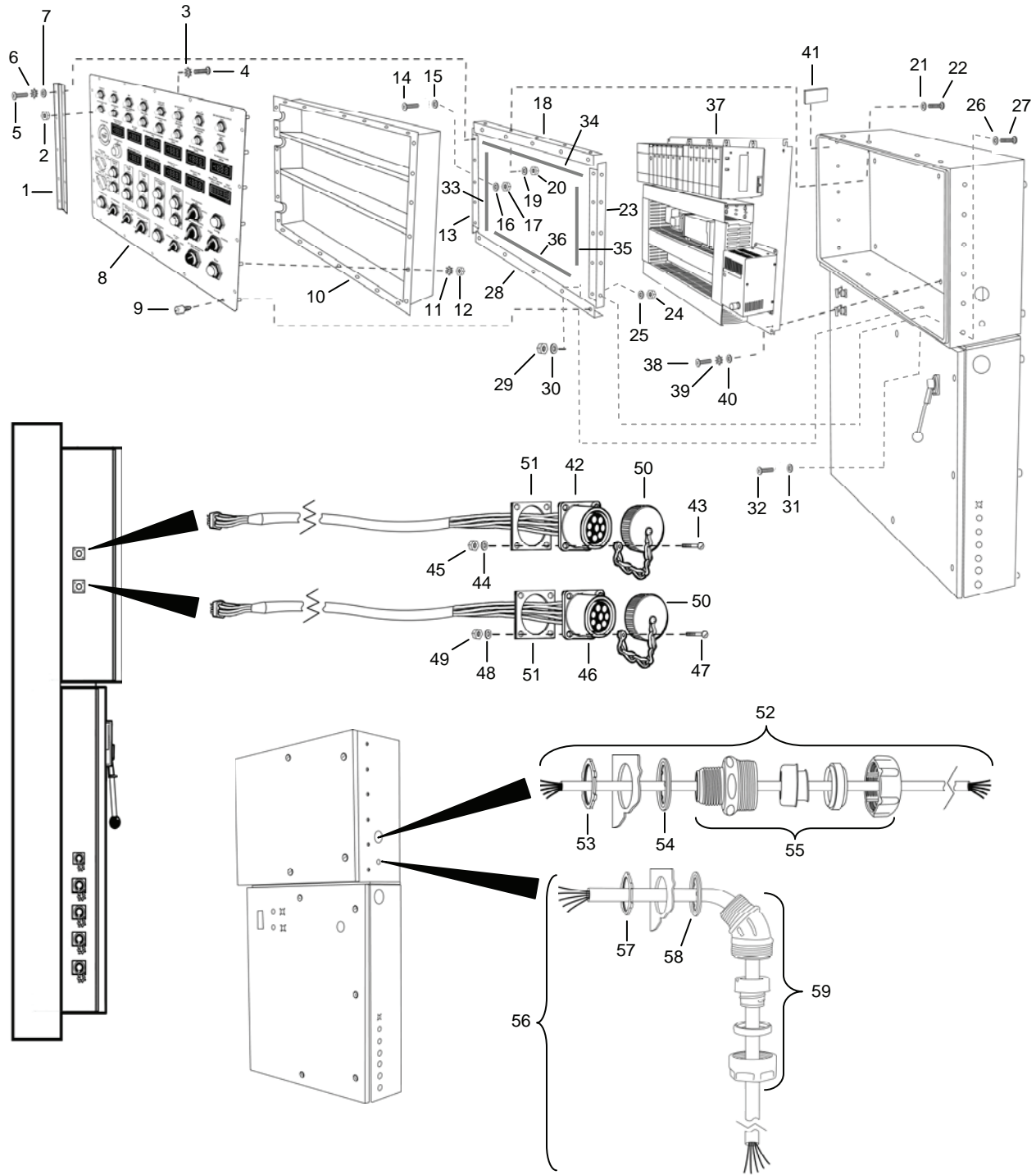
Figure 74. Operation Control System.
