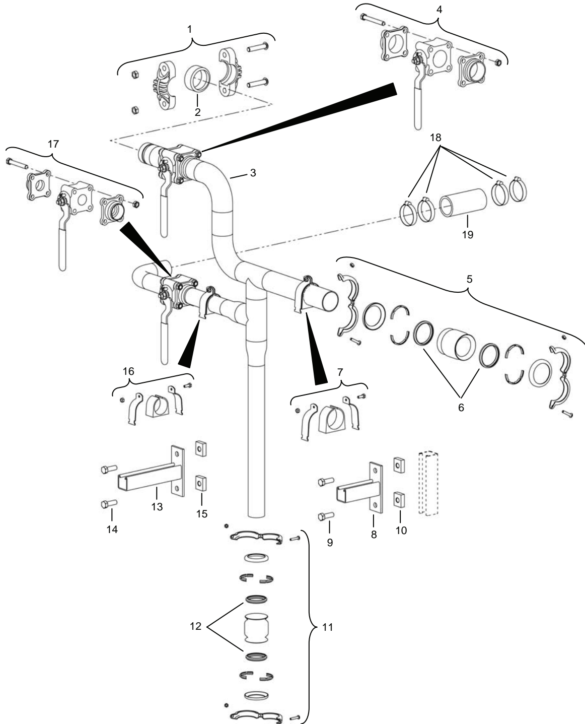
Figure 38. MF Piping Assembly C01.
