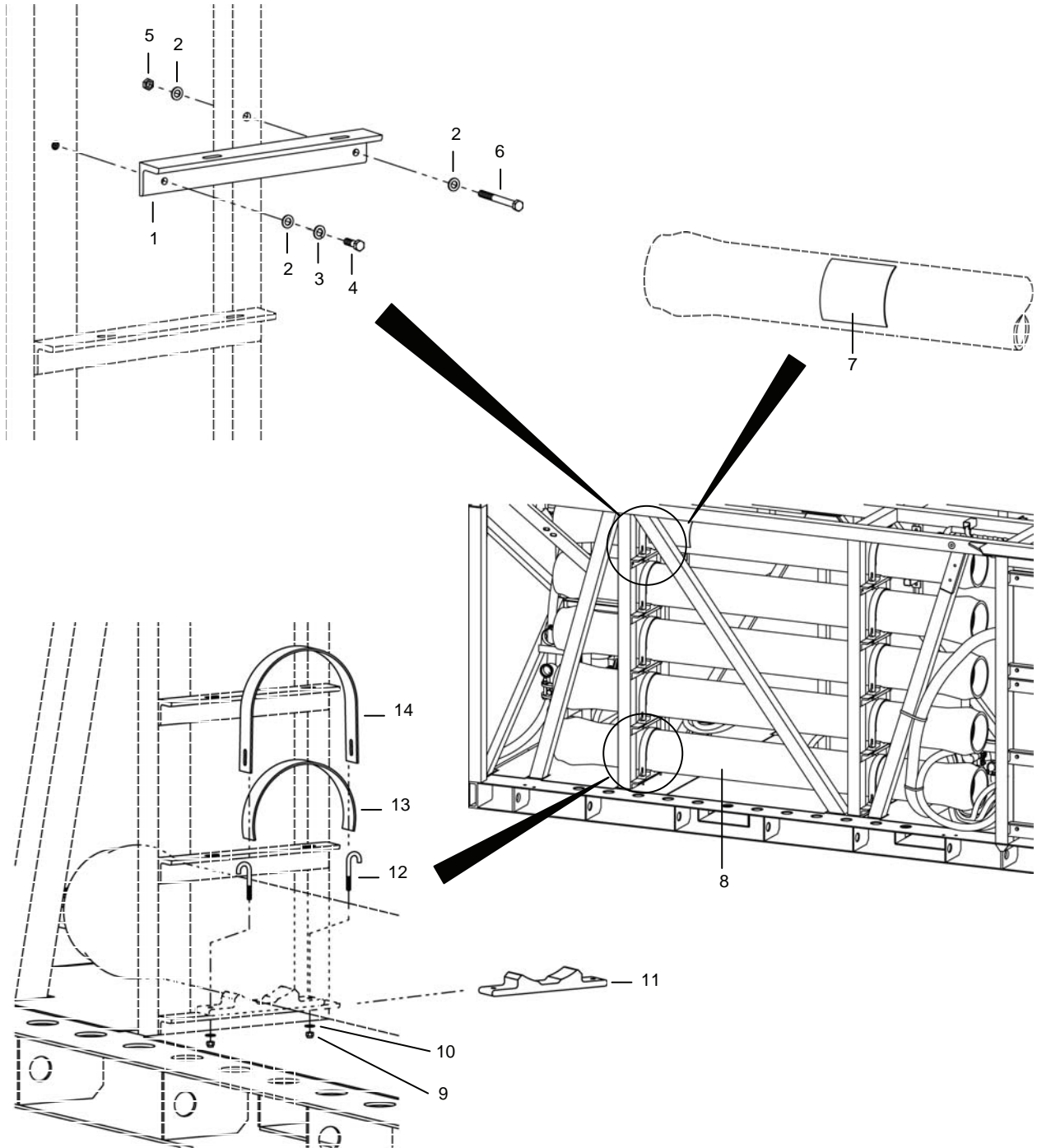
Figure 51. RO Vessel Installation.
