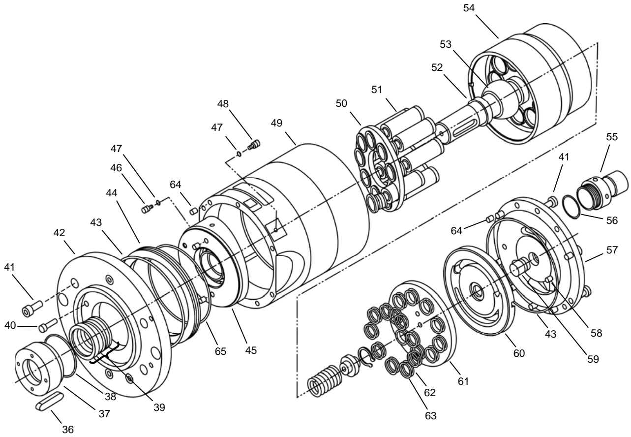
Figure 46. High-Pressure Pump (Sheet 2 of 2).
