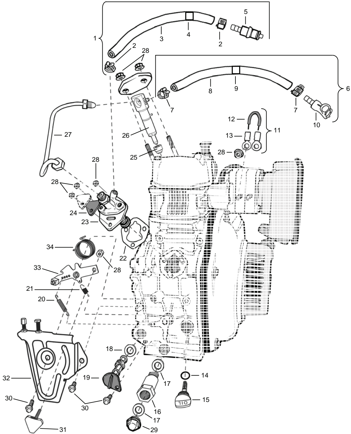
Figure 9. Fuel Injection and Oil Systems.
