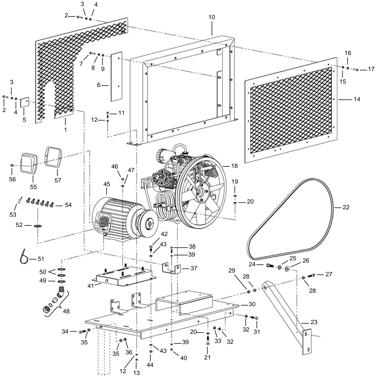
Figure 61. Air Compressor Assembly.
