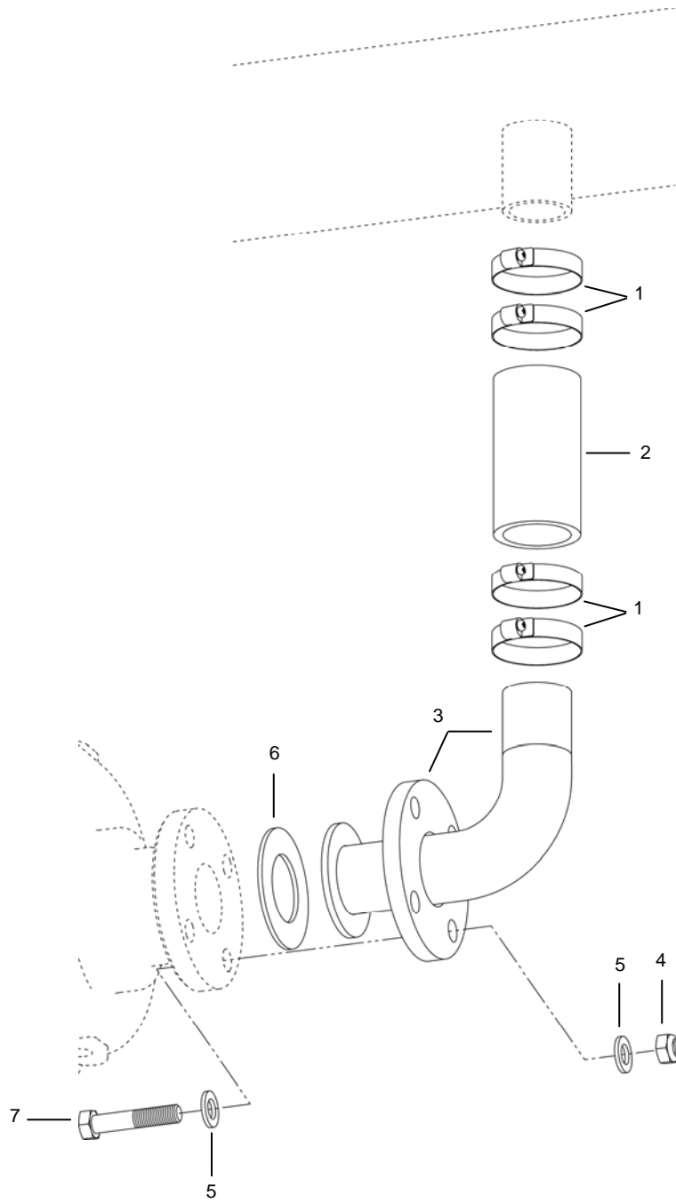
Figure 41. RO Piping Assembly M02.
