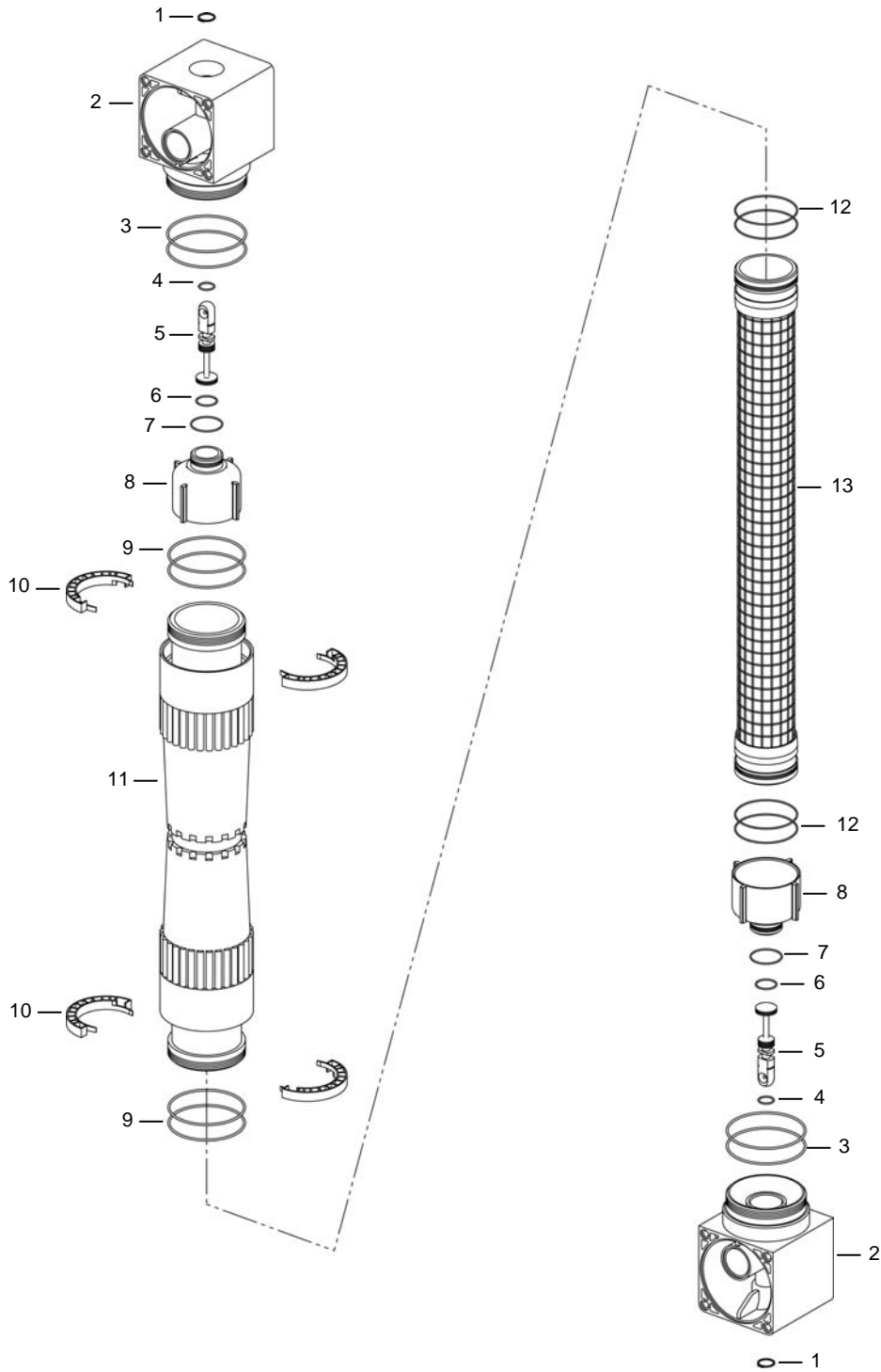
Figure 34. Filtration Module.
