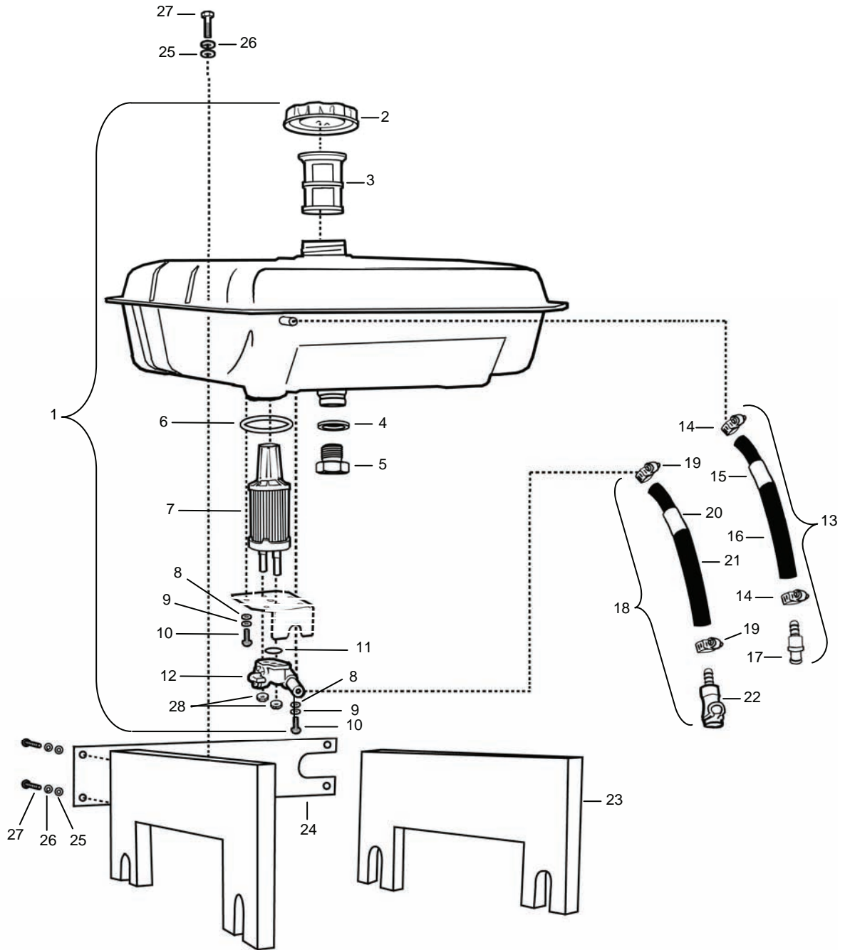
Figure 94. Fuel Tank Assembly.
