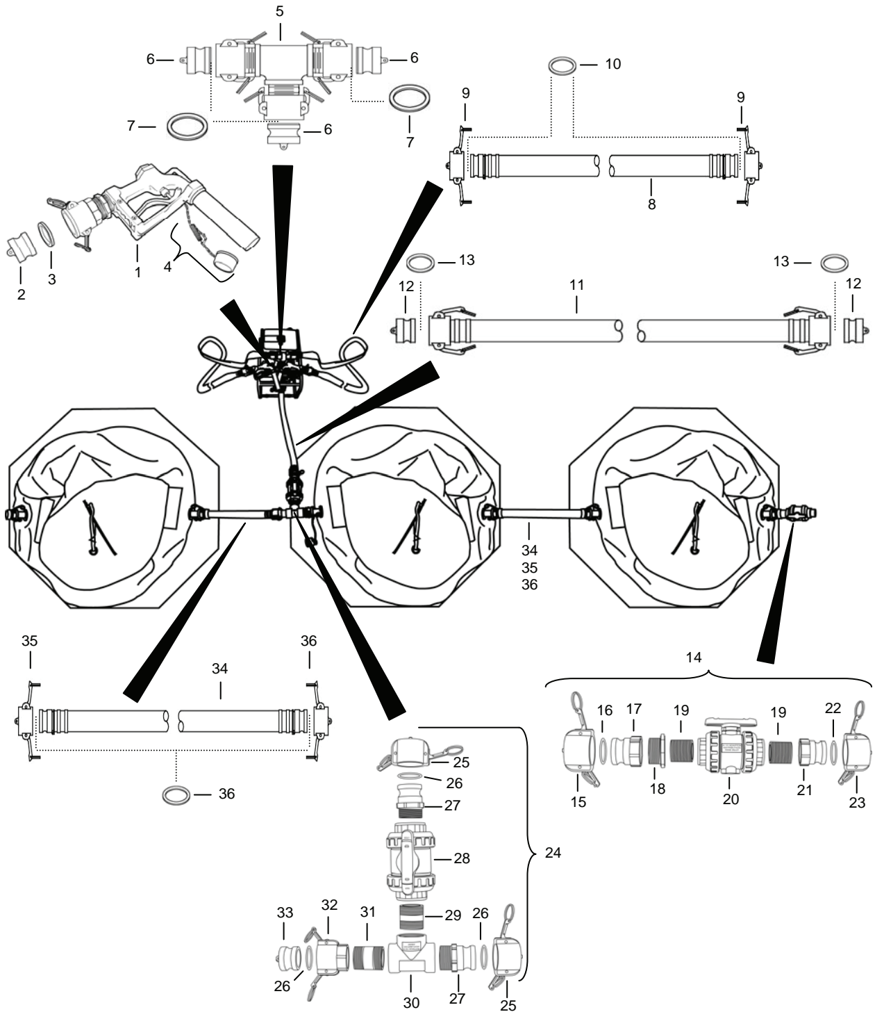
Figure 92. Extended Distribution System Hose Assemblies and Adaptors.
