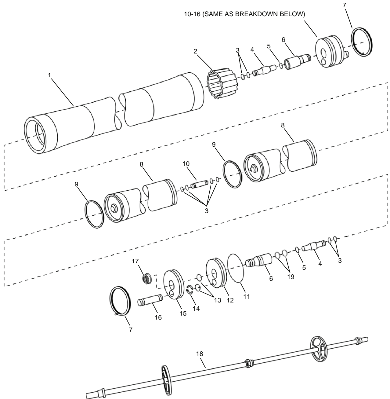
Figure 52. RO Vessel Assembly.
