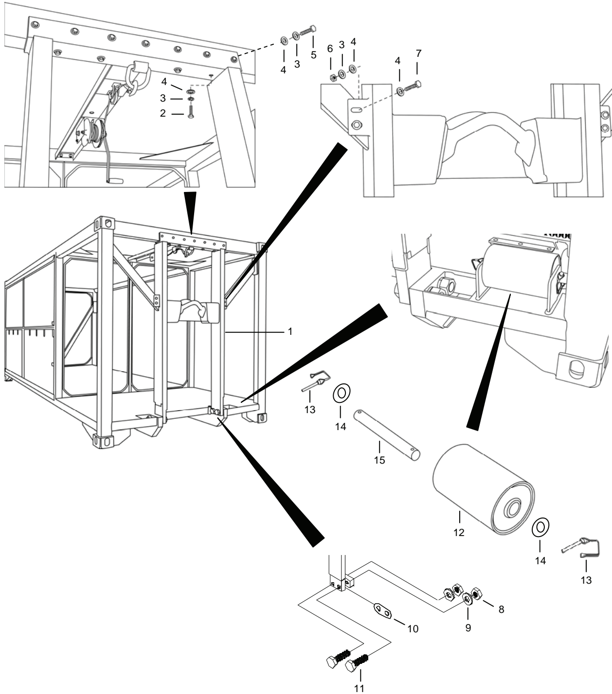
Figure 114. Bail Bar and Roller.
