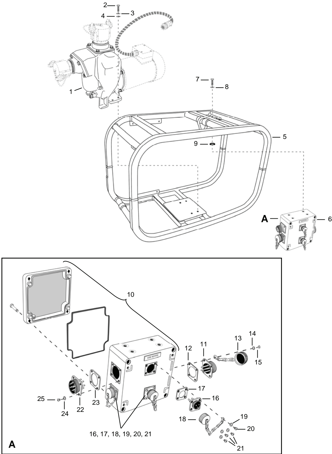
Figure 13. Electric Motor Driven Pump Assembly P-2.
