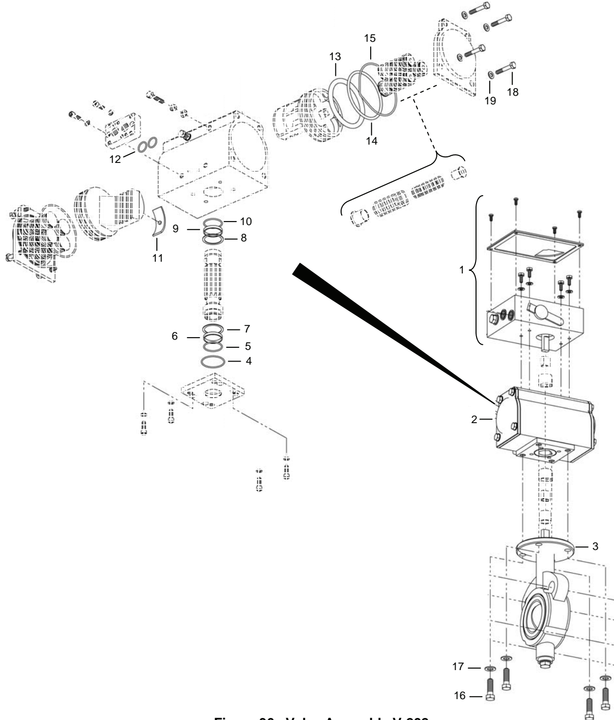
Figure 36. Valve Assembly V-202.
