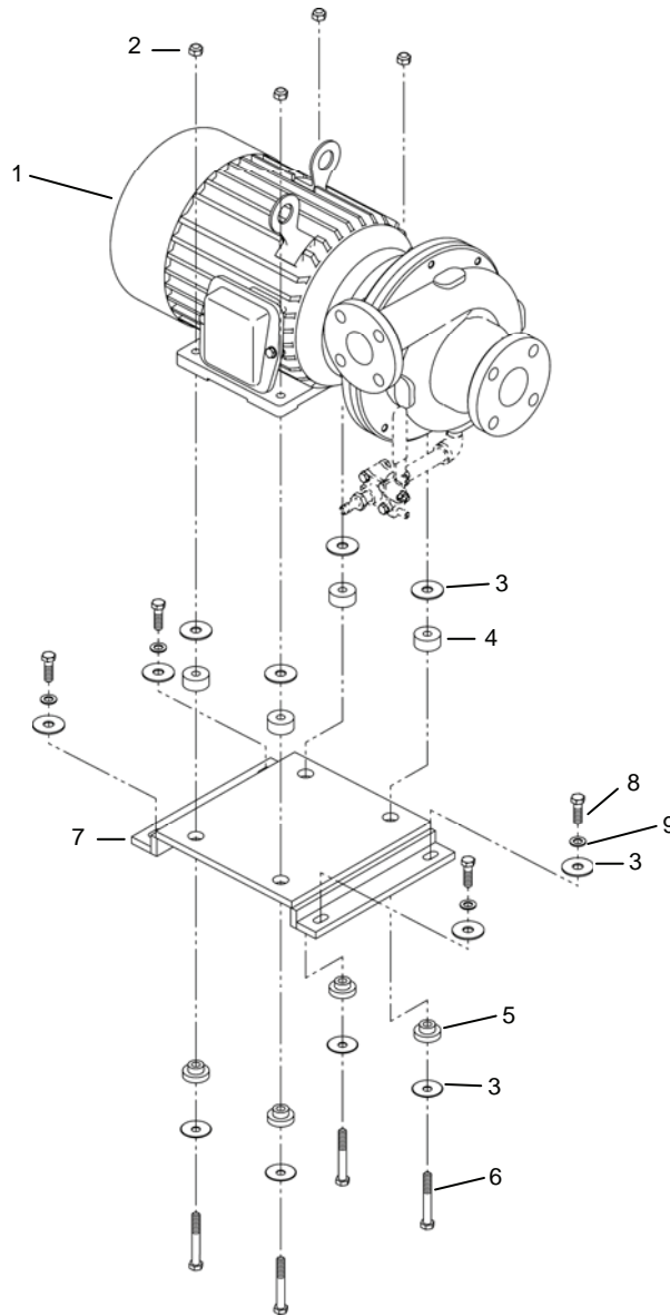
Figure 42. RO Feed Pump Assembly P-4.
