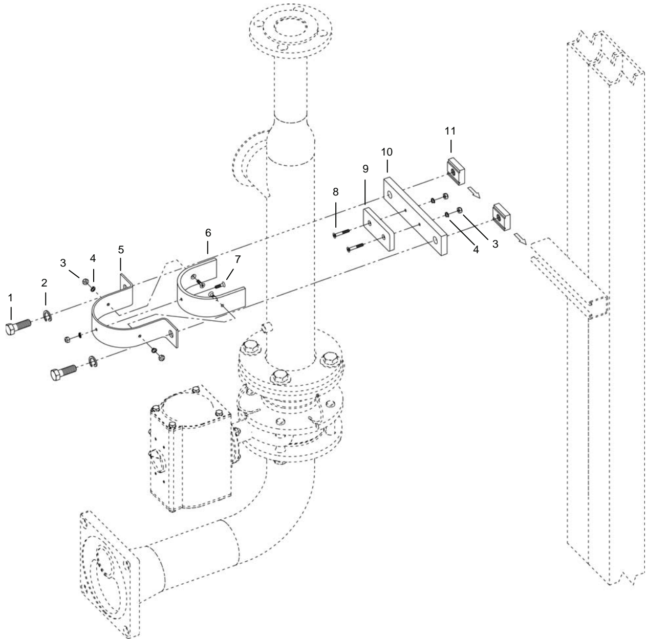
Figure 30. MF Pipe Restraint Assembly.
