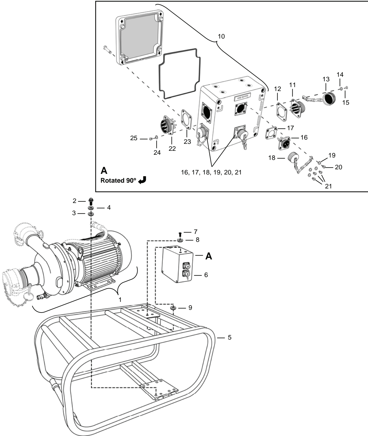
Figure 23. MF Feed Pump Assembly P-3.
