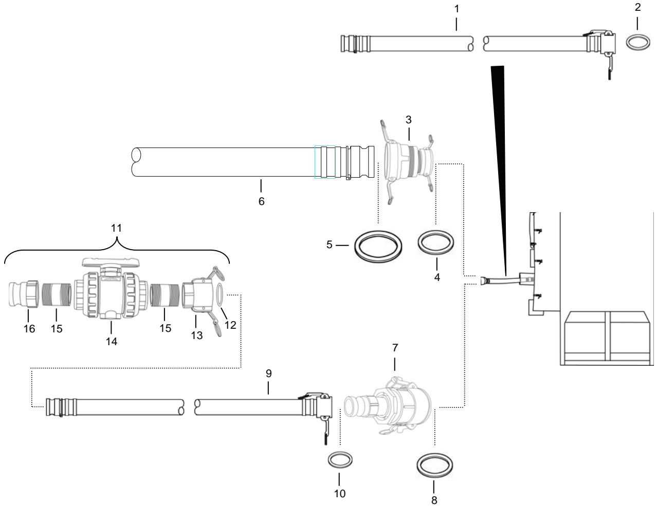
Figure 116. Waste Discharge System Hose Assemblies and Adaptors.
