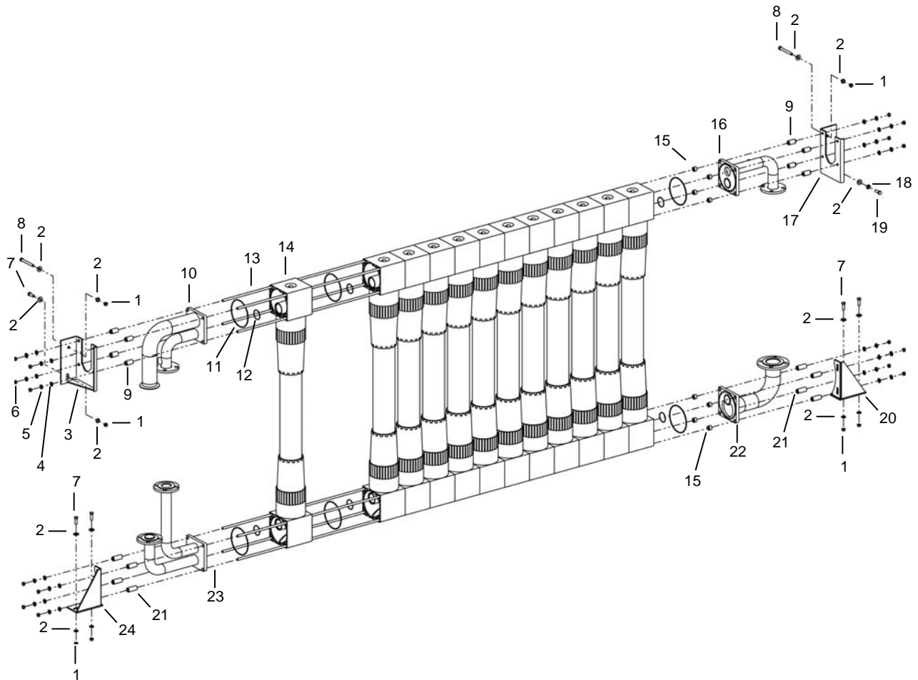
Figure 33. MF Filter Module Assembly (Rear View).
