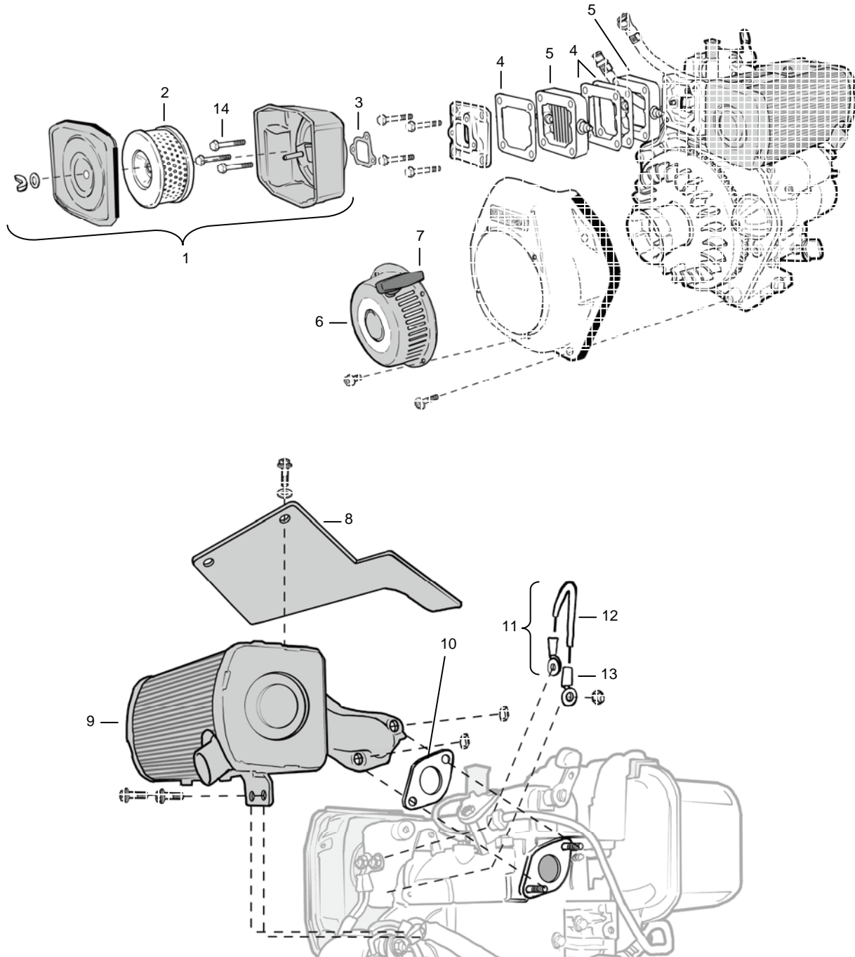
Figure 8. Air Cleaner, Hand Starter, and Muffler.
