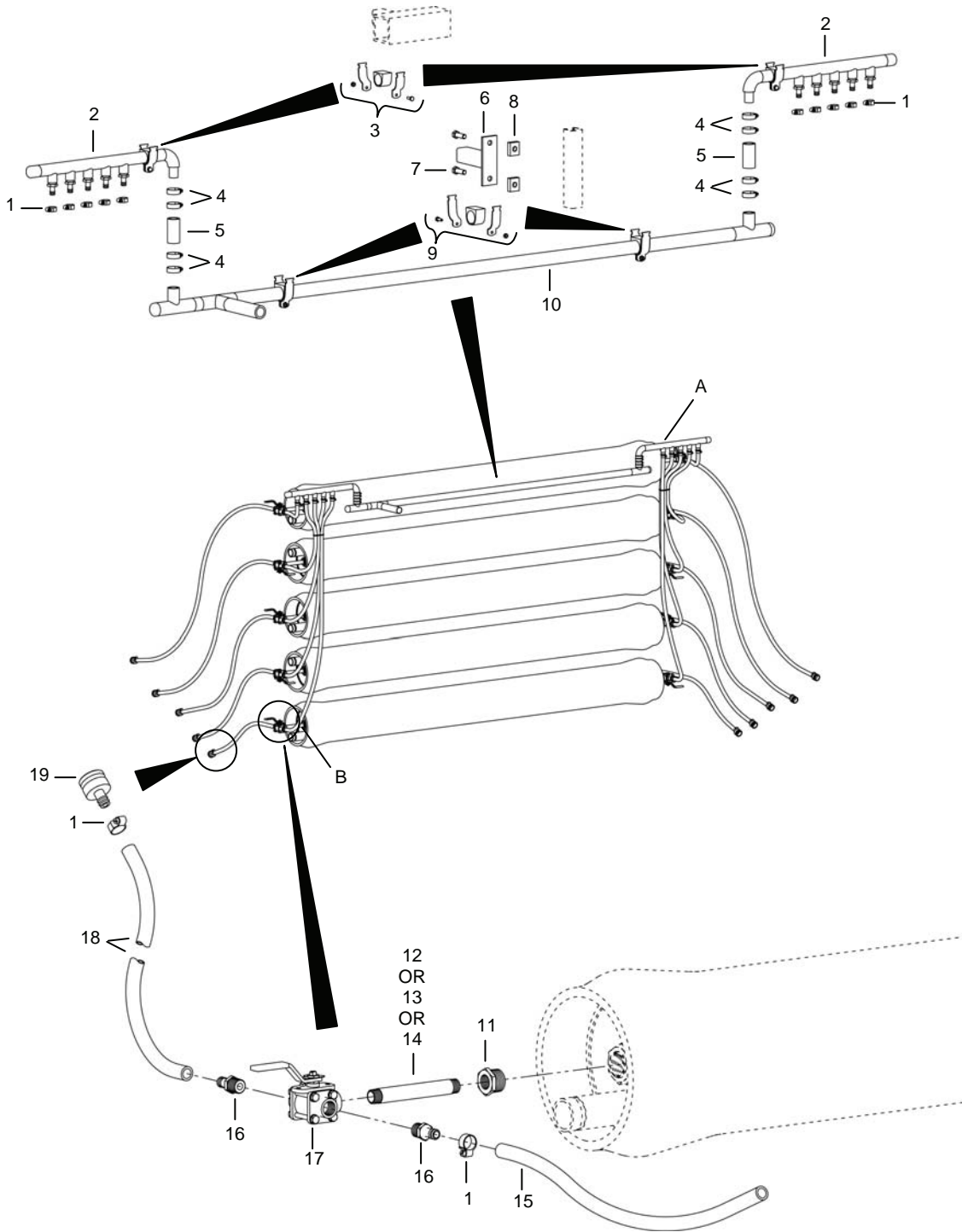
Figure 56. RO Piping Assembly P01 Manifold.
