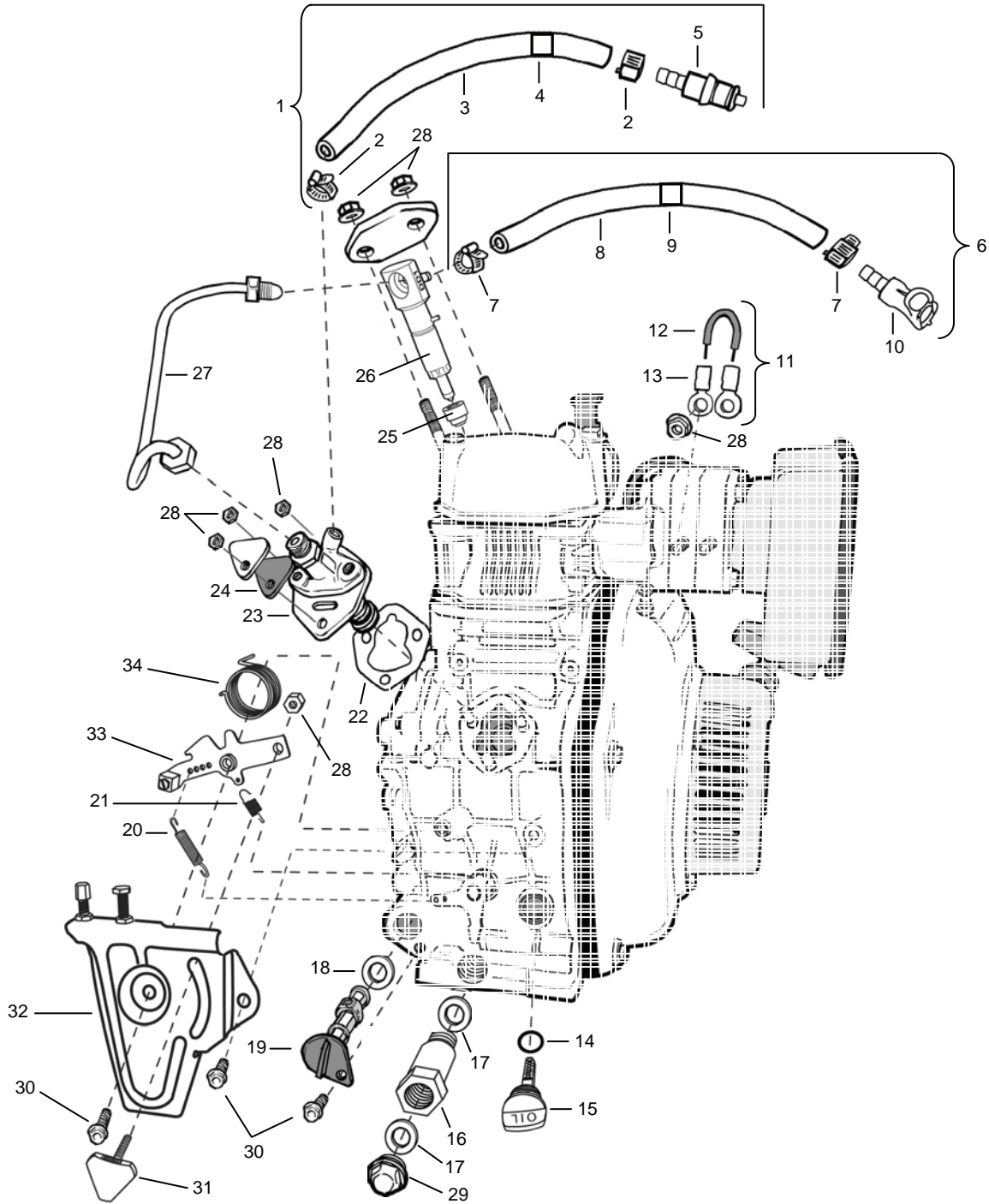
Figure 97. Fuel Injection and Oil Systems.
