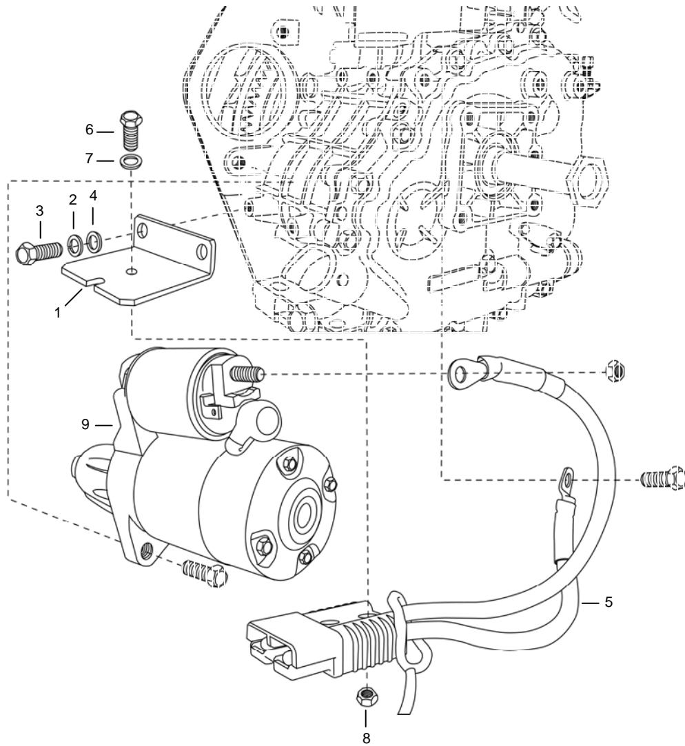
Figure 10. Electric Starter System.
