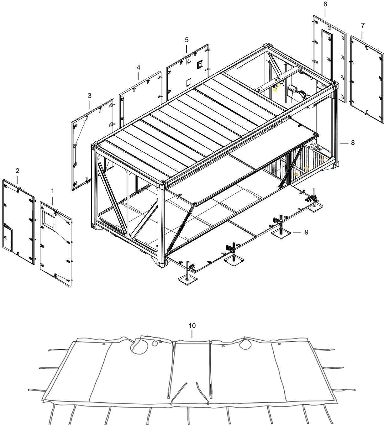
Figure 101. Flat Rack Assembly.
