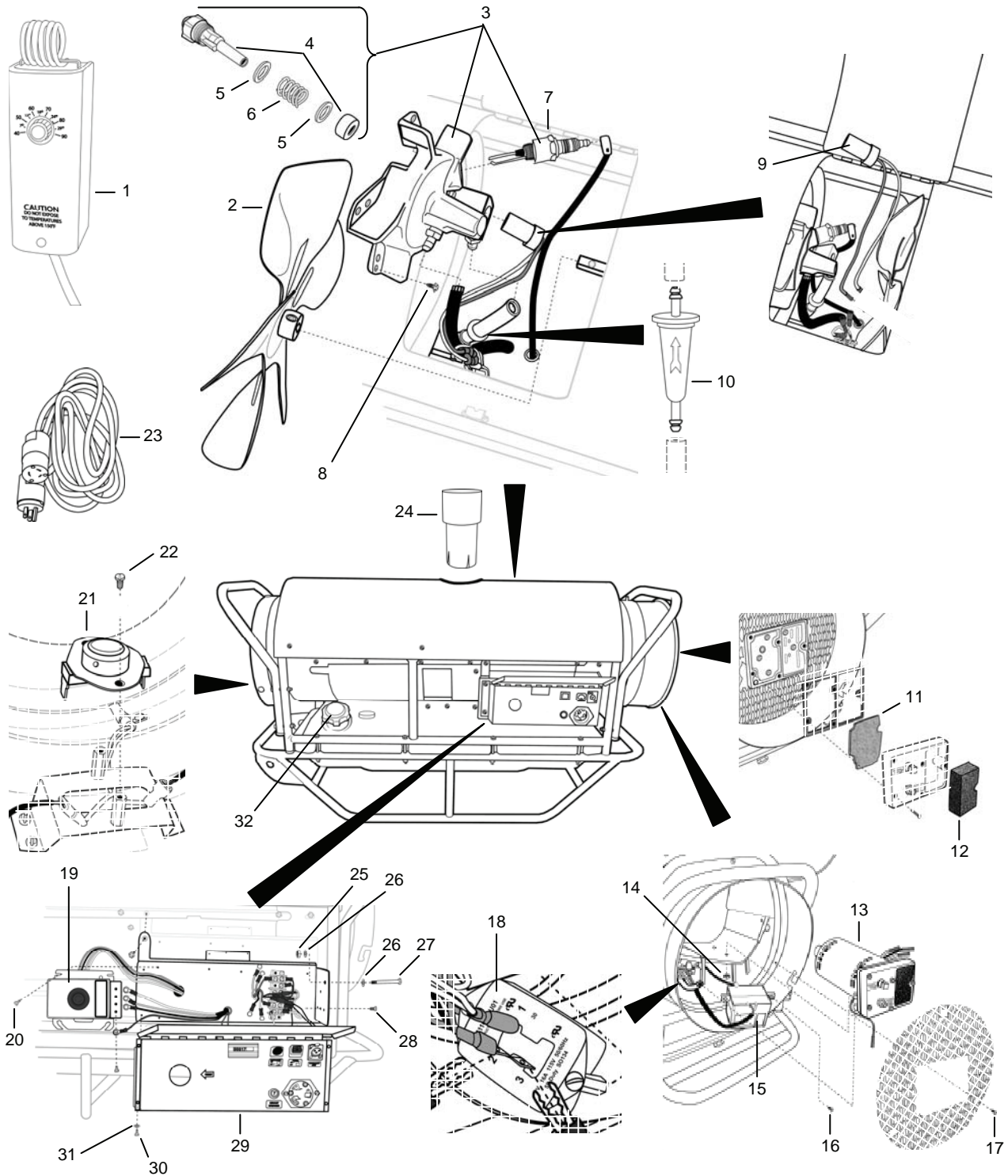
Figure 86. Space Heater.
