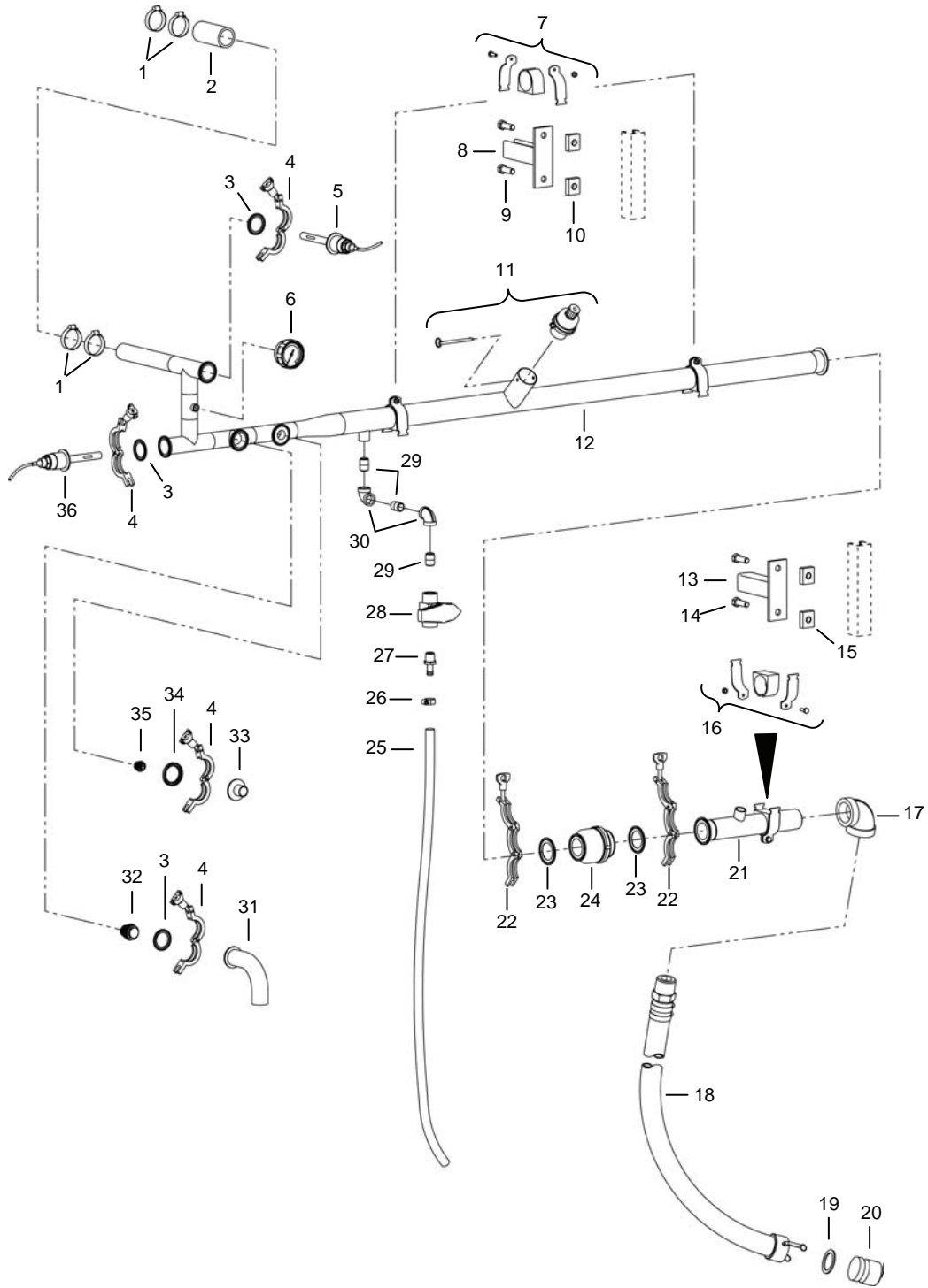
Figure 57. RO Piping Assembly P01 Outlet.
