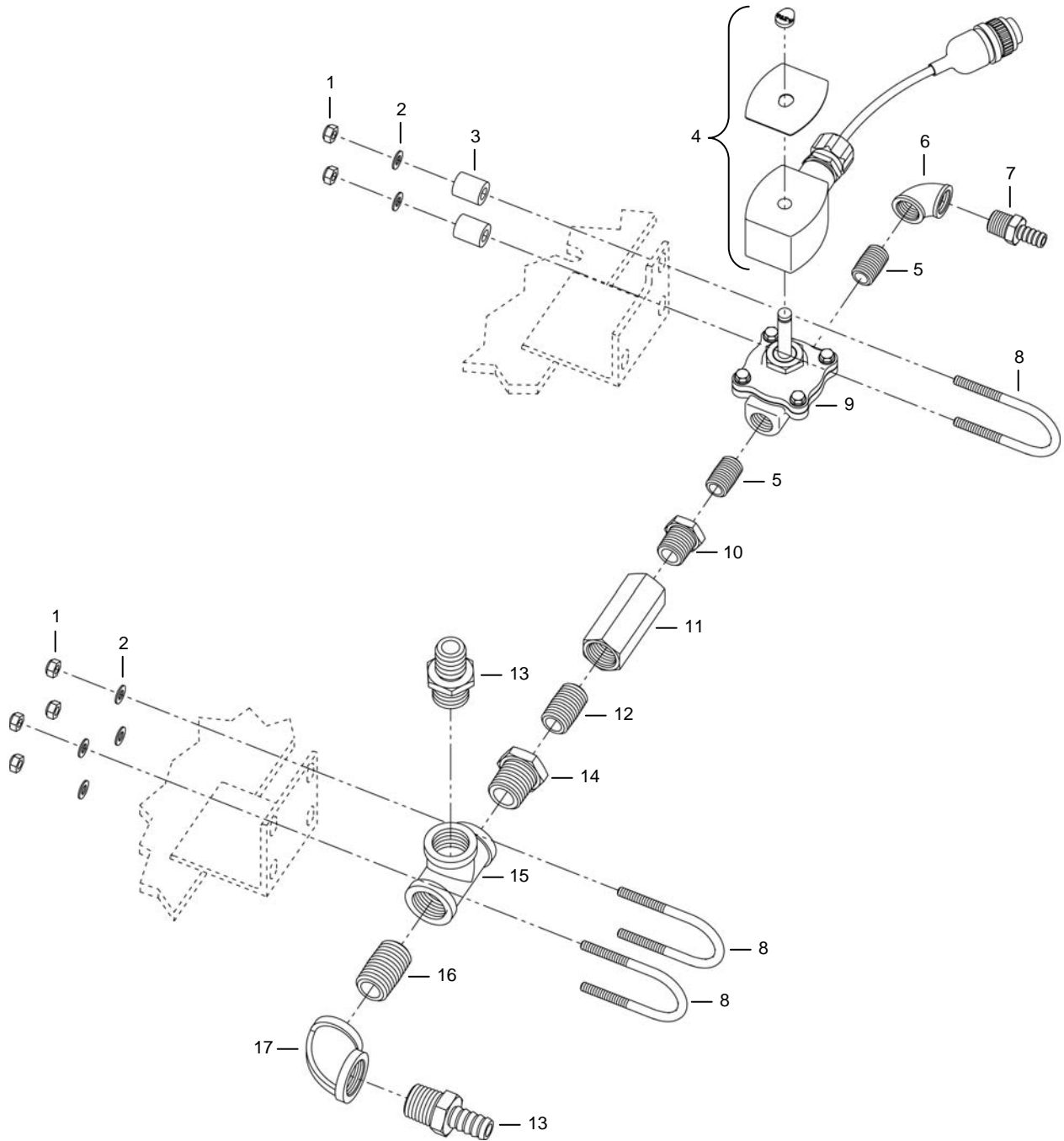
Figure 68. Air System Section 4.
