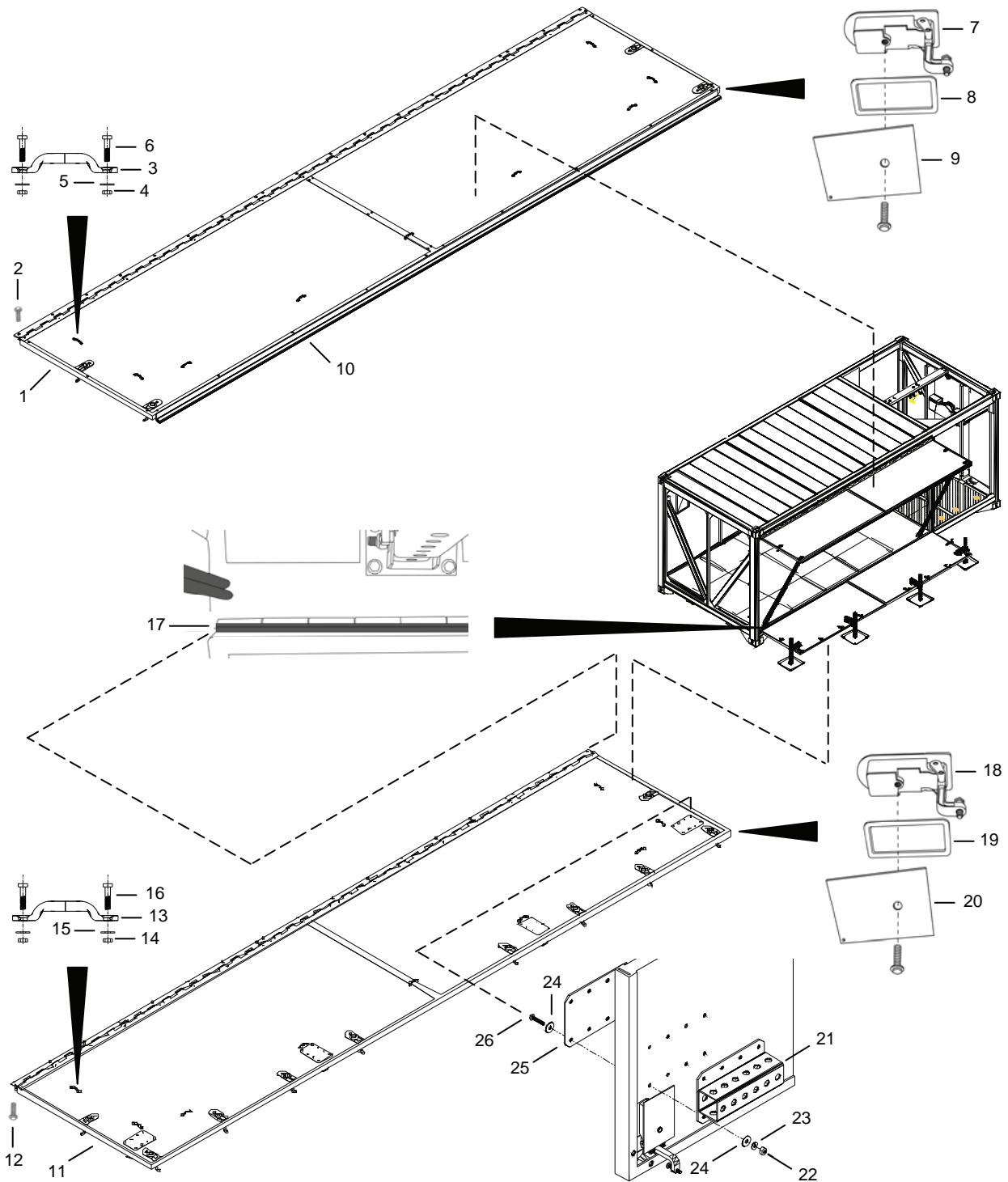
Figure 110. Upper and Lower Panel Assemblies.
