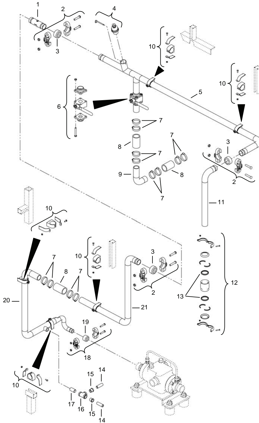
Figure 55. RO Piping Assembly R03.
