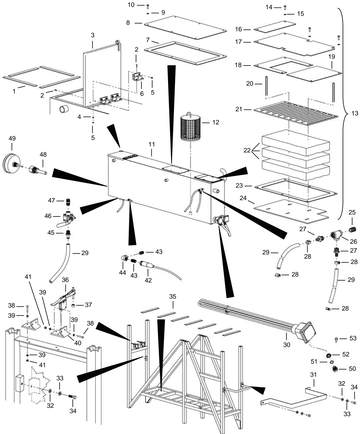
Figure 40. RO Feed Tank Assembly T-2.
