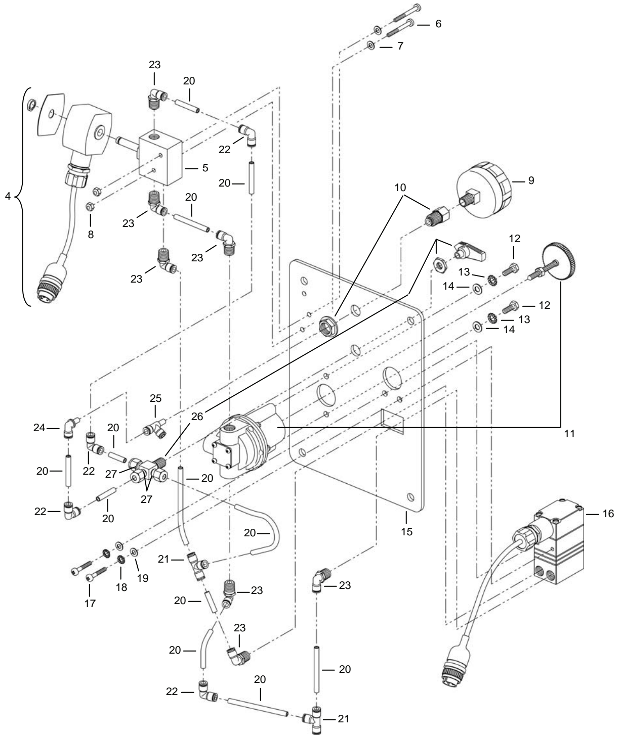
Figure 70. Feed Flow Control Panel Assembly (Sheet 2 of 2).
