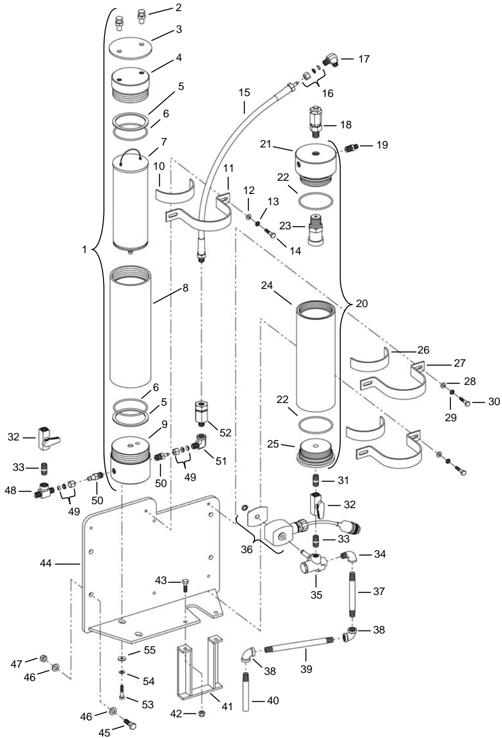
Figure 63. AF2 - CO1 Assembly.
