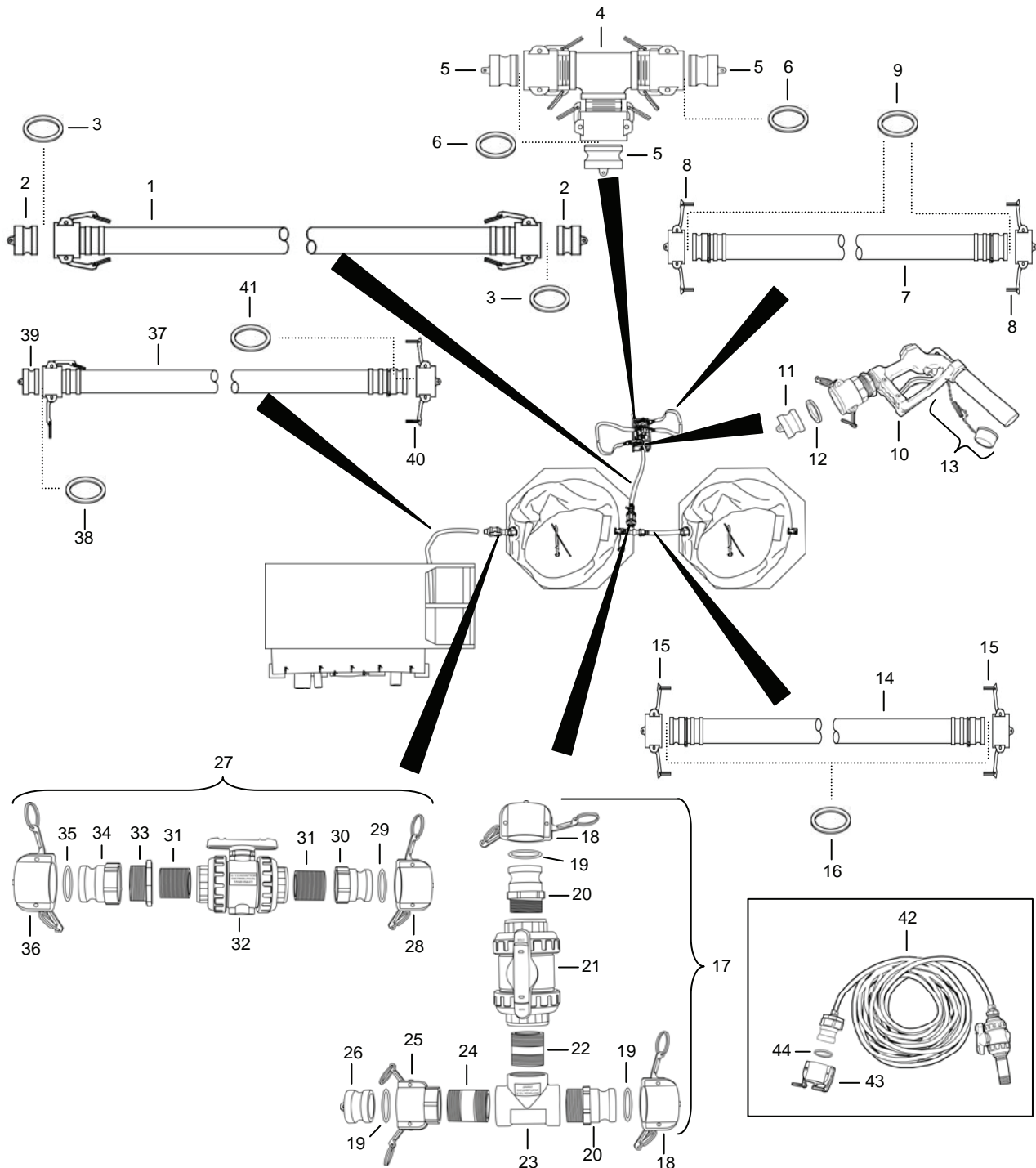
Figure 17. Hose Assemblies and Adaptors.
