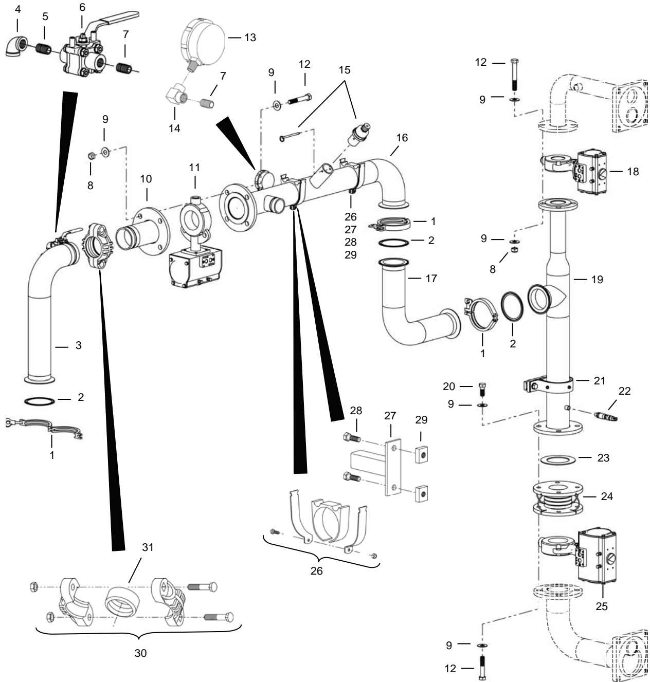
Figure 27. MF Piping Assembly F11.
