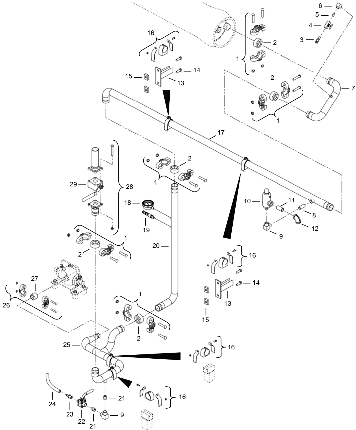
Figure 50. RO Piping Assembly H03.
