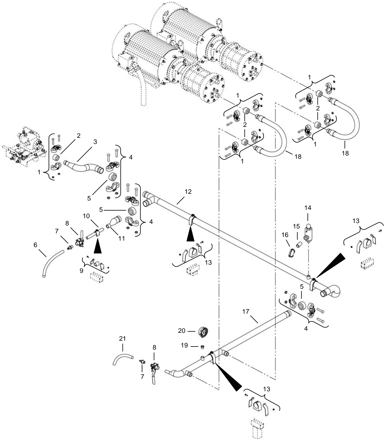
Figure 47. RO Piping Assembly H01.
