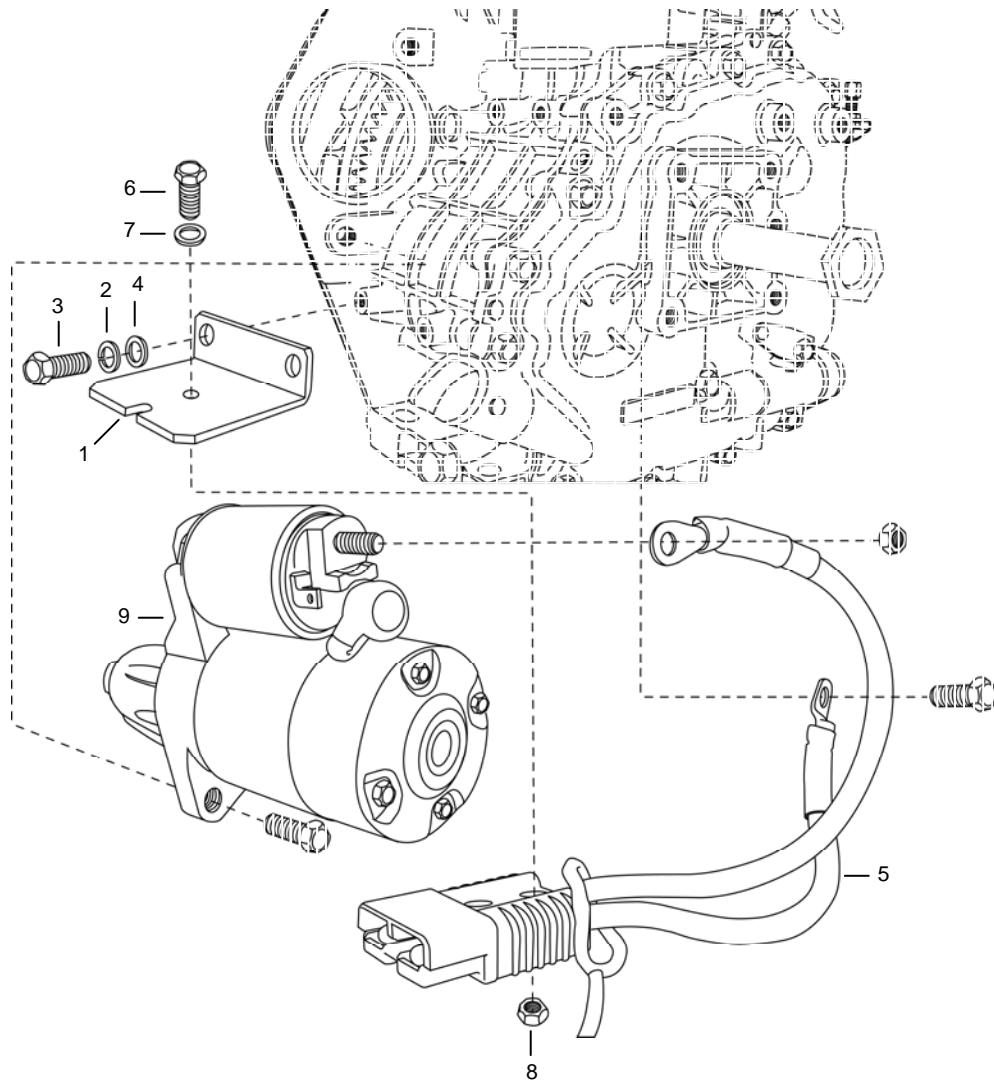
Figure 98. Electric Starter System.
