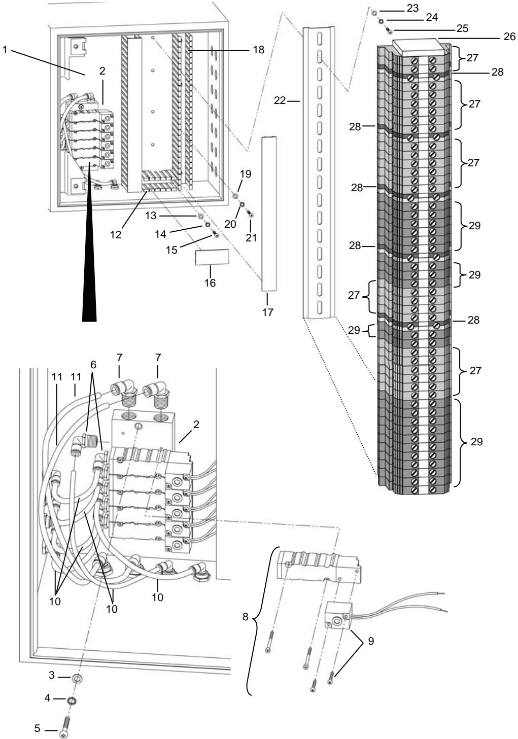
Figure 82. Solenoid Panel.
