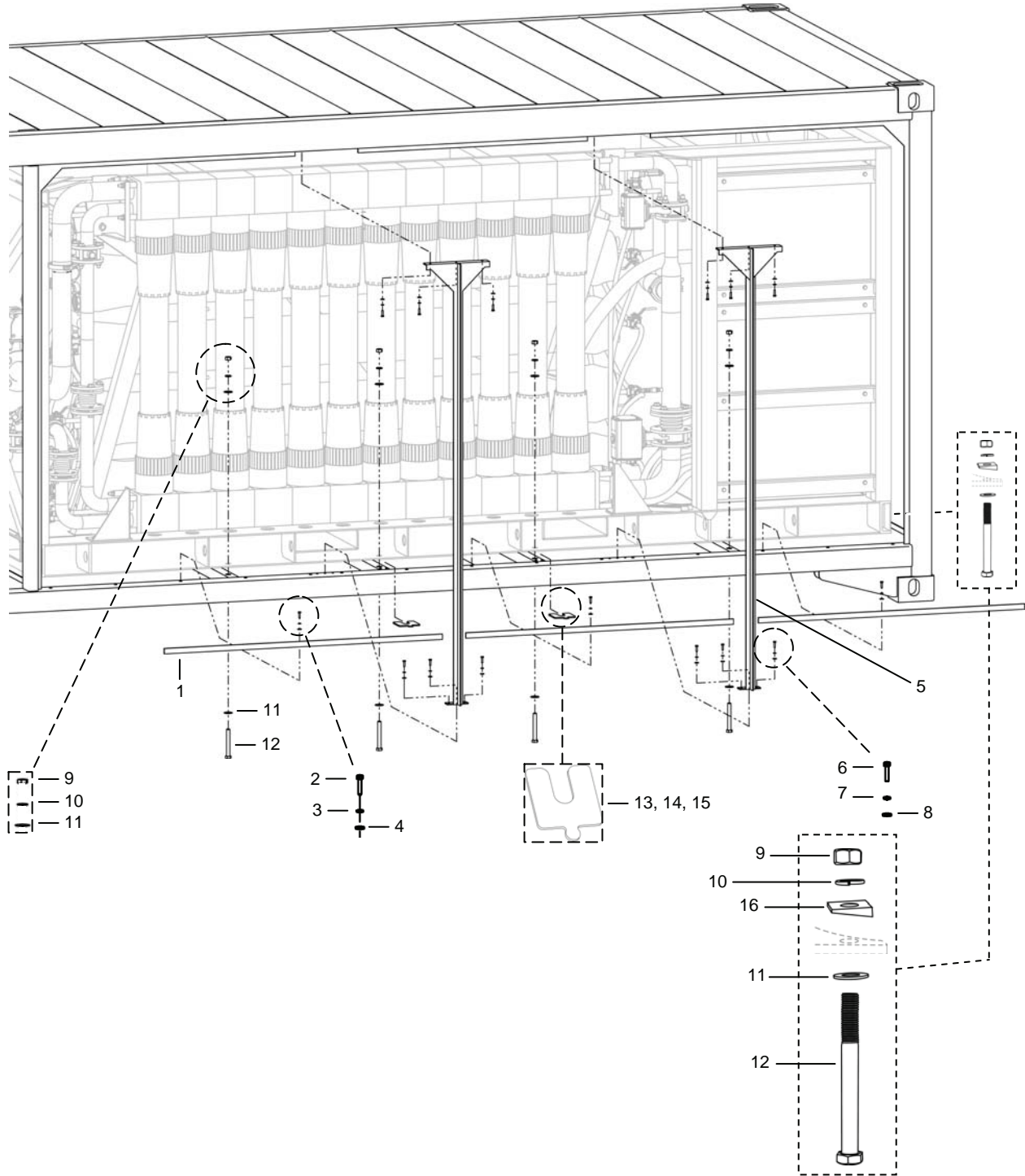
Figure 115. Panel Divider, Bottom Jamb, and TWPS and TQG Mounting Hardware (Sheet 1 of 2).
