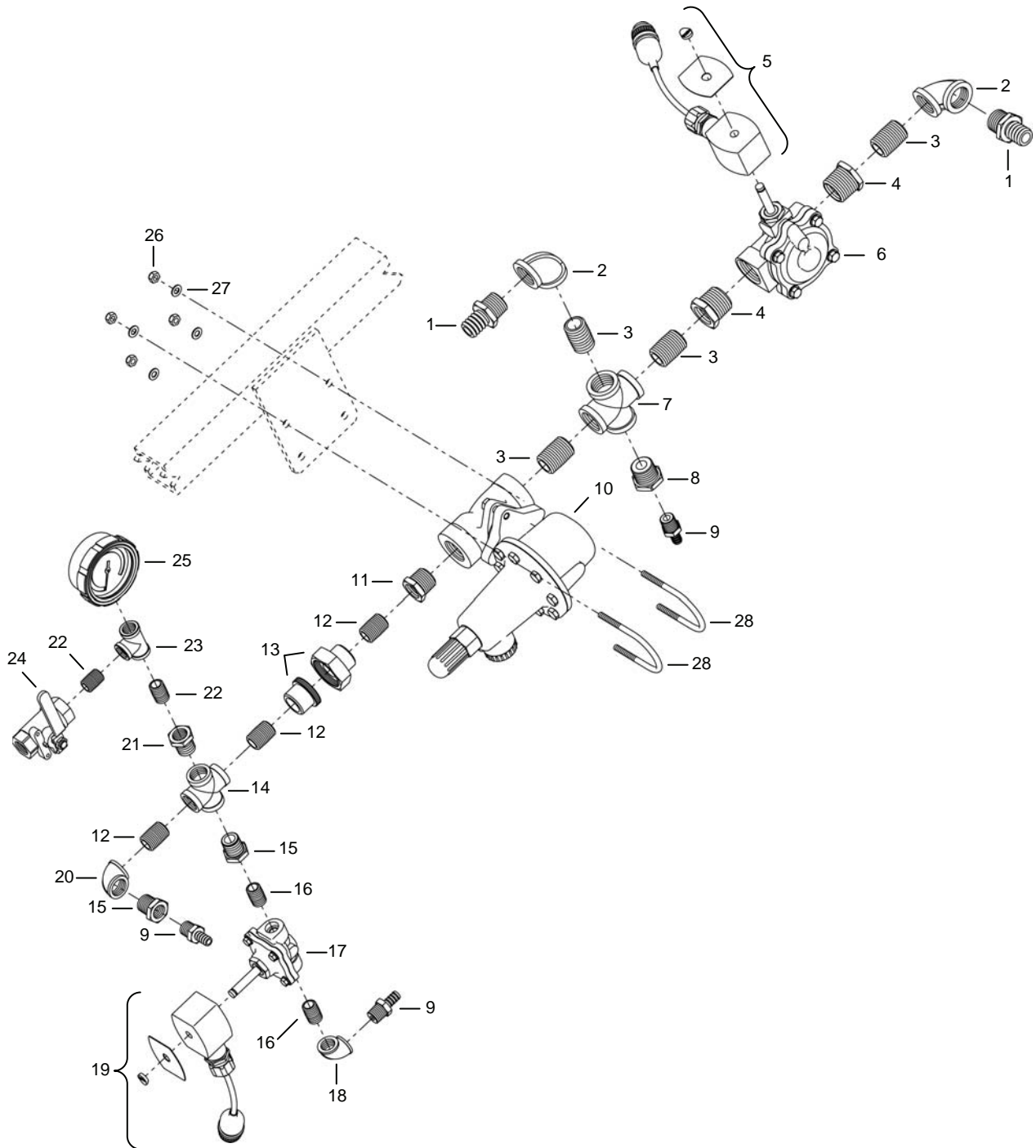
Figure 67. Air System Section 3.
