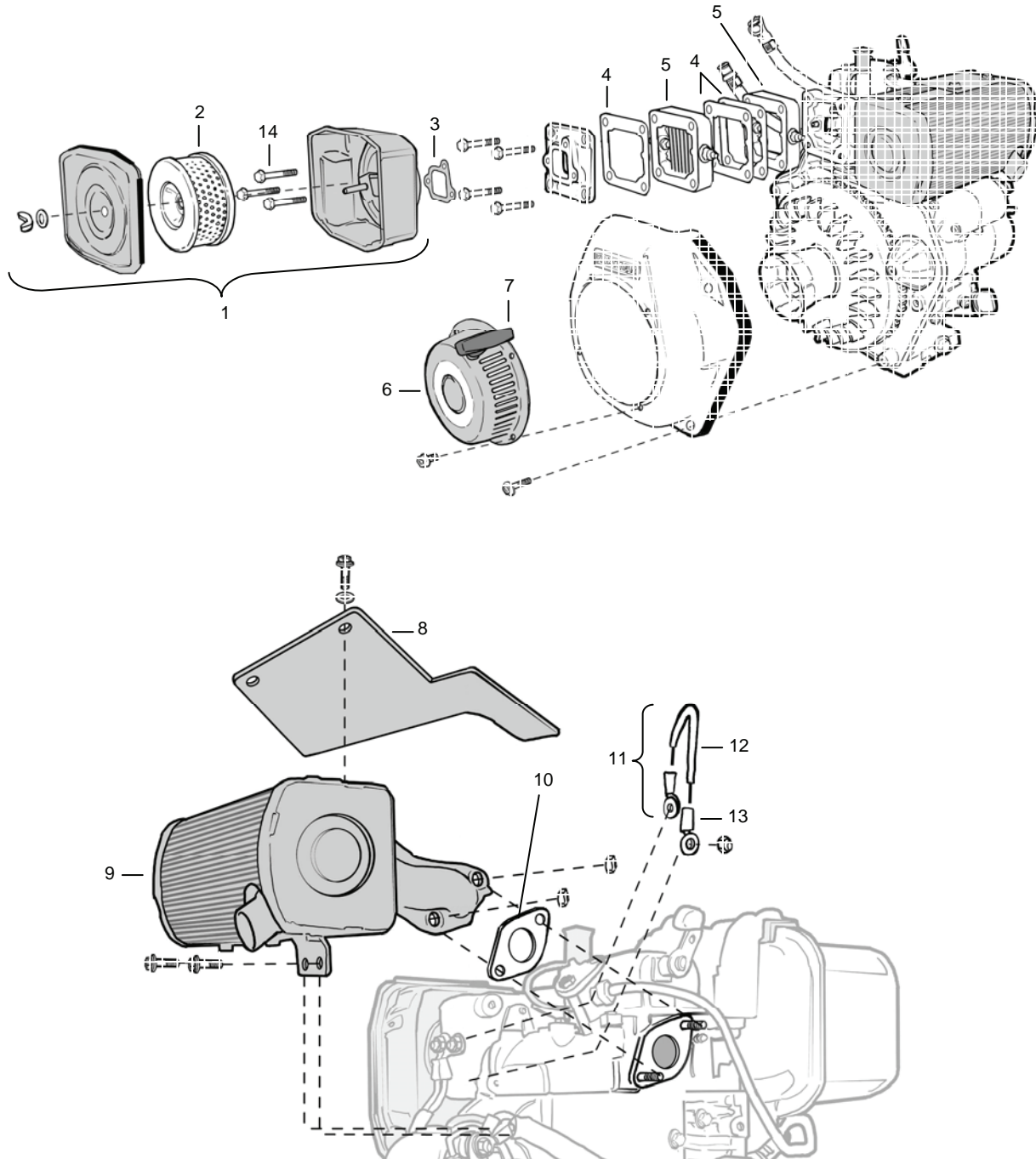
Figure 96. Air Cleaner, Hand Starter, and Muffler.
