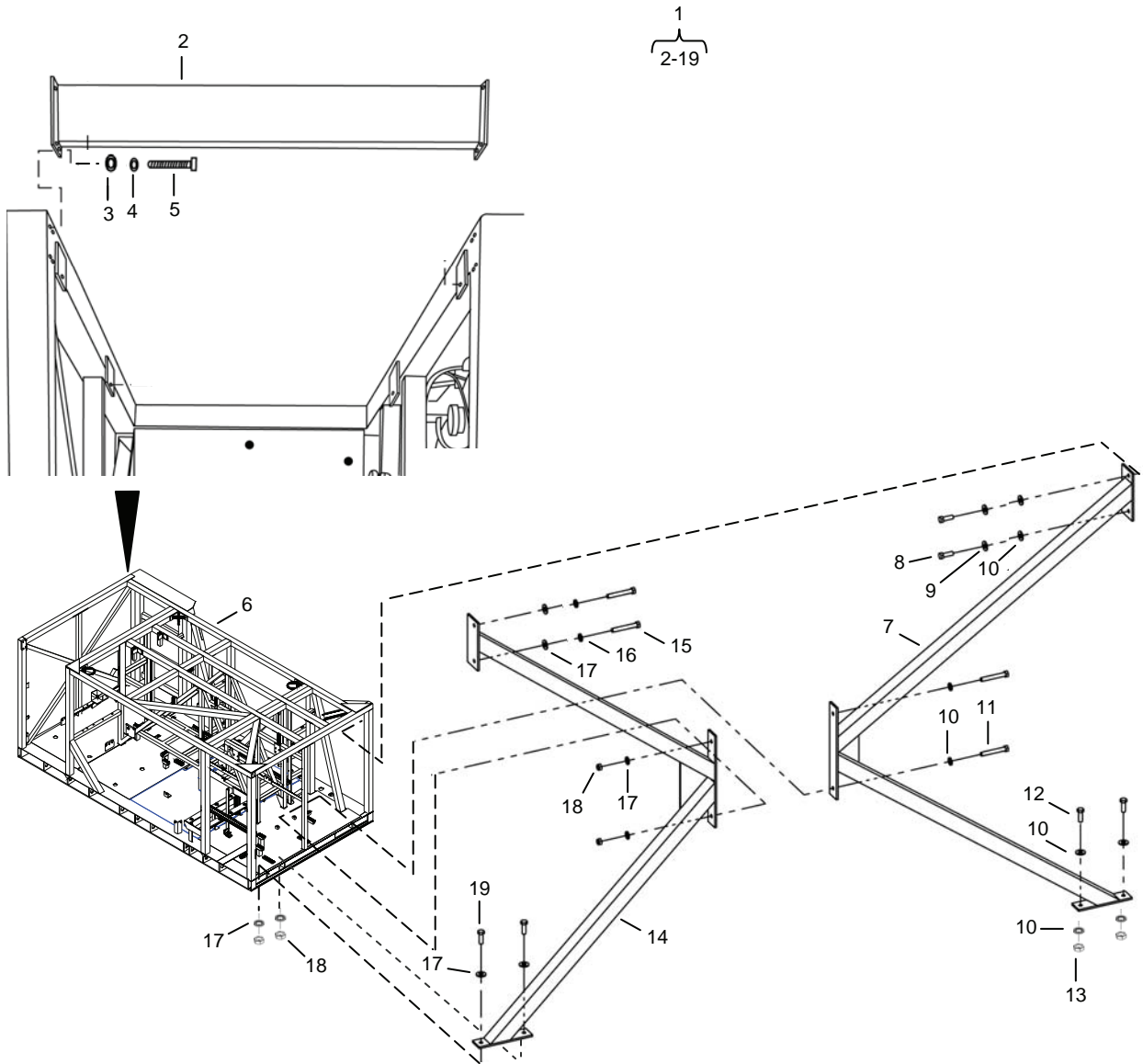
Figure 84. Army TWPS Skid Assembly.
