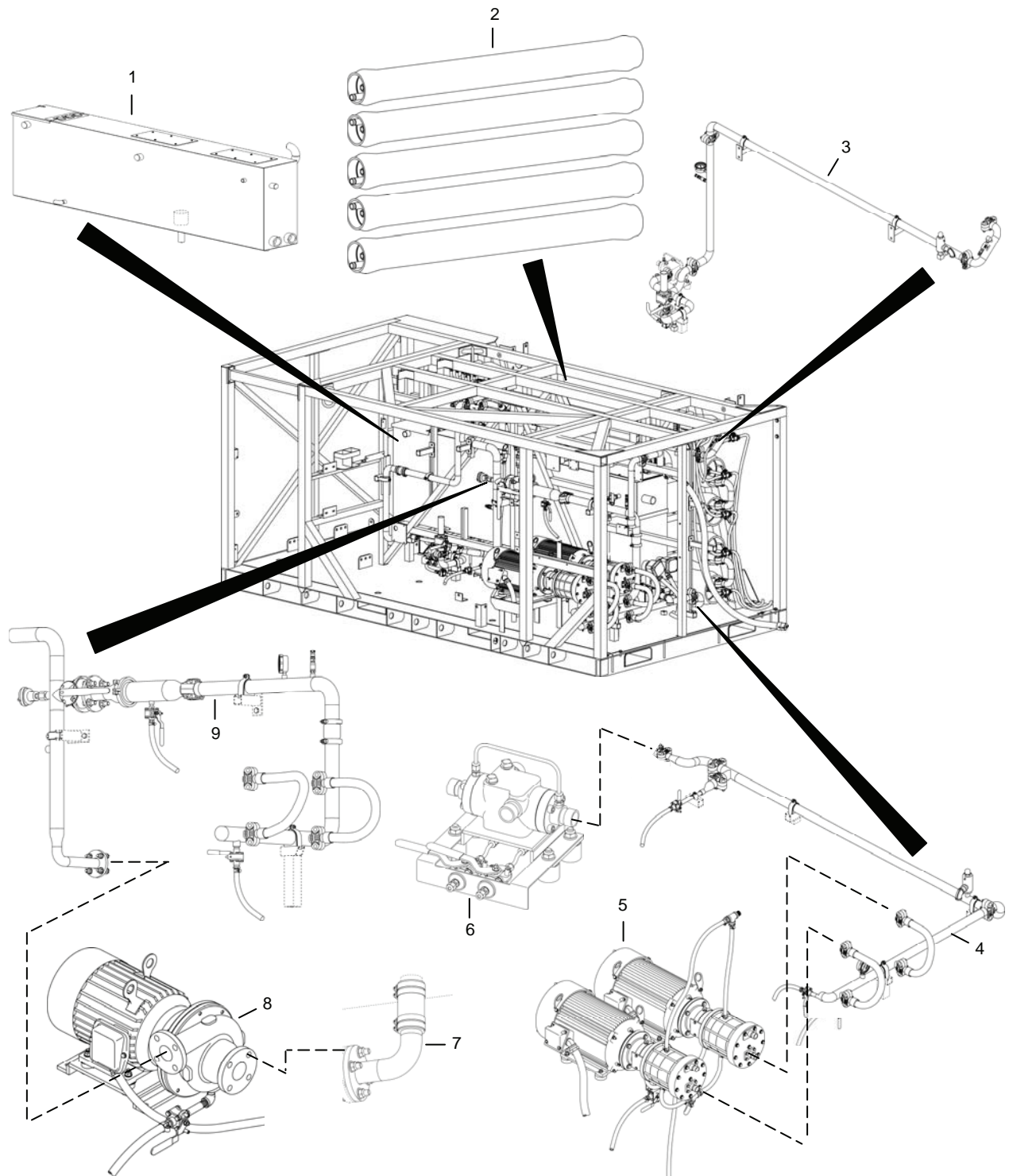
Figure 39. Reverse Osmosis System (Sheet 1 of 2).
