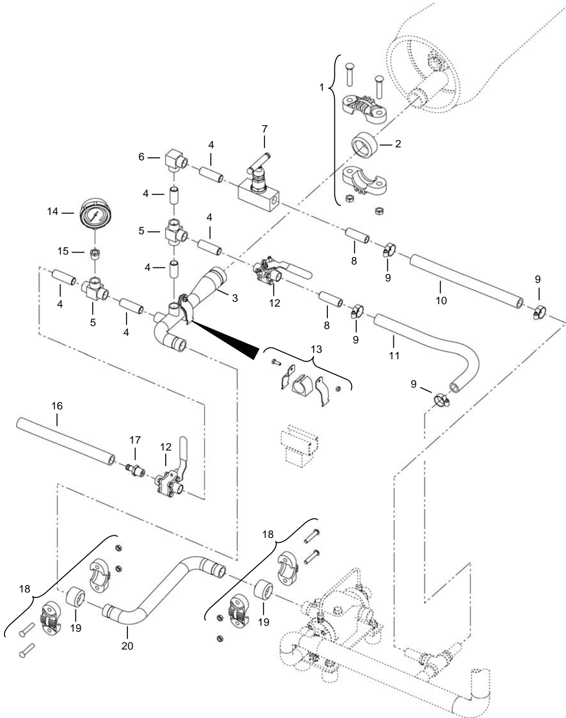
Figure 54. RO Piping Assembly R02.
