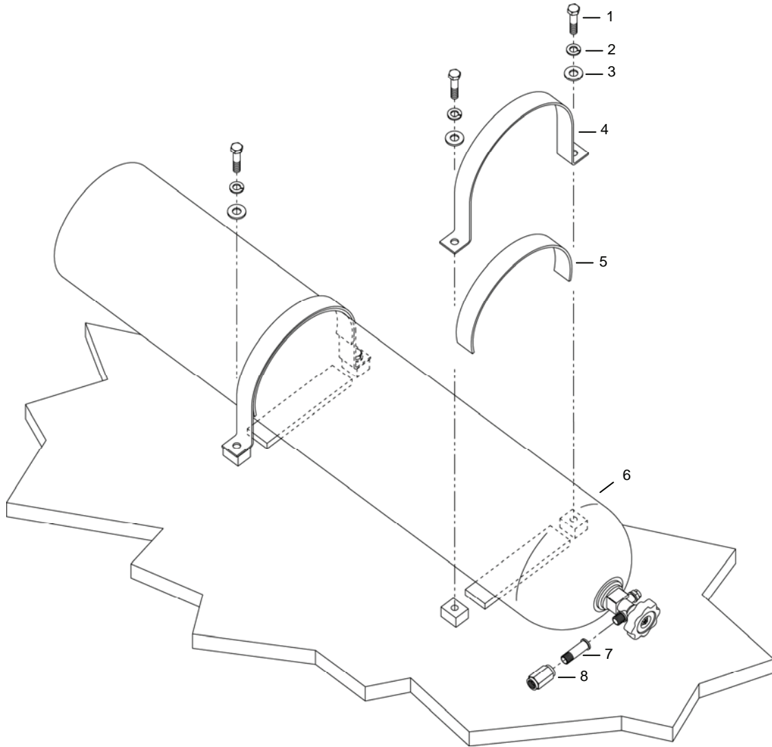
Figure 66. Air Receiver Tank R-1.
