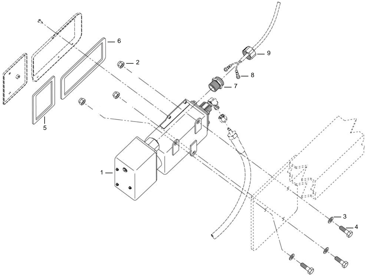
Figure 65. Pressure Switch Assembly.
