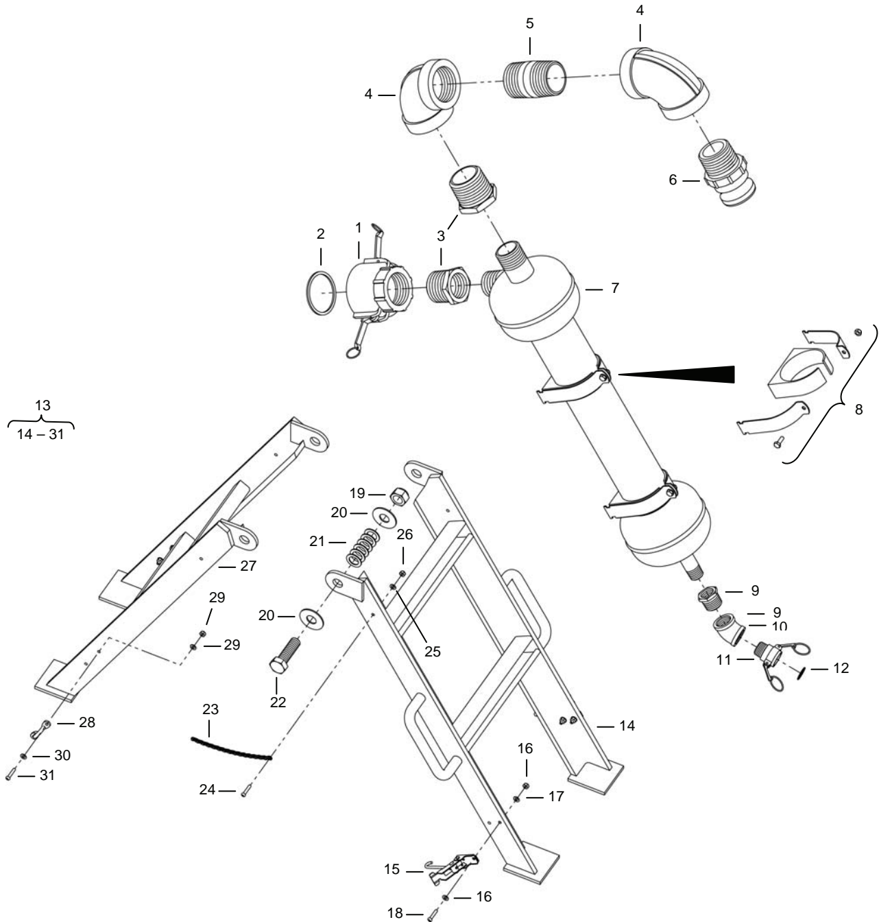
Figure 15. Cyclone Separator.
