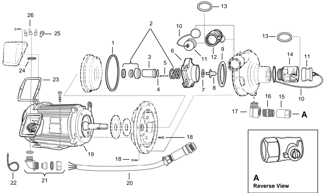
Figure 24. P-3 MF Feed Pump and Motor.
