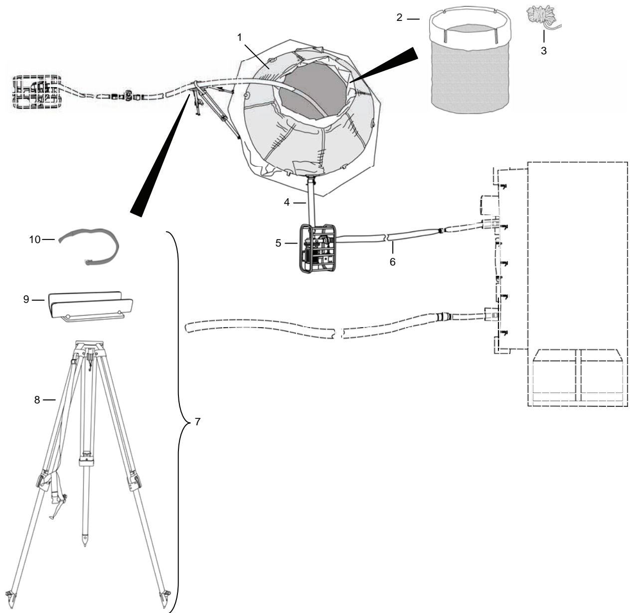
Figure 20. Micro-Filtration System – Off Skid.
