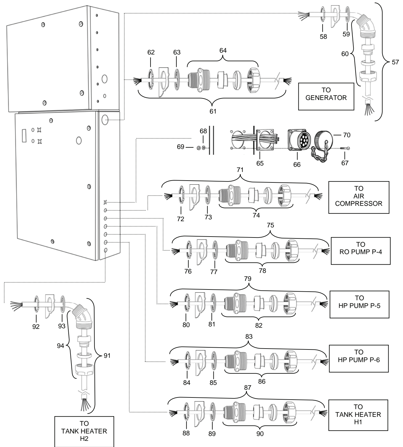
Figure 77. Power Distribution System (Sheet 3 of 3).
