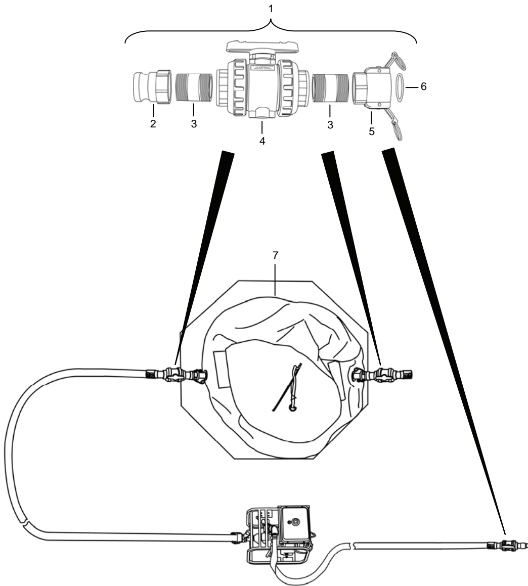
Figure 89. Cleaning Waste Storage System Adaptors.
