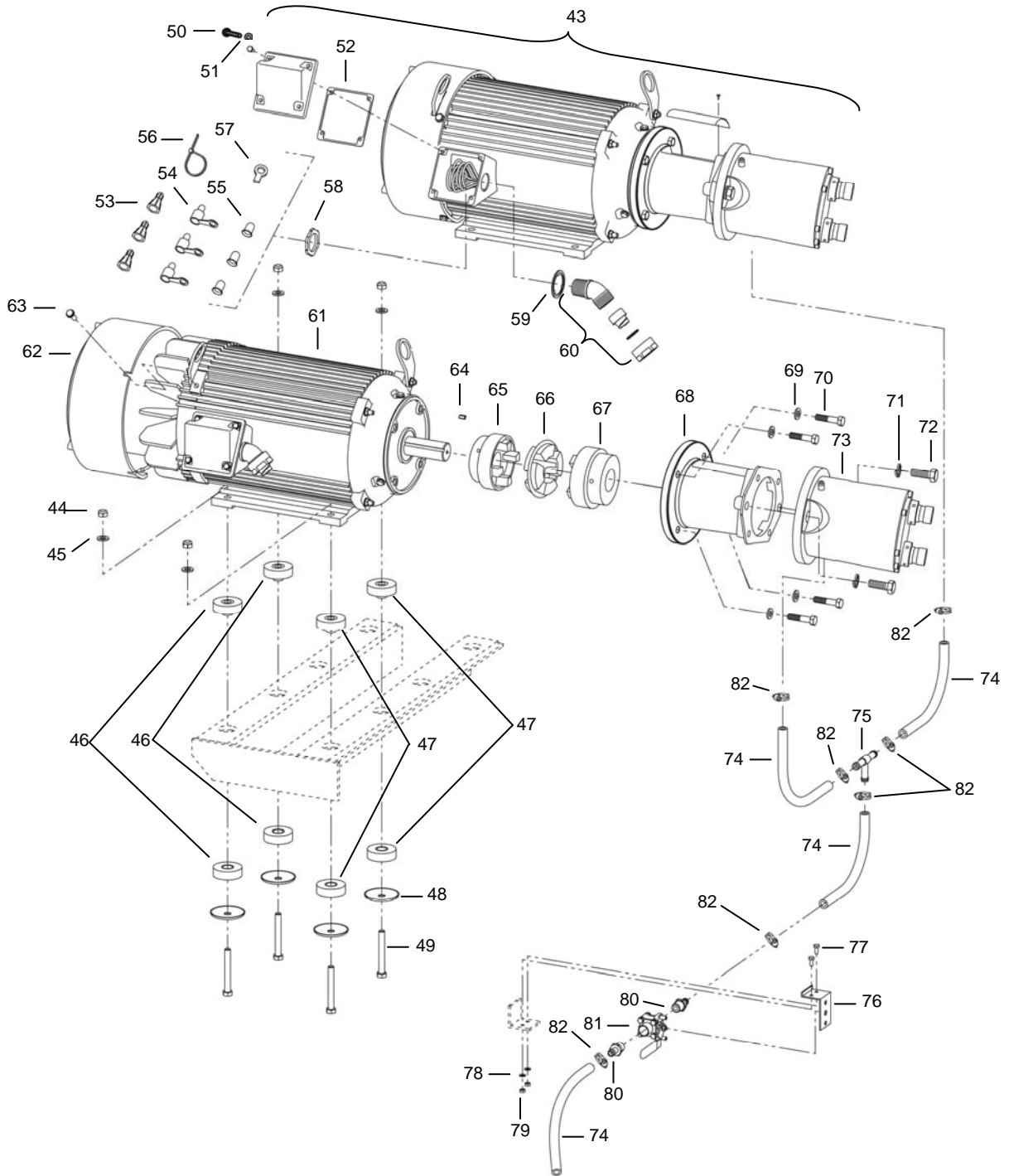
Figure 45. High-Pressure Pumps P-5 and P-6 Installation (Sheet 2 of 2).
