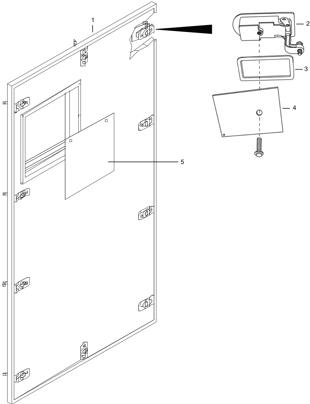
Figure 102. End Panel Assembly – Panel #1.
