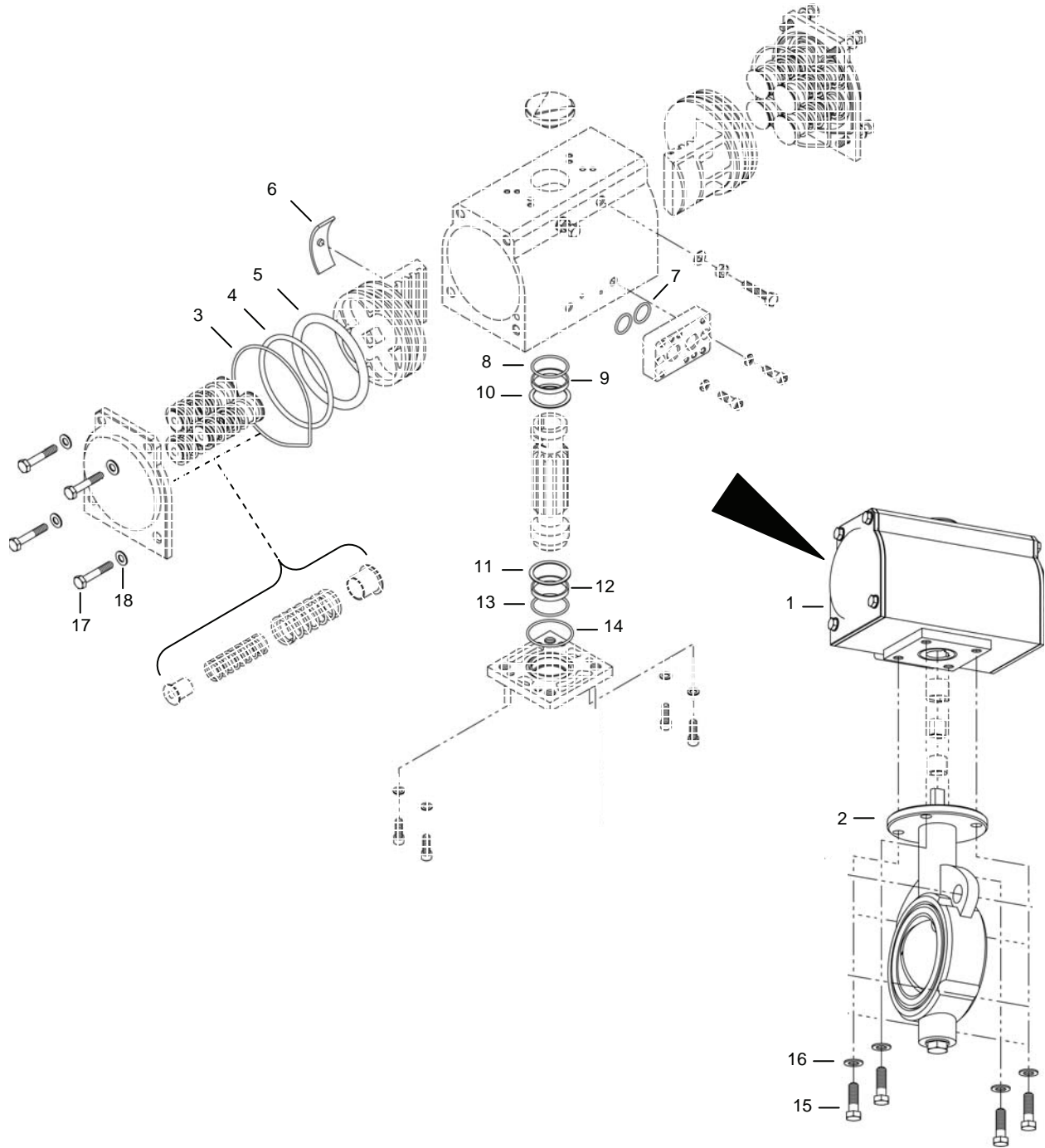
Figure 28. Valve Assembly V-111.
