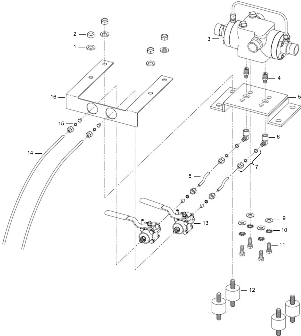
Figure 48. Turbocharger Assembly.
