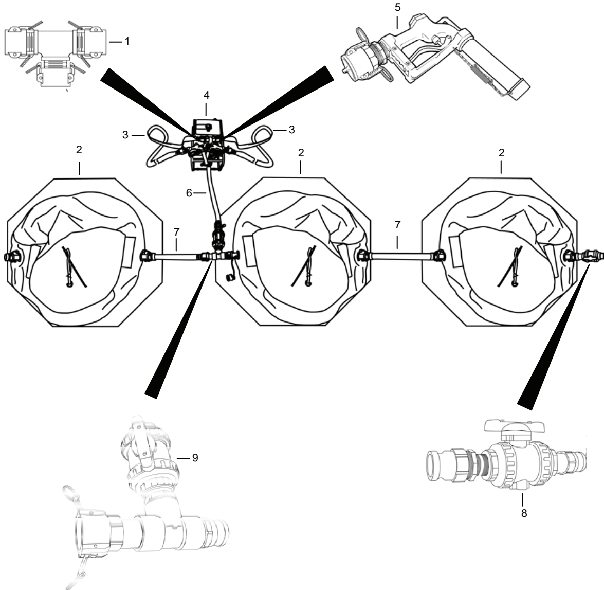
Figure 91. Extended Distribution System.
