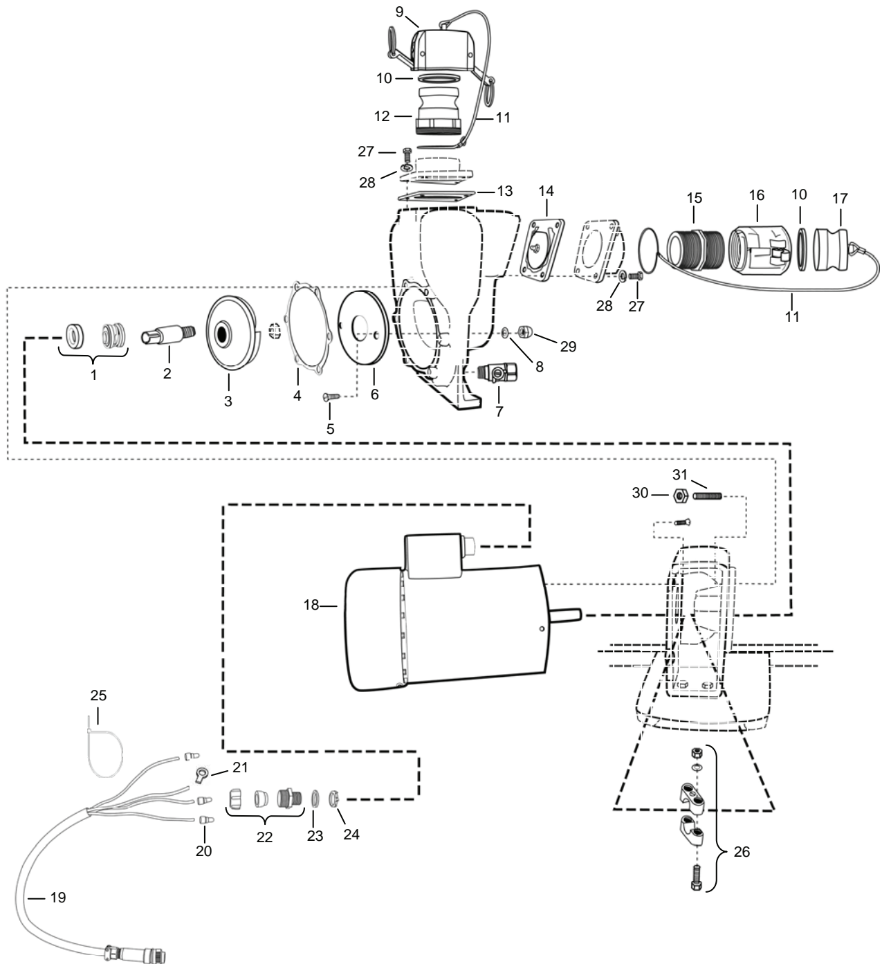
Figure 14. P-2 Centrifugal Pump.
