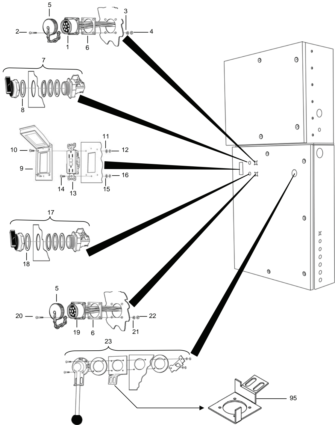
Figure 77. Power Distribution System (Sheet 1 of 3).
