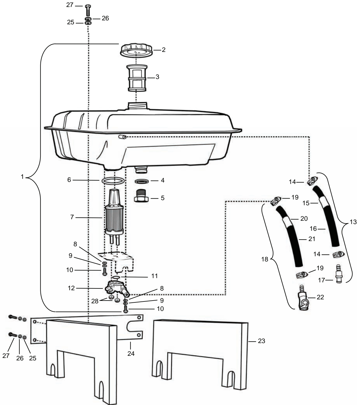
Figure 6. Fuel Tank Assembly.
