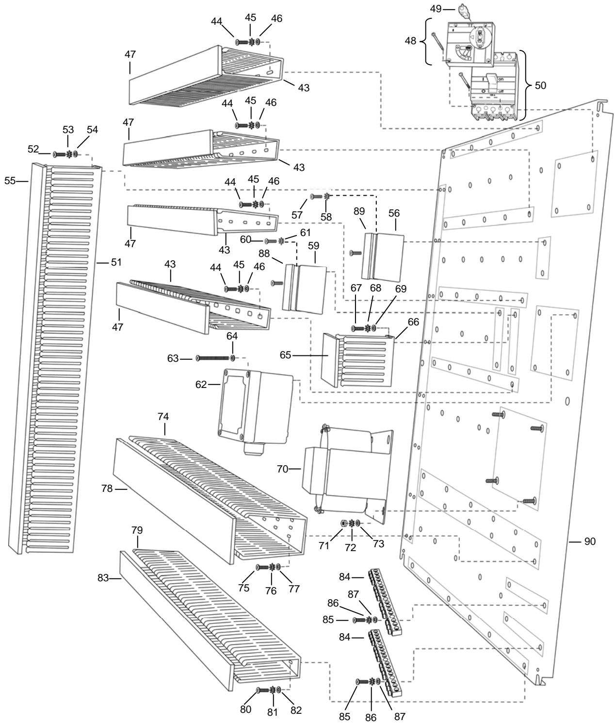
Figure 78. Power Distribution Panel (Sheet 2 of 2).
