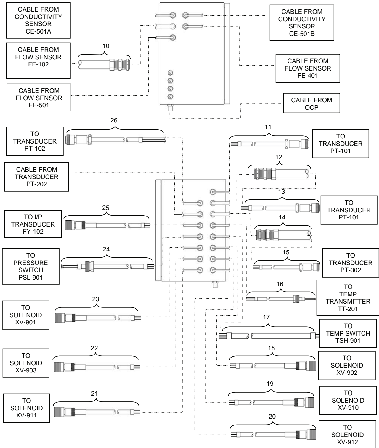
Figure 81. Instrument / Solenoid Panel (Sheet 2 of 3).
