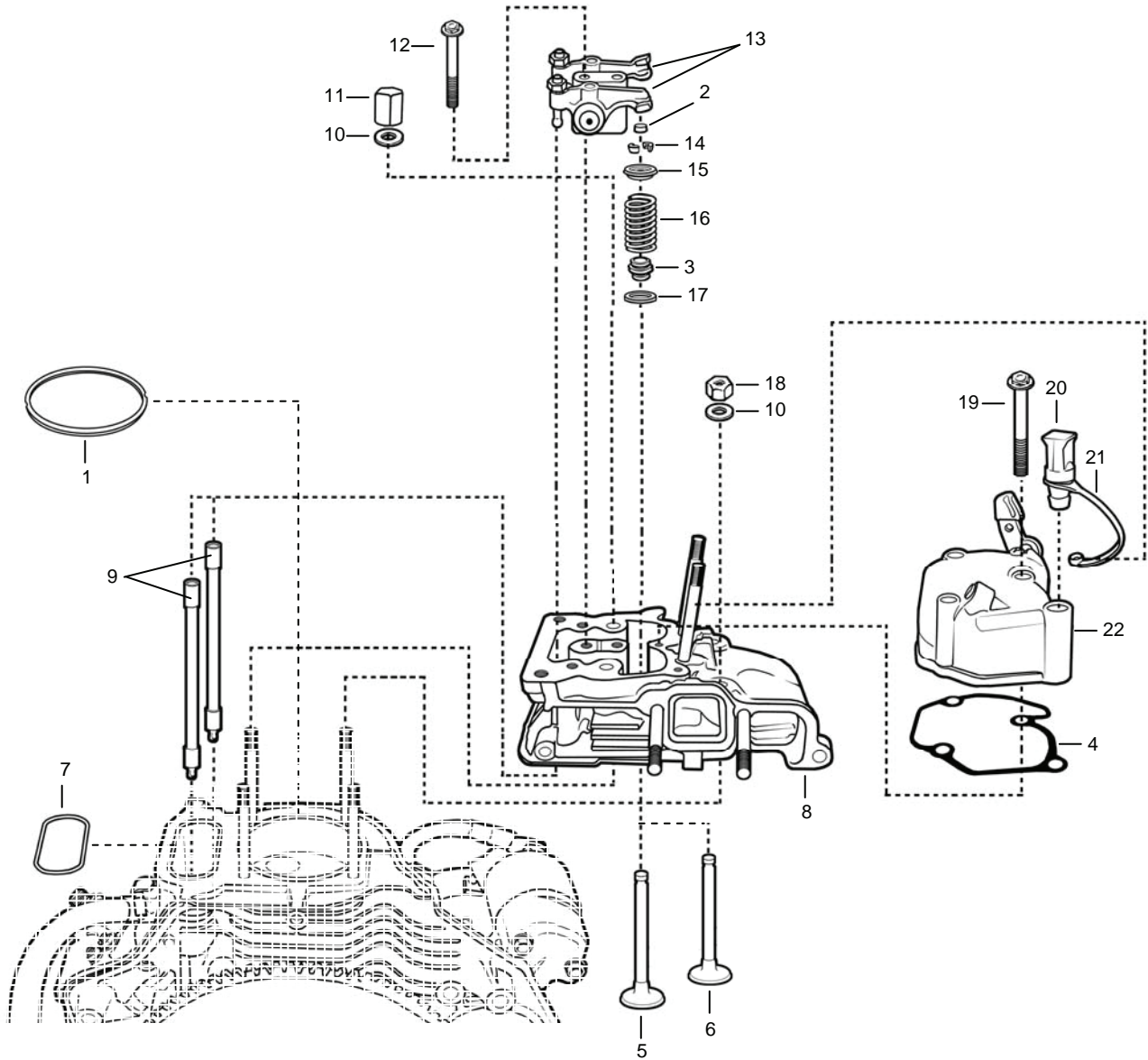
Figure 99. Cylinder Head Valves and Gaskets.
