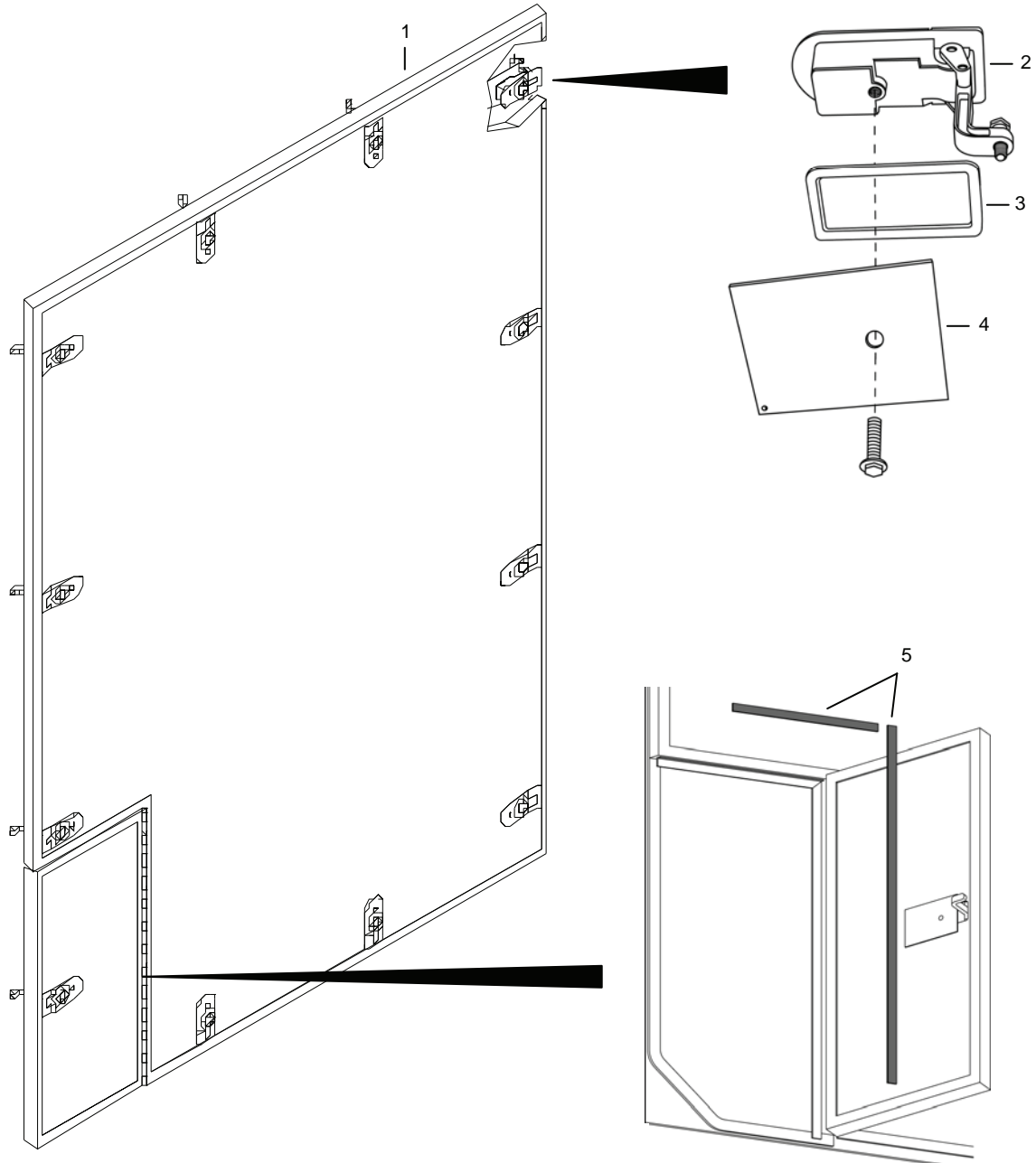
Figure 104. Panel Assembly Type I – Panel #3.
