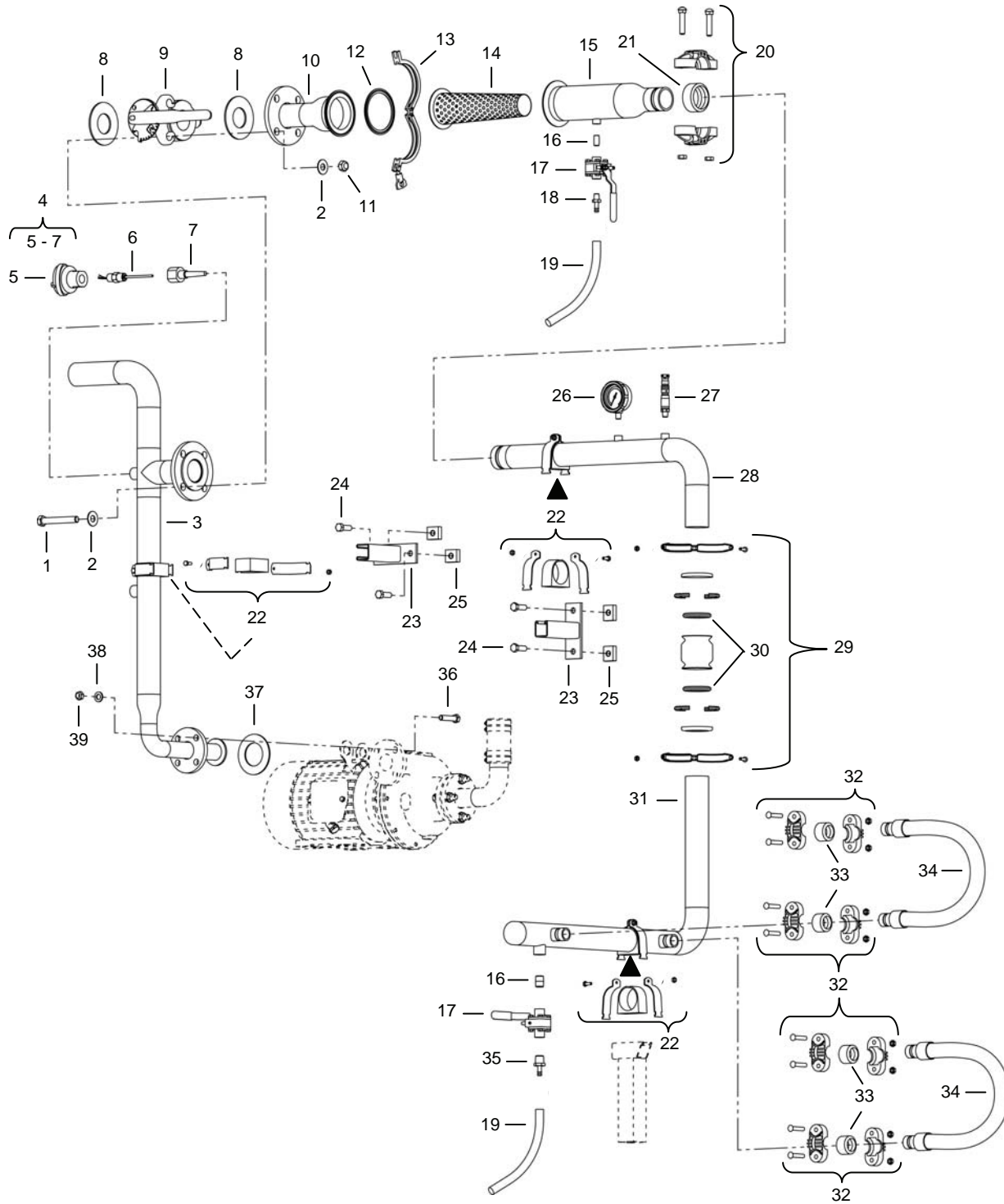
Figure 44. RO Piping Assembly M03.
