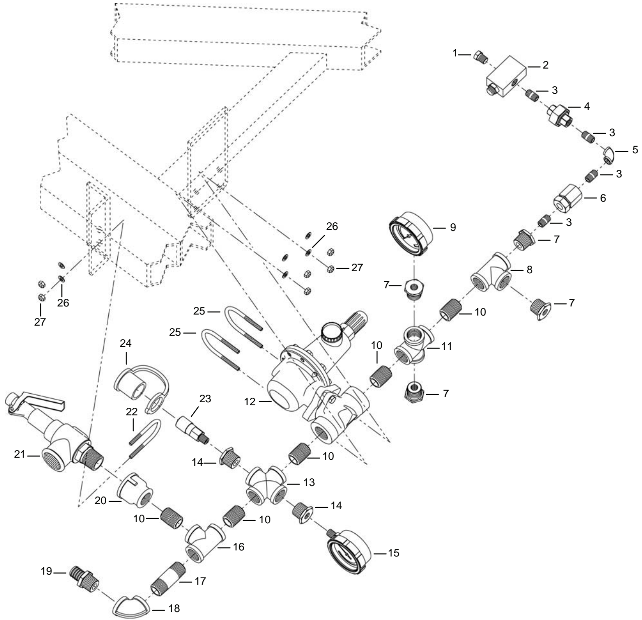
Figure 64. Air System Section 1.
