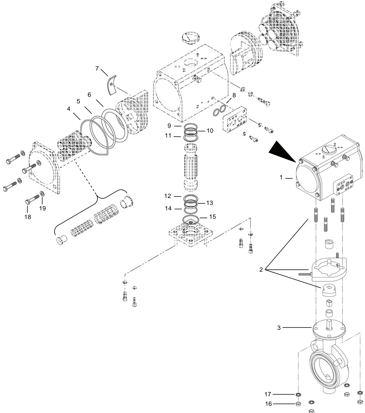
Figure 31. Valve Assembly V-113.
