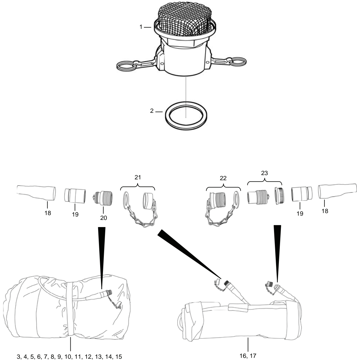
Figure 88. Ice Intake Strainer and Heating Blankets.
