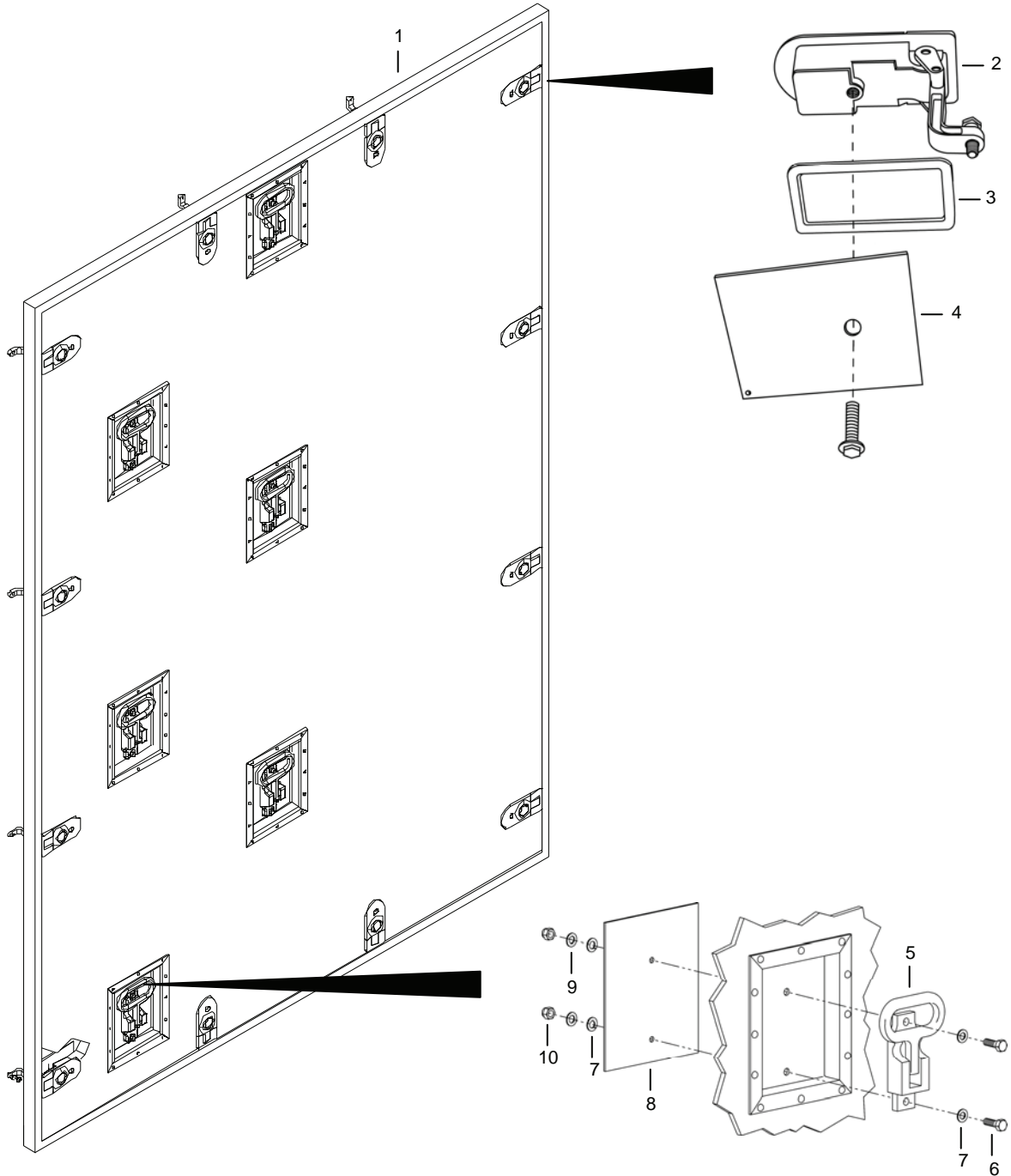
Figure 106. Panel Assembly Type III – Panel #5.
