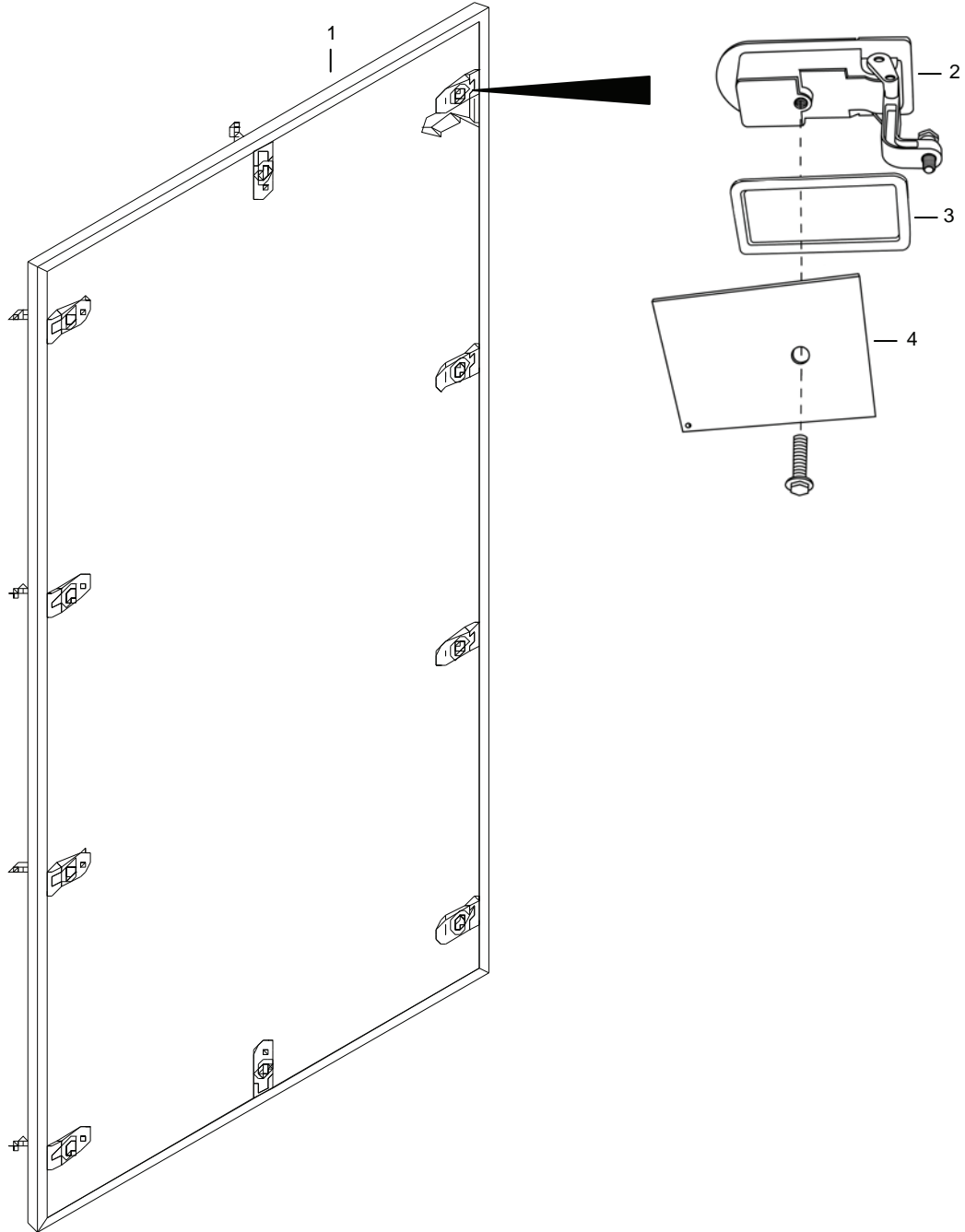
Figure 108. End Panel Assembly – Panel #7.
