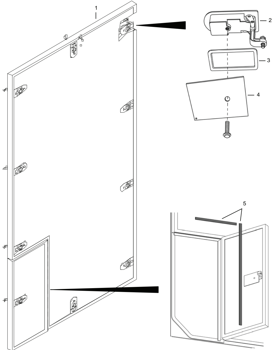
Figure 103. End Panel Assembly – Panel #2.
