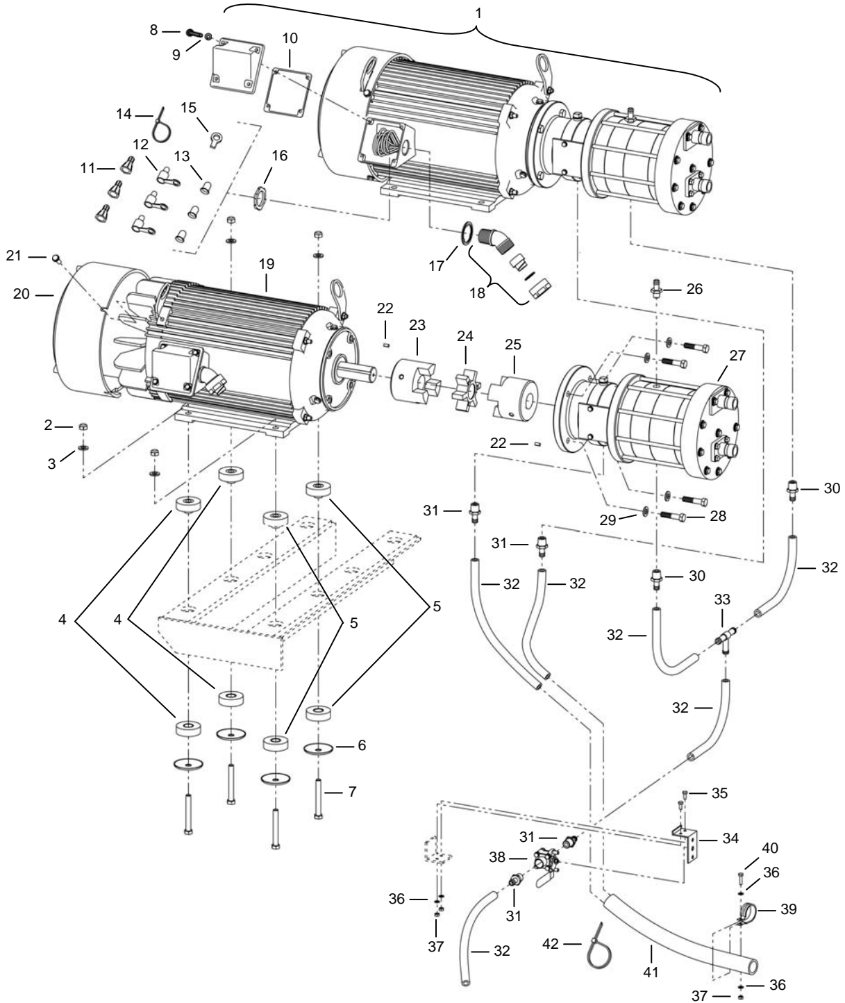
Figure 45. High-Pressure Pumps P-5 and P-6 Installation (Sheet 1 of 2).
