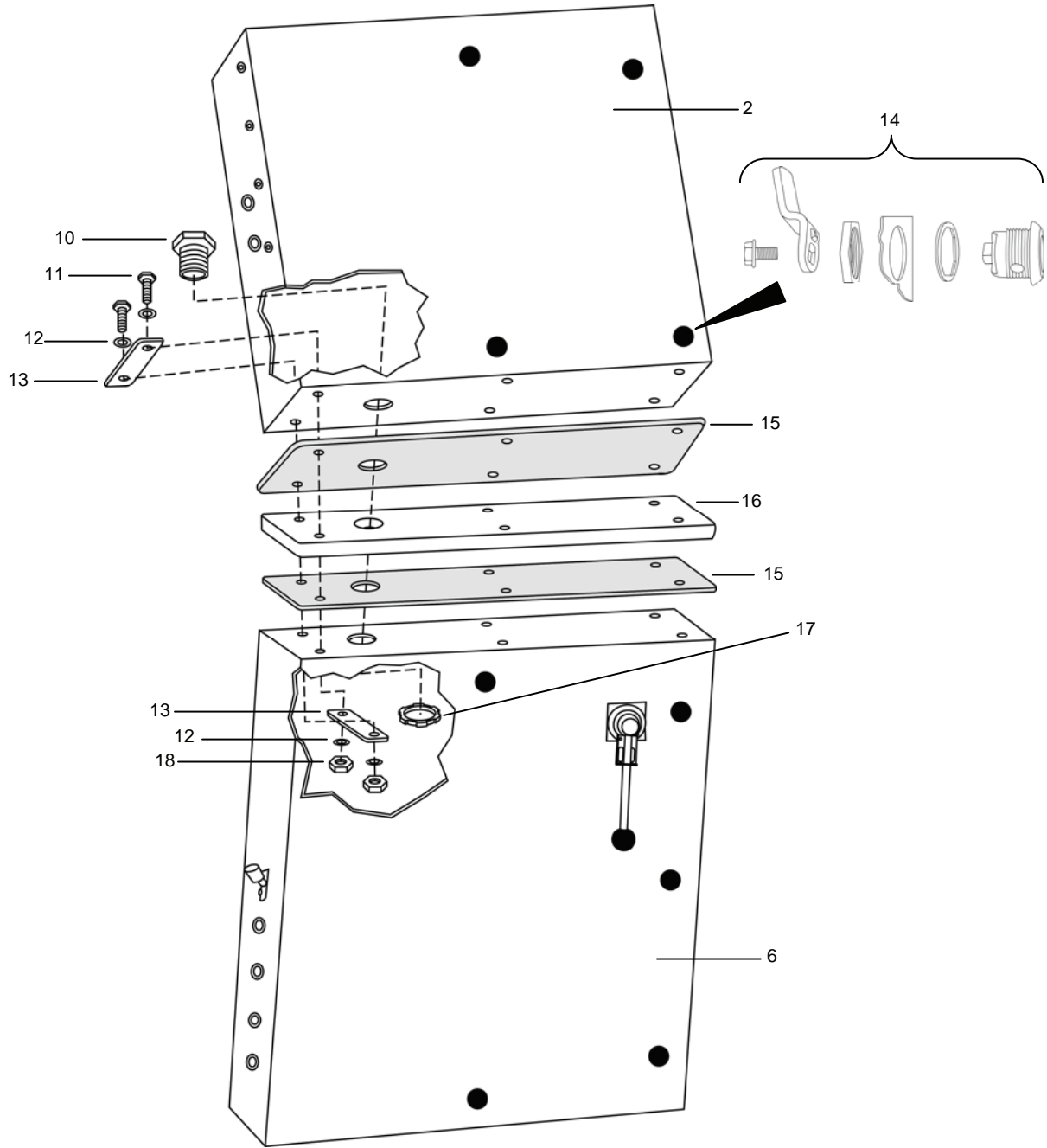
Figure 73. Operation Control and Power Distribution System (Sheet 2 of 2).
