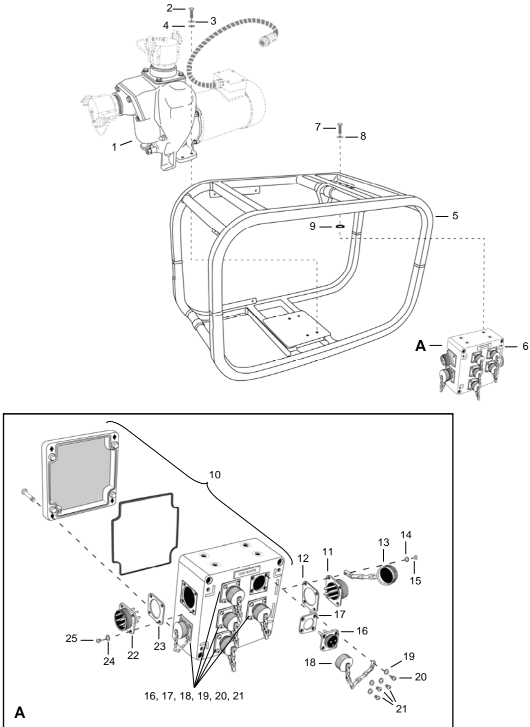
Figure 18. Electric Motor-Driven Pump Assembly P-7.
