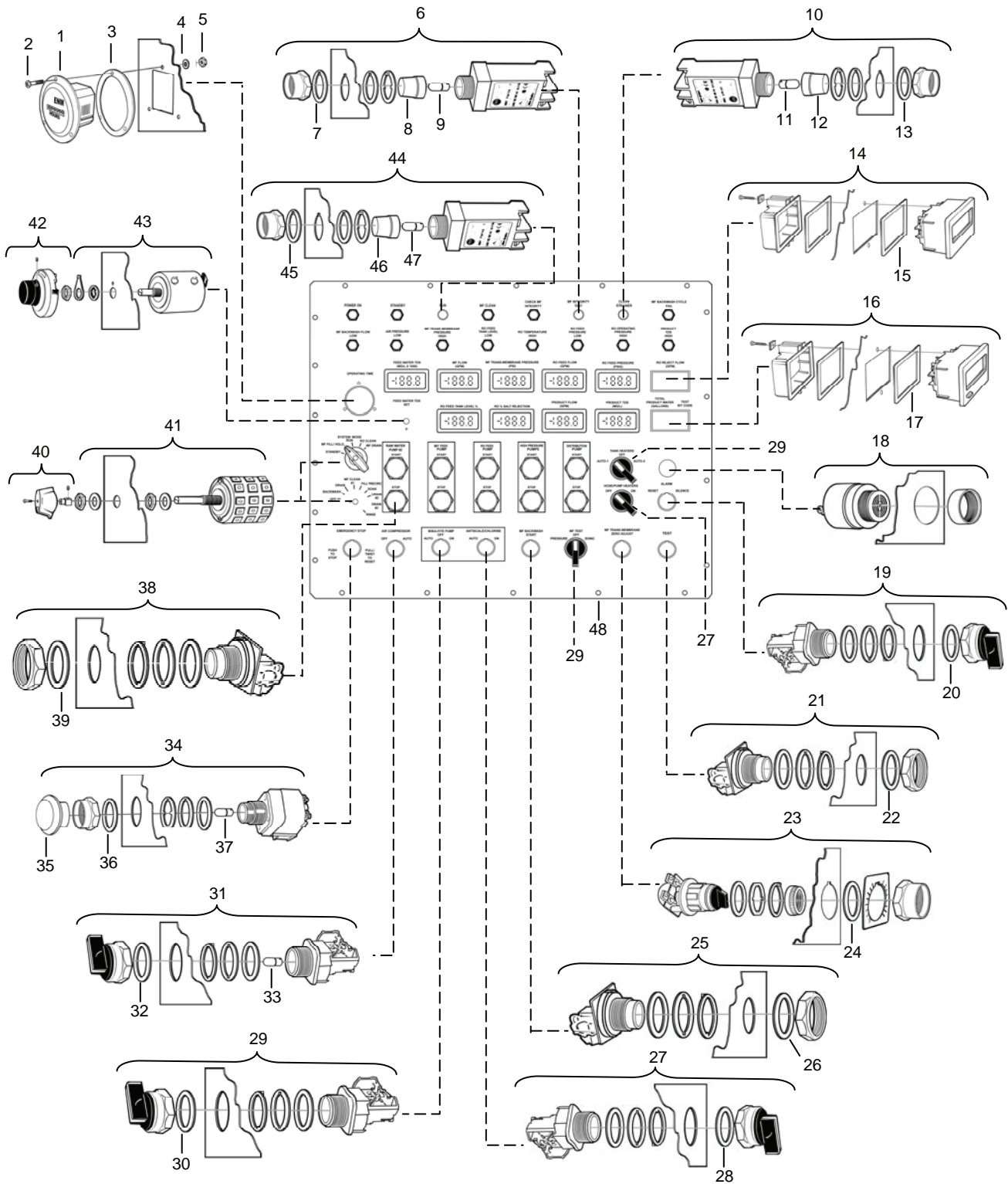
Figure 75. Top Panel Assembly.
