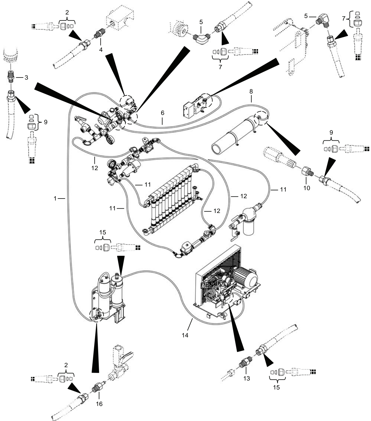
Figure 71. Air System Hoses.
