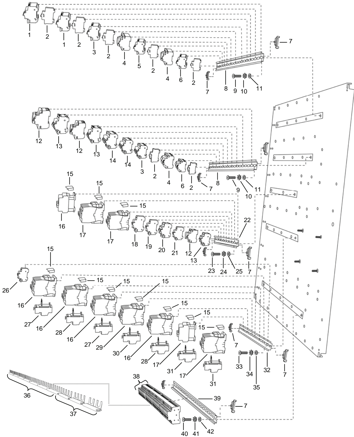
Figure 78. Power Distribution Panel (Sheet 1 of 2).
