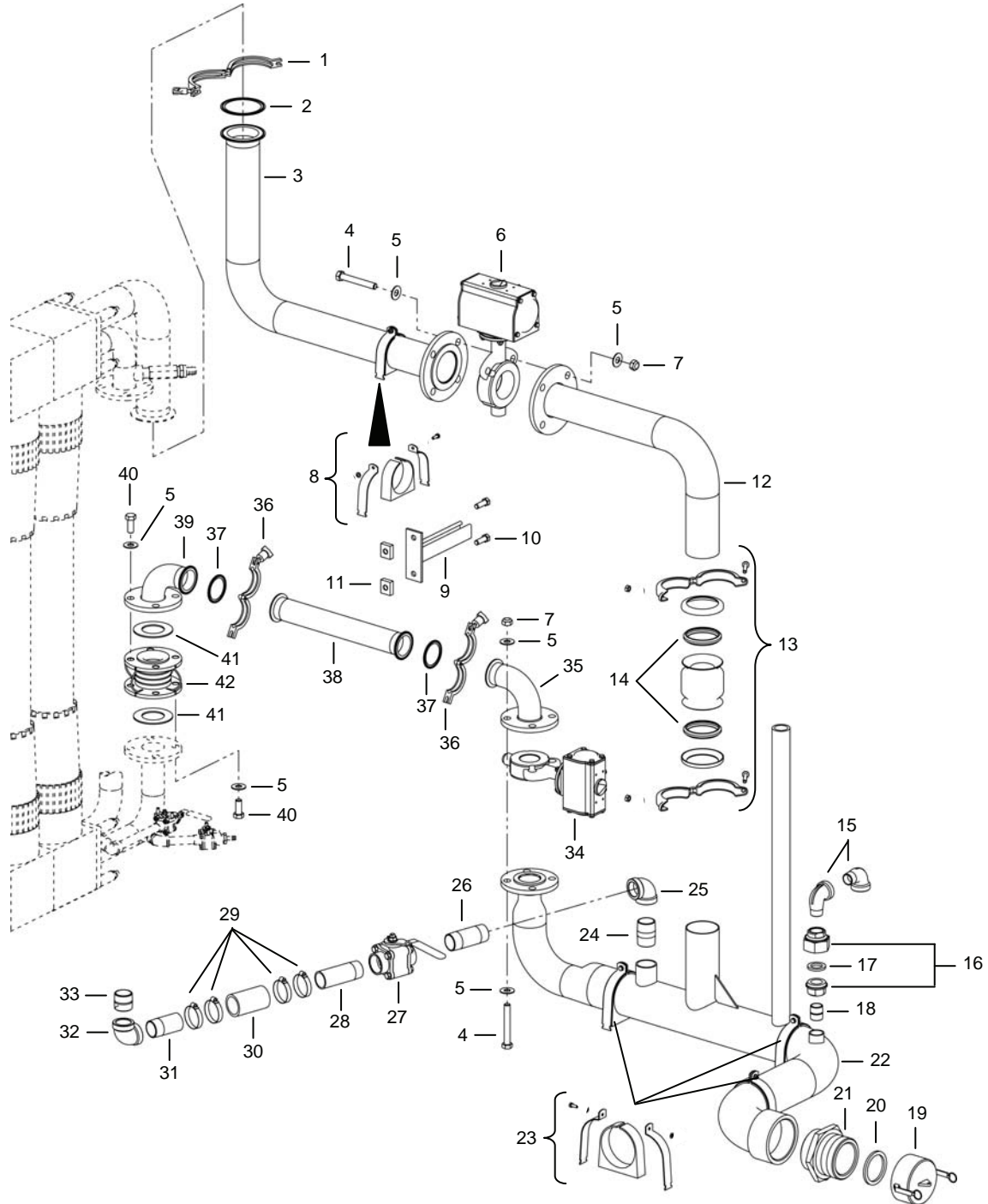
Figure 37. MF Piping Assembly R01.
