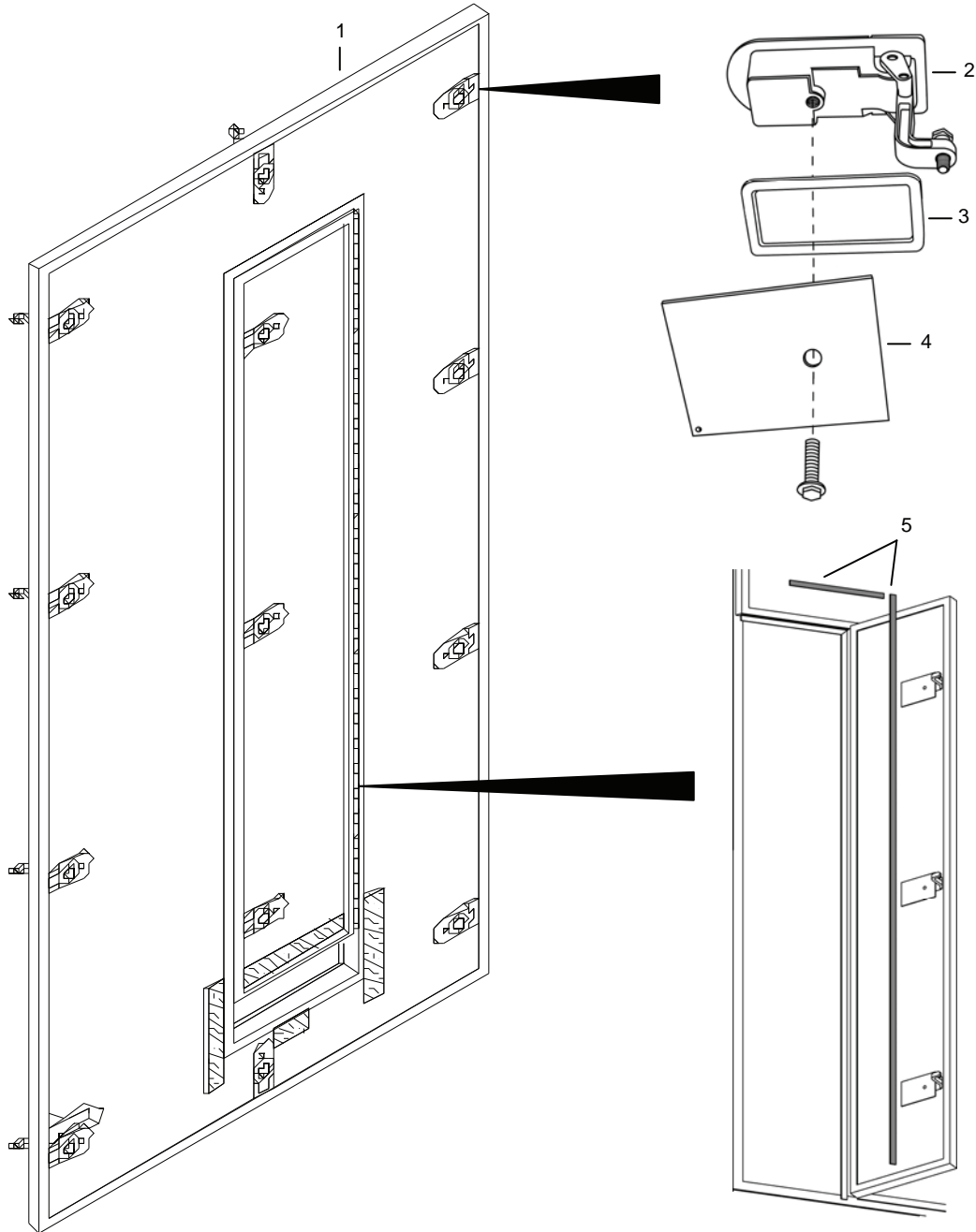
Figure 107. End Panel Assembly – Panel #6.
