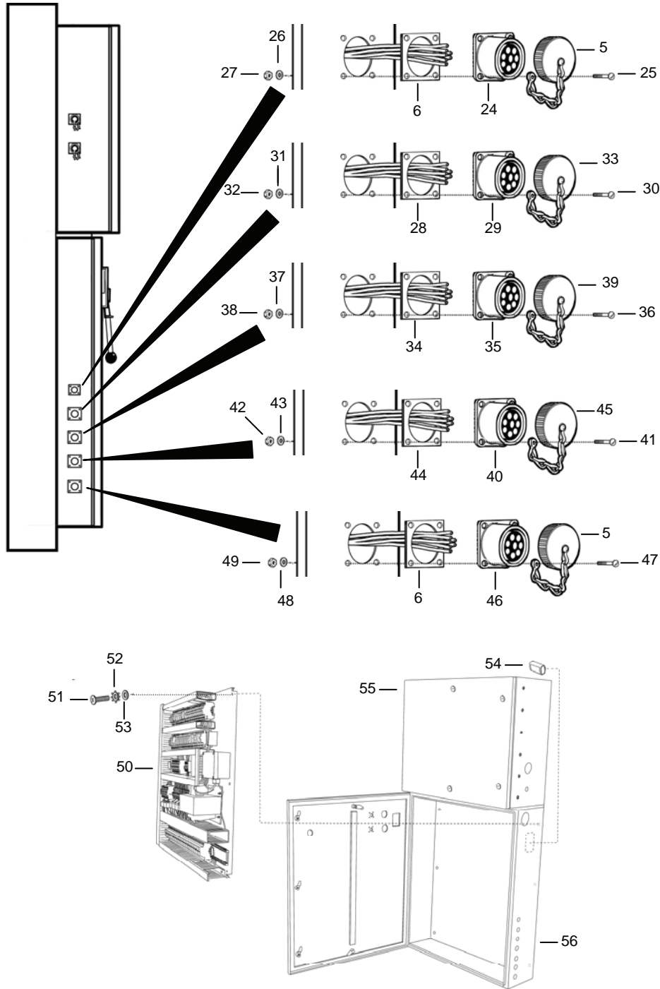
Figure 77. Power Distribution System (Sheet 2 of 3).
