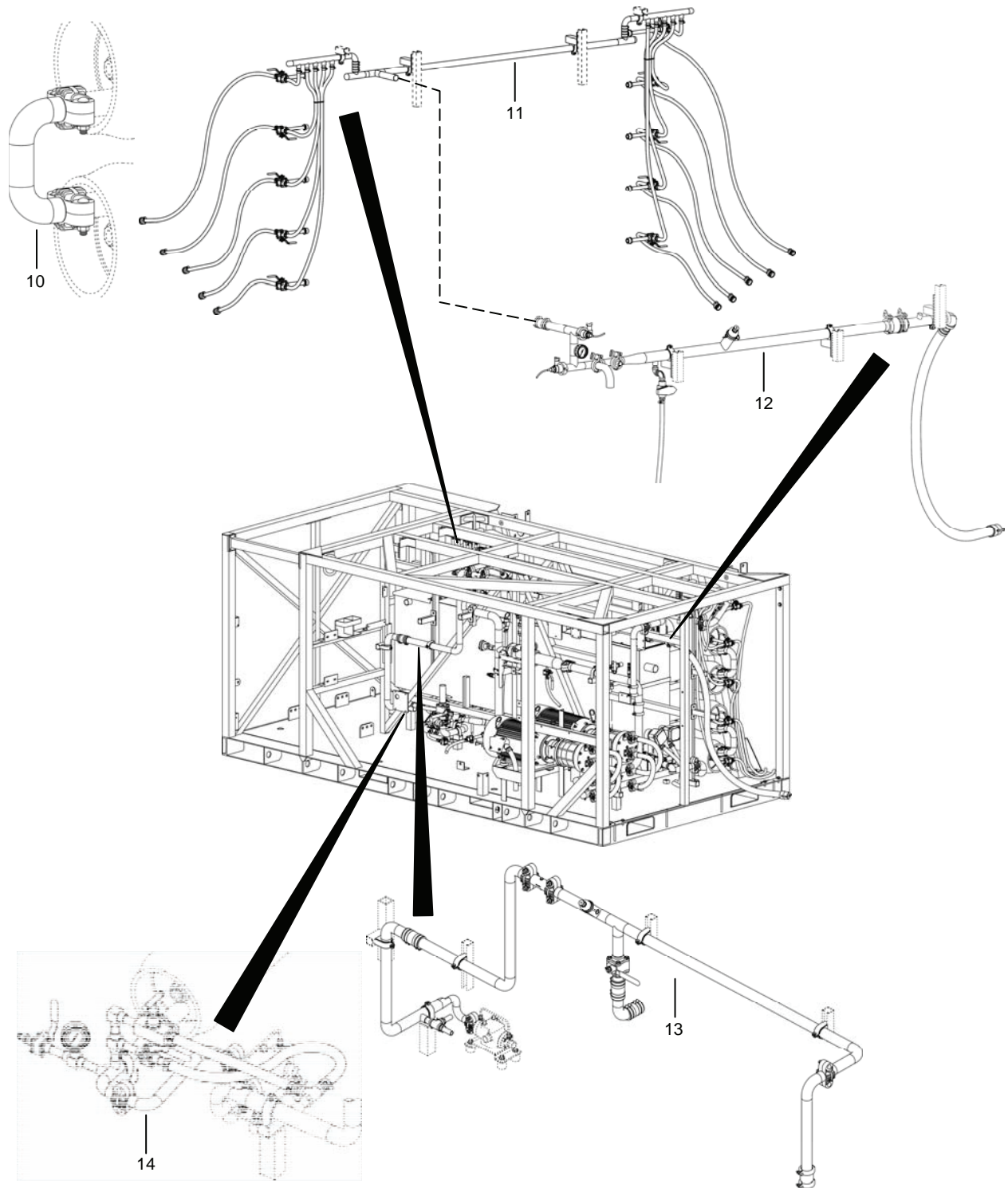
Figure 39. Reverse Osmosis System (Sheet 2 of 2).
