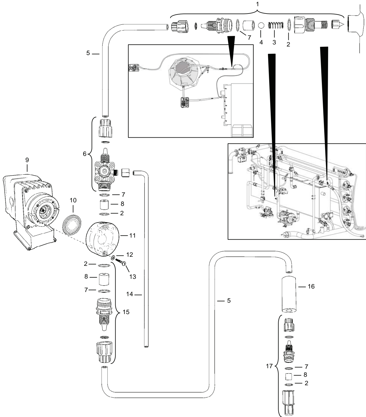
Figure 59. Chemical Injection Pump, Valves, and Injectors (Typical 1 of 3).
