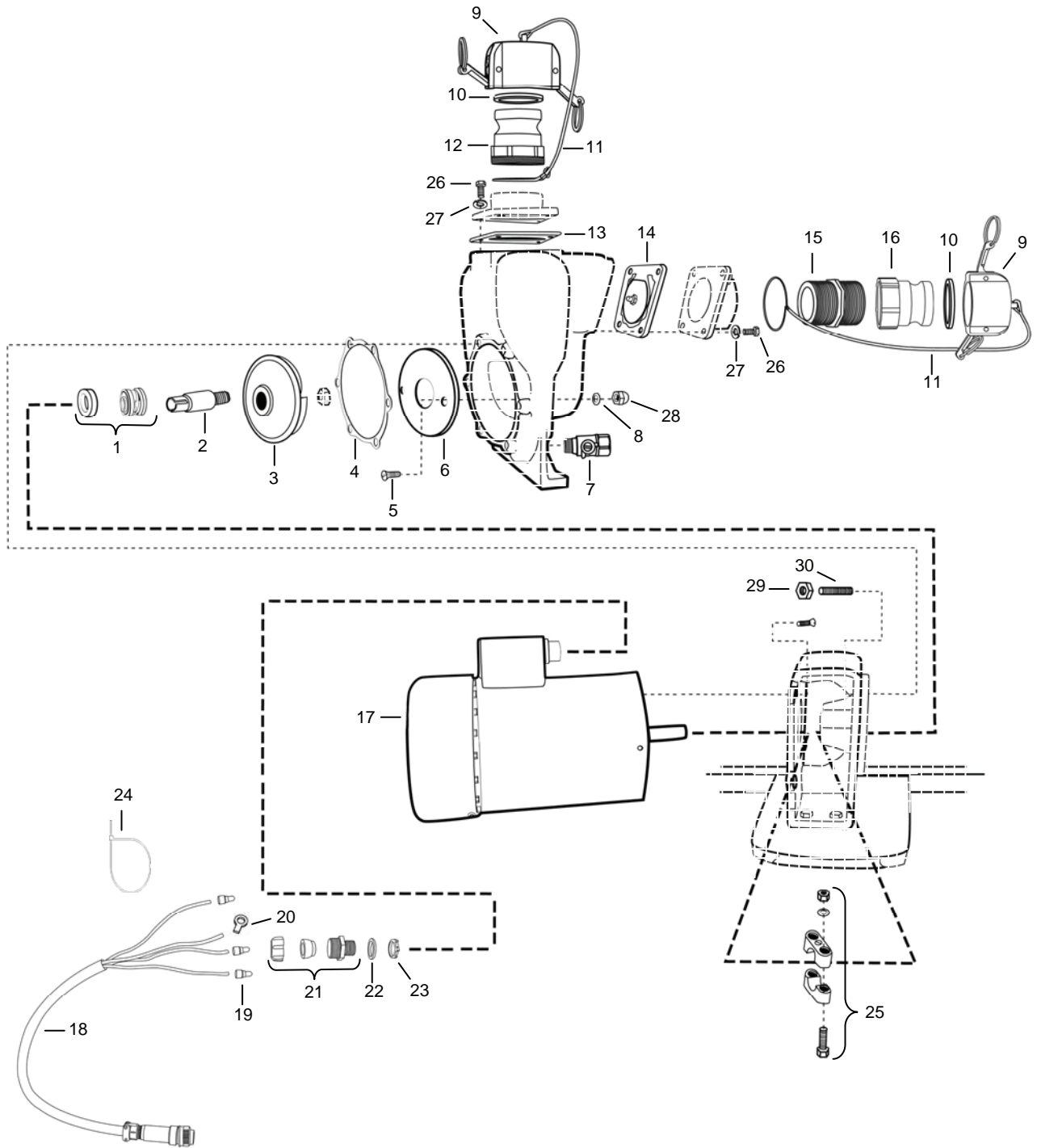
Figure 19. P-7 Centrifugal Pump.
